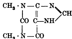
Theophylline
