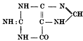
Guanine
