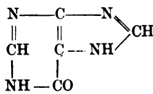
Hypoxanthine
