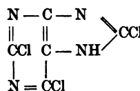
Trichloropurine
