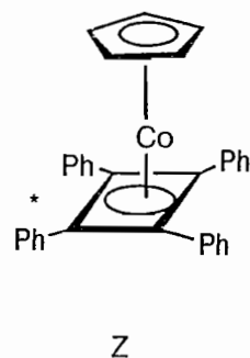
[(\text{C}_6\text{H}_5)_4\text{C}_4]\text{CoCp}
