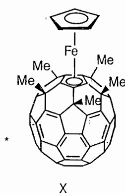
(\text{C}_{60}\text{Me}_5)\text{FeCp}
