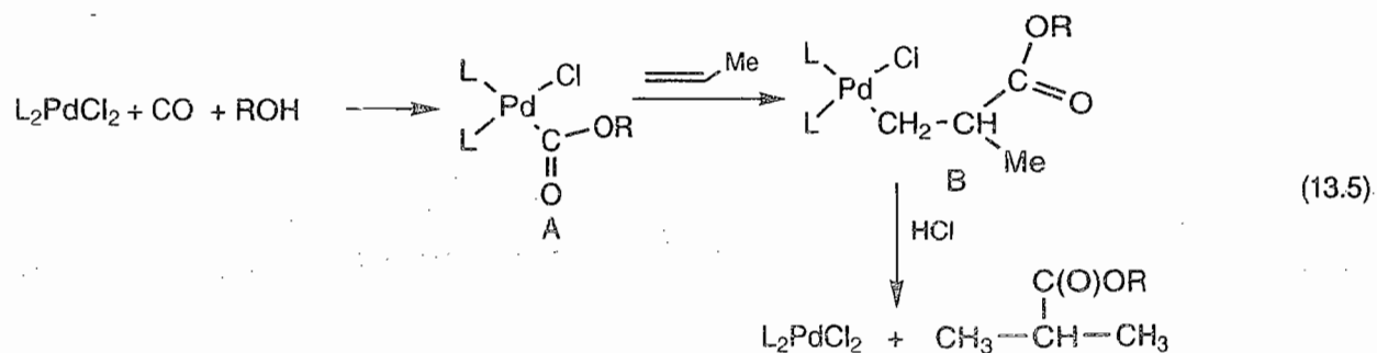
Fig. 13.3 Catalytic cycle for carboalkoxylation of olefins
