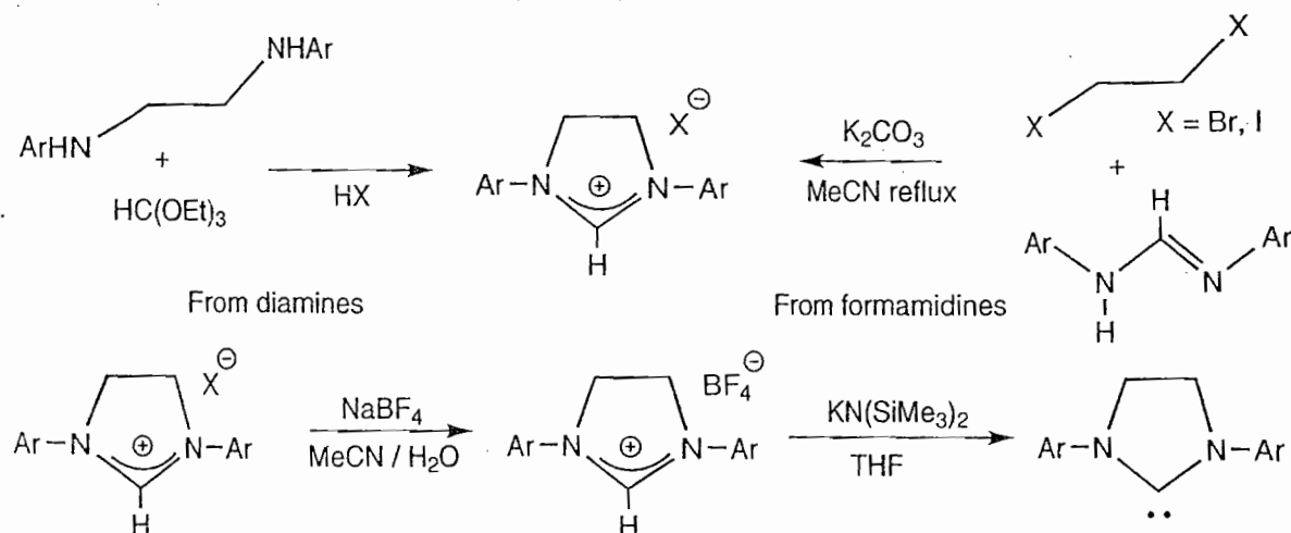
Fig. 4.4 Synthesis of NHCs with saturated carbene rings
