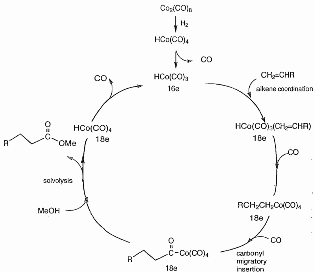
Fig. 13.3 Catalytic cycle for carboalkoxylation of olefins
