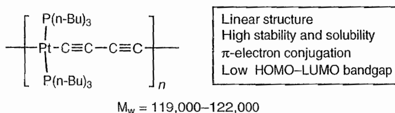
Fig. 19.1 Properties of Hagihara's first platinum based rigid rod polyyne
