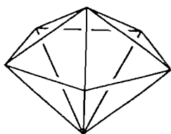
pentagonal bipyramid
