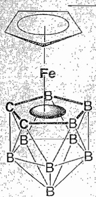
[1-Cp,1,2,3-FeC 2 B 9 H 11 ]
