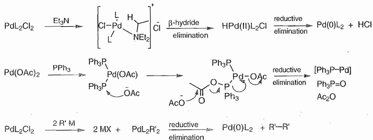
Scheme 16.1 Possible ways of generation of Pd(0) species in the reaction medium
