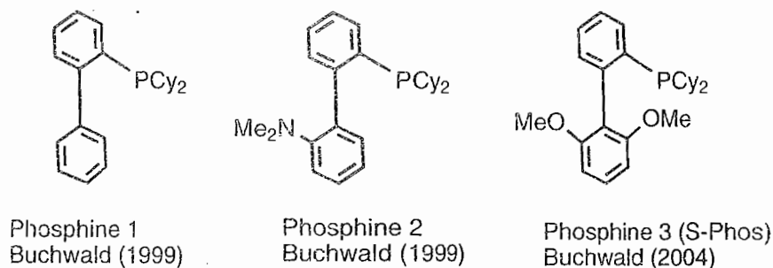
Fig. 16.1 Sterically hindered and electron rich Buchwald phosphines
