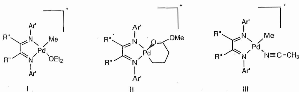
Fig. 17.15 Pd catalysts for copolymerisation of ethylene with polar monomers
