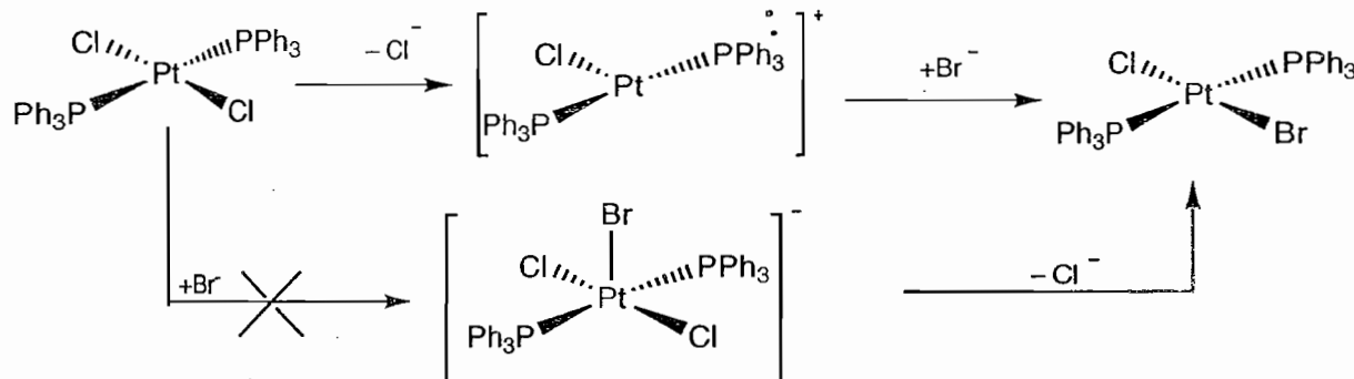
Scheme 9.1 Substitution reactions on square planar platinum complexes
