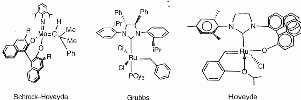
Scheme 15.23 Chiral olefin metathesis catalysts
