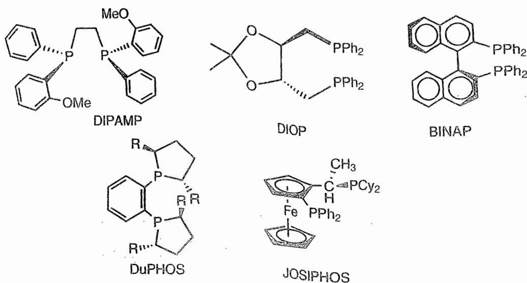
Fig. 12.7 Chiral diphosphines used in asymmetric hydrogenations
