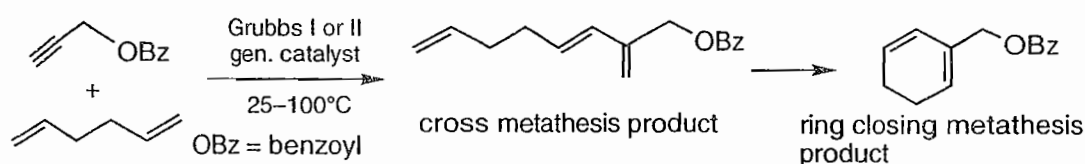
Scheme 15.16 Tandem dienyne cross metathesis/ ring closing metathesis
