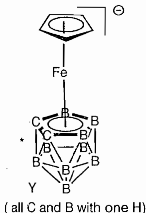
[(7, 8\text{-C}_2\text{B}_9\text{H}_{11})\text{FeCp}]^-
