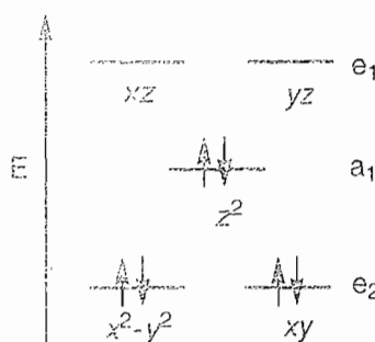
Fig. 18.1 Frontier orbital electronic configuration of ferrocene
