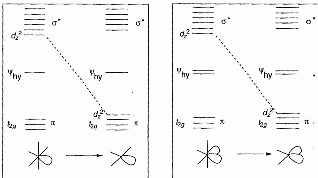
Fig. 10.12 Isolobal relationship between the 18e octahedral and 16e square planar fragments
