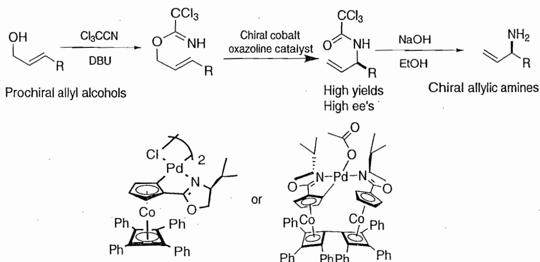
Fig. 7.5 Overman–Claisen rearrangement catalysed by chiral monomeric and dimeric cobalt oxazoline palladacycles
