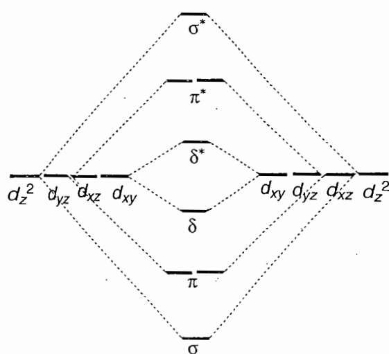
Fig. 10.3 Qualitative MO picture indicating relative energies of orbitals involved in metal–metal multiple bonding
