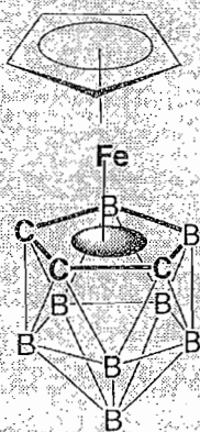
[1-Cp,1,2,3-FeC 2 B 9 H 11 ]
