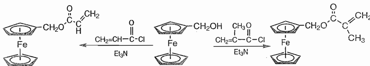
Scheme 19.2 Synthesis of acrylic and methacrylic ferrocene derived monomers
