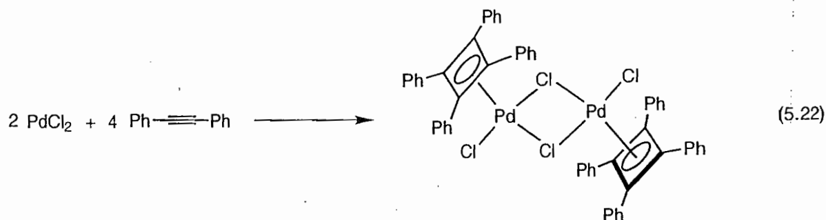
Fig. 5.6 Dimerisation of alkynes to cyclobutadiene with CpCo based reagents
