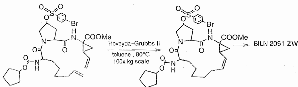
Scheme 15.24 Ring closing metathesis step in the synthesis of BILN 2061 ZW
