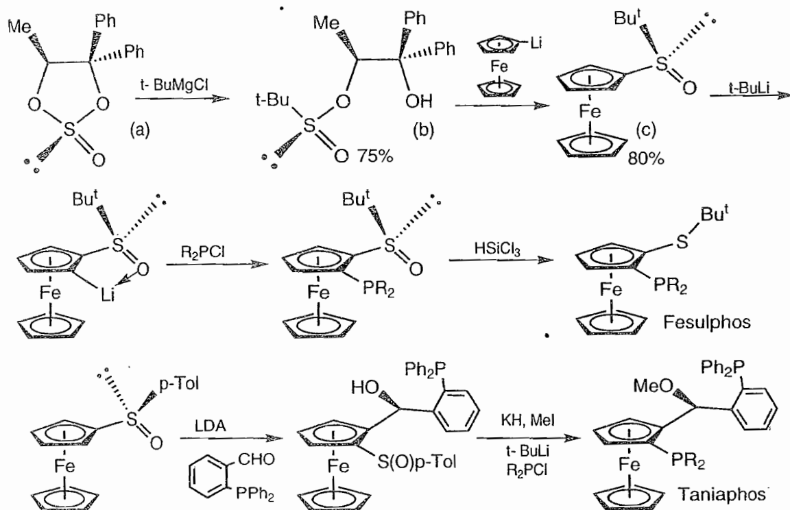
Scheme 18.13 Synthesis of Fesulphos and Taniaphos planar chiral ligands
