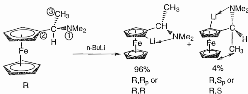
Fig. 18.6 Method of assigning planar chirality descriptor along with central chirality
