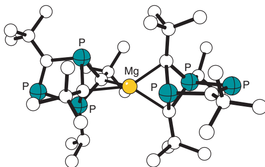
Figure 50 The structure of the magnesium–phosphorus cage compound 101 .
