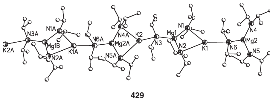
Figure 37 The structure of [(iPr) 2 N 3 KMg] ∞ 429 . Hydrogen atoms have been omitted for clarity. Agostic interactions between potassium and methyl groups are not shown.
