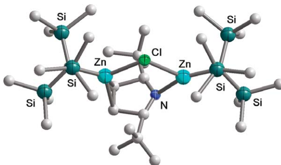
Figure 41 Solid-state structure and partial labeling scheme of 77 .
