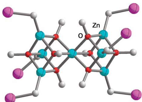
Figure 60 Solid-state structure and partial labeling scheme of 128 .
