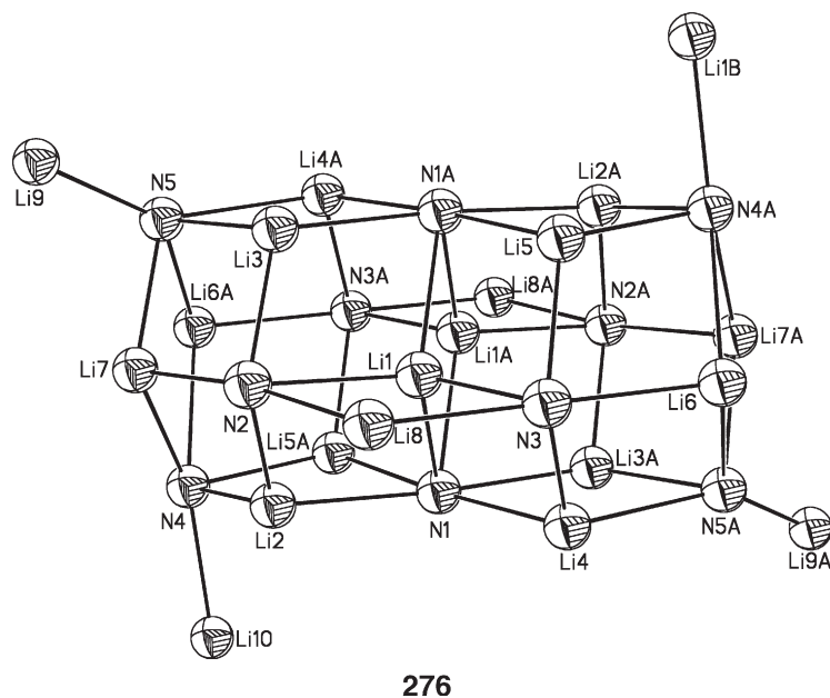
Figure 20 Core of the molecular structure of the dilithiated amide 276 .
