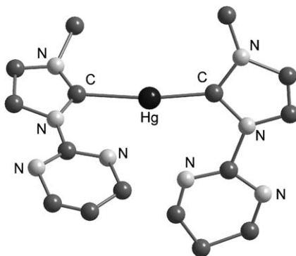
Figure 4 Structure of 153 . Hydrogen atoms omitted for clarity.
