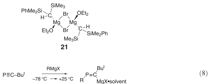
in Et 2 O and Li followed by treatment with magnesium metal. 110 The regio- and stereoselective addition of a series of Grignard reagents across Bu t C≡P yields 2-phospha-1-vinylmagnesium halide species, [MgX(RP=C(Bu t )(OEt 2 )) 2 ] (R = Et, Mes, Cy, cyclopentyl; 111 R = Pr i or Bu t ; 112 X = Cl or Br), in high yield (Equation (8)).
