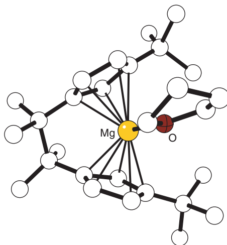
Figure 31 The structure of the ansa -magnesocene (\text{CH}_3)_3\text{C}-\text{C}_5\text{H}_4-\text{O}-\text{C}_5\text{H}_4-\text{Mg}(\text{THF}) 60 .
