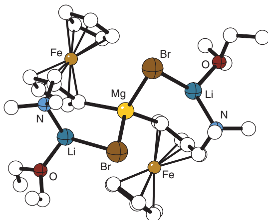
Figure 20 Structure of the magnesate complex \text{Li}_2\text{Mg}(\text{FcN})_2\text{Br}_2(\text{OEt})_2 44 .
