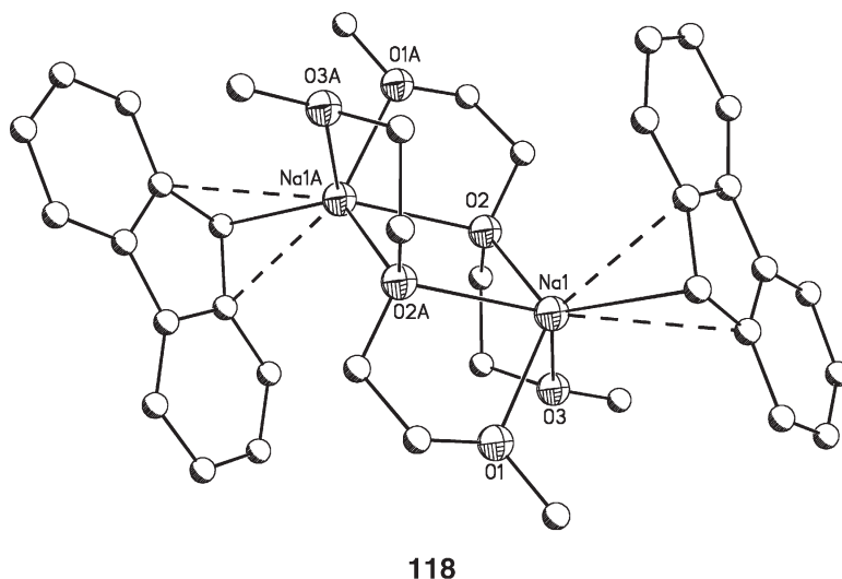
Figure 12 The structure of [\text{FNa}(\text{diglyme})]_2 118 . Hydrogen atoms have been omitted for clarity.
