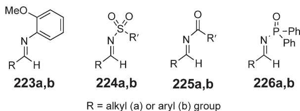
Figure 84 Imine derivatives alkylated by diorganozinc reagents.
