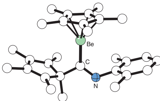
Figure 7 The structure of the iminoacylberyllium complex (\text{C}_5\text{Me}_5)\text{BeC}(=\text{NXyl})(\text{C}_5\text{Me}_5) 15 .
