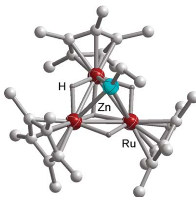
Figure 79 Solid-state structure and partial labeling scheme of 168 .
