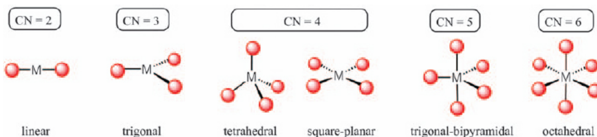
Figure 2.16 Relationship between coordination number (CN) and geometrical structure.
