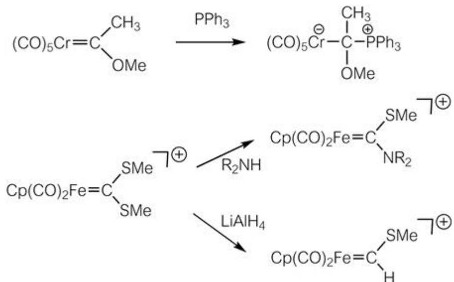
Figure 5.10 Reactions resulting from electrophilicity of Fischer carbene complexes.
