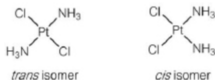
Figure 1.3 Two isomers of square planar [\text{PtCl}_2(\text{NH}_3)_2] .
