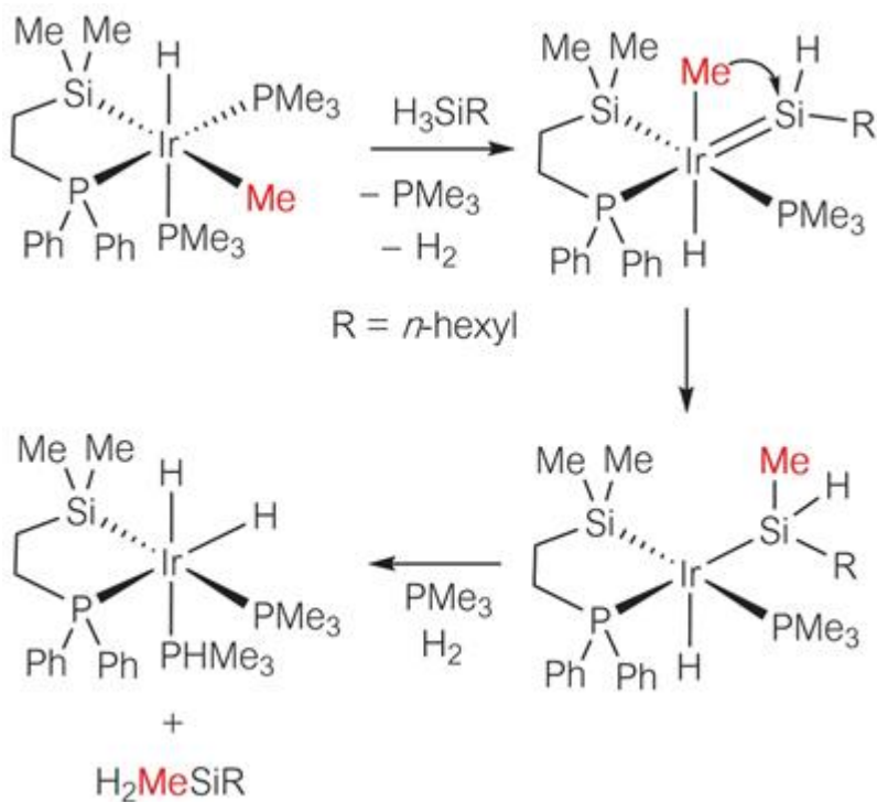
Figure 8.18 1,2-Me-shift in a silylene complex.
