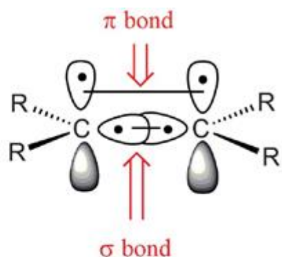
(b) olefin formation by dimerization of triplet carbene
