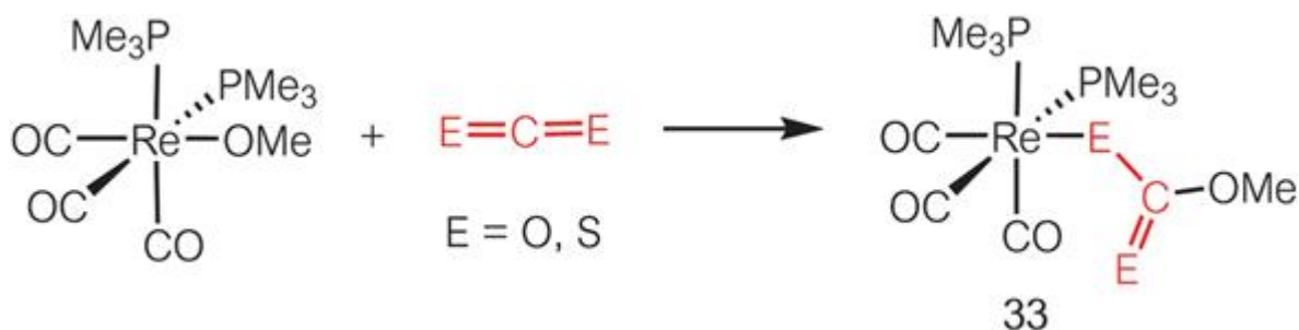
Figure 11.29 Insertion of \text{CO}_2 and \text{CS}_2 into a Re–O bond.
