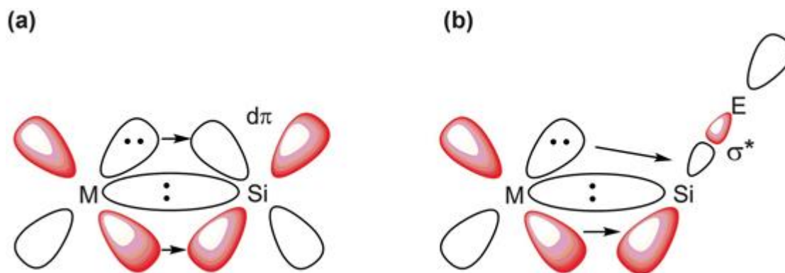
Figure 8.2 \pi -Back donation in transition metal–silyl complexes.
