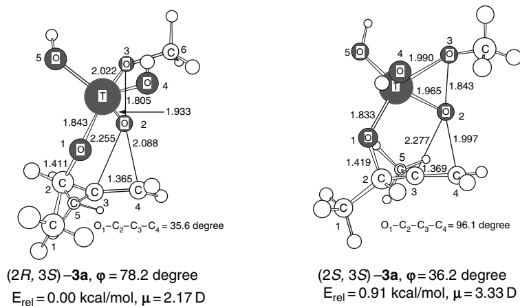
Fig. 12.7. Alternate orientations of 3-methylbut-3-en-1-ol ( 3a ) in the transition state for Ti-mediated epoxidation. Angle \phi is the inter-ring angle of the spiro rings. Reproduced from J. Org. Chem. , 67 , 1427 (2002), by permission of the American Chemical Society.
