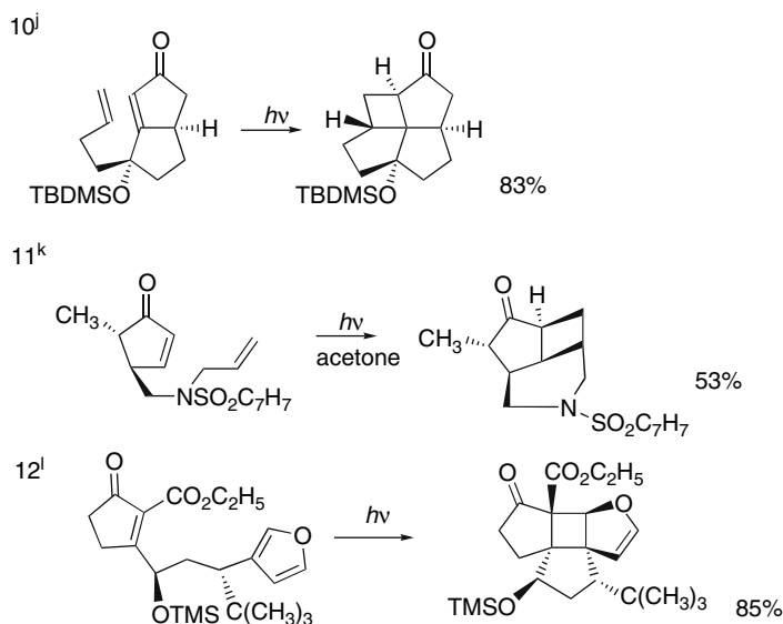
Scheme 6.10. (Continued)
