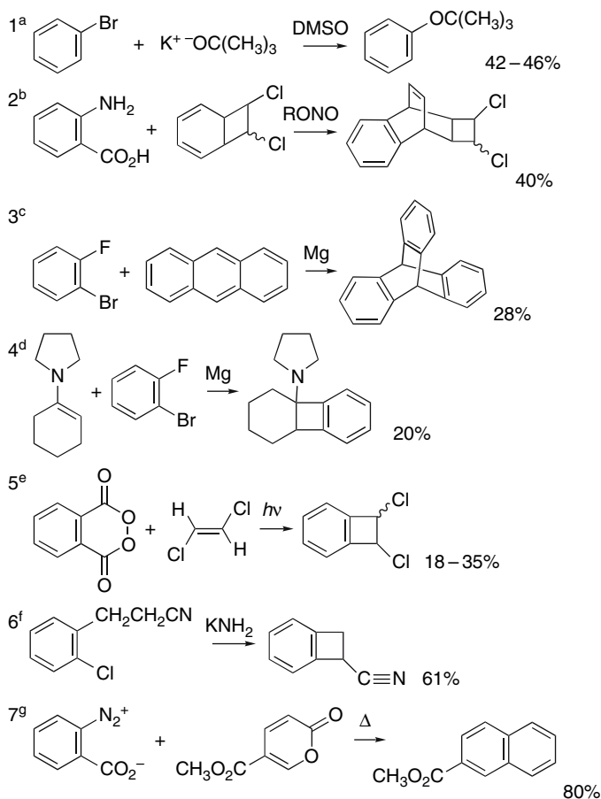
Scheme 11.9. Syntheses via Benzyne Intermediates
