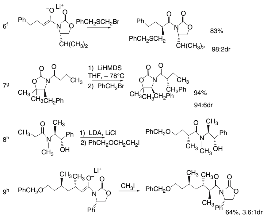
Scheme 1.9. (Continued)
