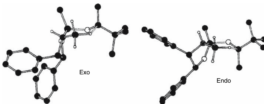
Fig. 5.8. Optimized (HF/3-21G) structures of the exo and endo transition states for reduction of t -butyl methyl ketone by model catalyst. The exo structure is favored by 2.1 kcal, in accord with an experimental e.e of 88%. Reproduced from J. Am. Chem. Soc. , 116 , 8516 (1994), by permission of the American Chemical Society.
