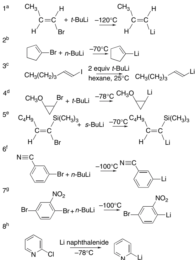
Scheme 7.2. Preparation of Organolithium Reagents by Halogen-Metal Exchange
