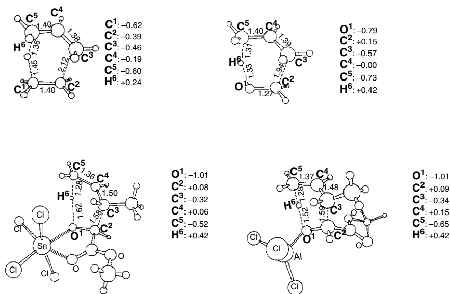
Fig. 10.1. Minimum-energy transition structures for ene reactions: (a) propene and ethene; (b) propene and formaldehyde; (c) butene and methyl glyoxylate– \text{SnCl}_4 ; (d) butene and methyl glyoxylate– \text{AlCl}_3 . Reproduced from Helv. Chim. Acta , 85 , 4264 (2002), by permission of Wiley-VCH.
