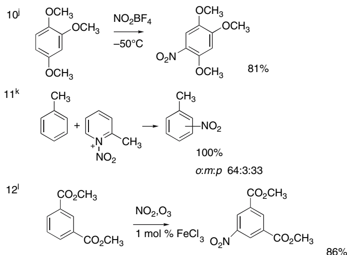
Scheme 11.1. (Continued)
