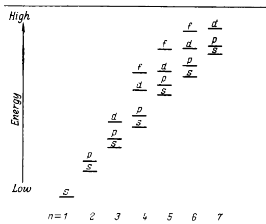
Fig. 2.5. Orbital energy levels for neutral atoms.
