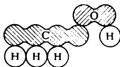
Methyl alcohol
