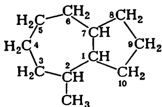
2-Methylbicyclo [5.3.0]decane
