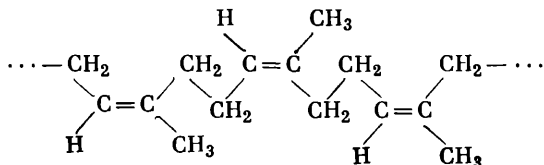
cis -Polyisoprene (natural rubber)
