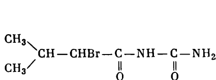
Bromural
