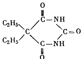
Veronal
