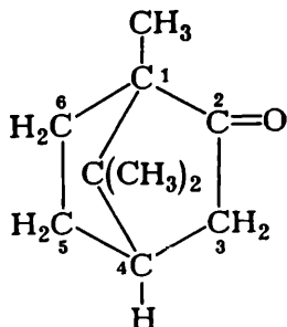
1,7,7- Trimethylbicyclo [2.2.1]- heptan -2- one (camphor)
