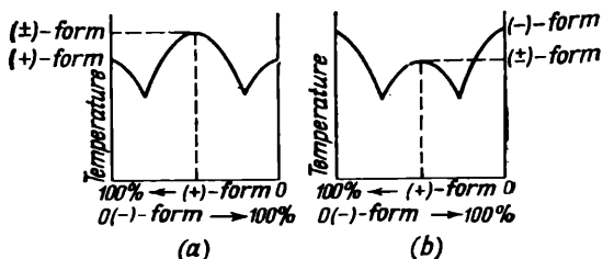
Fig. 4.1. Melting-point diagrams for racemates:
