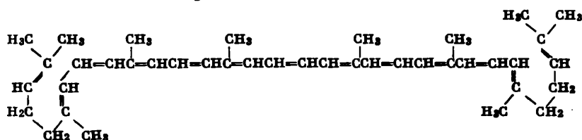
Lycopene
