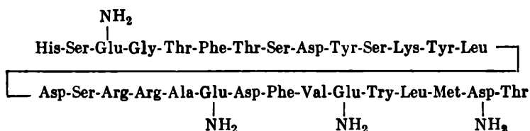
Glucagon
