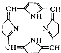
Porphin
