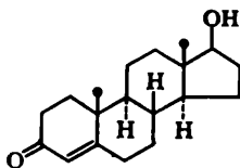
Testosterone
