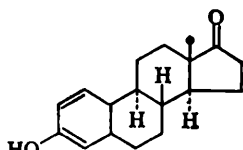
Estrone (folliculin)
