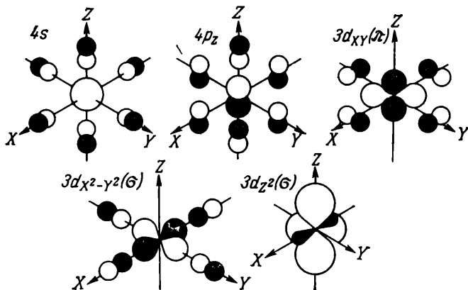
Fig. 12.10. The atomic orbitals of transition metals, which take part in the formation of molecular orbitals of octahedral complexes. The filled circles are regions of negative values of the orbital wave functions.
