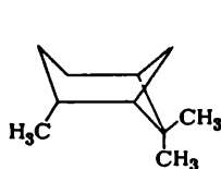
Pinane
