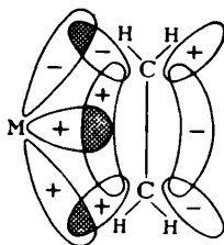
Fig. 12.9. The formation of an octahedral complex.
