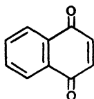
\alpha -Naphthaquinone
