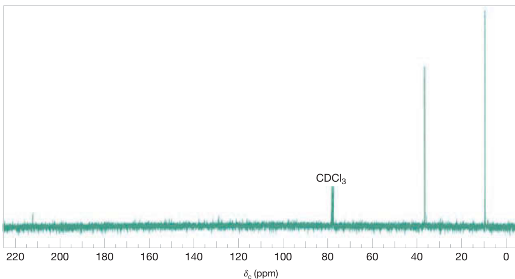
FIGURE A.5 ^{13}\text{C} NMR spectrum of a compound with molecular formula \text{C}_5\text{H}_{10}\text{O} (see Practice Problem A.1). (Adapted from the original (www.sigmaaldrich.com/spectra/fnmr/FNMR004058.PDF) with permission from Sigma Aldrich.)
