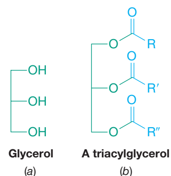
FIGURE 23.1 (a) Glycerol.
