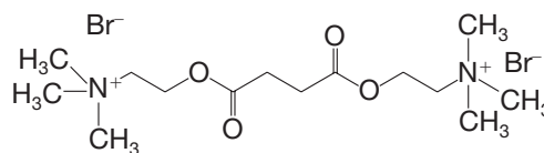
Succinylcholine bromide
