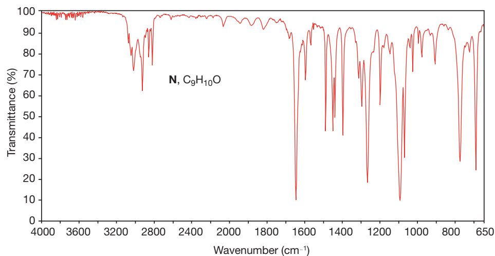
FIGURE 3 The IR spectrum of compound N , Problem 31.
