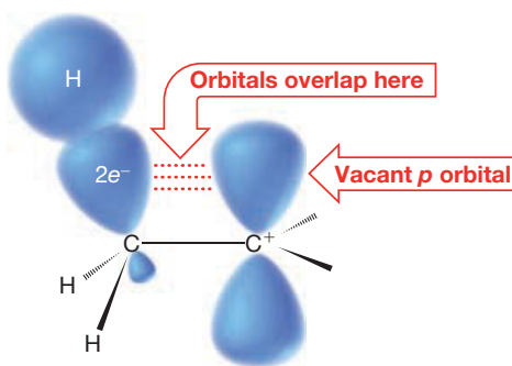
FIGURE 6.7 How an adjacent sigma bond helps stabilize the positive charge of a carbocation.
