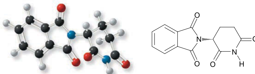
Thalidomide (Thalomid®)
