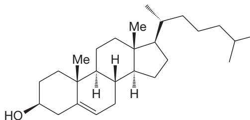
Cholesterol
