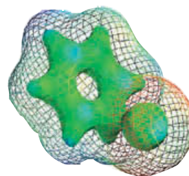
FIGURE 15.2 A calculated structure for the arenium ion intermediate formed by electrophilic addition of bromine to benzene (Section 15.3). The electrostatic potential map for the principal location of bonding electrons (indicated by the solid surface) shows that positive charge (blue) resides primarily at the ortho and para carbons relative to the carbon where the electrophile has bonded. This distribution of charge is consistent with the resonance model for an arenium ion. (The van der Waals surface is indicated by the wire mesh.)
