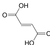
Fumaric acid
