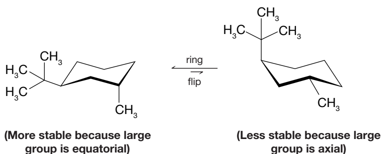
trans -1- tert -Butyl-3-methylcyclohexane
