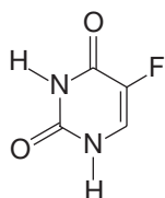
5-Fluorouracil
