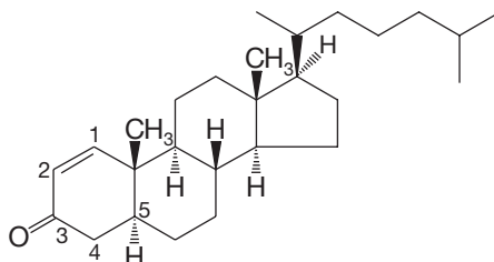
5\alpha -Cholest-1-en-3-one
