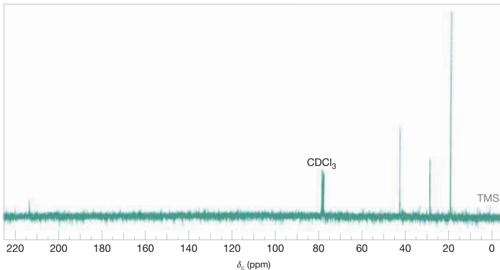
FIGURE A.6 ^{13}\text{C} NMR spectrum of a compound with molecular formula \text{C}_5\text{H}_{10}\text{O} , (see Practice Problem A.2). (Adapted from the original (www.sigmaaldrich.com/spectra/fnmr/FNMR003861.PDF) with permission from Sigma Aldrich.)
