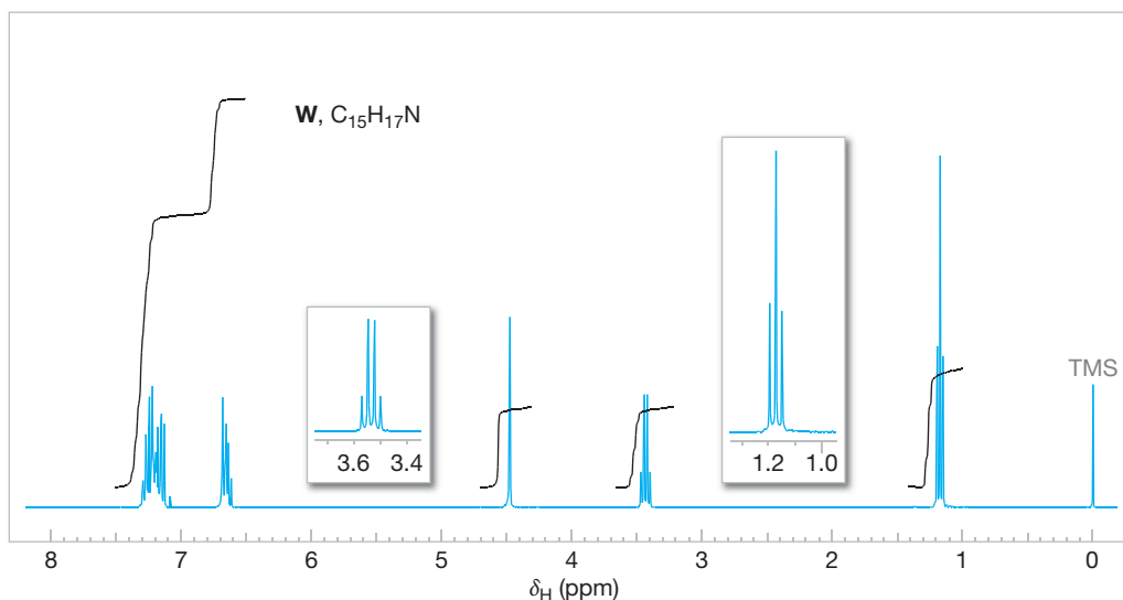
FIGURE 20.6 The ^1\text{H} NMR spectrum of compound W , Problem 20.45. Expansions of the signals are shown in the offset plots.
