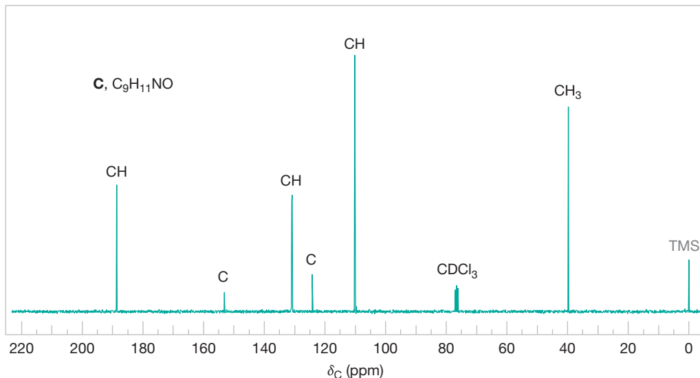
FIGURE 5 The broadband proton-decoupled ^{13}\text{C} NMR spectra of compound C , Problem 34. Information from the DEPT ^{13}\text{C} NMR spectra is given above each peak.
