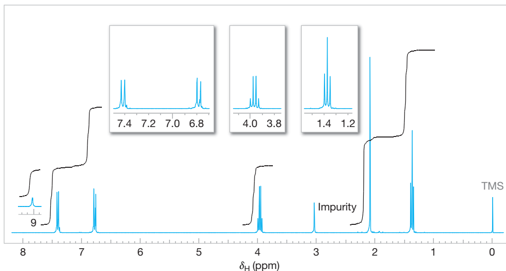
FIGURE 17.7 The ^1H NMR and IR spectra of phenacetin. Expansions of the ^1H NMR signals are shown in the offset plots.
