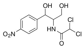
Chloramphenicol
