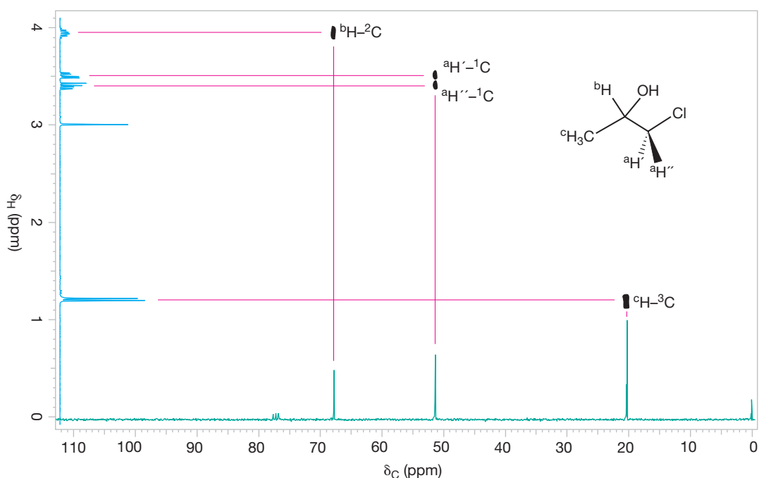
FIGURE 9.23 ^1\text{H} - ^{13}\text{C} heteronuclear correlation NMR spectrum of 1-chloro-2-propanol. The ^1\text{H} NMR spectrum is shown in blue and the ^{13}\text{C} NMR spectrum is shown in green. Correlations of the ^1\text{H} - ^{13}\text{C} cross peaks with the one-dimensional spectra are indicated by red lines.
