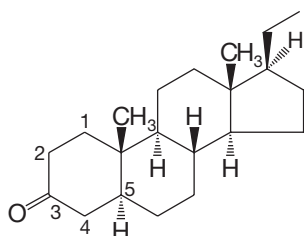
5\alpha -Pregnan-3-one
