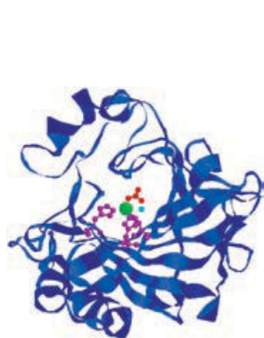
Carbonic anhydrase
