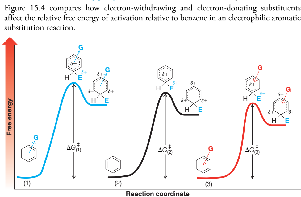
FIGURE 15.4 A comparison of free-energy profiles for arenium ion formation in a ring with an electron-withdrawing substituent ( \rightarrow G ), no substituent, and an electron-donating substituent ( \leftarrow G ). In (1) (blue energy profile), the electron-withdrawing group G raises the transition state energy. The energy of activation barrier is the highest, and therefore the reaction is the slowest. Reaction (2), with no substituent, serves as a reference for comparison. In (3) (red energy profile), an electron-donating group G stabilizes the transition state. The energy of activation barrier is the lowest, and therefore the reaction is the fastest. WILEYPLUS
