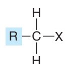
Primary ( 1^\circ )
