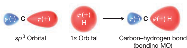
FIGURE 1.16 Formation of a C–H bond.
