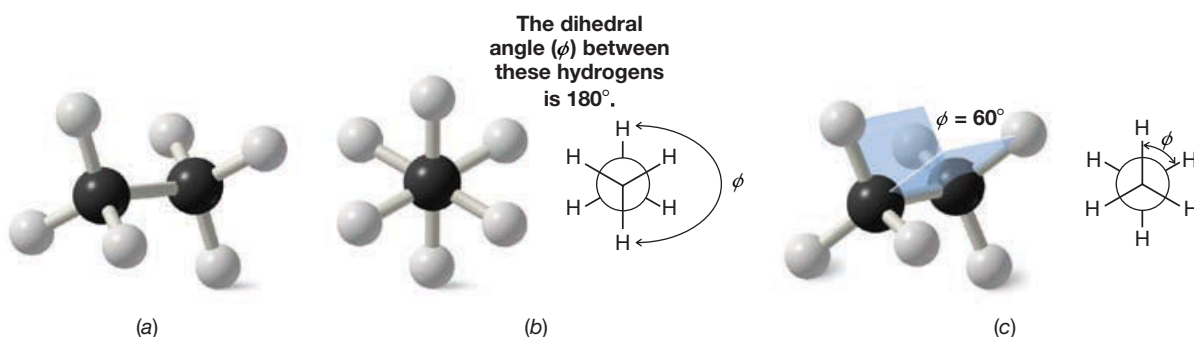
FIGURE 4.5 (a) The staggered conformation of ethane. (b) The Newman projection formula for the staggered conformation. (c) The dihedral angle between these hydrogen atoms is 60°.
