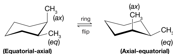
cis -1,2-Dimethylcyclohexane
