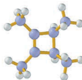
cis -Tetramethylcyclobutene
