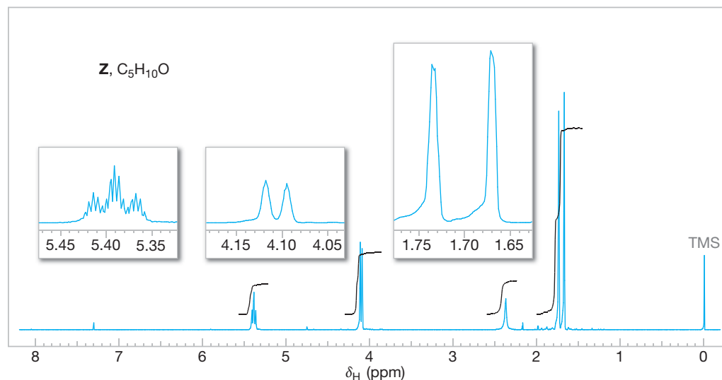
FIGURE 6 The ^1\text{H} NMR spectrum of compound Z (Problem 36). Expansions of the signals are shown in the offset plots.
