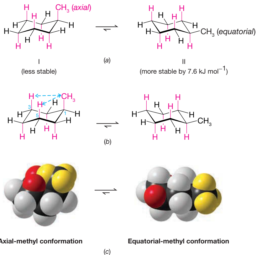
FIGURE 4.19 (a) The conformations of methylcyclohexane with the methyl group axial ( I ) and equatorial ( II ). (b) 1,3-Diaxial interactions between the two axial hydrogen atoms and the axial methyl group in the axial conformation of methylcyclohexane are shown with dashed arrows. Less crowding occurs in the equatorial conformation. (c) Space-filling molecular models for the axial-methyl and equatorial-methyl conformers of methylcyclohexane. In the axial-methyl conformer the methyl group (shown with yellow hydrogen atoms) is crowded by the 1,3-diaxial hydrogen atoms (red), as compared to the equatorial-methyl conformer, which has no 1,3-diaxial interactions with the methyl group.
