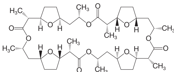
Nonactin
