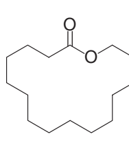
Pentalide
