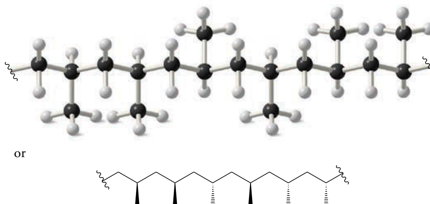
FIGURE C.1 Atactic polypropylene.
