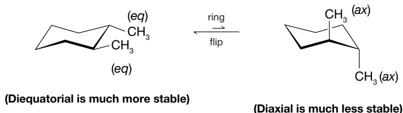
trans -1,2-Dimethylcyclohexane
