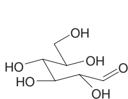
Glucose
