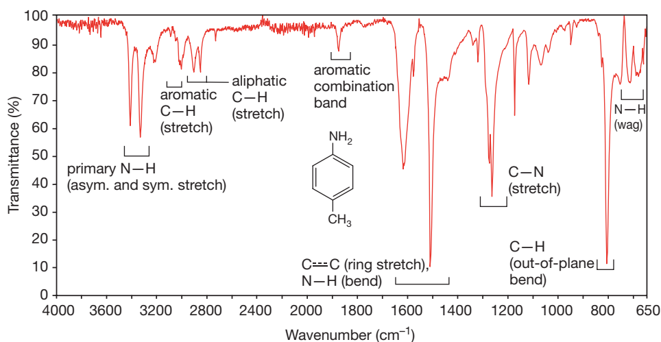
FIGURE 20.4 Annotated IR spectrum of 4-methylaniline.
