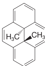
trans -15,16-Dimethyldihydropyrene
