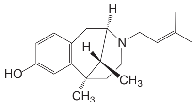
Pentazocine
