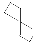
FIGURE 7.4 Hypothetical trans -cyclohexene. This molecule is apparently too strained to exist at room temperature.
