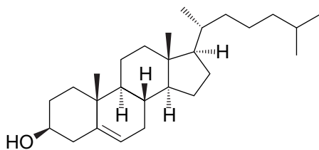
Cholesterol
