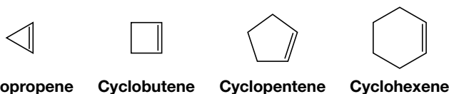
FIGURE 7.3 cis -Cycloalkenes.
