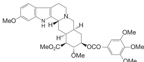
Reserpine
