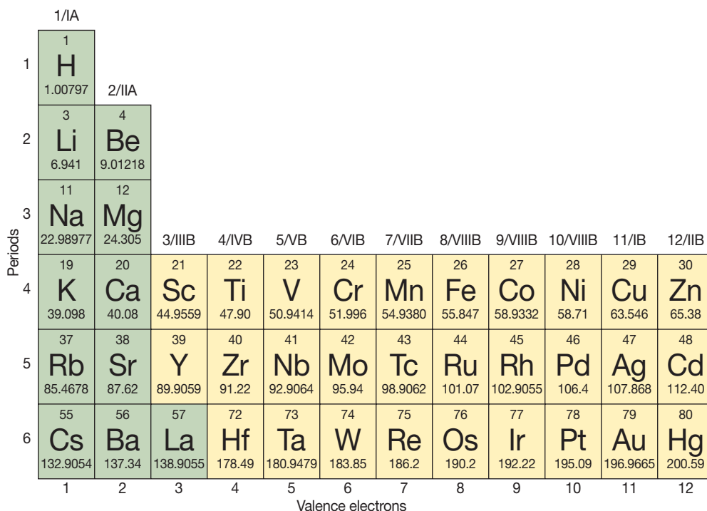
FIGURE 21.1 Important transition elements are shown in the green and yellow portion of the periodic table. Given across the bottom is the total number of valence electrons ( s and d ) of each element.
