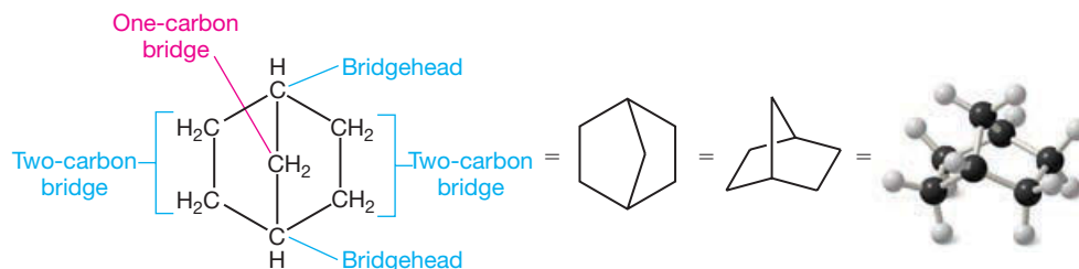
A bicycloheptane
