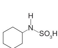
Cyclamate
