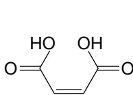
Maleic acid
