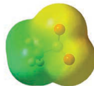
Acetate anion
