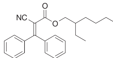
2-Ethylhexyl 2-cyano-3,3-diphenylacrylate (Octocrylene), \lambda_{\text{max}} 310 nm
