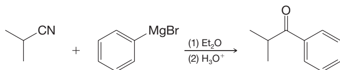
2-Cyanopropane
