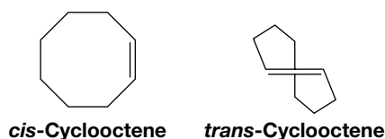
FIGURE 7.5 The cis and trans forms of cyclooctene.
