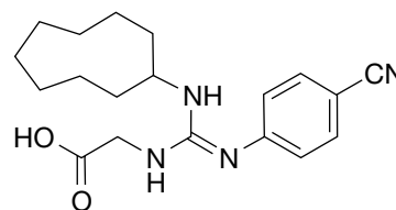
Sucronic acid
