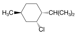
Neomenthyl chloride
