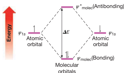
FIGURE 1.12 Energy diagram for the hydrogen molecule. Combination of two atomic orbitals, \psi_{1s} , gives two molecular orbitals, \psi_{\text{molec}} and \psi_{\text{molec}}^* . The energy of \psi_{\text{molec}} is lower than that of the separate atomic orbitals, and in the lowest electronic energy state of molecular hydrogen the bonding MO contains both electrons.
