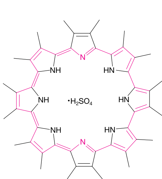
Octaporphyrin [30 electron system; n = 7 ]
