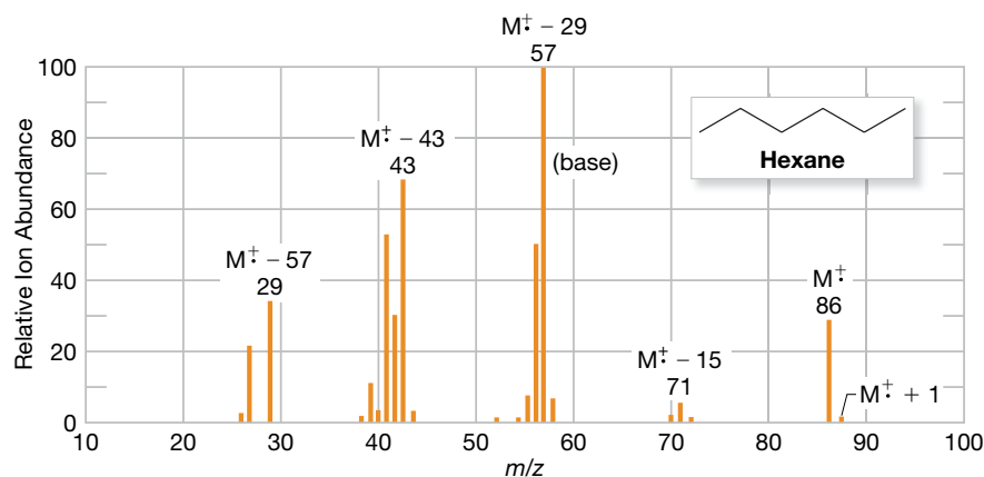
FIGURE 9.26 Mass spectrum of hexane.
