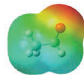
Acetaldehyde
