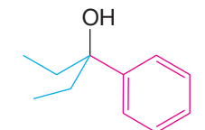
3-Phenyl-3-pentanol
