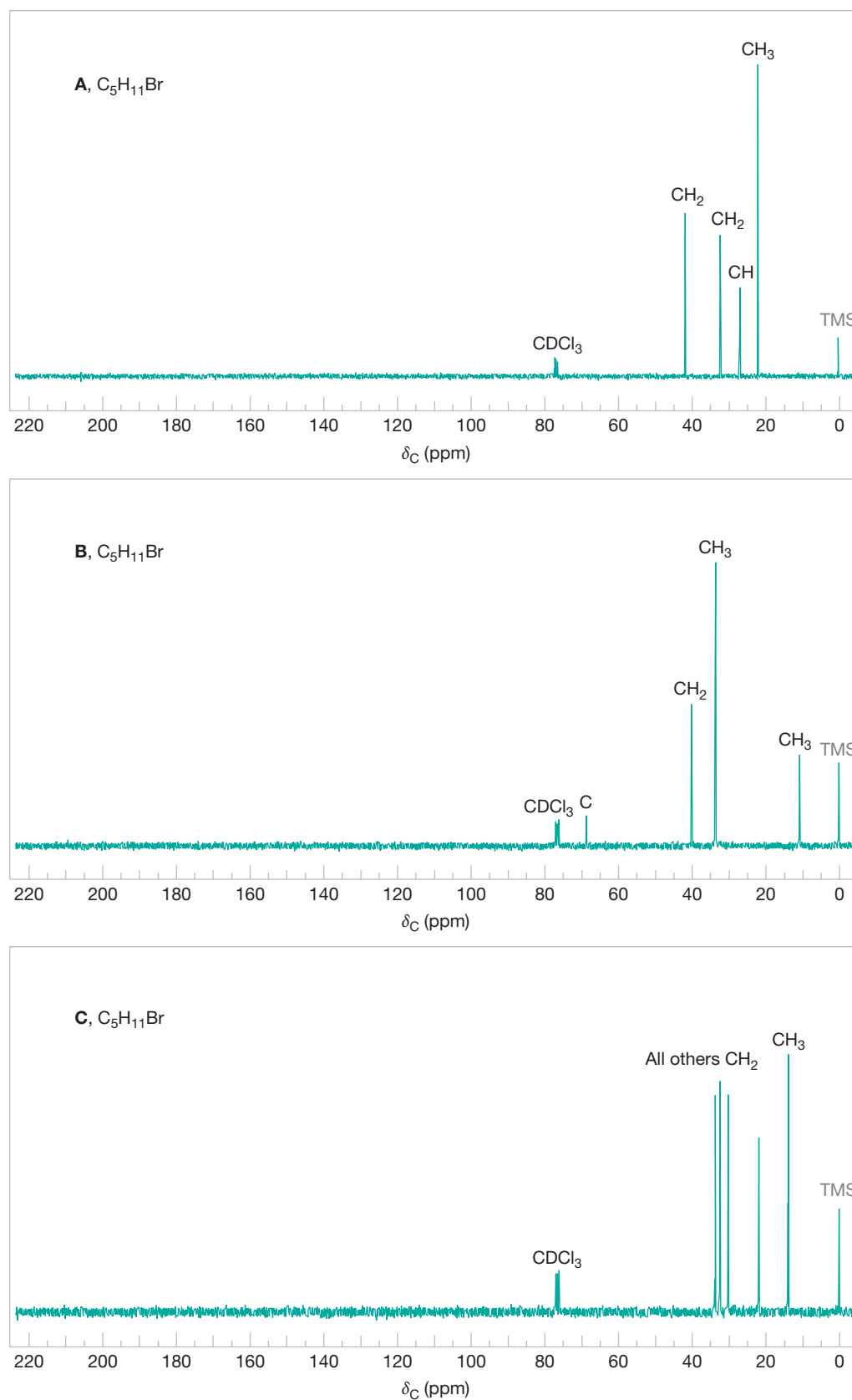
FIGURE 9.21 The broadband proton-decoupled ^{13}C NMR spectra of compounds A , B , and C , Practice Problem 9.14. Information from the DEPT ^{13}C NMR spectra is given above the peaks.
