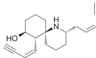
Histrionicotoxin
