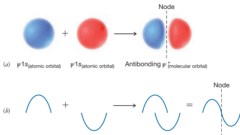
FIGURE 1.11 (a) The overlapping of two hydrogen 1s atomic orbitals with opposite phase signs (indicated by their different colors) to form an antibonding molecular orbital. (b) The analogous overlapping of two waves with the opposite sign, resulting in destructive interference and decreased amplitude. A node exists where complete cancellation by opposite phases makes the value of the combined wave function zero.
