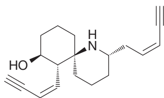
Histrionicotoxin
