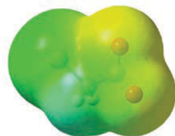
Chloroacetate anion
