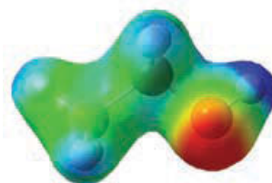
Ethanol
