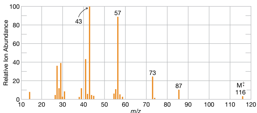
FIGURE 9.30 Mass spectrum for Practice Problem 9.17.
