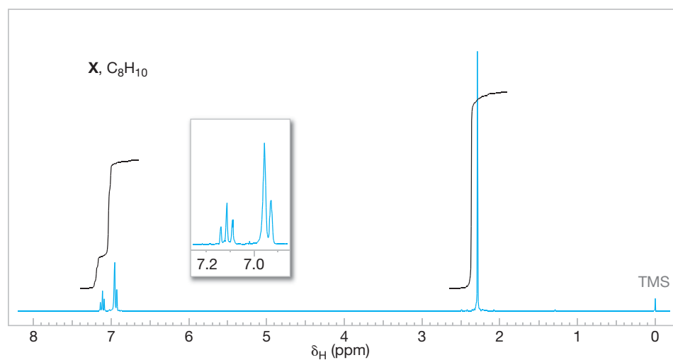
FIGURE 14.31 The IR and 1 H NMR spectra of compound X , Problem 14.36. Expansions of the signals are shown in the offset plots.
