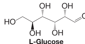
L-Glucose
