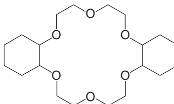
Dicyclohexano-18-crown-6
