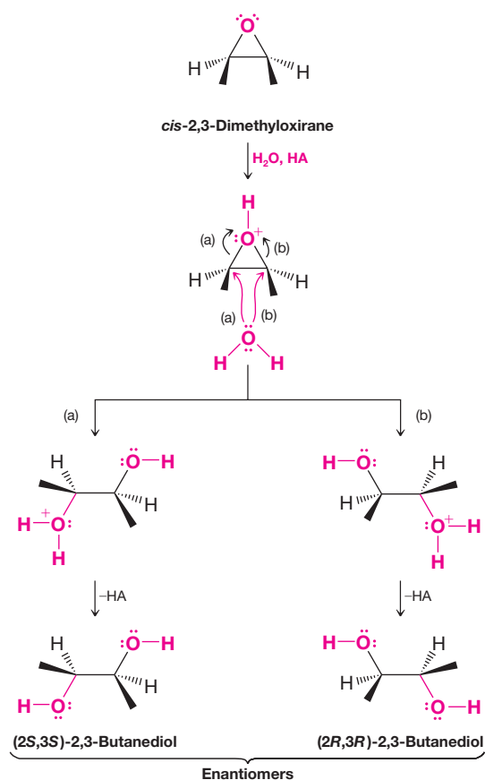
FIGURE 11.1 Acid-catalyzed hydrolysis of cis -2,3-dimethyloxirane yields (2 S ,3 S )-2,3-butanediol by path (a) and (2 R ,3 R )-2,3-butanediol by path (b). (Use models to convince yourself.)
