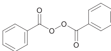
Benzoyl peroxide
