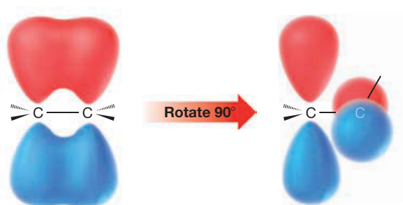
FIGURE 1.27 A stylized depiction of how rotation of a carbon atom of a double bond through an angle of 90^\circ results in breaking of the \pi bond.
