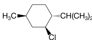
Menthyl chloride
