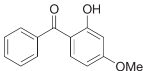
2-Hydroxy-4-methoxybenzophenone (Oxybenzone), \lambda_{\text{max}} 288 and 325 nm
