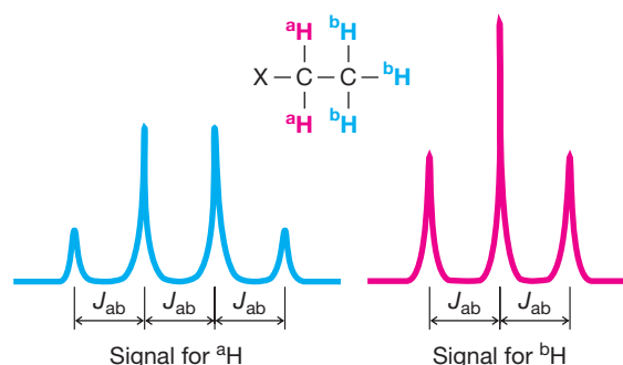
FIGURE 9.15 A theoretical splitting pattern for an ethyl group. For an actual example, see the spectrum of bromoethane (Fig. 9.1).
