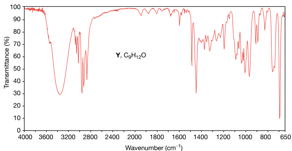
FIGURE 14.32 The IR and 1 H NMR spectra (next page) of compound Y , Problem 14.37. Expansions of the signals are shown in the offset plots.
