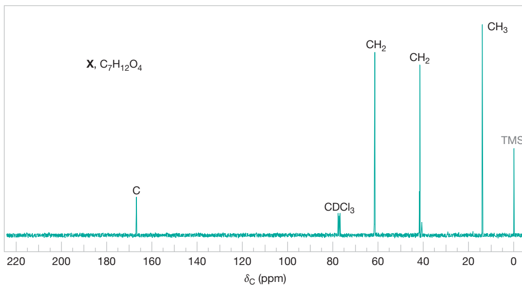
FIGURE 4 Broadband proton-decoupled ^{13}\text{C} NMR spectrum of compound X , Problem 32. Information from the DEPT ^{13}\text{C} NMR spectra is given above each peak.
