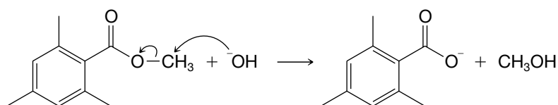
Methyl mesitoate
