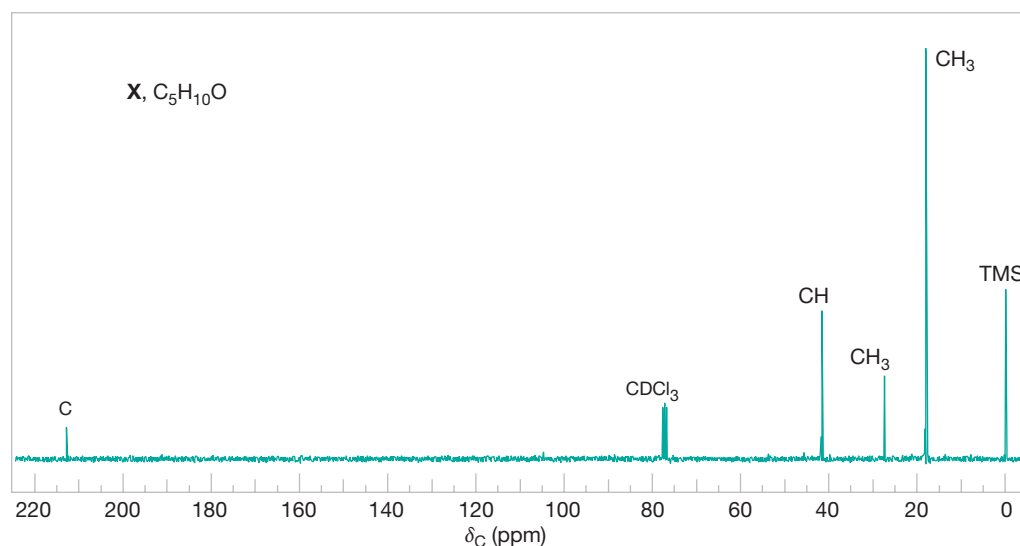
FIGURE 2 The broadband proton-decoupled ^{13}\text{C} NMR spectrum of compound X (Problem 36). Information from the DEPT ^{13}\text{C} NMR spectra is given near each peak.
