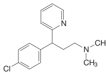
Chlorpheniramine
