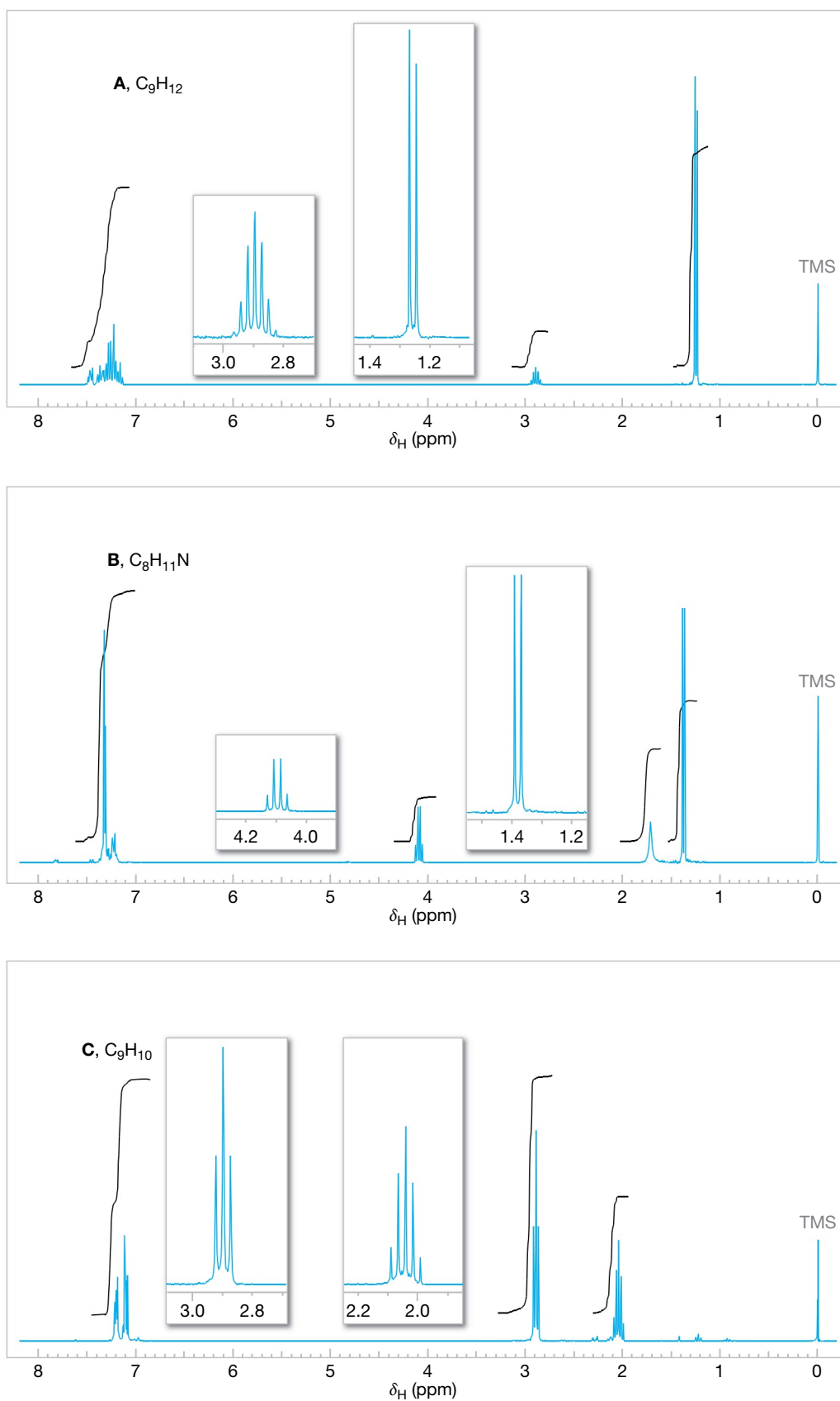
FIGURE 14.27 The ^1\text{H} NMR spectra for Problem 14.31. Expansions of the signals are shown in the offset plots.
