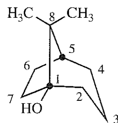
8,8-dimethyl- bicyclo[3.2.1]octan-1-ol
