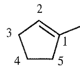
1-methylcyclopentene
