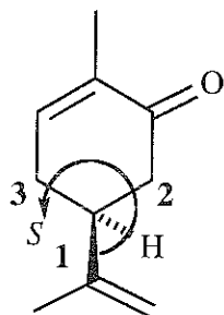
(+)-carvone (caraway seed)
