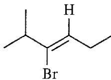
( Z )-3-bromo-2-methylhex-3-ene
