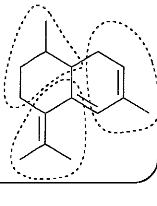
zingiberene sesquiterpene
