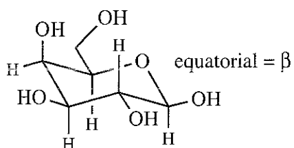
(b) \beta -D-galactopyranose
