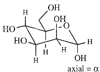
(a) \alpha -D-mannopyranose
