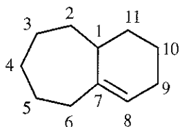
bicyclo[5.4.0]undec-7-ene
