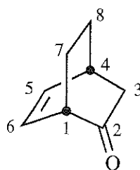
bicyclo[2.2.2]oct-5-en-2-one
