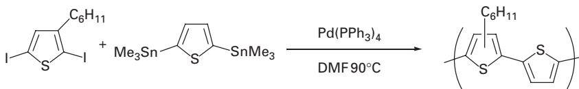
Scheme 4 Preparation of a regio-random poly(thiophene) derivative by a palladium-catalysed polycondensation.
