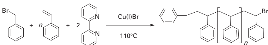
Scheme 7 Polymerization of styrene using ATRP.
