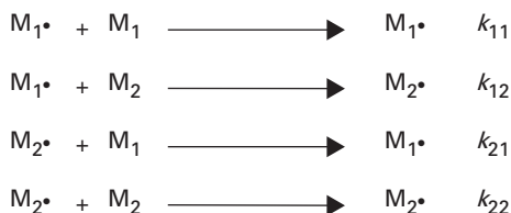
Scheme 6 Reactions occurring in a copolymerization; in the simplest model, the reactivity of the propagating chain is considered to be dependent only on the terminal monomer unit.
