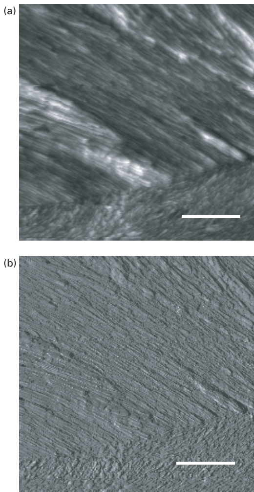
Fig. 1.9 AFM tapping mode images of a spherulitic texture in isotactic polypropylene. The sample was crystallized to completion at 145°C and subjected to permanganic etching prior to examination. Image (a) shows topography while (b) contains phase information. Scale bars 5 \mu\text{m} .
