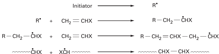
Scheme 1 Mechanism of free-radical polymerization.
