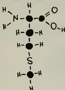
METHIONINE
