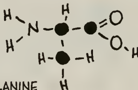
ALANINE
