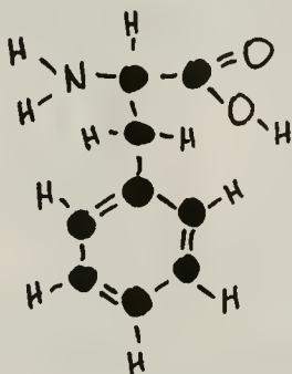
PHENYLALANINE
