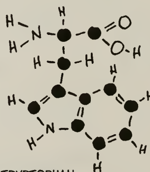
TRYPTOPHAN
