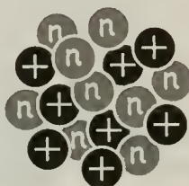
^{17}\text{O} NUCLEUS
