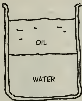
IMMISCIBLE
