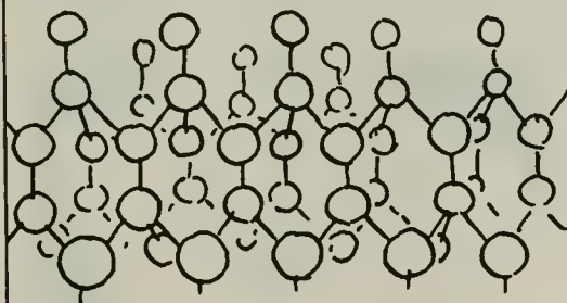
DIAMOND
