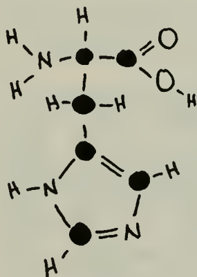
HISTIDINE
