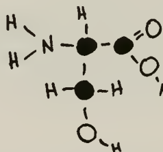
SERINE
