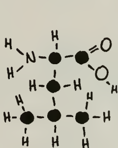
LEUCINE
