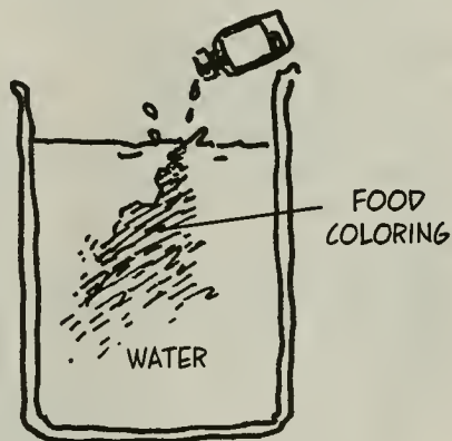
MISCIBLE
