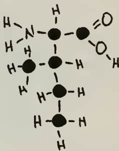
ISOLEUCINE
