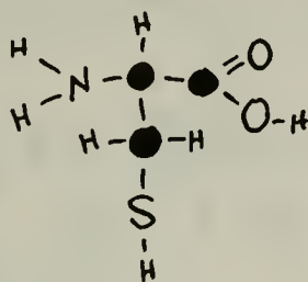
CYSTEINE
