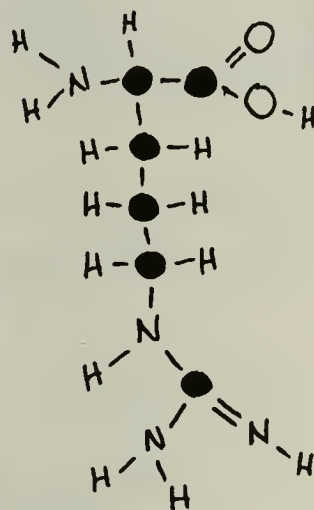
ARGININE
