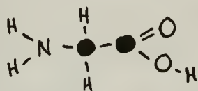
GLYCINE
