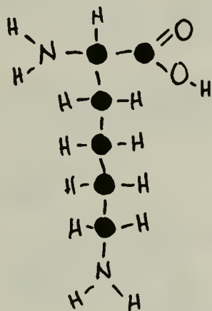
LYSINE
