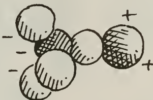
ION-DIPOLE ATTRACTION
