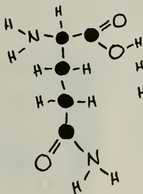
GLUTAMINE
