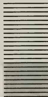
PRODUCTS
