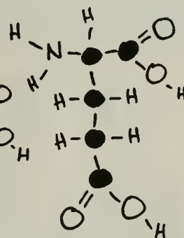
GLUTAMIC ACID
