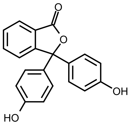
phenolphthalein
