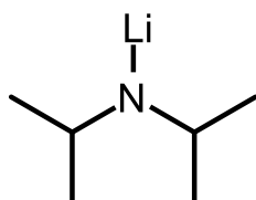
lithium diisopropylamide, synonym lithium diisopropylazanide.
