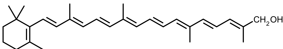
zeaxanthin, \beta,\beta -carotene-3,3'-diol (a xanthophyll)
