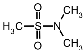
N,N -dimethylmethanesulfonamide,
