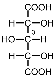
xylaric acid
