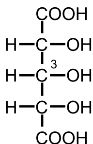
ribaric acid
