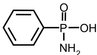
phenylphosphonamidic acid.
