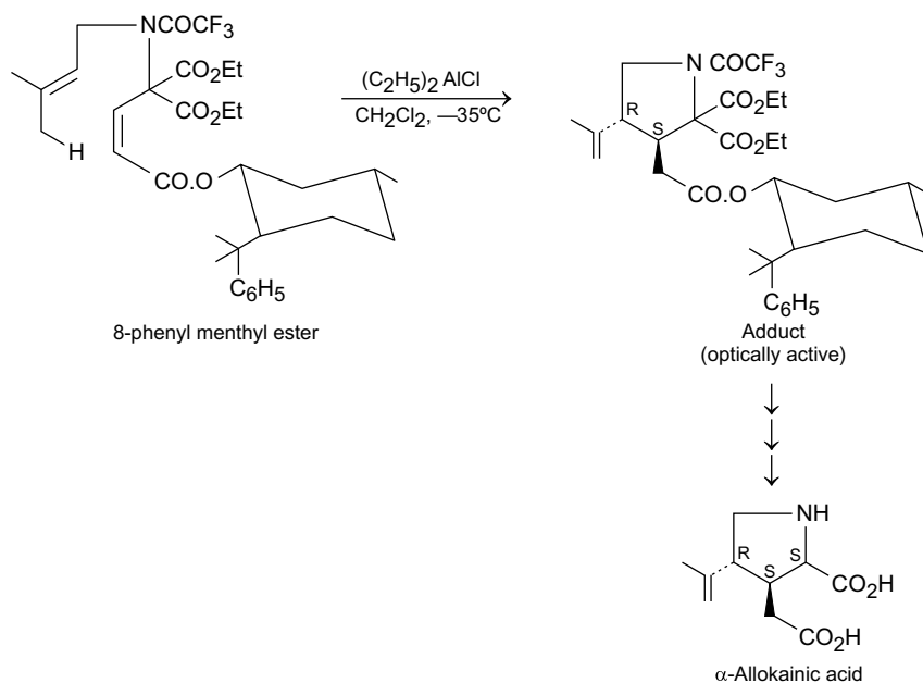
Fig. 19.41 Synthesis of \alpha -allokainic acid by an intramolecular ene reaction
