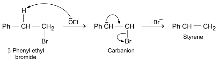
Fig. 7.35 Elimination reaction of carbanion
