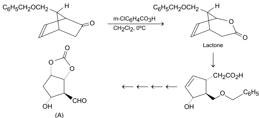
Fig. 19.16 Baeyer–Villiger reaction of bridged bicyclic ketone
