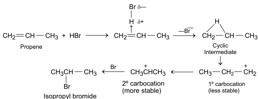
Fig. 7.81 Addition to \text{HBr} to propene gives isopropyl bromide
