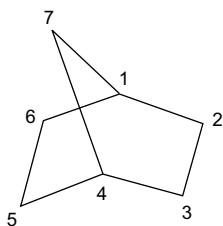
Bicyclo[2,2,1]heptane
