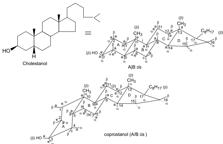
Fig. 8.18 Cholestanol and coprostanol
