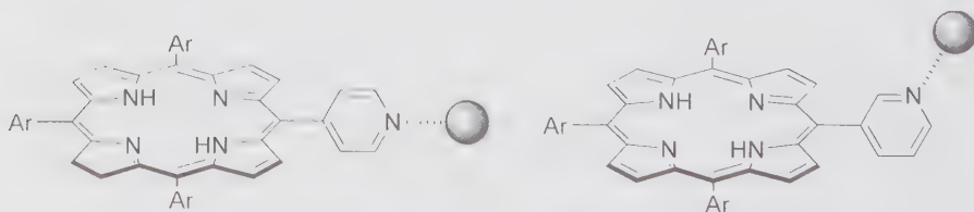
Fig. 2 Coordination interaction of meso -Py and metal
