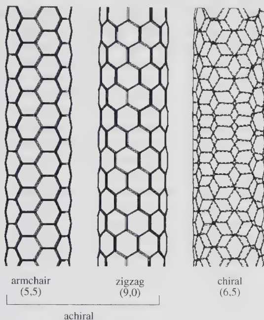
Fig. 2 Armchair, zigzag, chiral structures of SWNTs [52, 53]
