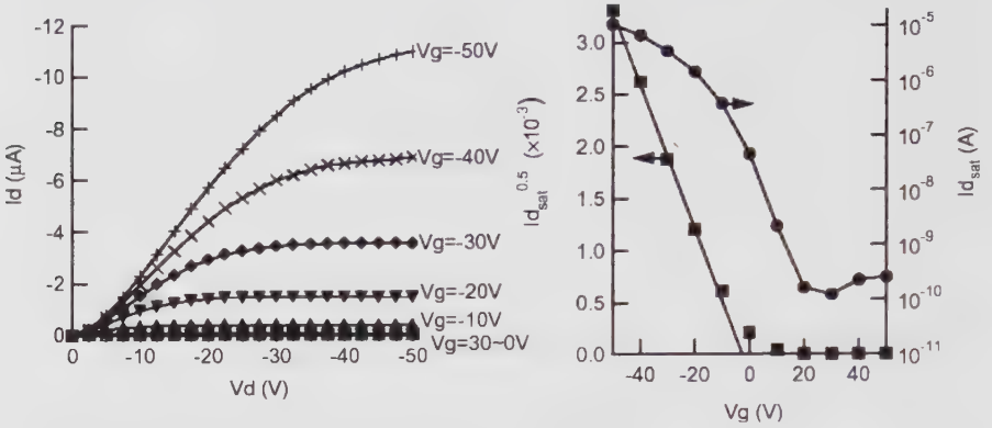
Fig. 32 Transfer characteristics of a TBP OFET on SiO 2 [126]
