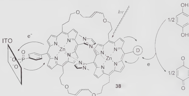
Fig. 24 Schematic illustration of the structure of donor|porphyrin 38 |ITO ( D = \text{Ph}, \text{Me}_3\text{Fc}, \text{Fc}, \text{PhMe}_3\text{Fc}, \text{PhFc}, \text{and } \text{C}_2\text{Fc} ) [98]
