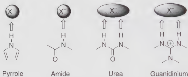
Fig. 7 Hydrogen bonding interactions for anion binding
