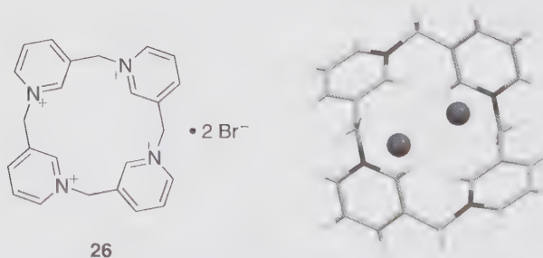
Fig. 10 Cyclic pyridinium tetramer 26 and its \text{Br}^- complex structure
