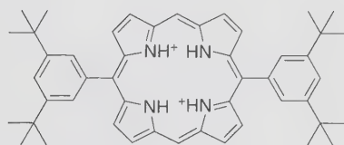
diacidic form of 34
