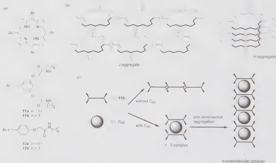
Fig. 10 a Structure of amino-appended porphyrins 11 and 12; b J - and H -aggregate of porphyrins 11 and 12, respectively, and c one-dimensional aggregate of C_{60} and 11b [26, 27]
