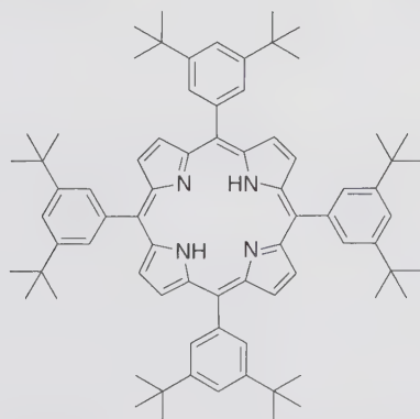
tetrakis(3,5-di- tert -butylphenyl)porphyrin 35
