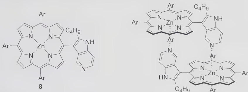
Fig. 6 Dimeric assembly of porphyrin 8 [22]
