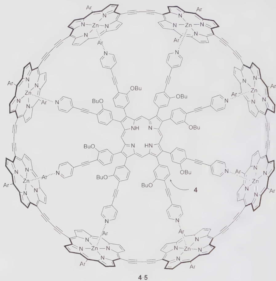
Fig. 4 Template-directed synthesis of porphyrin nanoring 5 [18]
