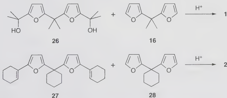
Scheme 5 Syntheses of calix[4]furans by the L2 fragment coupling method [28, 31]
