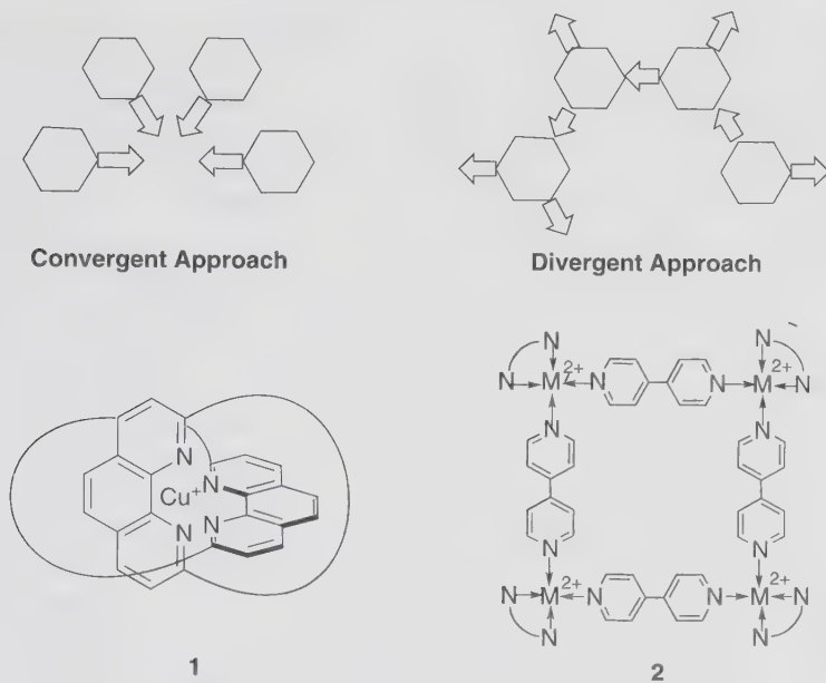
Fig. 1 Convergent and divergent approaches based on heterocyclic chemistry
