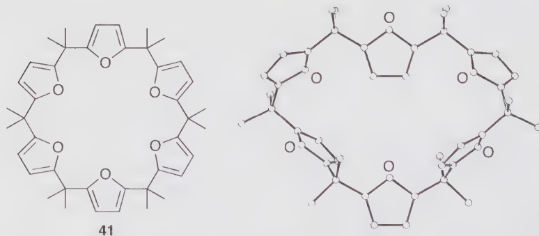
Fig. 5 Crystal structure of calix[6]furan 41 [40, 53]
