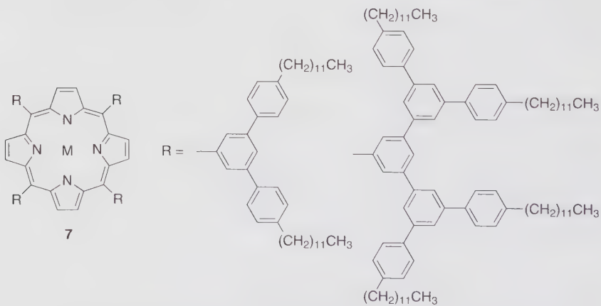
Fig. 5 Structures of porphyrin monomers 1–7 [66–79]
