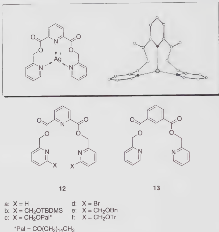
Fig. 3 Tridentate receptors 12 for selective \text{Ag}^+ cation recognition. Reprinted with permission from [17]. © (1998), American Chemical Society
