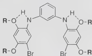
Fig. 1 Folding of the uncyclized precursor by intramolecular \text{NH} \cdots \text{OR} hydrogen bonding interactions [30]
