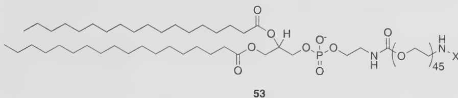
Fig. 16 Structure of PL (phospholipids)-PEG-X 53 [157, 158]
