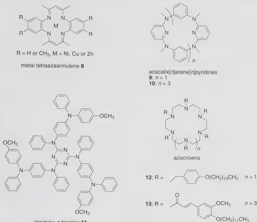
Fig. 6 Structures of nitrogen-containing heterocycles 8–13 [84–88]
