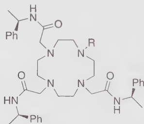
50a: R = H 50b: R = Me
