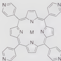
metal tetrakis(4-pyridyl)porphyrins 6
