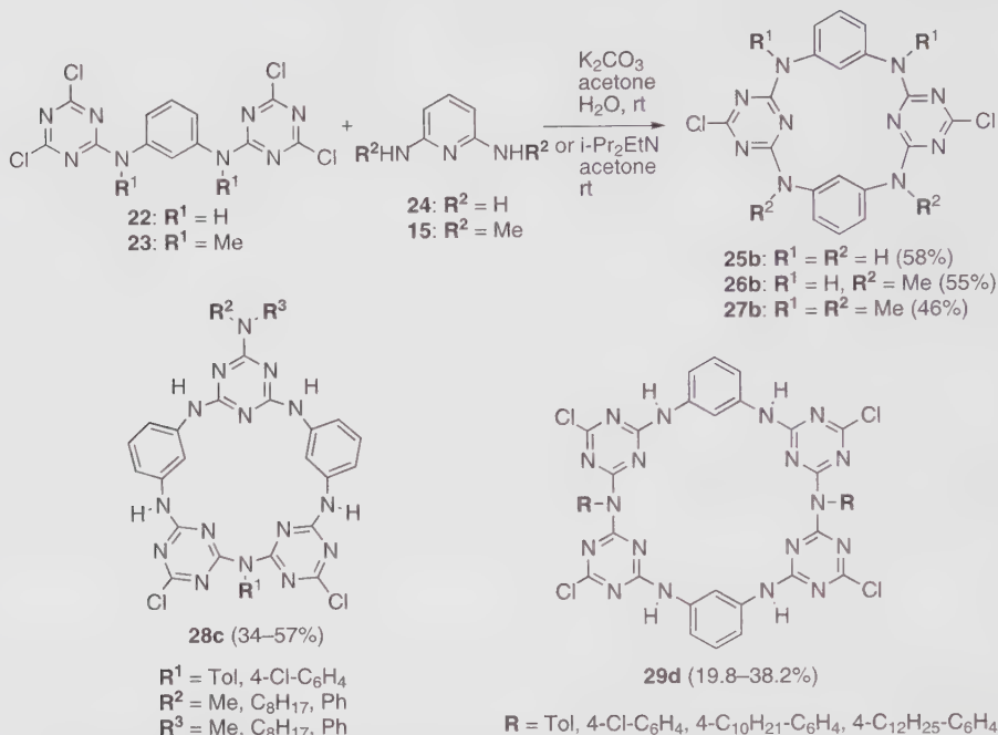
Scheme 7 Fragment-coupling synthesis of azacalixarenetriazines [27–29]
