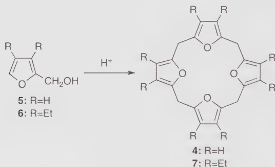
Scheme 1 Syntheses of calix[4]furans 4 and 7 [23, 24]
