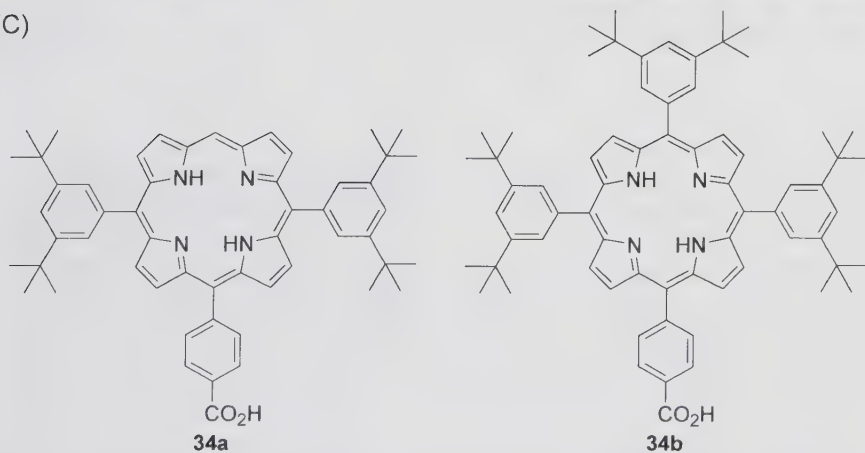
Fig. 21 Diagrammatic summary of the organization between porphyrin 34 and fullerene moieties using TiO 2 nanotubes (A) , nanoparticles (B) and molecular structures of 34a and 34b (C) (reprinted with permission from [93]. © (2007) WILEY-VCH)
