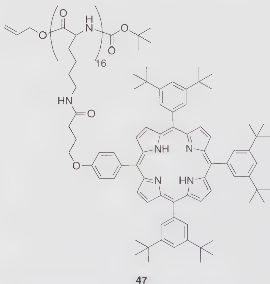
Fig. 14 Structure of porphyrin-peptide hexadecamer 47 [127]
