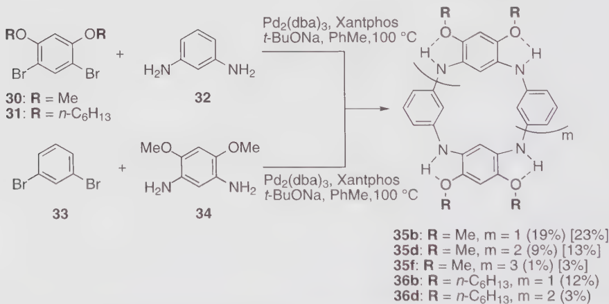
Scheme 8 Fragment-coupling synthesis of azacalixarenes with NH bridges. Numbers in parentheses indicate the reaction yields in the fragment-coupling syntheses using monomers 30 and 32, or 31 and 32 as substrates. Those in square brackets represent the yields in the reaction of 33 and 34 [30]
