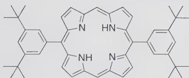
bis(3,5-di- tert -butylphenyl)porphyrin 34
