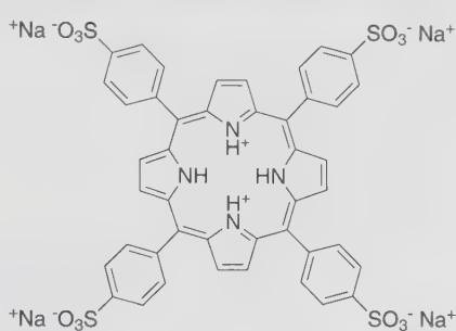
diacidic form of 32
