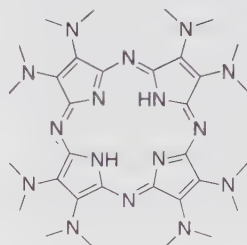
octakis(dimethylamino)porphyrazine 2
