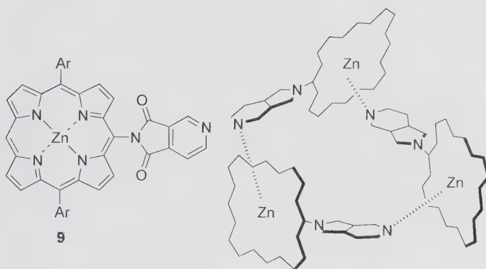
Fig. 7 Cyclic trimer of porphyrin 9 [23]
