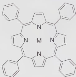
metal tetraphenylporphyrins 1
