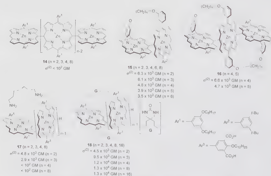
Fig. 12 Molecular structure of dihedral angle controlled, directly linked porphyrin dimers and arrays 14–18 [34]
