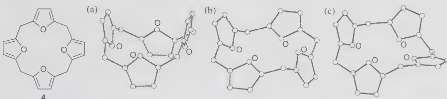
Fig. 2 Crystal structure of calix[4]furan 4 in monoclinic form (a), and two independent structures in triclinic form (b and c) [22]
