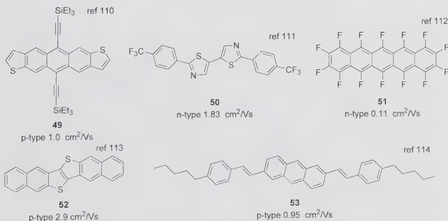
Fig. 30 Recently developed semiconductors for OFET [112–116]
