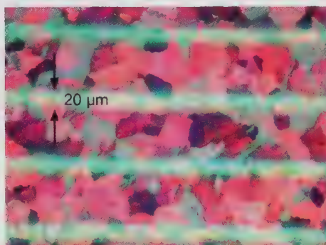
Fig. 35 Polarized optical micrograph of a continuous, spun-cast TBP(Cu) thin-film on thermally oxidized c-Si. The electrodes in the figure are 20 \mu\text{m} wide [127]
