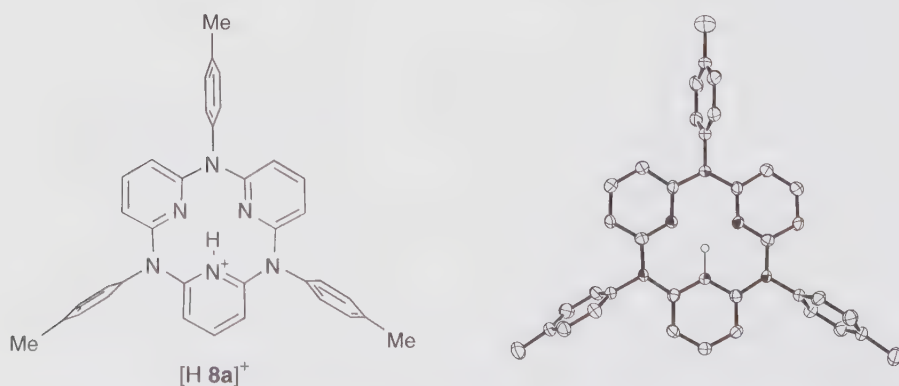
Fig. 13 X-ray crystal structures of monoprotonated azacalix[3]pyridine [\text{H } \mathbf{8a}]^+ [37]
