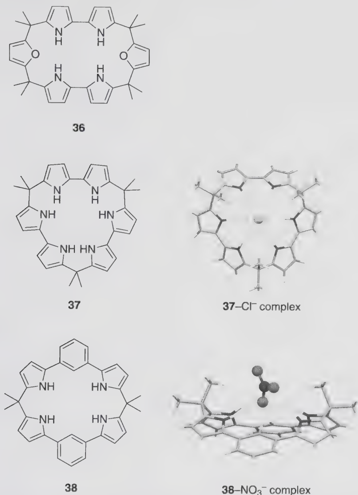
Fig. 14 Pyrrole-containing macrocycles 36–38 and crystal structures of their anion complexes
