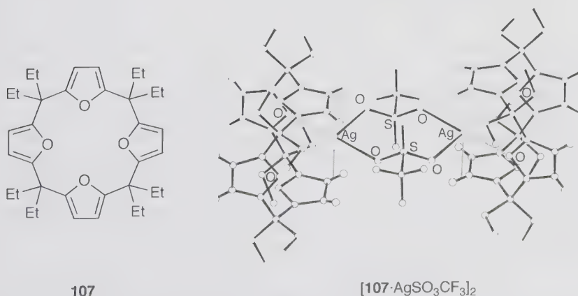
Fig. 6 Crystal structure of complex [107 \cdot \text{AgSO}_3\text{CF}_3]_2 [58]
