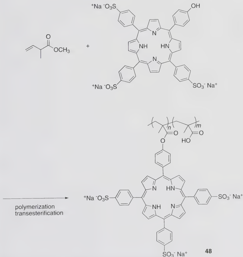
Scheme 3 Preparation of porphyrin/metacrylic acid polymer 48 [131]
