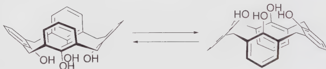
Scheme 11 Ring inversion of calix[4]arene [1, 3]
