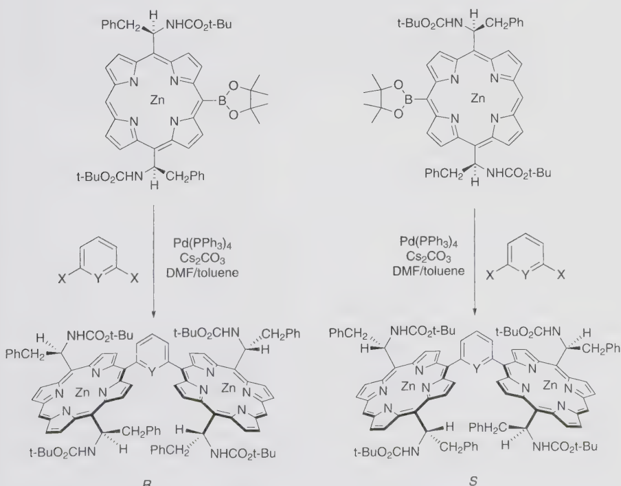
Scheme 2 Synthesis of gable-type porphyrin dimers 46 [56–58]
