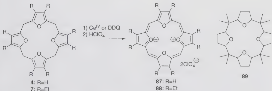
Scheme 11 Syntheses of the dication salts 87 and 88 [23, 25, 51]
