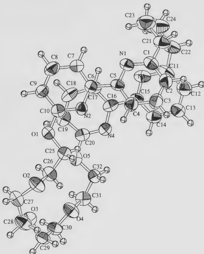
Fig. 2 ORTEP drawing of 58a [52]
