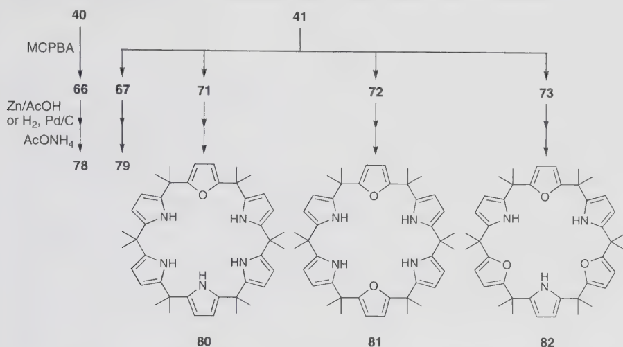
Scheme 10 Conversion of calixfurans to calixpyrroles and hybrid systems [42, 46, 48]
