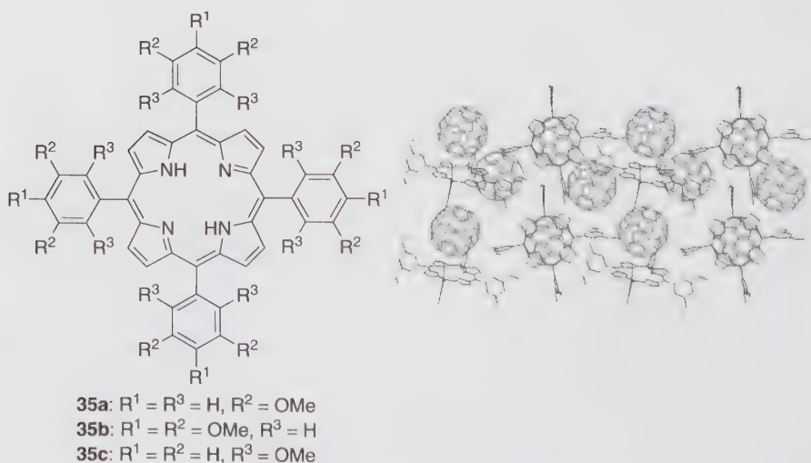
Fig. 22 Molecular structure of porphyrin 35 and molecular packing of 35a - \text{C}_{60} -toluene (reprinted with permission from [90]. © (2006) WILEY-VCH)
