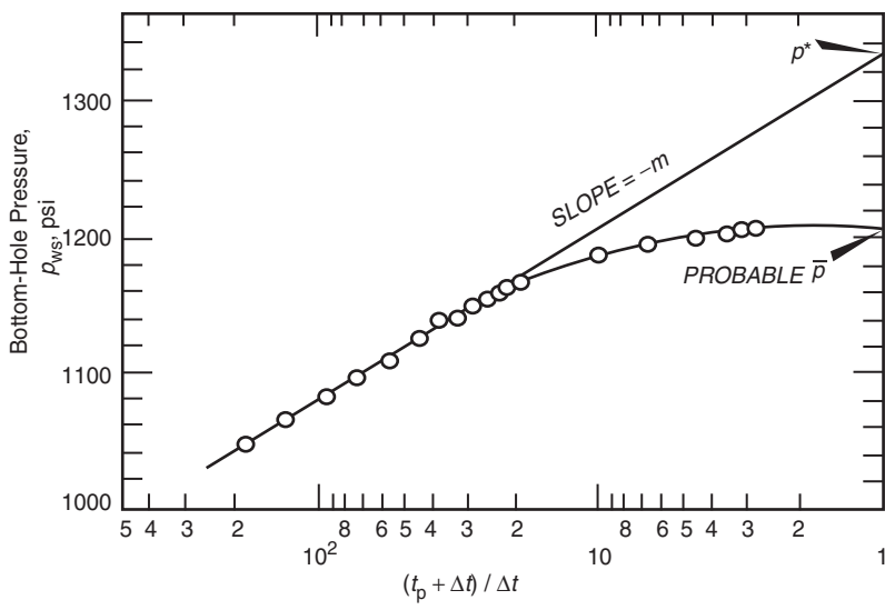
Figure 1.39 Typical pressure buildup curve for a well in a finite (After Earlougher, R. Advances in Well Test Analysis) (Permission to publish by the SPE, copyright SPE, 1977).
