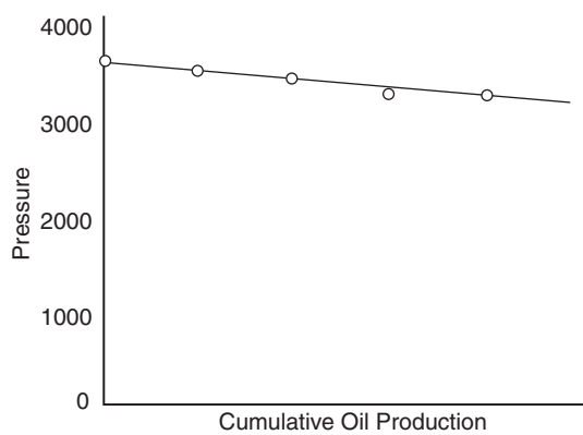
Figure 4.9 Pressure–production history for a water drive reservoir.
