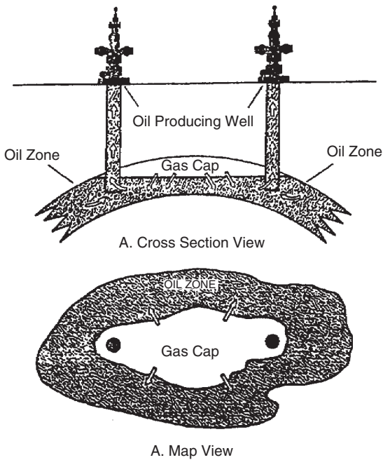
Figure 4.3 Gas cap drive reservoir (After Clark, N.J., Elements of Petroleum Reservoirs , SPE, 1969).
