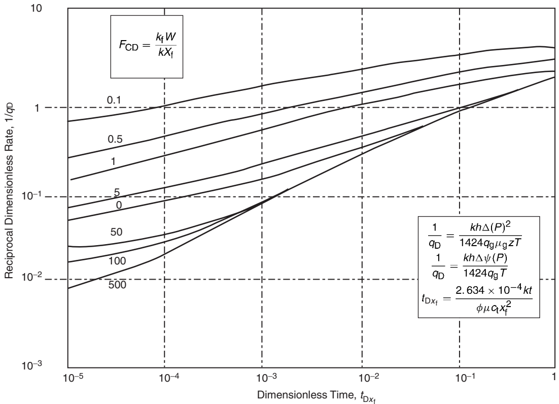
Figure 1.91 Log-log type curves for finite capacity vertical fractures; constant wellbore pressure (After Agarwal et al., 1979).
