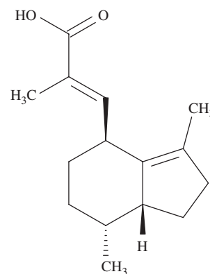
FIGURE 94.2. Chemical structure of valeronic acid.
