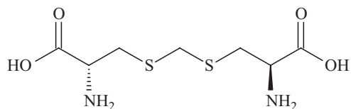
FIGURE 7.1. Chemical structure of djenkol acid.
