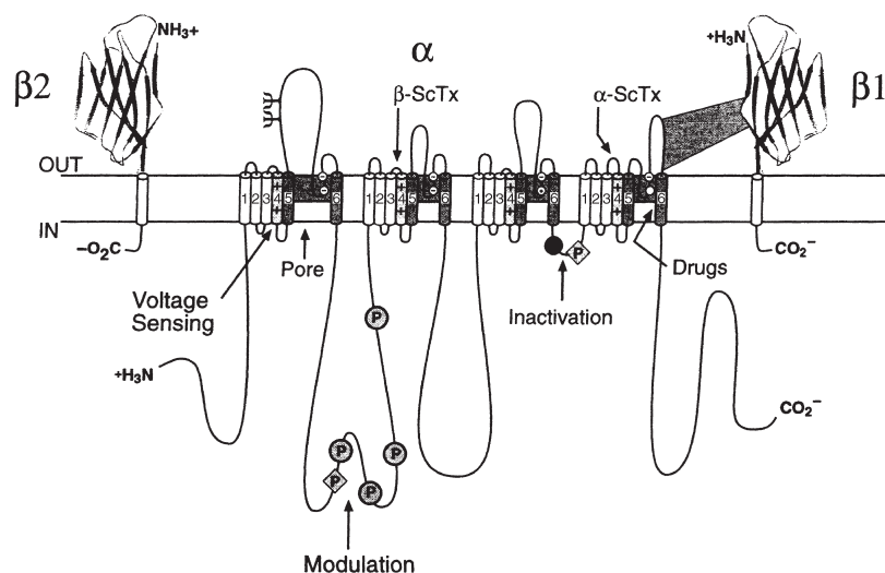
FIGURE 165.2. Structure of voltage-gated Na + channels in mammalian brains. The extracellular domains, \beta 1 and \beta 2 , are folds of \alpha -helical segments. Bold lines represent polypeptide chains. \psi is the probable site of N-linked glycosylation and P represents areas of protein phosphorylation. The lightly shaded S4 segment is the voltage sensor and the dark circle represents the inactivation particle in the inactivation gate loop. The sites of binding of \beta - and \alpha -scorpion toxins are domains II and IV, respectively. From Catterall WA. Molecular mechanisms of gating and drug block of sodium channels. Novartis Found Symp 2002;241:207. Reproduced with permission from John Wiley & Sons Limited.
