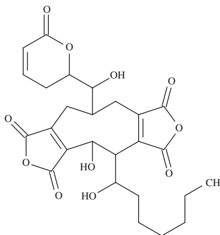
FIGURE 45.8. Chemical structure of rubratoxin B.
