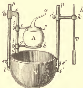
FIG. 18.—Dumas' Method of finding the Specific Gravity of Vapors.
