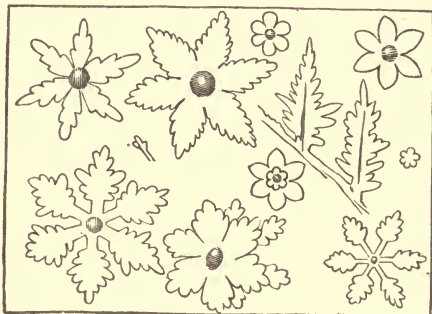
FIG. 10.—Ice-Flowers.
