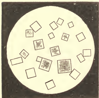
FIG. 23.—Crystals of Potassic Chloride.
