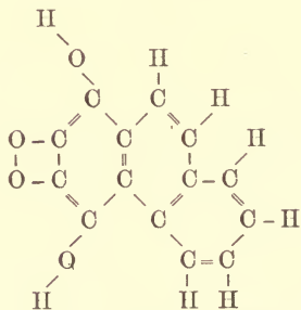
Anthraquinonic Acid (Alizarine).
