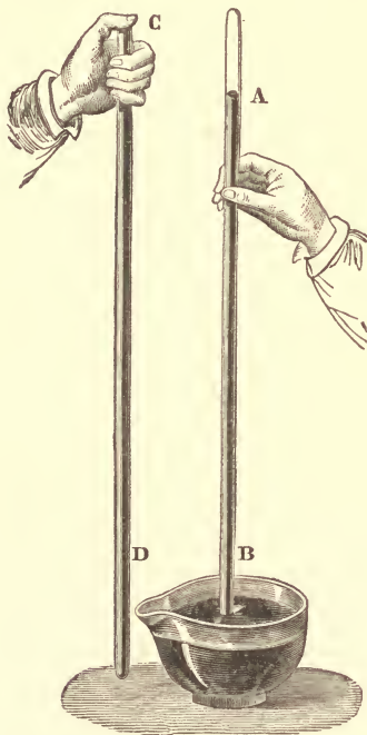
FIG. 20.—Torricelli's Experiment.
