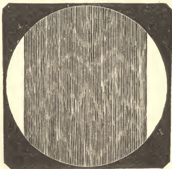
FIG. 3.—Nobert's 19th Band.
