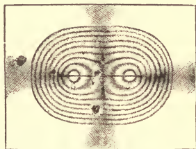
FIG. 15.—Rings, Biaxial Crystals.
