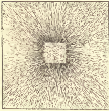
FIG. 12.—Magnetic Curves, one pole.
