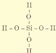
Normal Hydrate.
