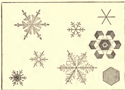
FIG. 11.—Snow-Crystals.
