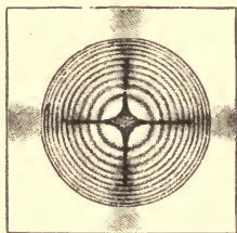
FIG. 14.—Rings, Uniaxial Crystals.
