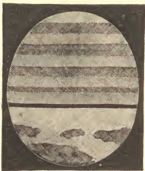
FIG. 4.—Bands on Soap-film.
