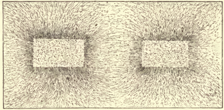
FIG. 13.—Magnetic Curves, two poles.
