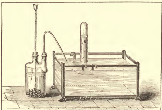
FIG. 22.—Pneumatic Trough, with Two-necked Gas-bottle.
