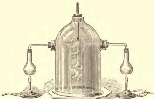
FIG. 26.—Combination of Ammonia and Hydrochloric-Acid Gases.
