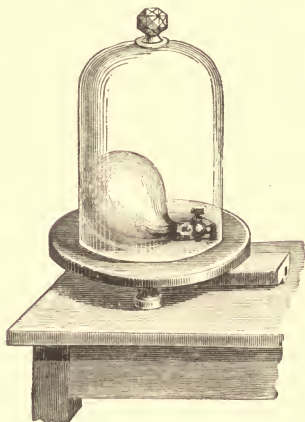
FIG. 6.—Expanding Bag under Air-pump.
