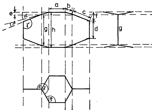
Fig. 1. Geometry of the [2.2]paracyclophane molecule in the crystal. (For numerical values see Table 1)
