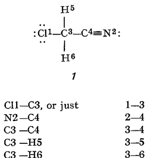
Fig. 1. Connectivity list of 1
