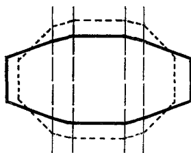
Fig. 3. Schematic representation of the molecular vibration of [2.2]paracyclophane, in which the benzene rings move to and fro in a concertina-like fashion with respect to each other
