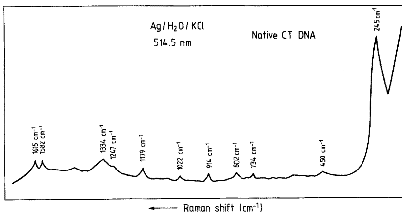
Fig. 12. SERS-spectrum of native CT-DNA. DNA concentration 200 \mu\text{g} \times \text{mL}^{-1} , 0.15 M KCl, 10^{-3} M cacodylate pH 6.8. Laser excitation line 514 nm, laser power at electrode 100 mW. Prior activation of silver electrode by two triangular voltage sweeps between -0.1 and +0.2 V at a sweep rate of 50 \text{ mV s}^{-1}
