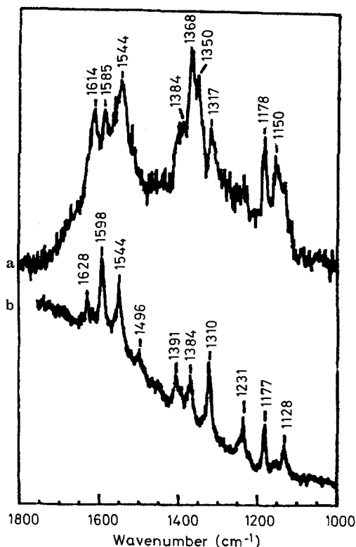
Fig. 34a and b. RR spectra of Pseudomonas aeruginosa cytochrome cd_1 complex, 514.5 nm excitation. a) SERRS spectrum, 3 \times 10^{-6} M in 0.1 M Na_2SO_4 , adsorbed on Ag at -0.6 V vs SCE. Laser power 20 mW; monochromator slit width 2\text{ cm}^{-1} . b) Solution RR spectrum of reduced complex; 5.5 \times 10^{-4} M; laser 20 mW; monochromator slit width 2\text{ cm}^{-1} (Cotton et al., Ref. 21 )
