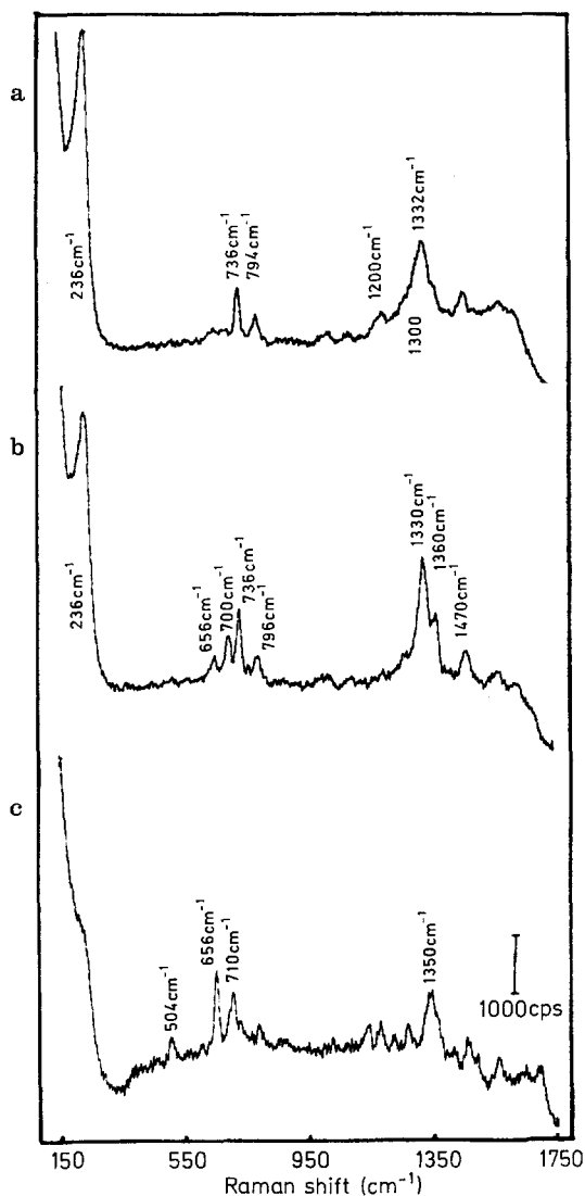
Fig. 17a-c. SERS spectra of native CT-DNA a), methylated CT-DNA (8% MeGua) before b) and after heating at 70^\circ\text{C} c) adsorbed on Ag electrode. Concentration of DNA 200\text{ }\mu\text{g mL}^{-1} , 0.15\text{ M NaCl} , 2 \times 10^{-3}\text{ M Tris} , pH 8, adsorption potential E_s -0.2\text{ V} vs. Ag/AgCl reference electrode (Ref. 41 )
