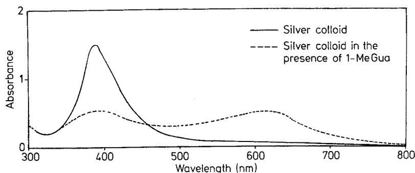
Fig. 4. Absorption spectra of silver sol (solid line) and silver sol in presence of 1-MeGua ( 7 \times 10^{-6} M of 1-MeGua) (broken line).
