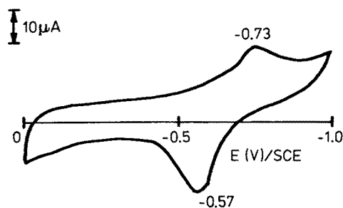
Fig. 30. Cyclic voltammogram for a roughened silver electrode in aqueous (pH 10.5) hemin chloride ( 0.5\text{ mM} ) containing 0.1\text{ M} KCl as supporting electrolyte. Scan rate 100\text{ mV/s} (Sanchez and Spiro, Ref. 188 )
