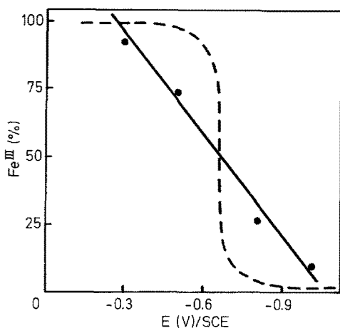
Fig. 31. Fraction of the heme adsorbed from aqueous base remaining as Fe(III) heme versus the electrode potential, as estimated from the intensities of the V_4 SERR bands at 1370\text{ cm}^{-1} Fe(III) and 1360\text{ cm}^{-1} Fe(II). The dotted curve is the expected equilibrium (Nernstian) behavior for a redox couple with a formal potential of -0.65\text{ V} versus SCE (Sanchez and Spiro, Ref. 188 )
