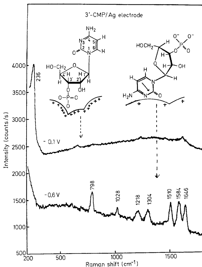
Fig. 8a and b. SERS spectra of cytidine 3'-monophosphate (3'-CMP). 3'-CMP concentration 2 \times 10^{-3} M, 0.15 M KCl, 2 \times 10^{-3} M. Tris buffer (pH 7.2), laser excitation line 514.5 nm, laser power at the electrode 10 mW, prior activation of the silver electrode: 1 \times 5 mCb between -0.1 V and +0.2 V (Ref. 40).
