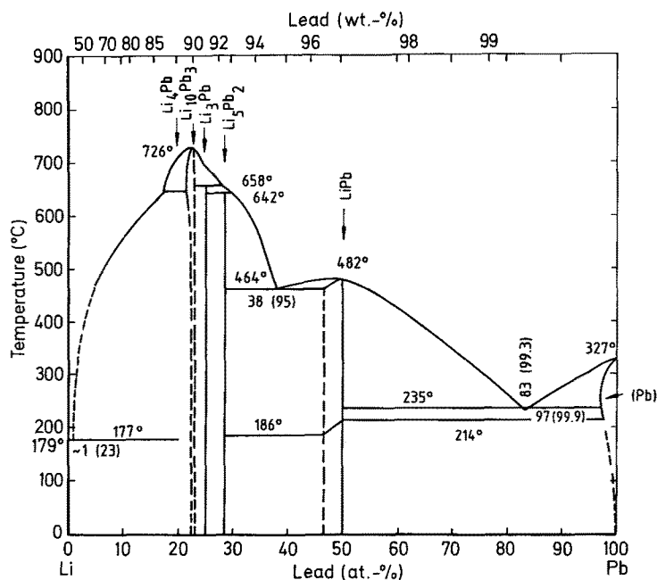
Fig. 13. The simplified Li—Pb phase diagram 74)
