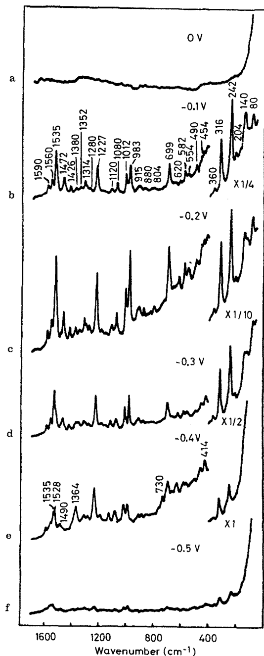
Fig. 27. SERS spectra of TSPP adsorbed on the Ag electrode at different electrode potentials in 0.05 M \text{H}_2\text{SO}_4 . Excitation wavelength: 488.0 nm (20 mW). (A) 0 V; (B) -0.1 V; (C) -0.2 V; (D) -0.3 V; (E) -0.4 V; (F) -0.5 V (versus Ag/AgCl electrode). (Itabashi et al., Ref. 187) )
