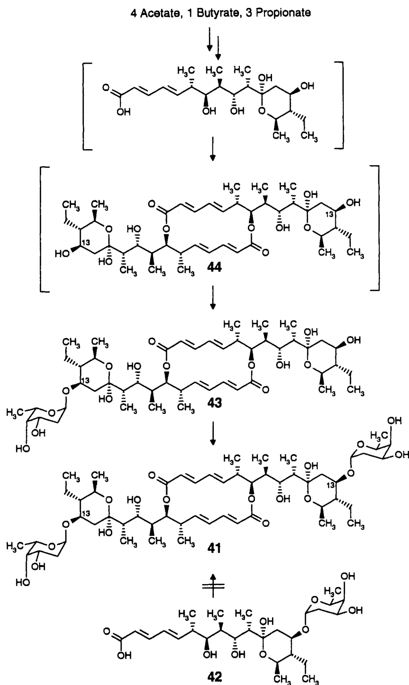
Scheme 16. Biosynthesis of the macrodiolide elaiophyllin (41). The glycosylation steps occur at the very end of the biosynthesis
