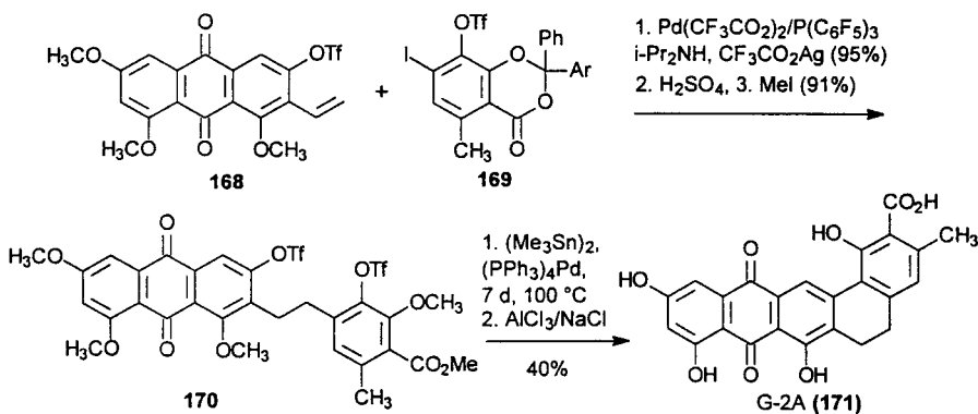
Scheme 43. Synthesis of G-2A (171) using Heck and Stille reactions [125]
