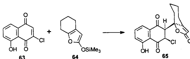
Scheme 18. Michael addition of the siloxyfurane 64 to the naphthoquinone 63 [39]
