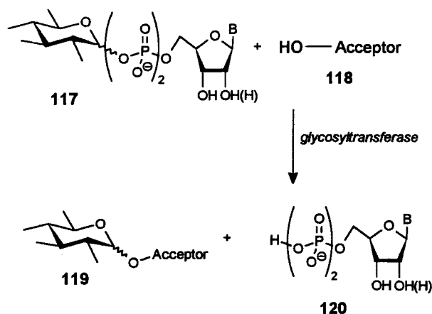
Scheme 40. Enzyme-catalyzed glycosidation
