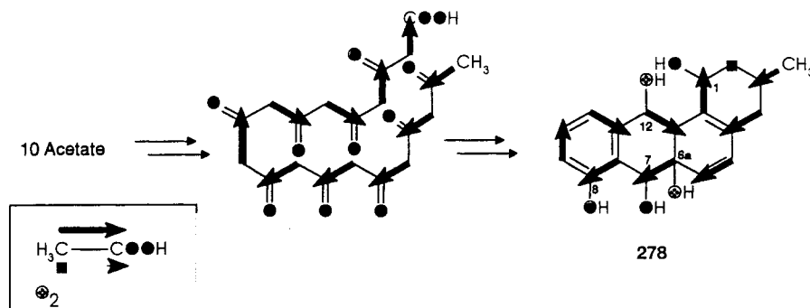
Scheme 59. Typical biosynthetic formation of an angucyclinone, e.g., elmycin D ( 278 ), from acetate and molecular oxygen
