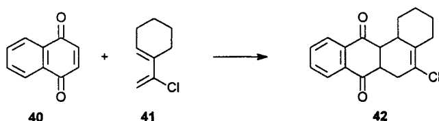
Scheme 11. Construction of a hydrogenated benzo[ a ]anthraquinone by Carothers and Coffman [50]
