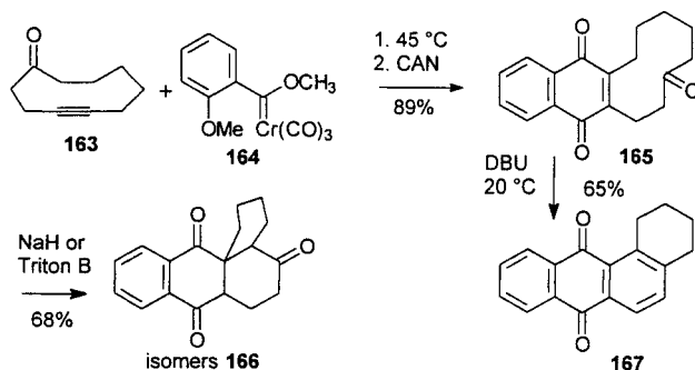
Scheme 42. Use of the Dötz reaction (CAN = ceric ammonium nitrate) in the synthesis of benzo[ a ]anthraquinone 167 [112]
