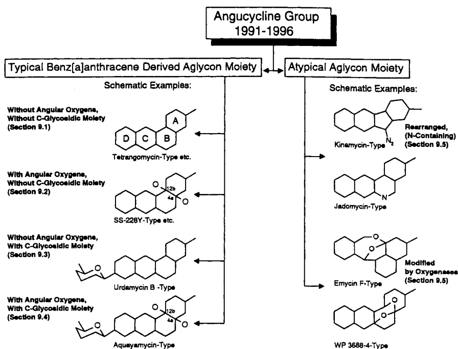
Scheme 50. Biogeneric classification of angucyclines (1991–1996)
