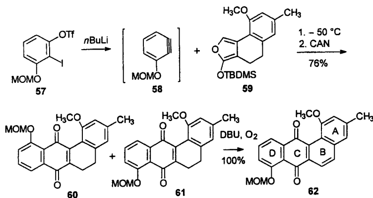
Scheme 17. Diels-Alder reaction of arine 58 with the siloxyfuran 59 [58, 59]
