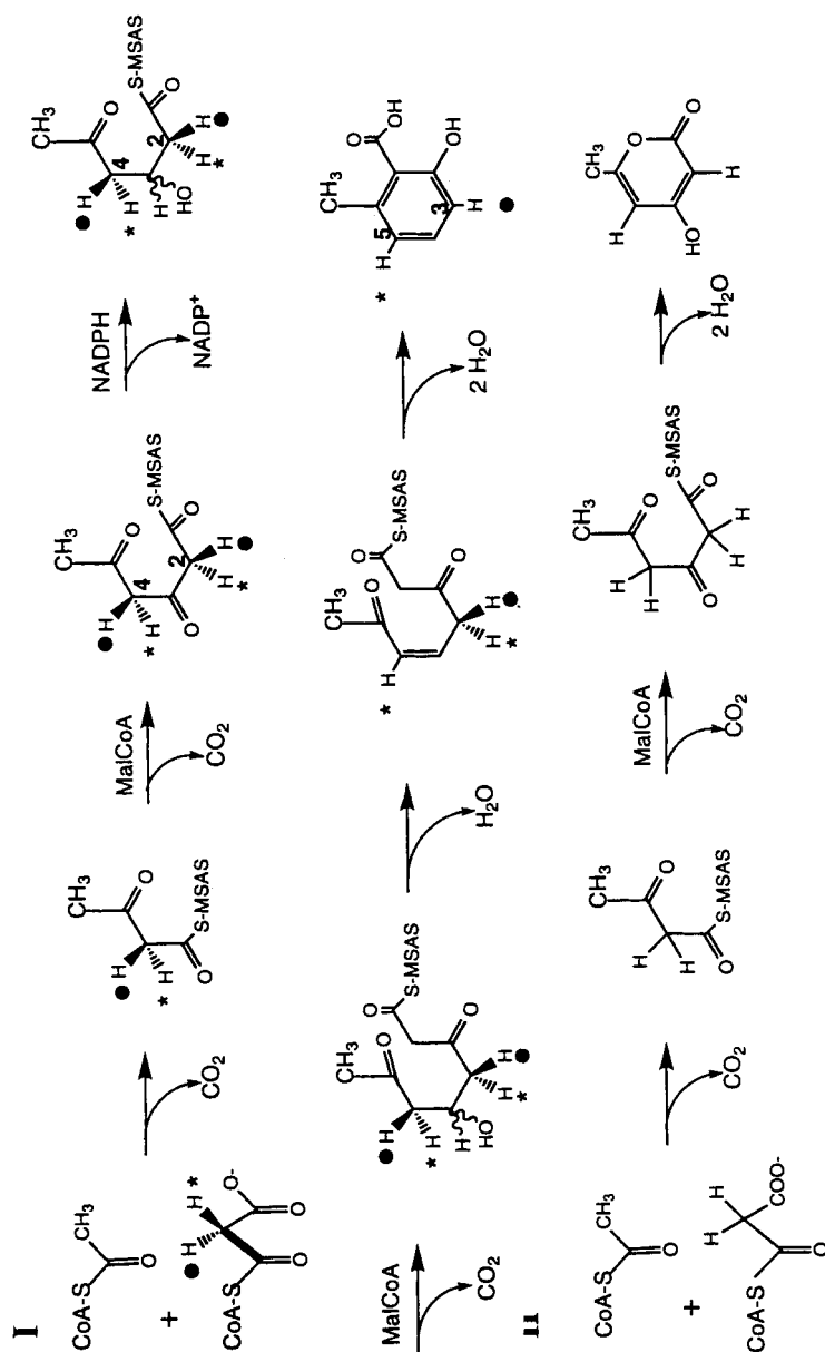
Fig. 5. Biosynthetic pathways for (I) 6-methylsalicylic acid and (II) the triacetic acid lactone. The structures of the intermediates have not been identified. The stereochemical course of the propyl carbons (C-2 and C-4 in the triketide intermediate, C-3 and C-5 in 6-MSA) was investigated using ( R )- and ( S )- [ 1\text{-}^{13}\text{C} , 2\text{-}^2\text{H} ]malonic acid extender substrate analogs in a coupled assay with 6-MSAS and succinyl-CoA transferase. The distinguishable hydrogens originating from the chiral malonyl CoA are labeled with * and H . Triacetic acid lactone synthesis is catalyzed by 6-MSAS in the absence NADPH
