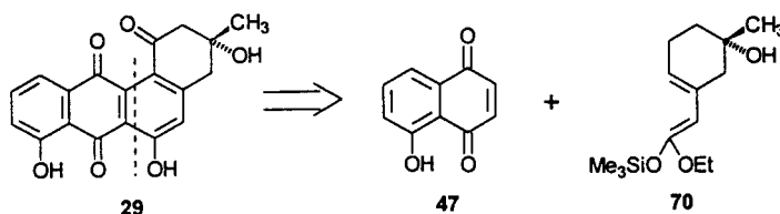
Scheme 20. Retrosynthetic analysis of rabelomycin (29) synthesis [68, 39]
