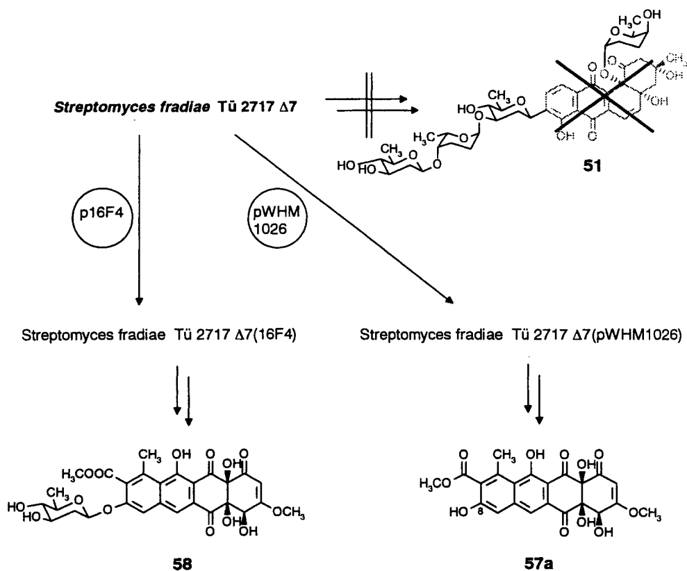
Scheme 23. Biosynthesis of olivosyltetracenomycin (58) by the construction strain S. fradiae Tü2717Δ7(16F4). Substitution of the elm genes (cosmid 164F) by the tcm genes (plasmid pWHM1026) resulted in absolutely no production of 58, although the same aglycon, 8-O-demethyltetracenomycin C (57a), is produced in high yields
