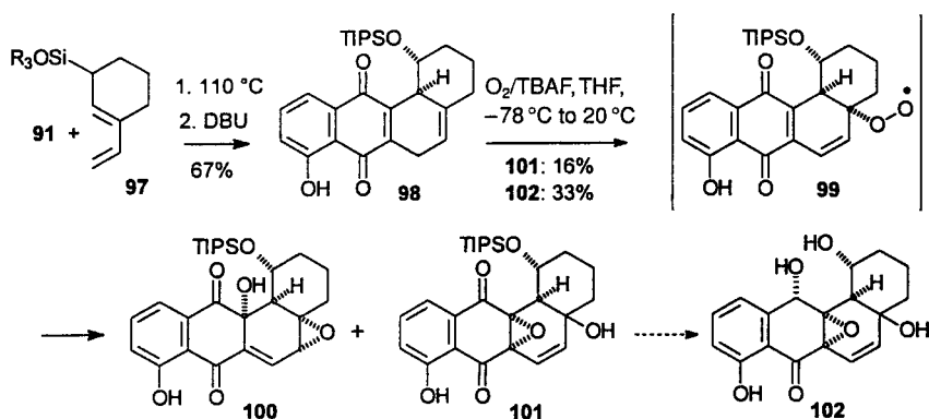
Scheme 28. Stereocontrolled assembly of the SF 2315 B ring system by air oxidation of adduct 98 [84]
