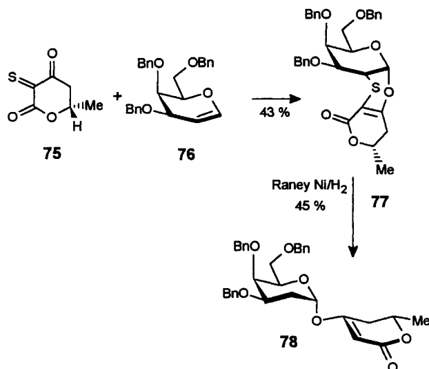
Scheme 31. Preparation of 2-deoxyglycosides using a cycloaddition strategy
