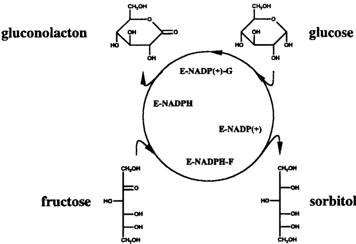
Fig. 6. Reaction of a glucose-fructose oxidoreductase from Zymomonas mobilis
