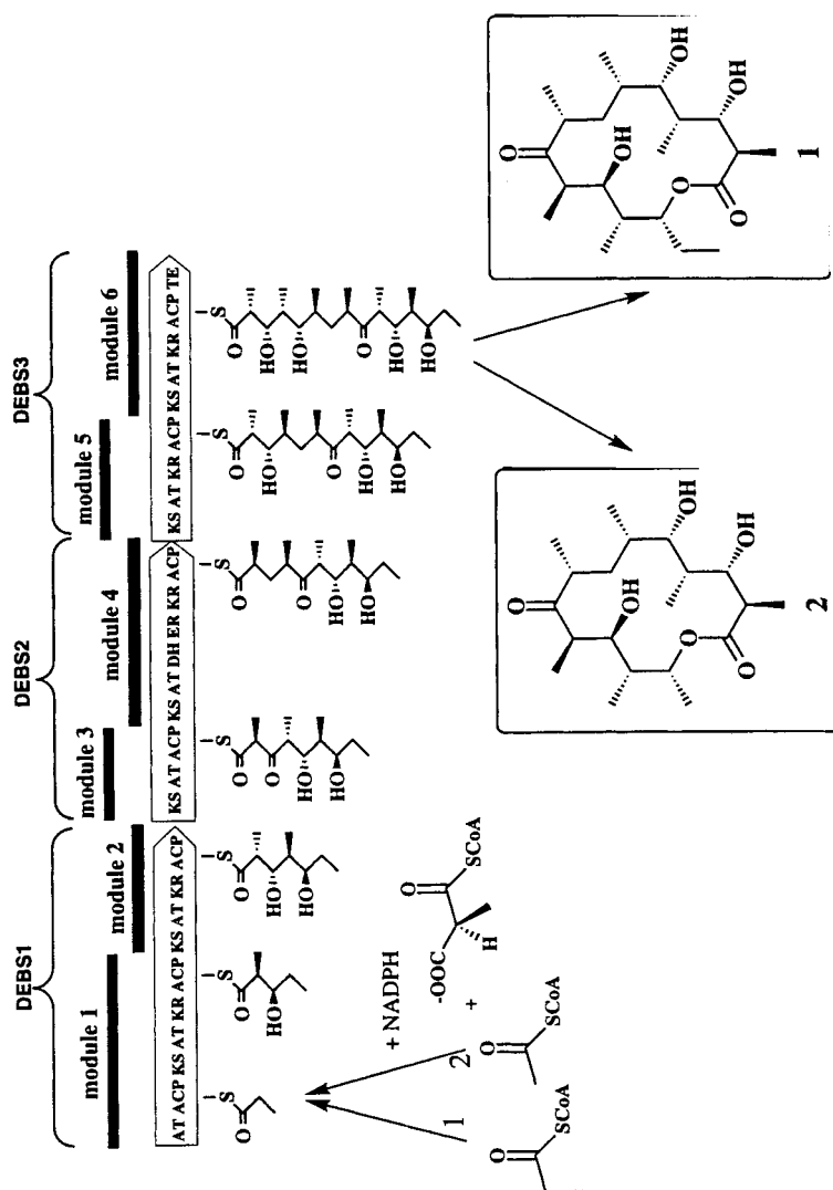
Fig. 7. Model for the modular organization of 6-deoxyerythronolide B synthase (DEBS) and the biosynthesis of 6-deoxyerythronolide B (1) and 8,8a-deoxyoleandolide (2) by DEBS [208]. Each of the six modules accounts for the one polyketide chain extension and \beta -ketoreduction cycle. The active sites are designated as follows: acyltransferase (AT), \beta -ketoacyl-ACP transferase (KS), acyl carrier protein (ACP), \beta -ketoreductase (KR), dehydratase (DH), enoylreductase (ER), and thioesterase (TE).
