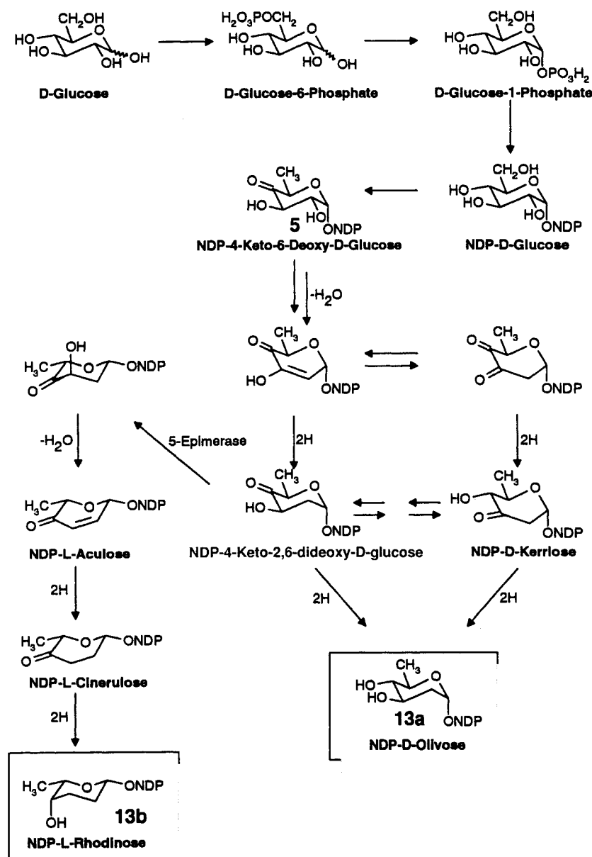
Scheme 6b. Favored hypothetical deoxygenation pathways to the deoxysugars of landomycin A, NDP-D-olivose (13a) and NDP-L-rhodinose (13b)
