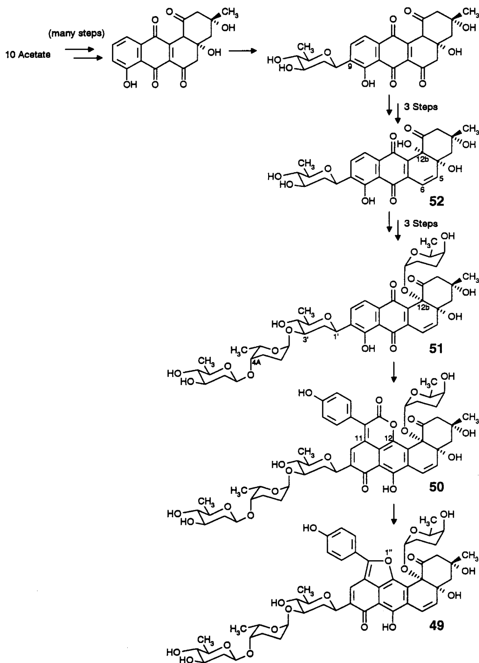
Scheme 19. The last steps of urdamycin biosynthesis: The first (C-) glycosylation step occurs long before the end of the biosynthetic cascade, with the final product urdamycin H (49)
