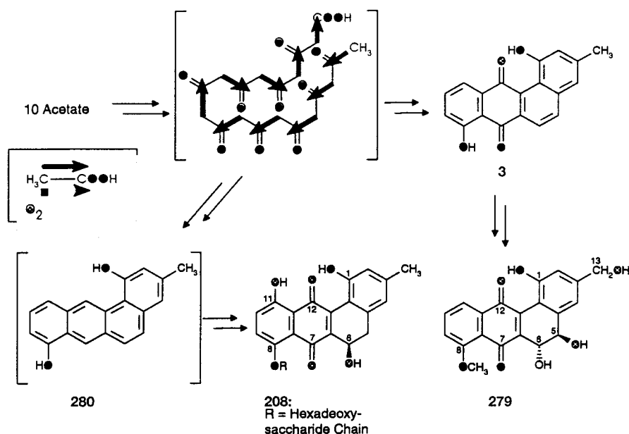
Scheme 60. The unexpected biogenetic origin of oxygen atoms in landomycin A (208) and PD 116740 (279) indicates prearomatic deoxygenation steps
