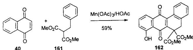
Scheme 41. Manganese (III)-induced radical addition to 1,4-naphthoquinone ( 40 ) [111]
