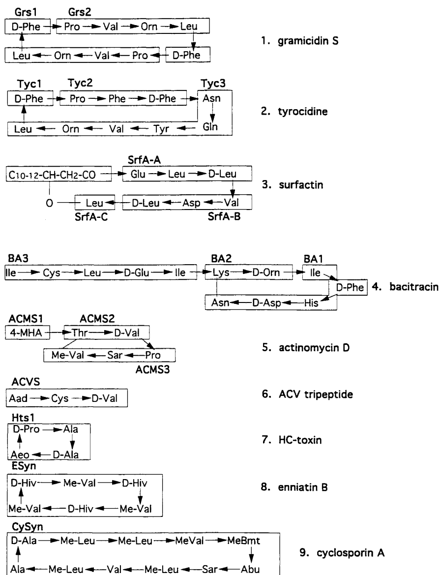
Fig. 10. Structures of nonribosomally synthesized peptides of bacterial origin (1–6) and fungal origin (7–9). Me , N -methylated peptide bond; Orn , ornithine; 4-MHA , 4-methyl-3-hydroxyanthranilic acid; Aad , aminoadipic acid; Aeo , 2-amino-9,10-epoxy-8-oxodecanoic acid; D-Hiv , D -hydroxyisovaleric acid; Bmt , (4 R )-4-[( E )-2-butenyl]-4-methyl-L-threonine; Abu , \alpha -aminoisobutyric acid; Sar , sarcosine. The boxes signify gene products for peptide synthetases composed of modules which activate and process the indicated amino acids
