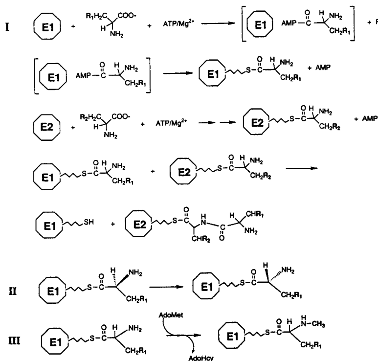
Fig. 11. Reaction scheme for (I) substrate amino acid activations and dipeptide formation, (II) racemization, and (III) N -methylation. E1 and E2 are symbols for enzyme activities (from peptide synthetase modules) either on the same or separate proteins. R1 and R2 are amino acid side chains, where R1 is part of the first amino acid activated by the peptide synthetase indicates the linkage between 4'-phosphopantetheinylated enzyme and the substrate or peptide intermediate. AdoMet , S-adenosylmethionine; AdoHcy , S-adenosylhomocysteine
