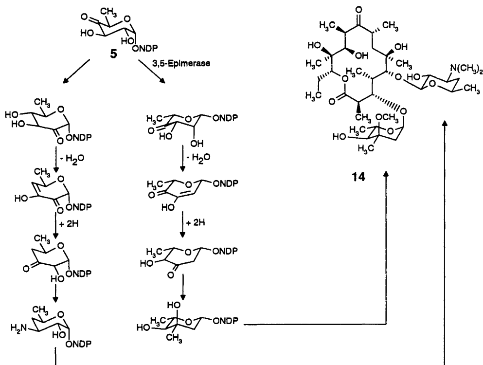
Scheme 7. Hypothetical deoxygenation pathways to the two deoxysugar moieties in erythromycin A (14)
