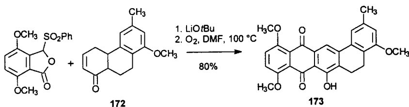
Scheme 44. Sulphonylphthalide condensation with enone 172 to construct a benzo[ a ]naphthacene-8,13-dione 173 [126]
