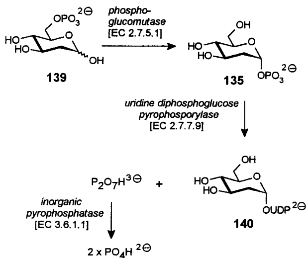
Scheme 46. Enzymatic synthesis of UDP-2-deoxy-D-glucose 140
