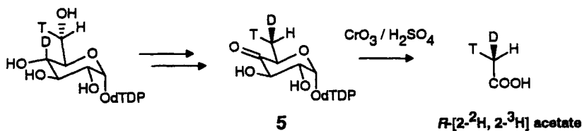
Scheme 2. Generation and stereochemical course of NDP-4-keto-6-deoxyglucose (5)
