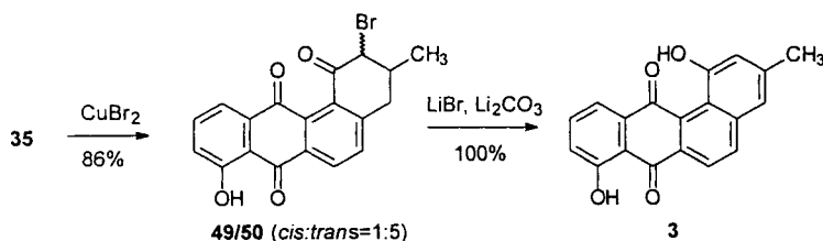
Scheme 14. Aromatization of ochromycinone (35) to tetrangulol (3) via bromides 49 [54]
