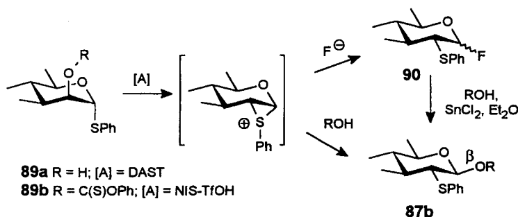
Scheme 35. Arylthio-migration of thioglycosides and \beta -glycosidation
