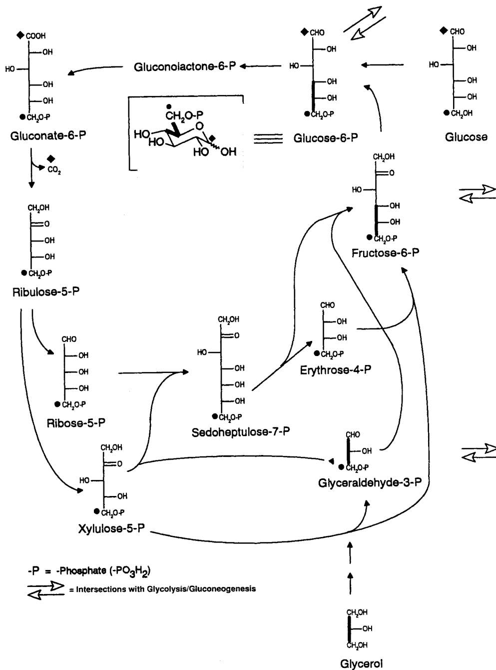
Scheme 25. ^{13}\text{C} labels in the pentose phosphate cycle
