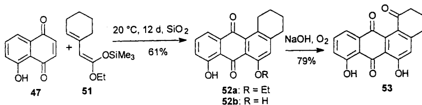
Scheme 15. Diels-Alder reaction using ketene acetal 51 and base-catalyzed air oxidation at C-1 [47]
