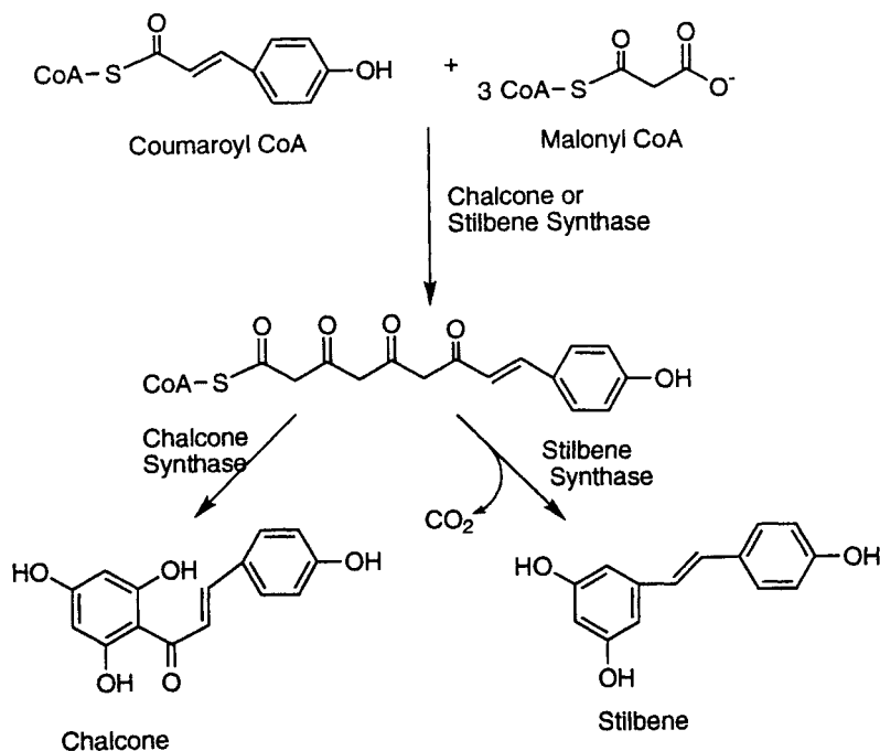
Fig. 6. Reactions catalyzed by chalcone and stilbene synthases. Each enzyme condenses three malonyl CoA extender units onto p -coumaroyl-CoA. Stilbene synthases catalyze an additional decarboxylation, resulting in a different pattern of cyclization for chalcone versus stilbene products
