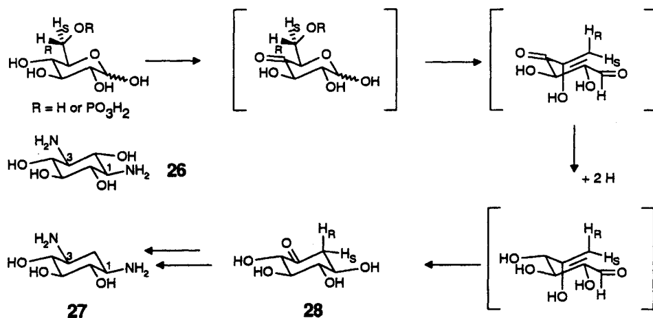
Scheme 12. 5-Deoxygenation during the biosynthesis of 2-deoxystreptamine (27; the core moiety of neomycin 25, streptamine 26 is its analog in streptomycin 24) through transamination of the intermediate 2-deoxy- scyllo -inosose (28). Note that C-5 of glucose becomes C-3 of 26 and 27
