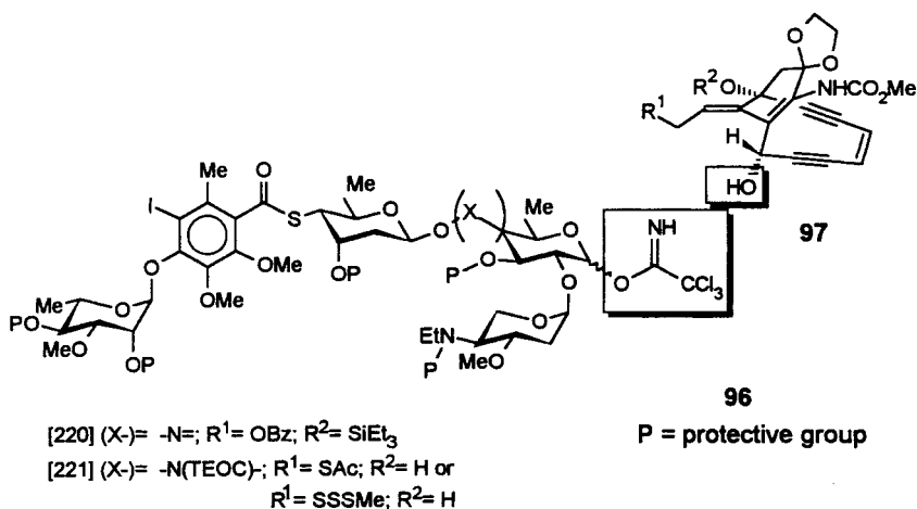
Scheme 37. Synthesis of calicheamicin \gamma_1^I (65): The appropriately protected trichloroacetimidate derivative (96), and the calicheamicinone \gamma_1^I precursor (97) are shown
