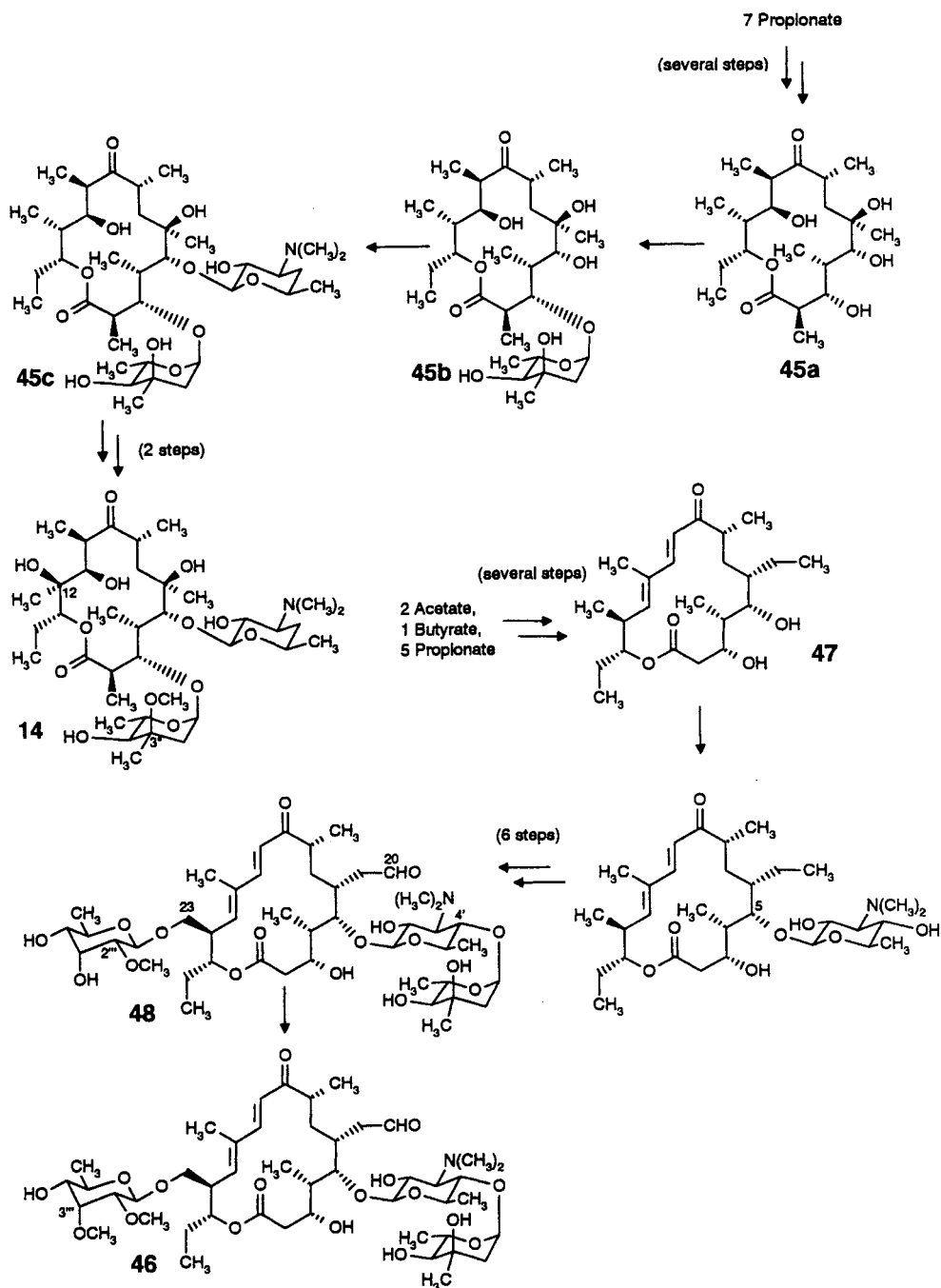
Scheme 18. The biosyntheses of erythromycin A (14) and tylosin (46). Glycosylation steps occur prior to the complete biosyntheses of the aglyca
