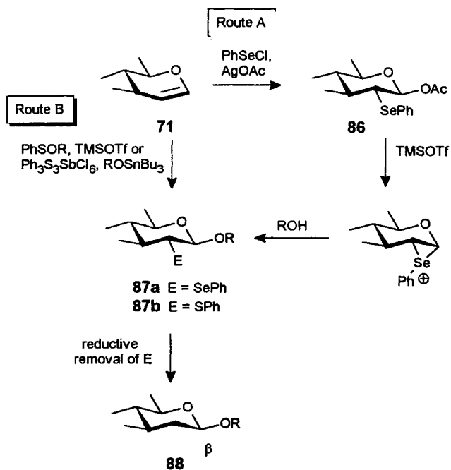
Scheme 34. Routes to 2-deoxy- \beta -glycosides from glycals
