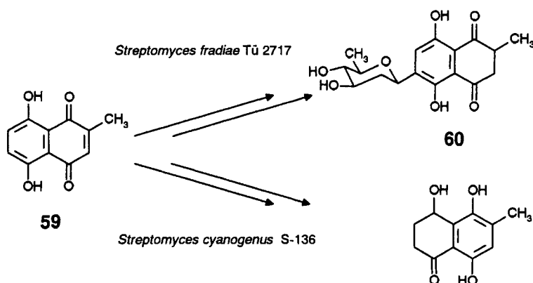
Scheme 22. C-glycosylation and reduction of methylnaphthazarine (59) by Streptomyces fradiae Tü2717 vs reduction only by S. cyanogenus S-136
