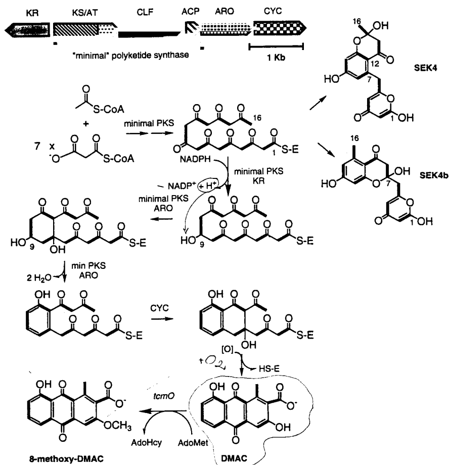
Fig. 4. Polyketide biosynthesis by gene products of the act PKS cluster. Presence of the KS/AT, CLF, and ACP is sufficient for the production of two 16-carbon polyketides, SEK4 and SEK4b both in vivo [103] and in vitro [107]. In the presence of the act ketoreductase (KR), aromatase (ARO) and cyclase (CYC), the octaketide intermediate is converted into DMAC. DMAC can be converted into 8-methoxy DMAC both in vivo and in vitro through the S-adenosylmethionine (Adomet)-dependent action of the tcmO methyltransferase [207]
