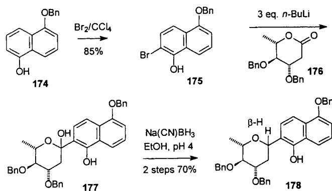
Scheme 45. C-glycoside synthesis by reaction of sugar lactones with lithium aryls [137]
