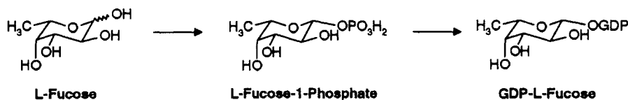
Scheme 26. “Short activation” of L-fucose
