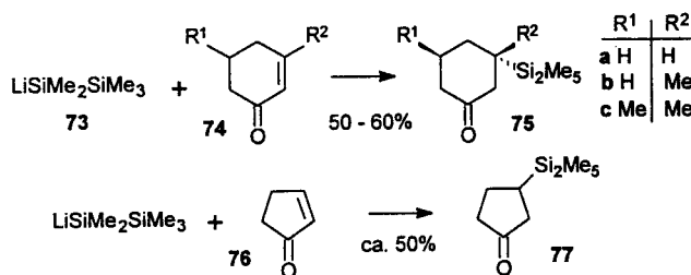
Scheme 22. Conjugate addition of lithium pentamethyldisilane (73) to cyclic enones [68]
