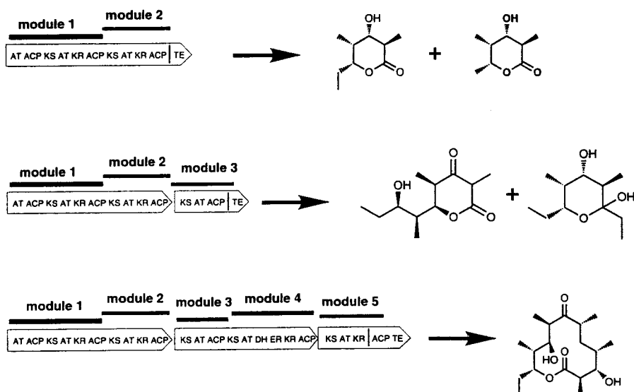
Fig. 8. Polyketides produced by S. coelicolor strains expressing truncated forms of DEBS [157, 158]. Structures were determined by isotope enrichment and NMR spectroscopy
