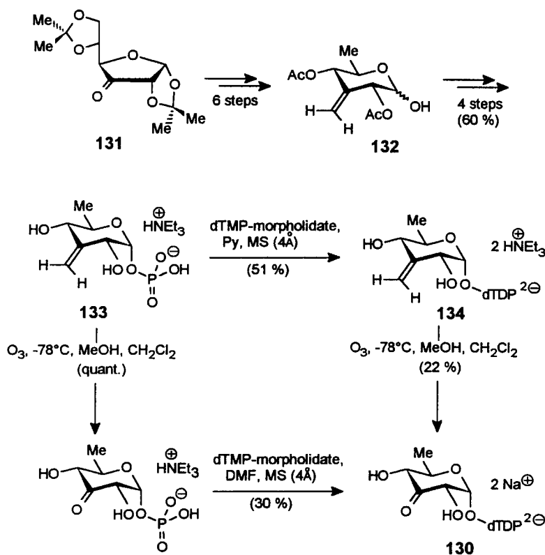
Scheme 44. Chemical synthesis of dTDP-6-deoxy-D-3-hexulose (130)
