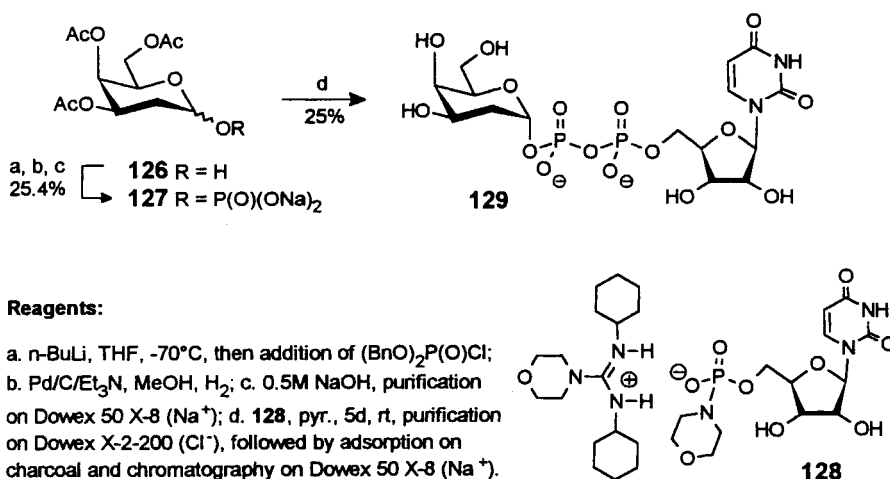
Scheme 43. First chemical synthesis of a NDP-2-deoxysugar
