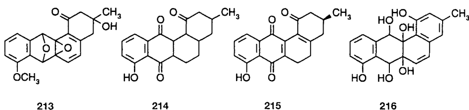
Scheme 51. Further angucyclinones of the tetrangomycin type with unusual oxygenations or reductions
