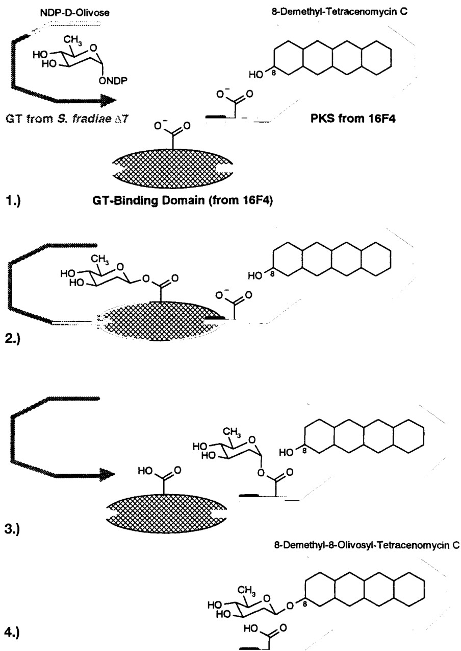
Scheme 24. Hypothesis regarding a glycosyl transfer supporting “domain” in cosmid 16F4
