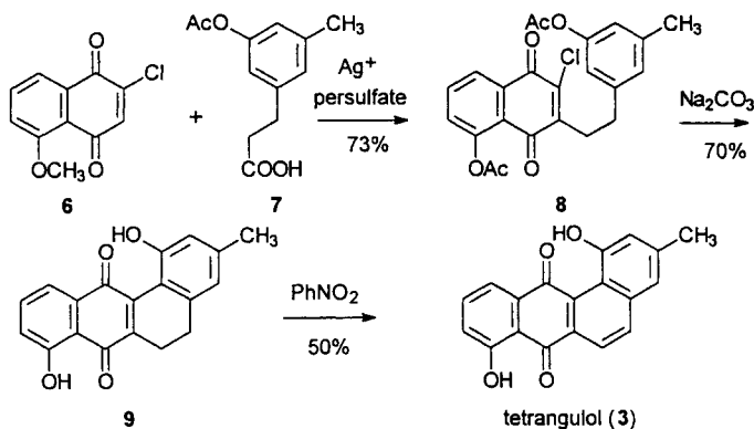
Scheme 3. Synthesis of tetrangulol (3) by Brown and Thomson [18] using a Michael reaction
