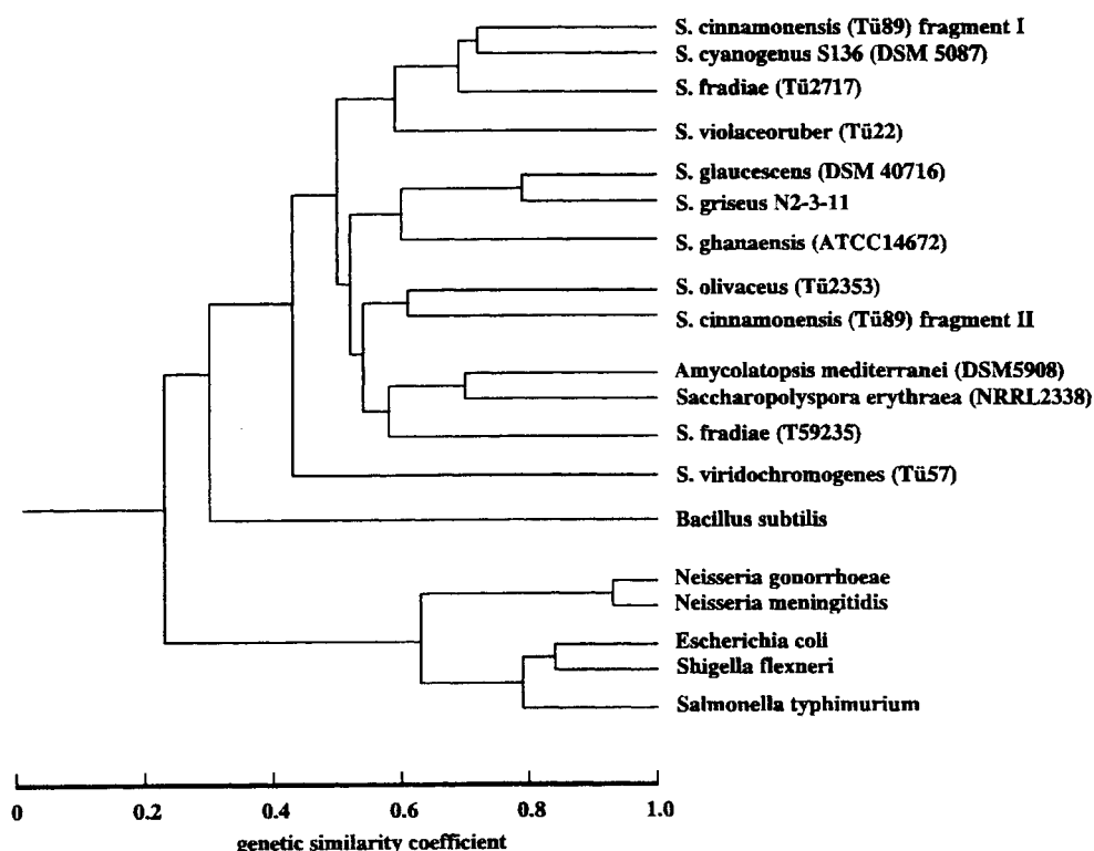
Fig. 2. Phylogenetic trees are based on genetic similarities. The sequences were taken from the following sources: S. cinnamomensis (Tü89) fragment 1 (EMBL X97834); S. cyanogenus S136 (DSM 5087) (EMBL X97833); S. fradiae (Tü2717) (EMBL X97836); S. violaceoruber (Tü22) (gpL37334); S. glaucescens (DSM 40716) (EMBL X97837); S. griseus (N2-3-11) (sp P29782); S. olivaceus (Tü2353) (EMBL X97838); S. cinnamomensis (Tü89) fragment 2 (EMBL X97835); Amycolatopsis mediterranei (DSM 5098) (EMBL X97861); Saccharopolyspora erythraea (NRRL 2338) (gp L37354); S. fradiae (T59235) (gp U08223); S. viridochromogenes (Tü57) (EMBL X98039); Bacillus subtilis (sp P39630); Neisseria gonorrhoeae (sp P37761); N. meningitidis (gp L09188); E. coli (gp U23775); Shigella flexneri (sp P37777); S. typhimurium (sp P26391)
