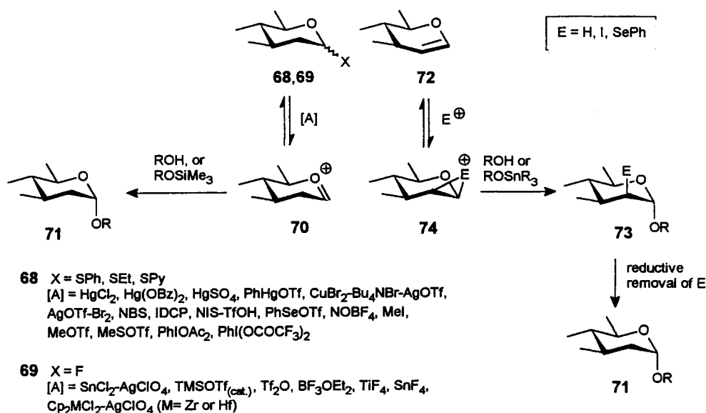
Scheme 30. Strategies for the chemical synthesis of 2-deoxy- \alpha -glycosides
