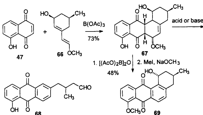
Scheme 19. Synthesis of racemic epi -rubiginone \text{B}_1 ( 69 ) by Diels-Alder reaction [62]
