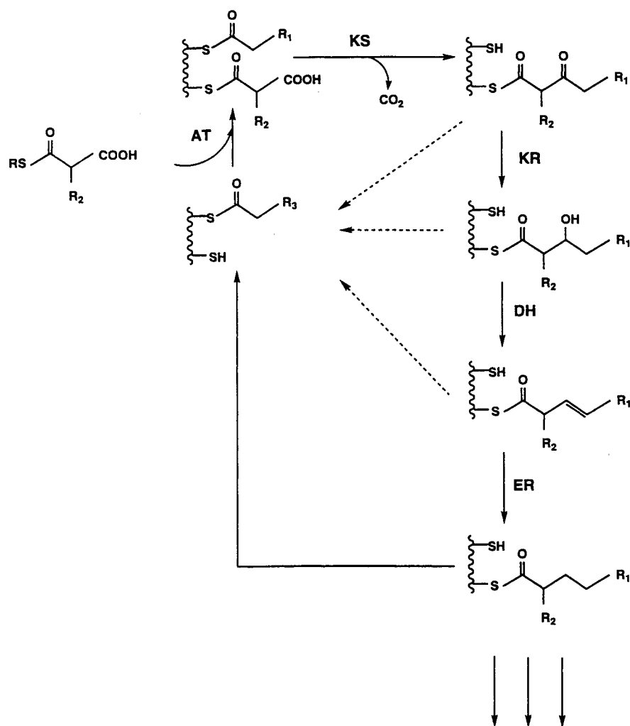
Fig. 1. The overall catalytic cycle of polyketide synthases. Within this biosynthetic scheme, different polyketide synthases can show variability with regard to the length of the polyketide chain, the choice of monomer incorporated at each step, the degree of reduction of each \beta -keto group, and the stereochemistry at each chiral center. For example, the dashed arrows illustrate how the degree of \beta -ketoreduction can vary at any given carbonyl
