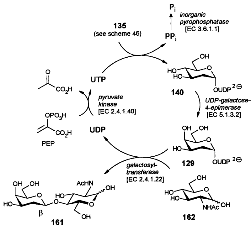
Scheme 49. Enzymatic Synthesis of 2'-Deoxy-N-acetylactosamine 161
