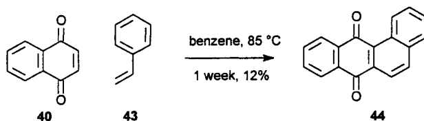
Scheme 12. Synthesis of benzo[ a ]anthraquinone by Diels-Alder reaction using styrene as the diene [51]
