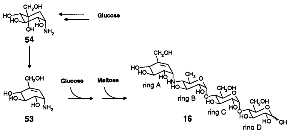
Scheme 20a, b. Disaccharide transfers are thought to be involved in the biosynthesis of acarbose (16, transfer of maltose) and landomycin A (12, transfer of diolivoside units)
