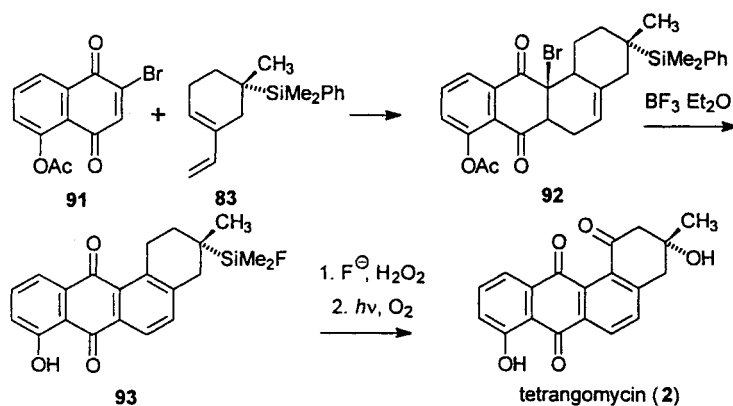
Scheme 26. Synthesis of tetrangomycin ( 2 ) by Diels-Alder reaction [73]
