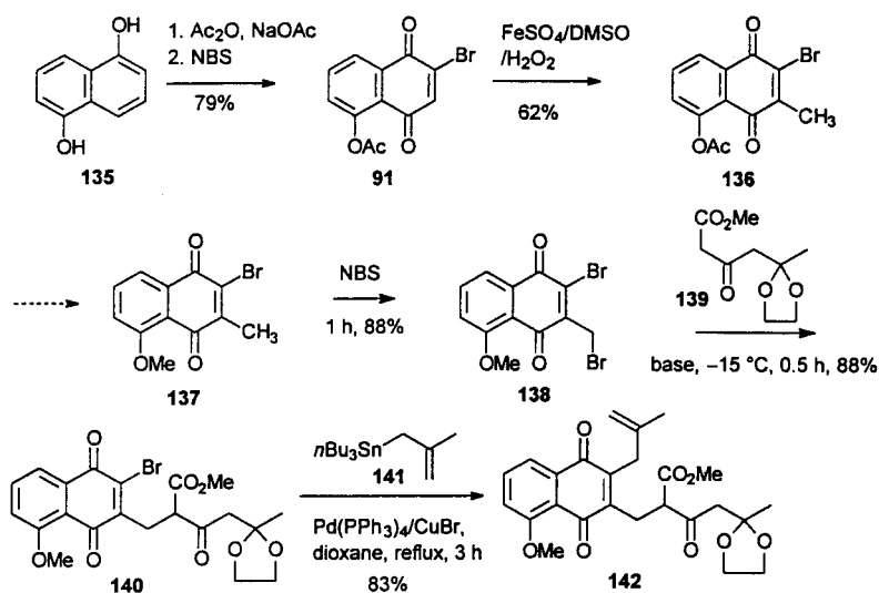
Scheme 36. Attachment of two side chains on the 1,4-naphthoquinone core [86]
