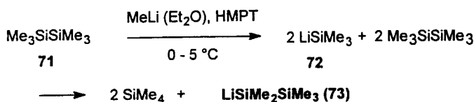
Scheme 21. Formation of lithium pentamethyldisilane (73) by reaction of \text{Si}_2\text{Me}_6 (71) with \text{LiMe} [68, 39]
