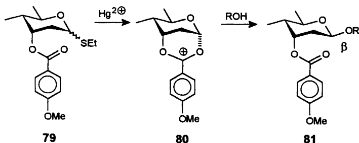
Scheme 32. 2-Deoxy- \beta -glycosides by 1,3 achimeric assistance
