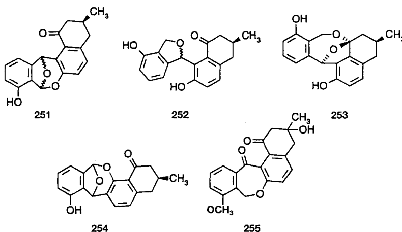
Scheme 55. Novel, through oxygenases modified, angucyclinones: emycins D–G (251–254)
