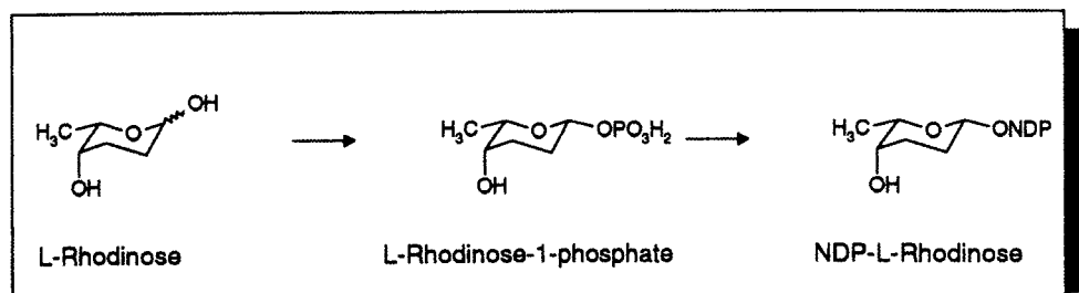
Scheme 27. Successful incorporation of [2, 3- 2 H 2 ]-L-rhodinose [121] into landomycin A (12) provides evidence for a short activation pathway
