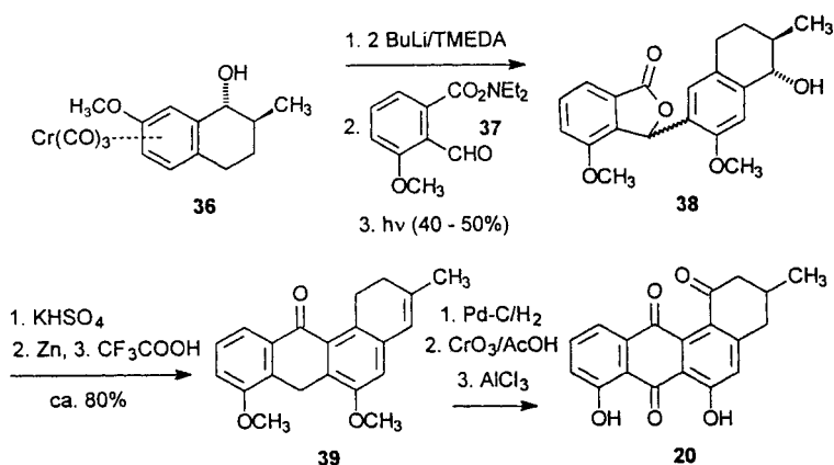
Scheme 10. Synthesis of 3-deoxyrabelomycin (20) by Uemura et al. [48, 49]
