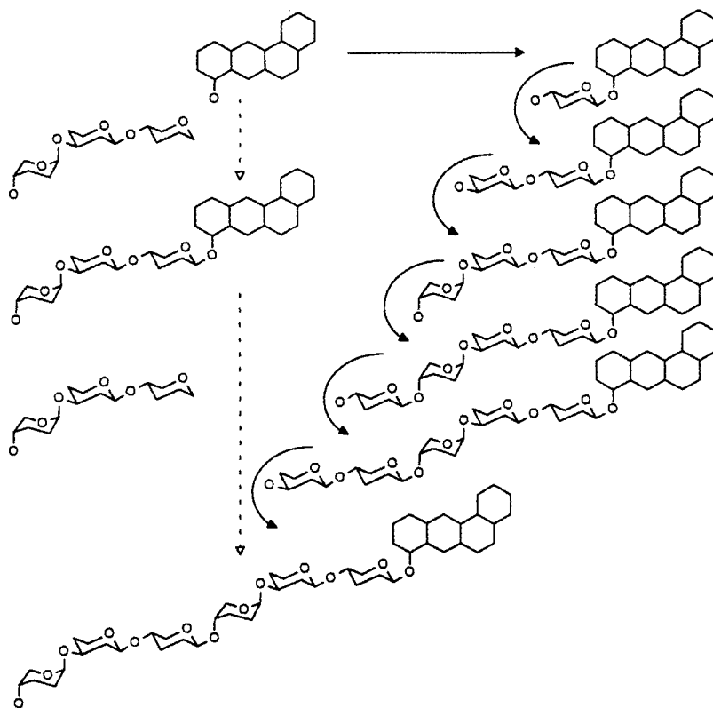
Scheme 65. Alternatives for the biosynthetic assembly of the glycan chain of landomycin A (208); the alternative depicted on the right side ( solid arrows ) is correct
