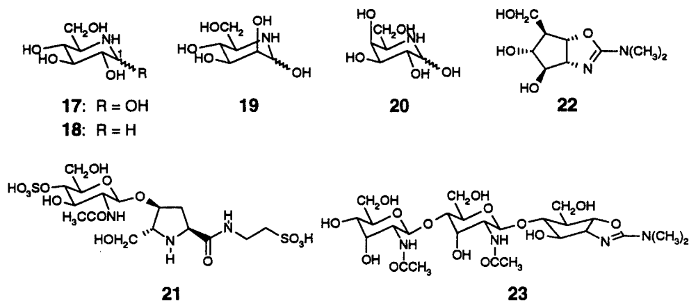
Scheme 9. 5-Deoxysugars: The 5-amino-5-deoxysugars (piperidinoses) nojirimycin (17), 1-deoxynojirimycin (18), mannojinirimycin (19) and galactostatin (20). The tetrahydropyrrol moiety of bulgecin A (21) and the allosamizoline unit 22 of allosamidine (23) can also be considered as 5-deoxysugars. The derivation of 22 from the pool has already been proven
