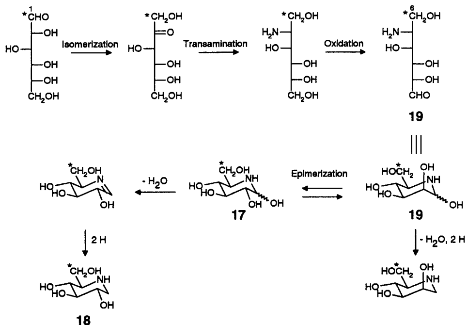
Scheme 10. Biosynthetic formation of 1-deoxynojirimycin (18) and mannojinirimycin (19). Note the “inversion” of the label (the 1-label becomes a 6-label), i. e., the “5-deoxygenation” is really a 2-deoxygenation
