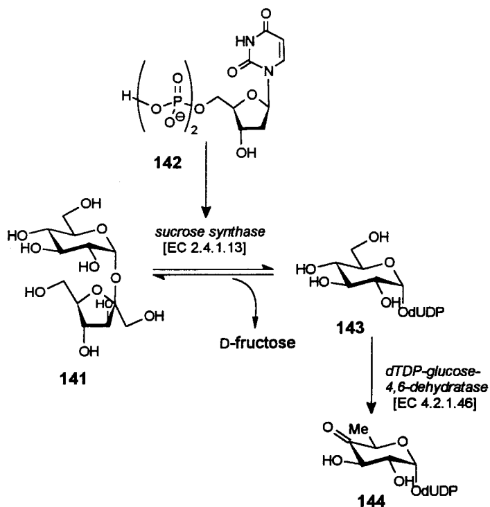
Scheme 47. Enzymatic synthesis of dUDP-6-deoxy-4-hexulose 144 from sucrose 141
