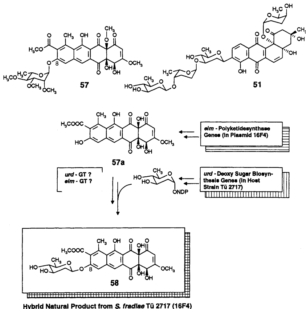
Scheme 21. The biosynthetic formation of the hybrid antibiotic 8- \alpha -D-oliviosyl-8-demethyl-tetracenomycin C (58) depends on genes from both parent organisms: The elloramycin (57) producer Streptomyces olivaceus Tü2353 provides the aglycon moiety ( elm genes), the urdamycin (51) producer Streptomyces fradiae Tü2717 the deoxysugar moiety ( urd genes). The origin of the combining glycosyltransferase (GT) is unclear
