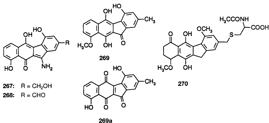
Scheme 57. Further novel benzo[ b ]fluorene antibiotics
