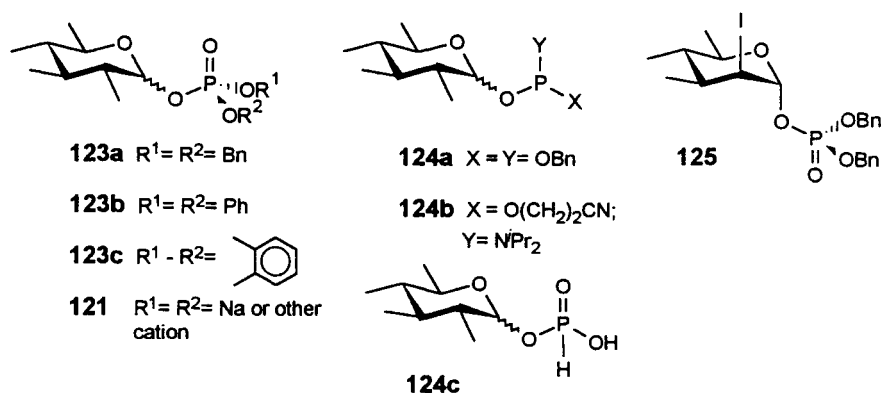
Scheme 42. Strategies for the synthesis of glycosyl 1-phosphates
