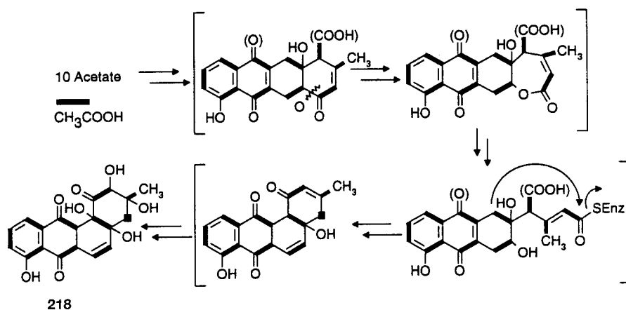
Scheme 61. Biosynthetic studies on PD116198 (218) reveal an unusual rearrangement of an anthracyclinone into an angucyclinone, caused by an oxygenase
