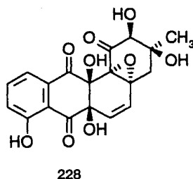
Scheme 53. Compound 228 (WP 3688-3), a novel angucyclinone exhibiting an unusual 4a, 12b epoxide
