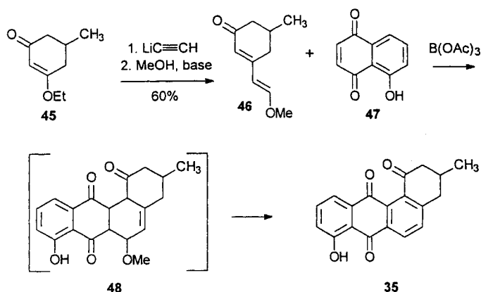
Scheme 13. Diels-Alder approach to ochromycinone (35) [53]
