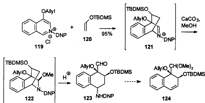
Scheme 32. Synthesis of the protected enediol 124 by Bradsher cycloaddition [94]
