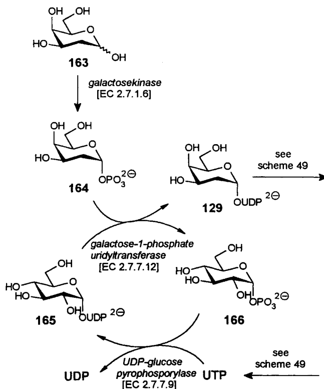
Scheme 50. Modified enzymatic route to UDP-2-desoxy-D-galactose 129
