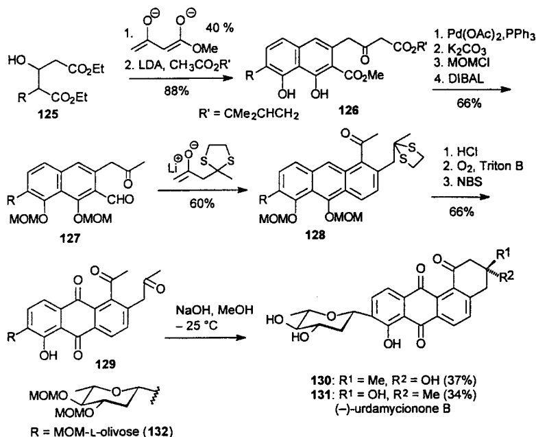
Scheme 34. Biomimetic-type synthesis of (–)-urdamycinone B ( 131 ) by Yamaguchi et al. [97]
