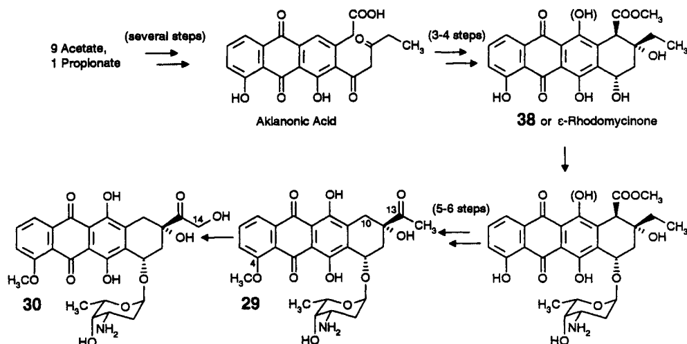
Scheme 17. The biosynthesis of adriamycin (30), demonstrating that glucosyl transfer can occur relatively early in the biosynthetic process
