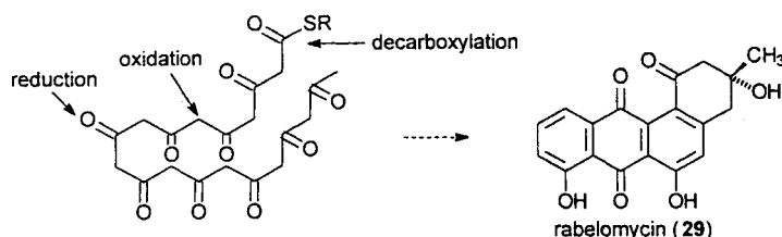
Scheme 33. Postulated decaketide cyclization to angucyclines [3]
