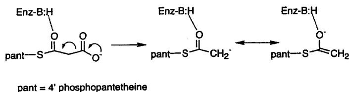
Fig. 3. Decarboxylation of malonyl CoA to create the resonance-stabilized carbanion that is the nucleophilic species of the condensation reaction. A hypothetical interaction with a neutral (as shown) or positively charged basic group on the enzyme is indicated [51, 54]. Although the interaction is shown as a hydrogen bond, an equally feasible mechanism involves complete transfer of the proton
