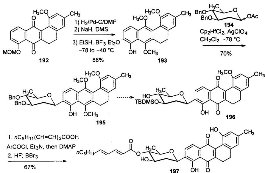
Scheme 49. Total synthesis of the antibiotic C104 by Suzuki et al. [58]
