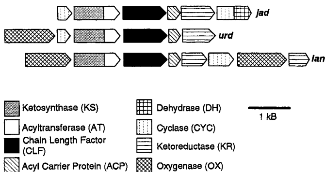
Scheme 62. Genes coding for the polyketide synthases of angucyclinones
