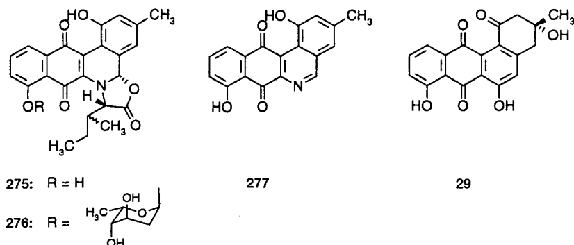
Scheme 58. Jadomycins A,B (275, 276) and their biosynthetic intermediate rabelomycin (29)
