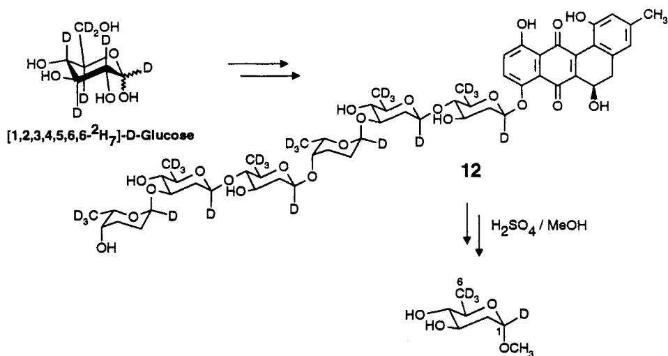
Scheme 6a. Feeding experiment with [U\text{-}^2\text{H}_7] glucose on landomycin A ( 12 ). Only the 1- and 6-positions show detectable amounts of ^2\text{H} label
