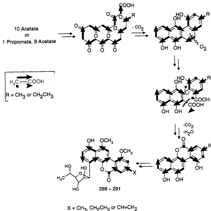
Scheme 69. Biosynthetic formation of the gilvocarcins via an angucyclinone. As in Scheme 66, the key biosynthetic step is an oxidative 5,6-bond cleavage
