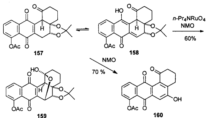
Scheme 40. Mechanism of NMO-oxidation of tetrahydroanthraquinones 157/158 [85]
