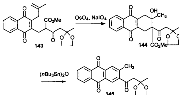
Scheme 37. Linear cyclization of ketoester 143 [86]
