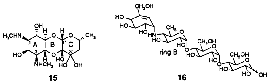
Scheme 8. Spectinomycin (15) [41] and the \alpha -glucosidase inhibitor acarbose (16)
