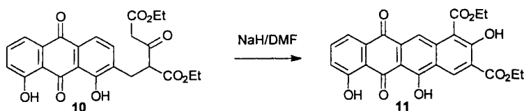
Scheme 4. Formation of naphthacenequinone 11 by intramolecular nucleophilic substitution [22]
