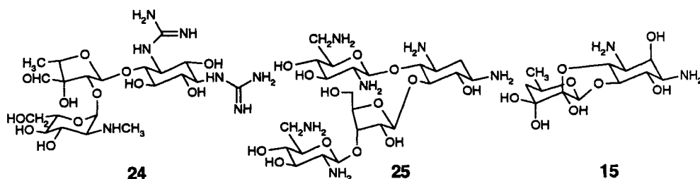
Scheme 11. The aminoglycoside antibiotics, typified by streptomycin (24), neomycin C (25), and spectinomycin (15)
