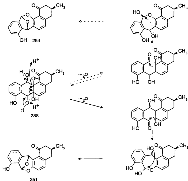
Scheme 68. Alternative rationale for the formation of emycins D (251) and G (254): 1,3-diol cleavage of emycin H analog 288
