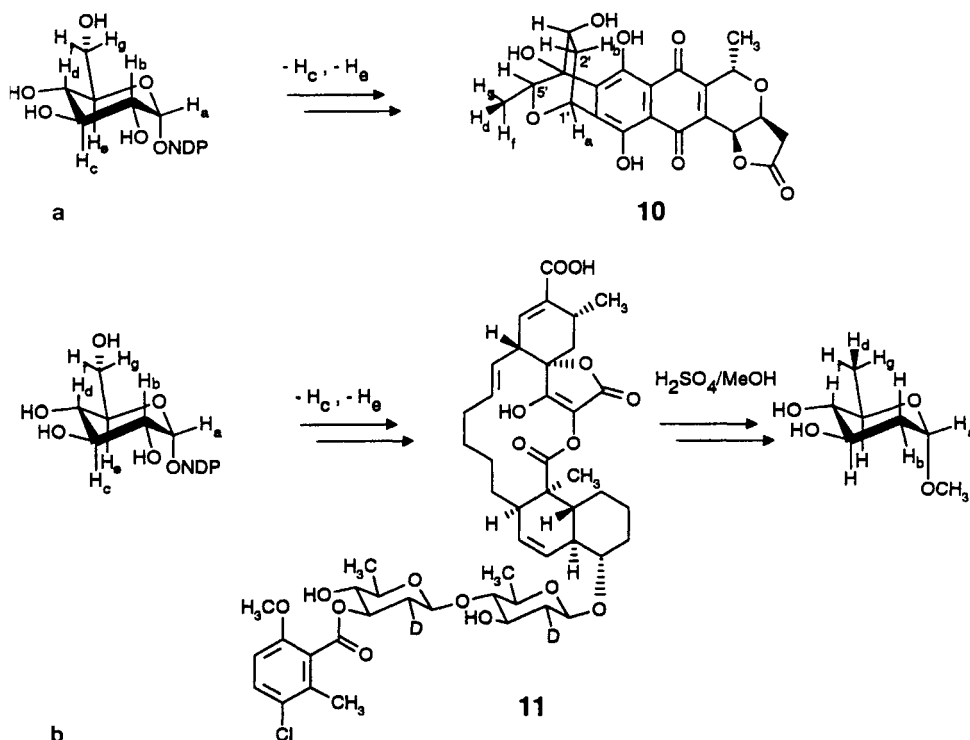
Scheme 5a, b. Deoxygenation steps in the biosynthesis of 2,6-dideoxysugars in granaticin (10) and chlorothricin (11). Note that the 6-deoxygenation occurs in both cases under inversion, while the 2-deoxygenation occurs under retention (in 10) or under inversion (in 11)
