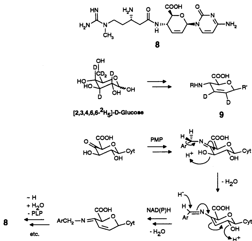
Scheme 4. Deoxygenation of the nucleoside antibiotic blasticidin S ( 8 ). A PMP (pyridoxamine phosphate) may control both the 3- and the 2-deoxygenation (both under retention of protons) from the 4-keto group. PLP, pyridoxal phosphate
