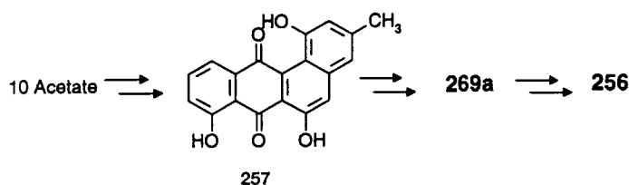
Scheme 56. Dehydroabelomycin (257), a biosynthetic angucyclinone intermediate of the kinamycins
