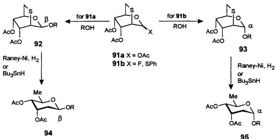
Scheme 36. Glycosidation of 2,6 anhydro-2-thio-sugars
