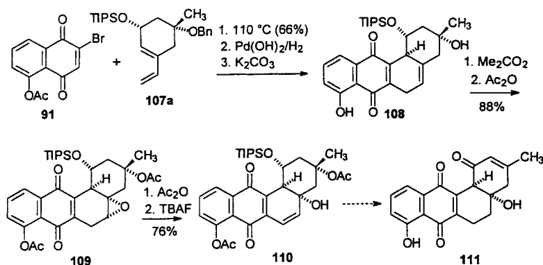
Scheme 30. Enantioselective synthesis of (+)-SF 2315 A ( 111 ) by Kim and Sulikowski [89]
