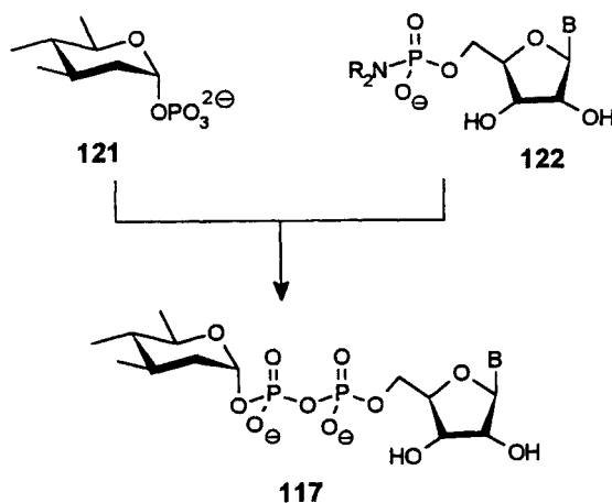
Scheme 41. Chemical strategy for the preparation of nucleoside diphosphate sugars
