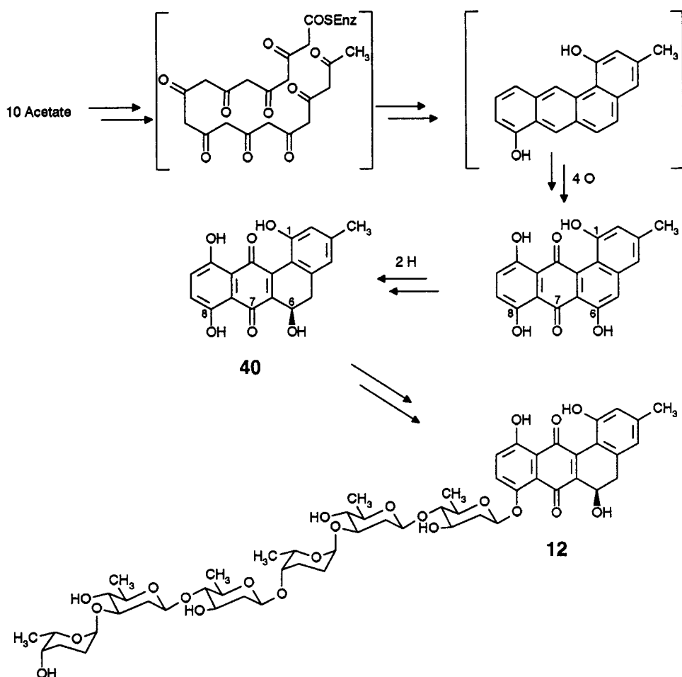
Scheme 15. The biosynthesis of landomycin A (12): landomycinone (40) is the ultimate substrate for the glycosyl transfer cascade to 12
