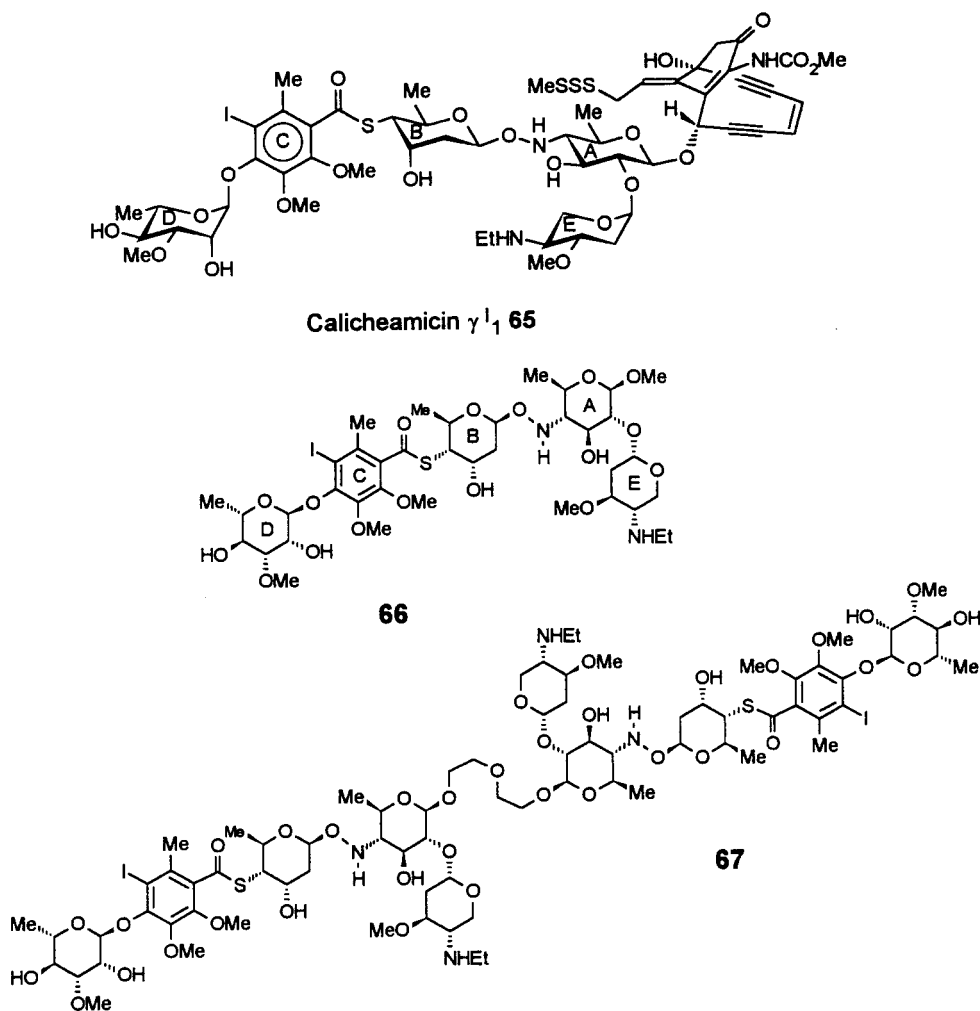
Scheme 29. Calicheamicin \gamma^I_1 (65) and its methyl deoxyoligosaccharide chain (66); the tethered head-to-head dimer (67)
