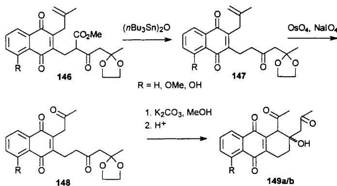
Scheme 38. Construction of ring B in the biomimetic-type angucycline synthesis [86]
