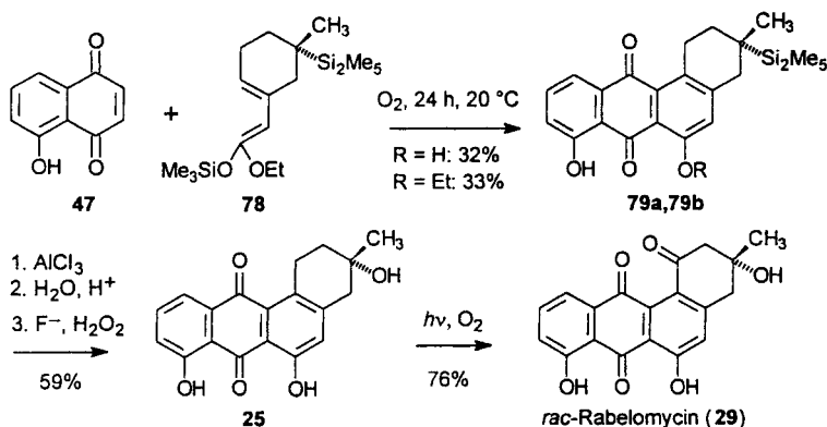
Scheme 23. Synthesis of rac -rabelomycin (29) using the silyldiene 78 in a Diels-Alder reaction [68]
