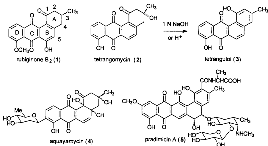
Scheme 2. A few representative examples of angucyclinones (review [3])
