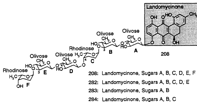
Scheme 64. The landomycins A, B, D and E (208, 282 – 284) differ only with respect to the length of their glycan chain
