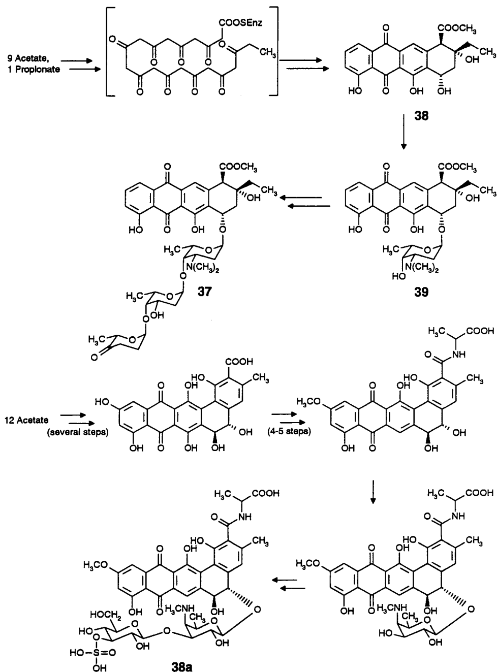
Scheme 14. The biosynthesis of aclacinomycin A (37 proceeds via aklavinone (38) and the monosaccharide aklavin (39), i.e., the glycosylation steps follow the complete construction of the aglycon. A similar process occurs in the biosynthesis of pradimicin S (38a); the glycosyl transfer steps occur after complete assembly of the polyketide aglycon moiety
