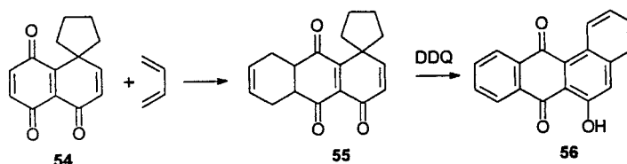
Scheme 16. Rearrangement of a spirodienone 55 to a benzo[ a ]anthraquinone [57]
