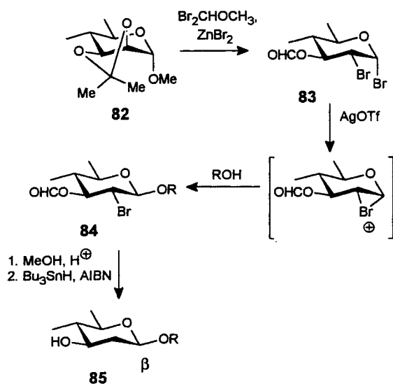
Scheme 33. Br as the stereodirecting group in the preparation of 2-deoxy- \beta -glycosides
