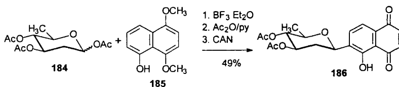
Scheme 47. Synthesis of C -glycosides by direct electrophilic substitution [139]
