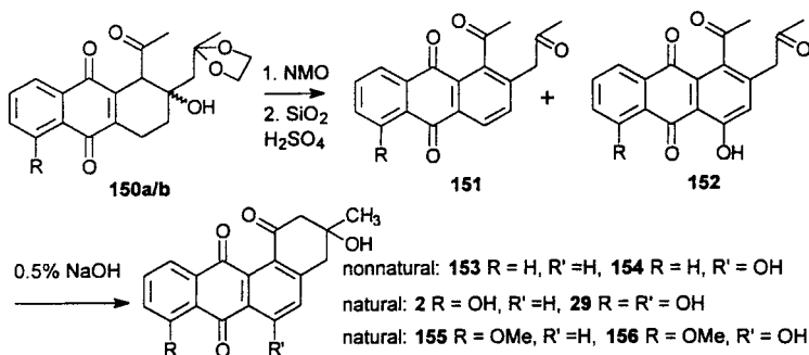
Scheme 39. Construction of ring A and hydroxylation at C-6 in biomimetic-type angucycline synthesis [86]
