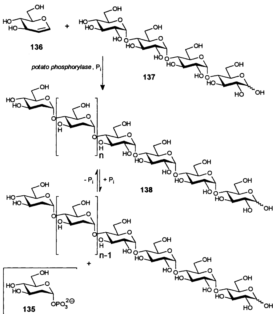
Scheme 45. Potato phosphorylase-catalyzed synthesis of 2-deoxy-D-glucose 1-phosphate 135
