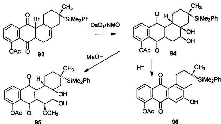
Scheme 27. Some reactions of the cis -diol 94 [82]
