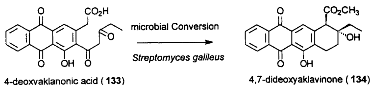
Scheme 35. Microbial conversion of 4-deoxyaklanonic acid (133) to 4,7-dideoxyaklavinone (133) [100]
