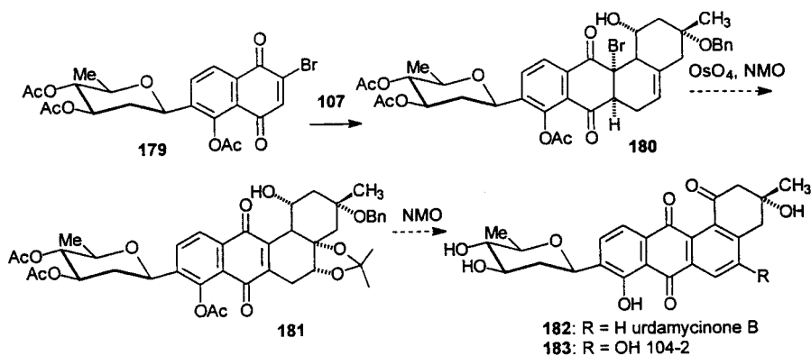
Scheme 46. Total synthesis of urdamycinone B (182) and 104-2 (183) [87]
