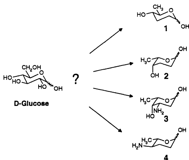
Scheme 1. Deoxygenation mechanisms of highly deoxygenated sugars are still widely unknown
