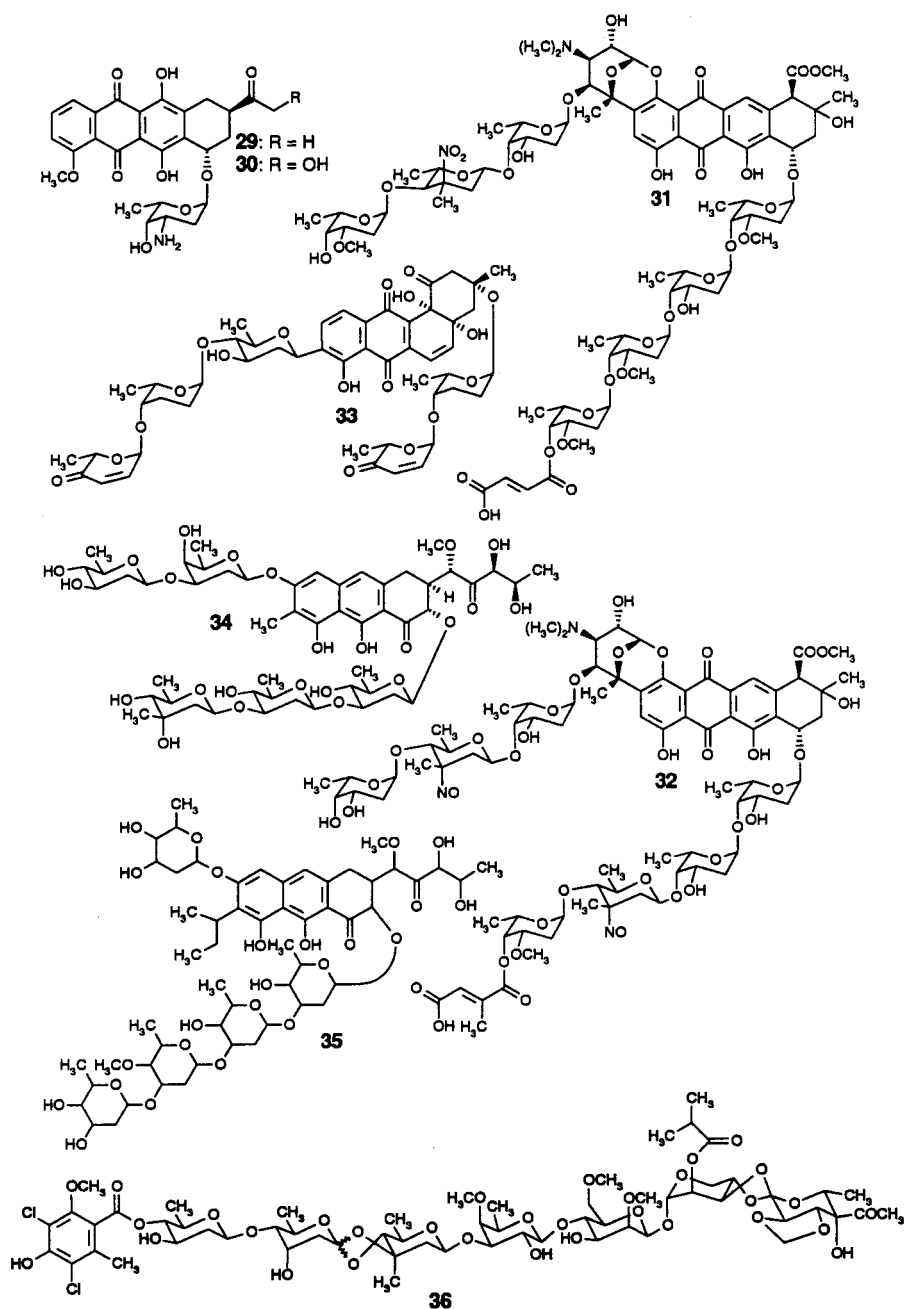
Scheme 13. The antitumor antibiotics daunomycin (29 = daunorubicin) and adriamycin (30 = doxorubicin) are polyketides with an attached deoxysugar moiety. Polyketide oligodeoxysaccharides characterized by one or more deoxysaccharide chains include the anthracyclines arugomycin (31) [73a] and viriplanin (32), the angucyclines landomycin A (see 12 in Scheme 6) and vineomycin A 1 (33 = P1894B [74]), and the aureolic acid antibiotics mithramycin (34) and UCH9 (35). Also, orthosomycin antibiotics, such as avilamycin A (36) can be considered as polyketide oligodeoxysaccharides
