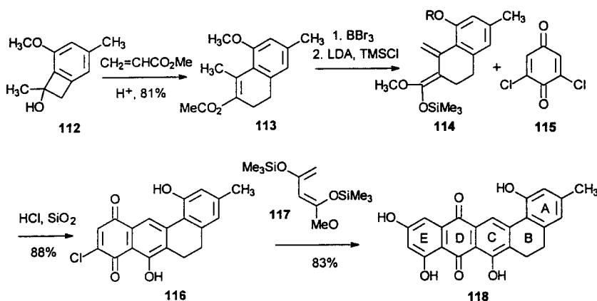
Scheme 31. Synthesis of G-2N ( 118 ) by three successive [2+4] cycloadditions [93].
