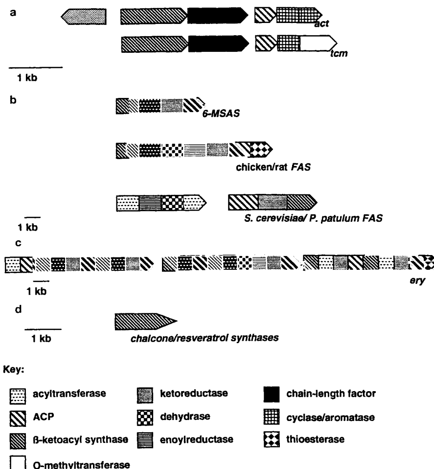
Fig. 2a–d. The major architectural paradigms of fatty acid and polyketide synthases. Relationships between genes encoding: a bacterial aromatic polyketide synthases, b eukaryotic fatty acid synthases and fungal polyketide synthases, c modular polyketide synthases, and d plant polyketide synthases
