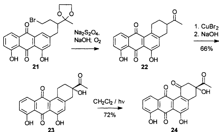
Scheme 7. Electrophilic cyclization of 21 to 22 followed by the introduction of an oxygen atom in the synthesis of a daunomycinone-rabelomycin hybrid 24 [37]
