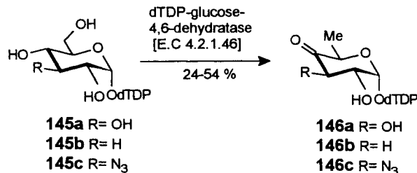
Scheme 48. Substrate specificity of dTDP-glucose-4,6-dehydratase
