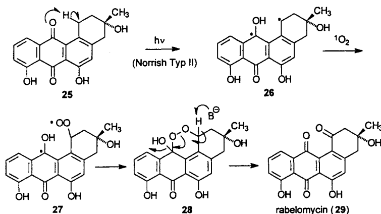
Scheme 8. Photooxygenation of 1-deoxyrabelomycin (25) to afford rabelomycin (29) [39]
