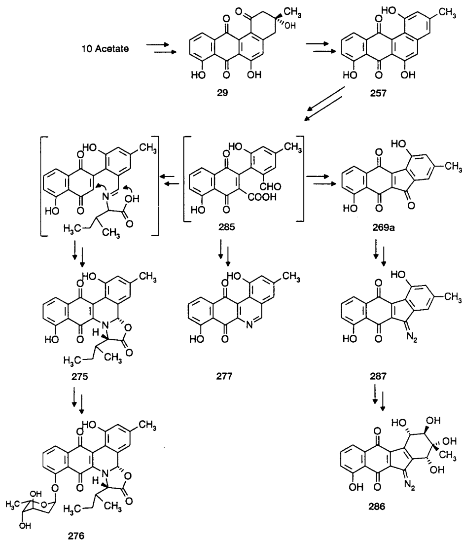
Scheme 66. Hypothetical biosynthetic pathway leading to the phenanthroviridin aglycon (277), the jadomycins (275, 276) and the kinamycin family, e.g., kinamycin F (286). The biosynthetic key step is the oxidative 5,6-bond fission, presumably from dehydrorabelomycin (275) to 285
