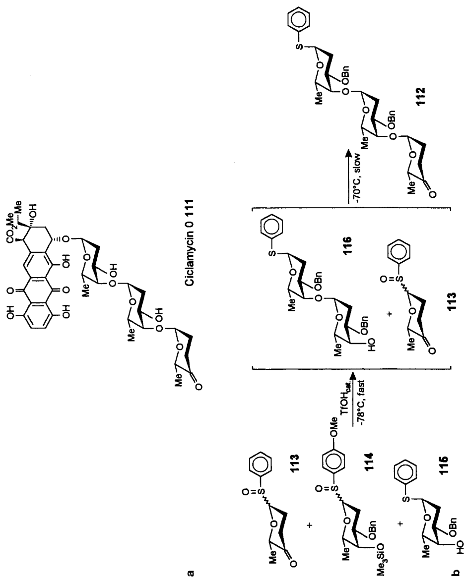
Scheme 39 a, b. a The anthracycline antibiotic cyclamycin 0 (111) and b its „one-pot“ synthesis
