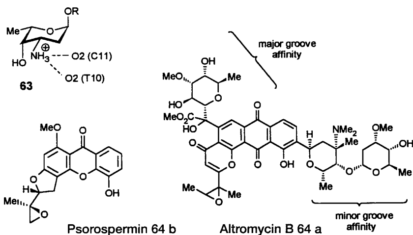
Scheme 28. The aminosugar daunosamine (63) is located in the minor groove of the DNA duplex. The disaccharide form of altromycin B (64a) is located in the minor groove of the DNA palindrome. A parallel orientation of the xanthone ring structure to adjacent base pairs is favored by psorospermin (64b)
