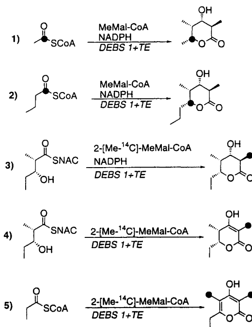
Fig. 9. Polyketide products generated via in vitro biosynthesis by the fusion protein DEBS 1+TE. 1 and 2, 14 C-labeled alternate starter unit substrates were used to synthesize the C 8 - and C 10 -lactones, respectively. 3 and 4, (2 S ,3 R )-2-methyl-3-hydroxypentanoyl- N -acetylcysteamine (NAC) thioester was used as an intermediate to synthesize the C 9 -lactone and the 3-oxo analog, respectively. 5, In the absence of NADPH, a pyran-2-one is generated using propionyl-CoA and 14 C-labeled methylmalonyl CoA
