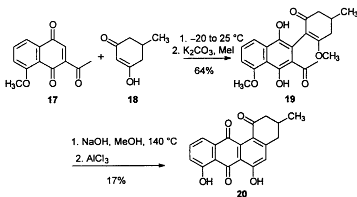
Scheme 6. Synthesis of 3-deoxyrabelomycin (20) using Michael additions [31, 32]
