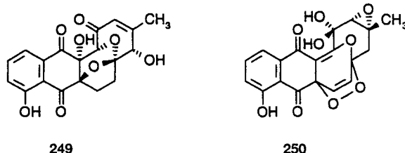
Scheme 54. Two novel, through oxygenase(s) modified, angucyclinones: 249 (WP 3688-4) and 250 (WP 3688-5)
