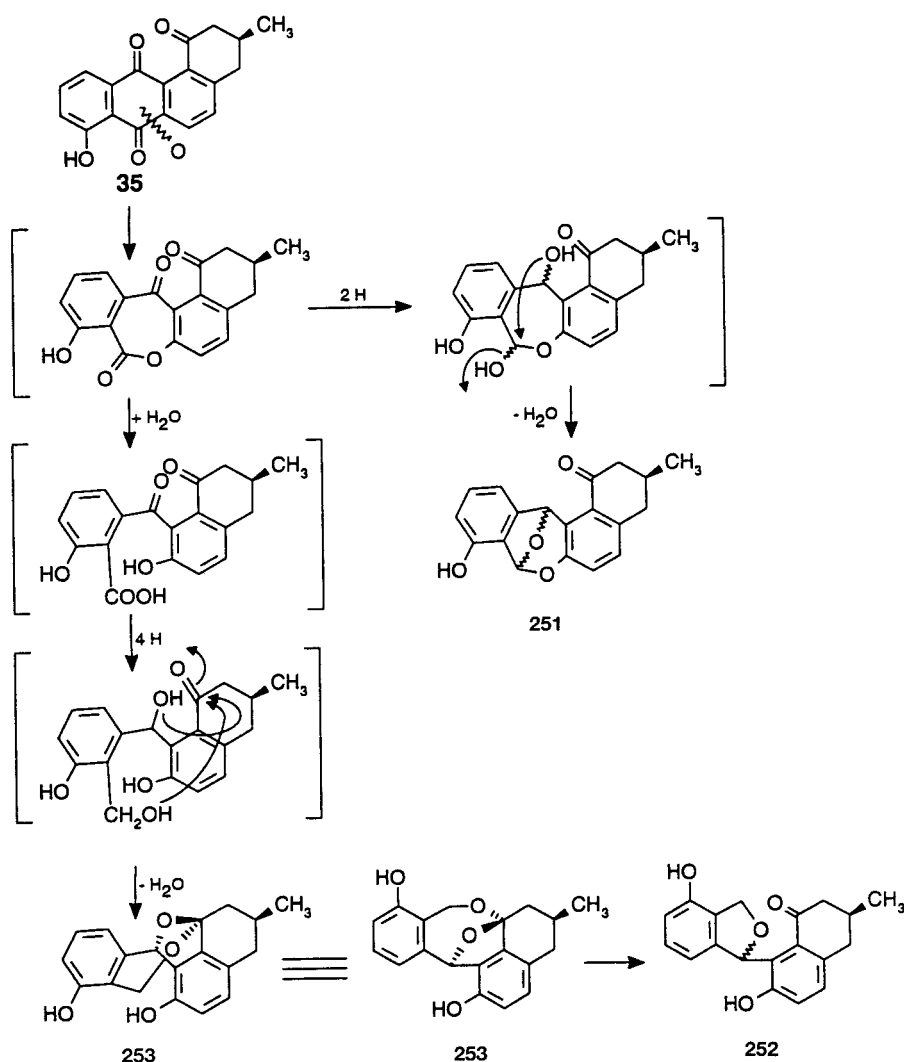
Scheme 67. Rationale for the biosynthetic formation of emycins D (251), E (252) and E (253). The key biosynthetic step is an oxidative cleavage of the 6a,7-bond of an angucyclinone, presumably ochromycinone (35)
