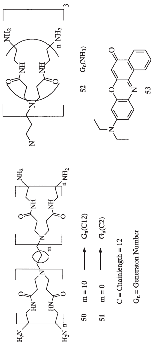
Fig. 23. Dendritic bolaamphiphiles reported by Tomalia et al.
