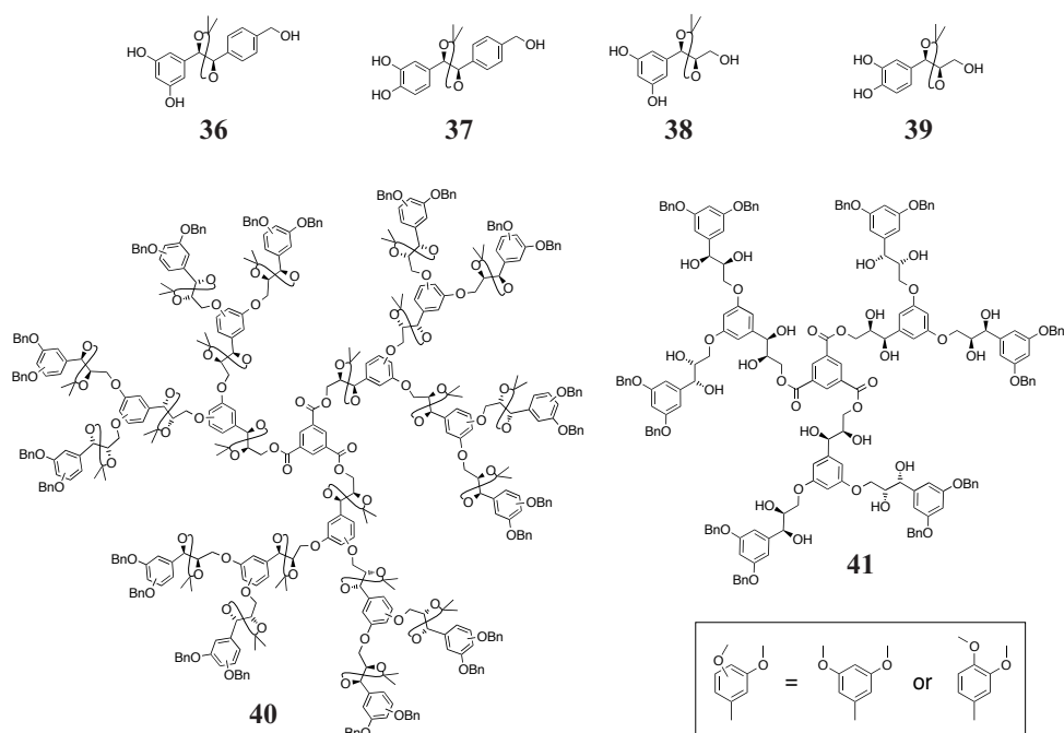
Fig. 17. Chiral acetonide building blocks 36 – 39 , protected 3rd-generation dendrimer 40 and deprotected 2nd-generation dendrimer 41 , derived from enantioselectively dihydroxylated styrenes and cinnamic alcohols [74–76]
