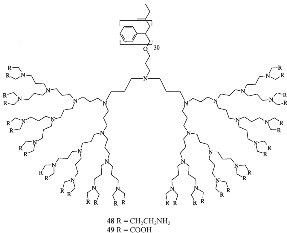
Fig. 22. Amphiphilic copolymers reported by Meijer et al.
