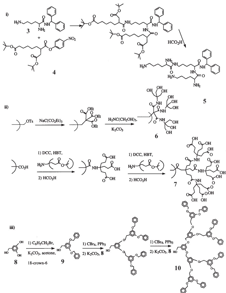
Fig. 3i–iii. Dendrimer synthesis using branched building blocks: i Denkewalter's polylysine dendrimers; ii Newkome's polyamide dendrimers; iii Fréchet's aryl ether dendrimers
