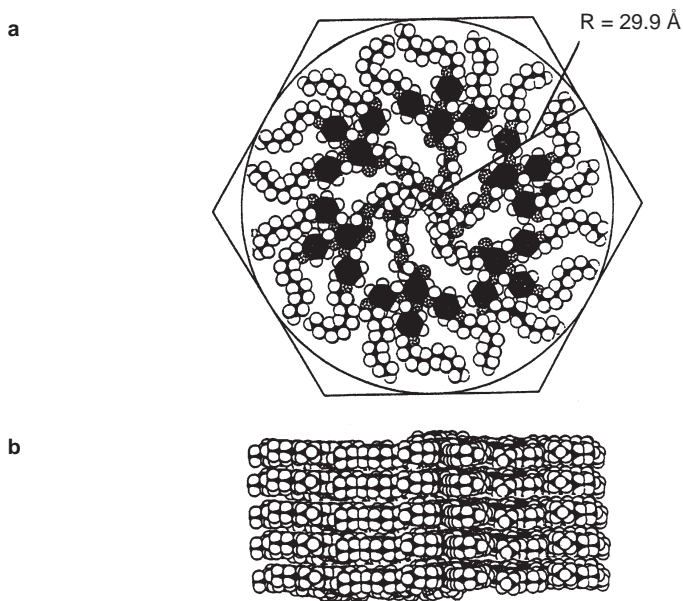
Fig. 2. Schematic representation of the supramolecular cylinders of the dendrimer derived from macromonomer 9 ( R = OC_{12}H_{25} , n = 3 ) in the Qh mesophase: a top view of a cylinder containing six repeat units in a stratum with the alkyl tails melted to match the average column radius determined by X-ray scattering experiments; b side view of a cylinder containing 30 repeat units of the polymer assembled with melted alkyl tails. Reproduced with permission from references 5a
