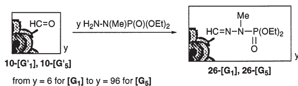
Fig. 6. Dendrimers of generation 5 with 96 various terminal phosphorus groups
