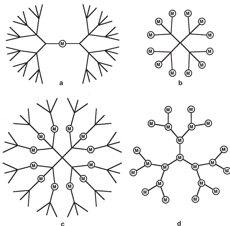
Fig. 1 a–d. Different kinds of metal-containing dendrimers: a a metal complex as a core; b metal complexes only as peripheral units; c metal complexes only in the branches; d metals as branching centers
