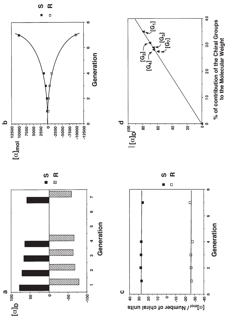
Fig. 4. a Specific rotation [\alpha]_D vs generation for dendrimers 19 S-[G n ] and 19 R-[G n ]. b Molar rotation [\alpha]_{mol} vs generation for dendrimers 19 S-[G n ] and 19 R-[G n ]. c Molar rotation [\alpha]_{mol} divided by the number of chiral groups vs generation for dendrimers 19 S-[G n ] and 19 R-[G n ]. d Absolute value of the specific rotation |[\alpha]_D| vs the percentage of contribution of the chiral groups to the molecular weight for the dendrimers 19 S-[G n ] and 19 R-[G n ]
