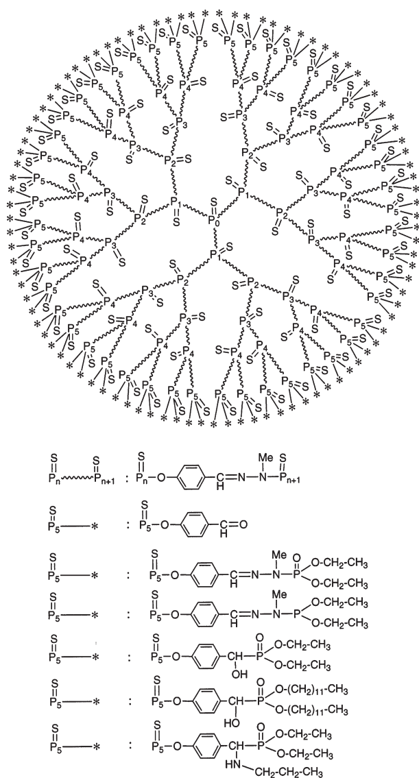
Fig. 6. Dendrimers of generation 5 with 96 various terminal phosphorus groups
