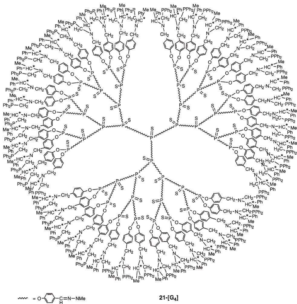
Fig. 3. Representation of the dendrimer 21-[G 4 ] (generation 4, 48 terminal (S) or (R) amino-phosphines)
