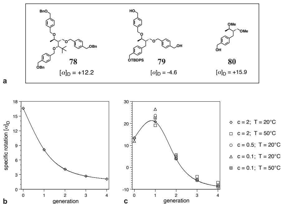
Fig. 26. a Specific optical rotations for the model building blocks for “core” 78, “interior building block” 79 and “peripheral unit” 80 of dendrimers of type 77; b calculated average optical rotations for the doubly branching dendrimers of 0th to 4th generation; c measured optical rotations in \text{CHCl}_3 at different temperatures and concentrations [94]
