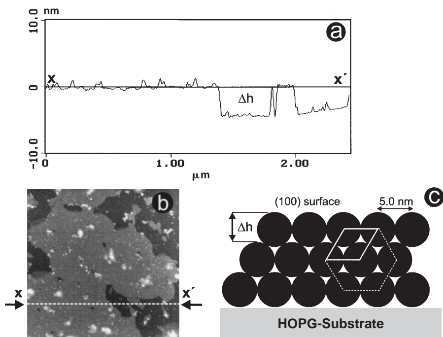
Fig. 7. a Cross sectional profile of an ultrathin film of dendrimer 23 on HOPG along x-x' as indicated in (b) . The height difference between adjacent terraces has the dimension of a monolayer [ \Delta h = 4.3 (\pm 0.2) nm]. Large scale ( 2.4 \times 2.4 \mu\text{m}^2 ) SFM image of monomolecular terraces. c Schematic model of closely packed molecular cylinders in thin films of 23 on HOPG
