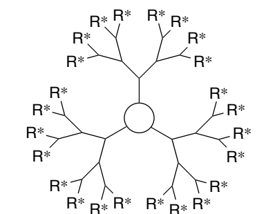
dendrimer with chiral peripheral units (achiral or chiral core and building blocks)
