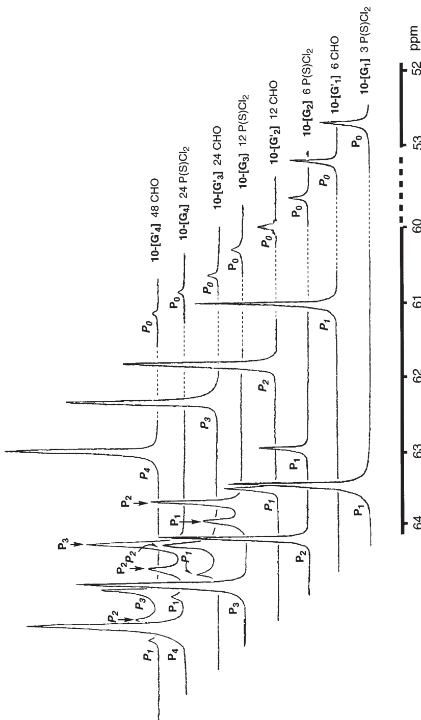
Fig. 1. ^{31}\text{P} { ^1\text{H} }-NMR spectra (THF) of dendrimers of generation 1, 2, 3 and 4. 10\text{-}[\text{G}'] , 10\text{-}[\text{G}_1] , 10\text{-}[\text{G}_2] , 10\text{-}[\text{G}_3] , 10\text{-}[\text{G}_4] , 10\text{-}[\text{G}'_1] , \text{P}_0 phosphorus of the core, \text{P}_1 phosphorus of generation 1, \text{P}_2 phosphorus of generation 2, \text{P}_3 phosphorus of generation 3, \text{P}_4 phosphorus of generation 4.
