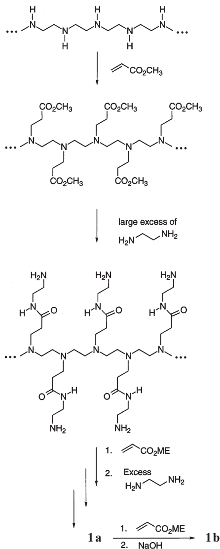
Scheme 2. Tomalia's divergent synthesis of dendronized polyethylene imine (PEI)
