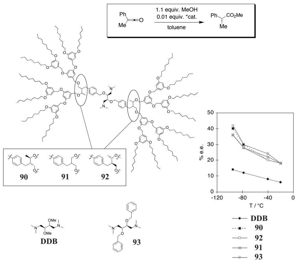
Fig. 32. Dendritically enlarged diamines 90 – 92 and benzylated ligand 93 (DDB analogs) in the enantioselective addition of methanol to ketene using 0.01 equiv. catalyst [114]
