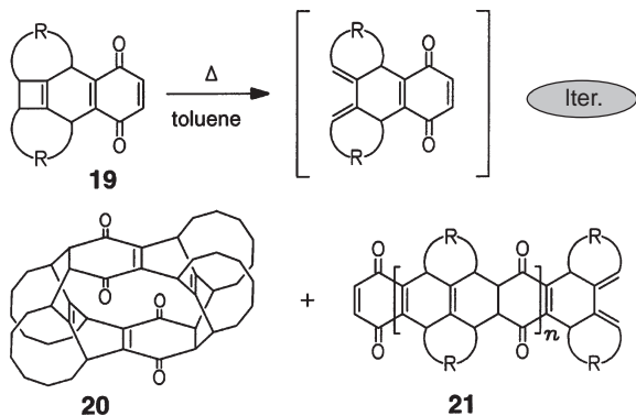
Fig. 11. Synthesis of the beltene 20
