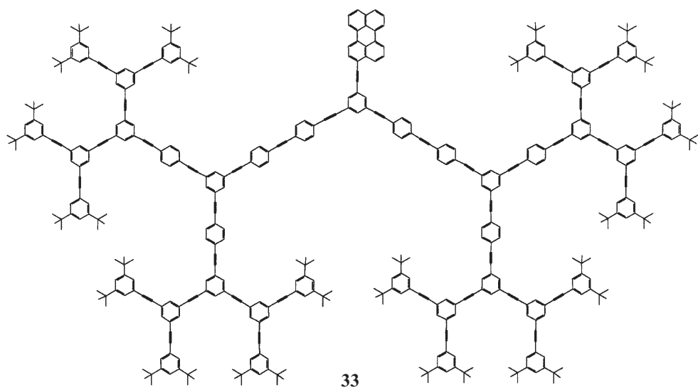
Fig. 16. Moore's dendritic molecular antenna
