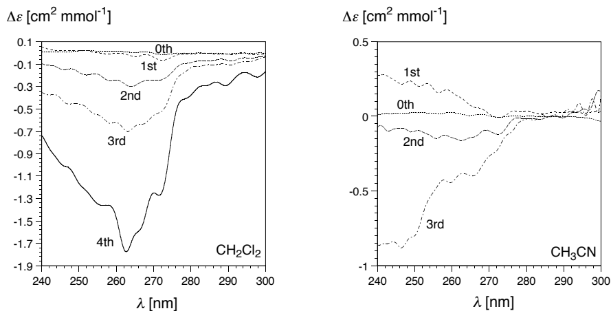
Fig. 27. CD spectra of “fully chiral” dendrimers (0th up to 4th generation of type 77) in \text{CH}_2\text{Cl}_2 and in \text{CH}_3\text{CN} [94]
