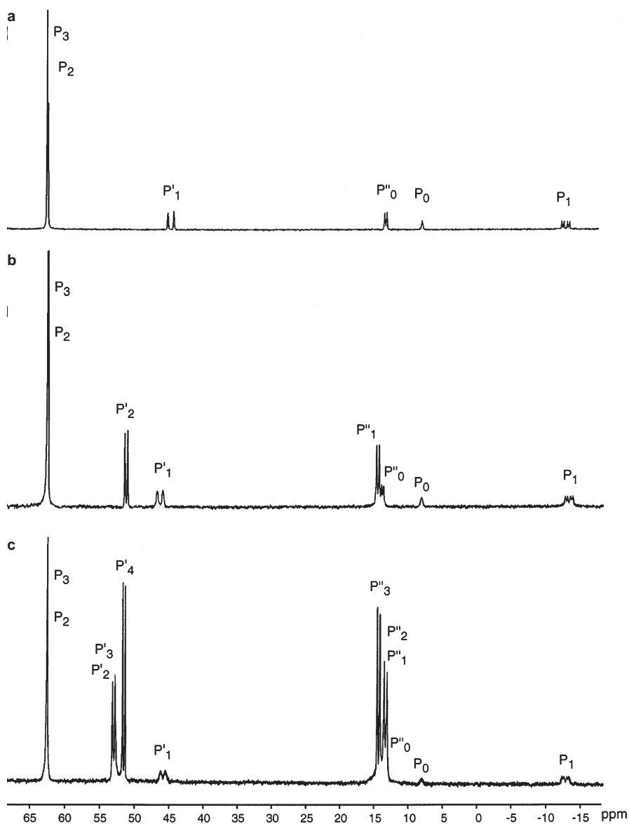
Fig. 9a–c. ^{31}\text{P} -NMR spectra of the polydendritic macromolecules: a compound 89 – central dendrimer \text{P}_0, \text{P}'_0, \text{P}_1, \text{P}_2, \text{P}_3 – internal dendron \text{P}'_1 ; b compound 90 – central dendrimer \text{P}_0, \text{P}'_0, \text{P}_1, \text{P}_2, \text{P}_3 – internal dendrimers \text{P}'_1, \text{P}'_1, \text{P}'_2 ; c compound 91 – central dendrimer \text{P}_0, \text{P}'_0, \text{P}_1, \text{P}_2, \text{P}_3 – internal dendrimers \text{P}'_1, \text{P}'_1, \text{P}'_2, \text{P}'_2, \text{P}'_3, \text{P}'_3, \text{P}'_4
