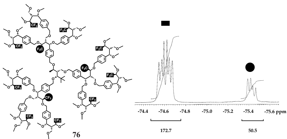
Fig. 24. Fluorine-containing 2nd-generation dendrimer 76 and 19 F-NMR spectrum showing the different chemical environment in the two dendrimer-layers [91]
