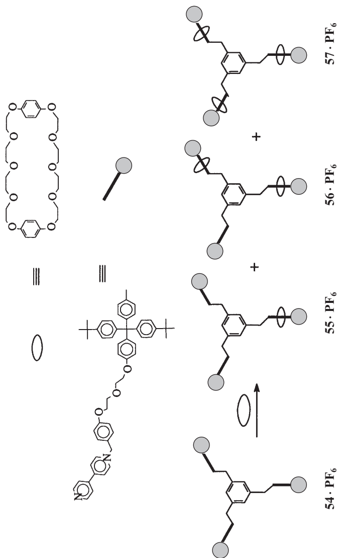
Fig. 24. Dendritic rotaxanes reported by Stoddart et al.
