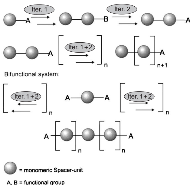
Fig. 1. Principle of iterative synthesis. In the first reaction step (Iter. 1) a monomeric unit, which may possess another functional group, is attached to the starting material. In the second step of the reaction sequence (Iter. 2) the functional group A is reobtained, so that Iter. 1 and 2 can be repeated
