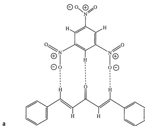
Fig. 13a–c. The complex of a dibenzylidene ketone with 1,3,5-trinitrobenzene, showing C-H \cdots O hydrogen bonds [38]: a a chemical formula
