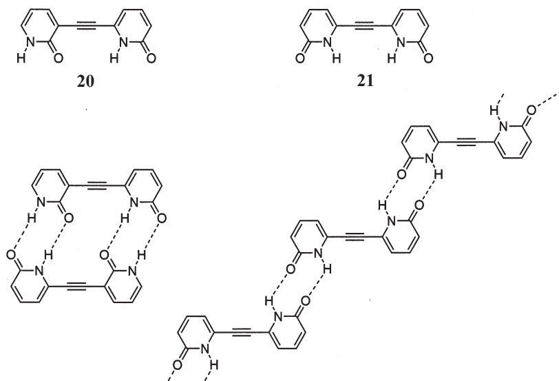
Fig. 17. Dimers and ribbons formed by asymmetric 20 and symmetric dipyrindiones 21
