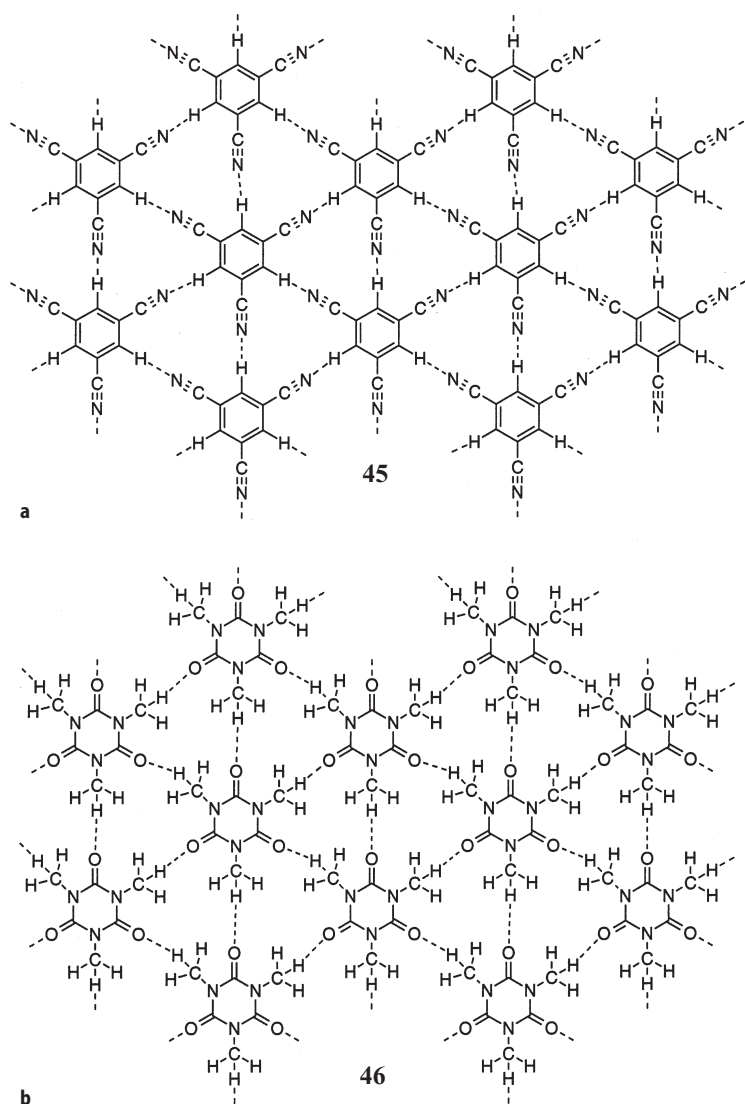
Fig. 30. Formation of sheets stabilized by \text{C}-\text{H}\cdots\text{N} (45) and \text{C}-\text{H}\cdots\text{O} (46) hydrogen bonds
