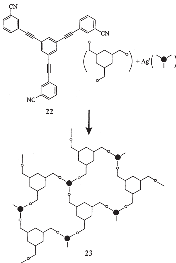
Fig. 7. 12-Annulene-like motif formed by 22 · AgOTf. The counteranion is not shown for clarity. The sheets ( 23 ) are layered to form intersheet channels
