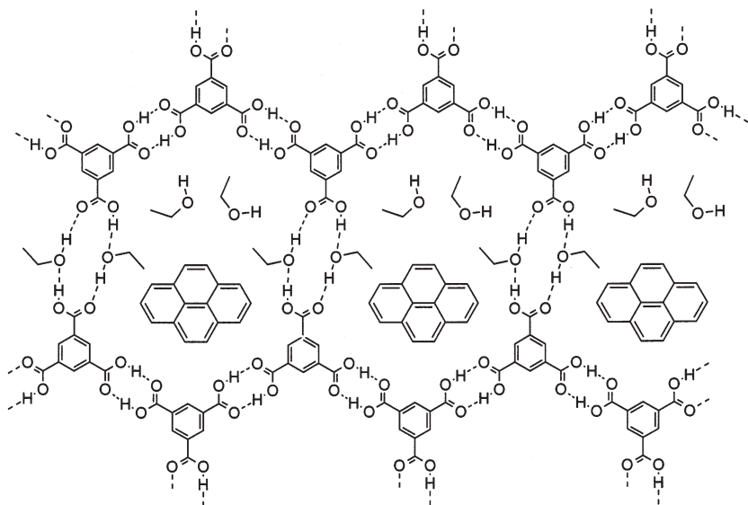
Fig. 13. Sheets formed in the crystal structure of [2 2 · pyrene · 2EtOH]
