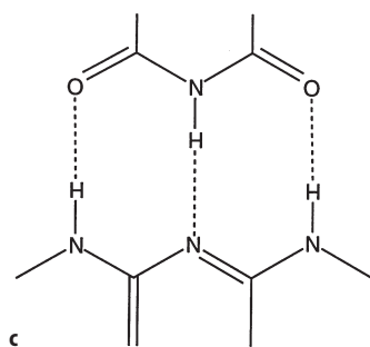
Fig. 13 b, c. b view in crystal structure; c comparison of the interactions in (b) and those in which conventional O-H \cdots N and N-H \cdots N hydrogen bonds are formed
