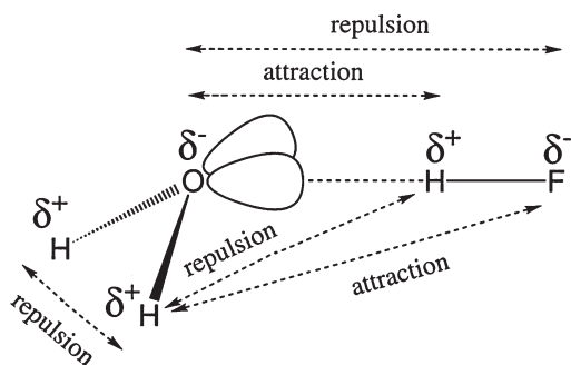
Fig. 10. Repulsions and attractions in the \text{H}_2\text{O} \cdots \text{HF} complex
