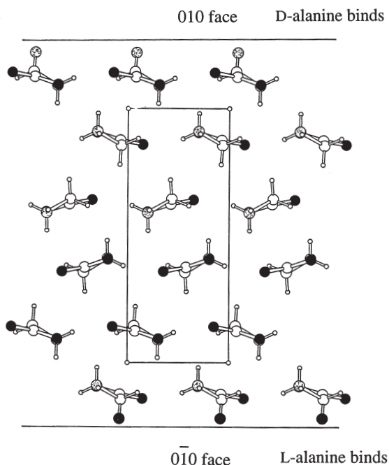
Fig. 34. Glycine crystals binding optically active amino acids [86, 116]. Shown is the binding of D-alanine to the 010 face and L-alanine to the \bar{0}\bar{1}0 face. The methyl groups of alanine are stippled circles for the former, and filled circles for the latter
