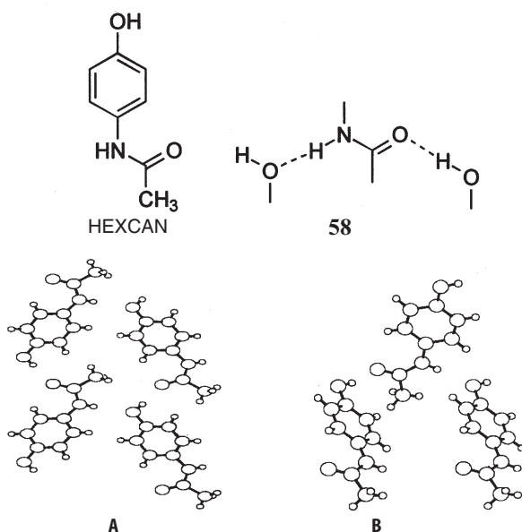
Fig. 7. Polymorphs A and B of 4-hydroxyacetanilide (HEXCAN)
