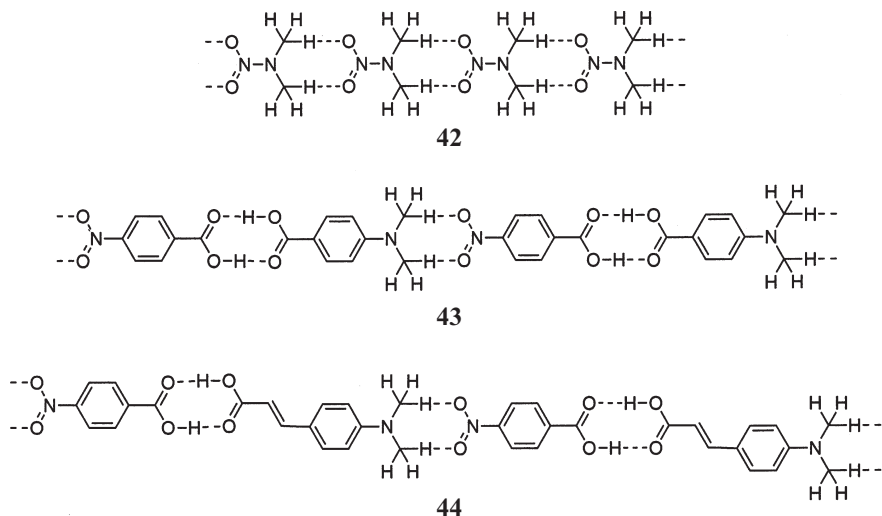
Fig. 29. \text{C-H}\cdots\text{O} hydrogen bonding is evident in the tapes formed by 42, 43 and 44
