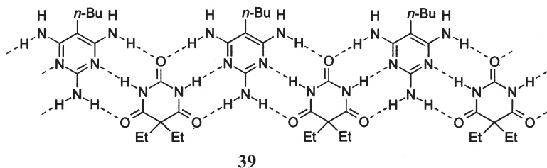
Scheme 9. 1:1 Complex of the barbituric acid-triaminopyrimidine type. Note that like residues, Et and n -Bu are located on either side of the hydrogen bonded tape
