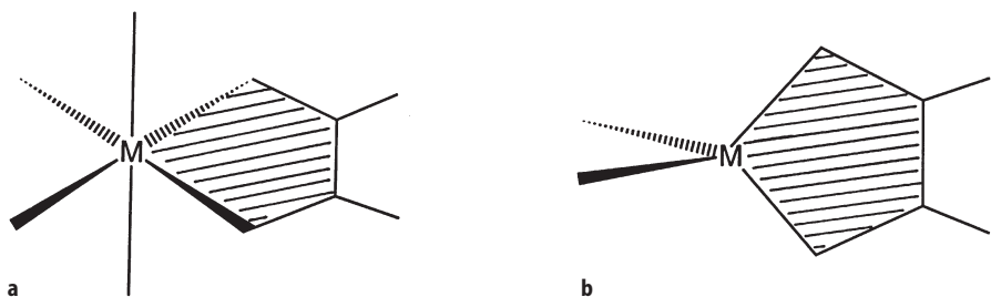
Fig. 25 a, b. If two locations on a rigid coordination polyhedron are fixed, the directions of binding of the other ligands is also fixed: a 2 \text{Mg}^{2+} \cdots \text{O} interactions fixed in an octahedral coordination scheme; b 2 \text{Zn}^{2+} \cdots \text{S} interactions fixed in a tetrahedral coordination scheme
