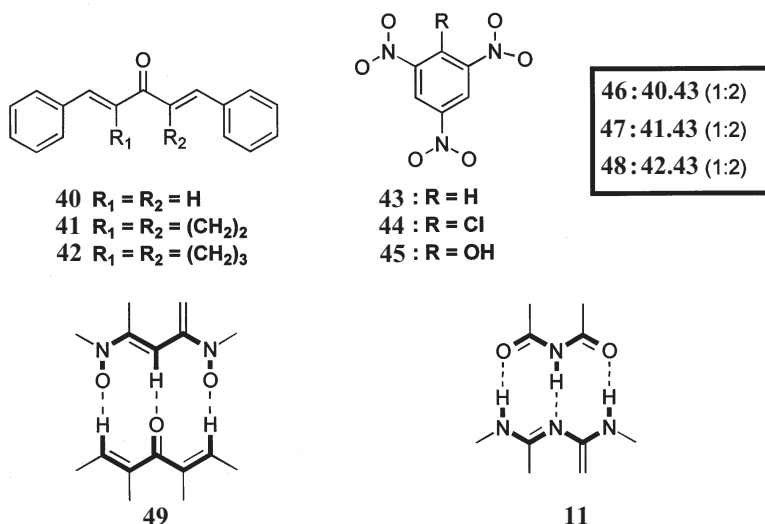
Scheme 10. DAD:ADA complexes 46 – 48 of dibenzylidene ketones and trinitrobenzene (see [49])
