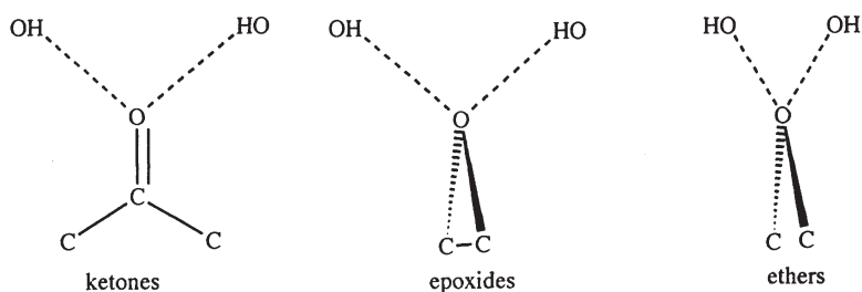
Fig. 11. Scatterplot around C=O [9]. Hydrogen bonds are indicated by broken lines. Note that the distribution of hydrogen bond donors is similar for ketones (in the plane of the carbonyl group), and epoxides (perpendicular to the epoxide ring plane). These are the directions of the lone pair of electrons in both cases. The directions of hydrogen bonding around ethers are closer together, as diagrammed
