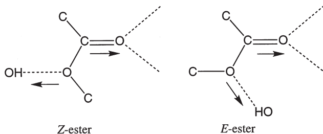
Fig. 12. Interactions around esters [39]. Hydrogen-bond directions are indicated by broken lines. The directions of OH and C=O dipoles are indicated by arrows. Note the difference between ( Z )- and ( E )-esters
