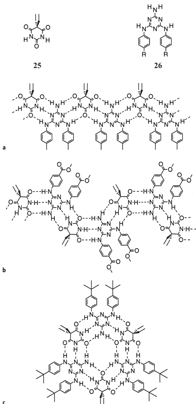
Fig. 20. Formed by 25 and 26: a tapes; b ribbons; c cyclic aggregates
