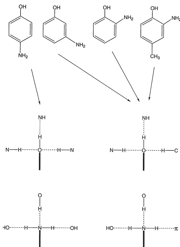
Fig. 16. The different styles of packing in the crystalline state of some aminophenols [44–46]. It is shown that p -aminophenol utilizes O-H \cdots N and N-H \cdots O hydrogen bonds in crystal packing, while the o - and m -compounds and 2-amino-4-methylphenol also utilize C-H \cdots O and N-H \cdots \pi interactions
