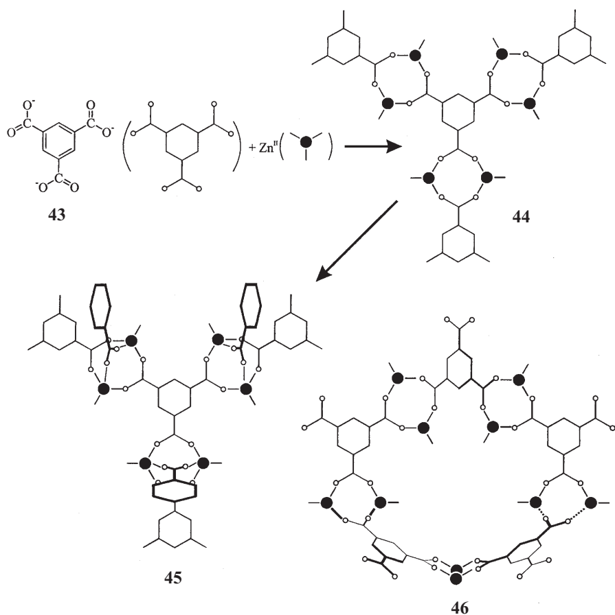
Fig. 12. 3D net formed by \mathbf{43} \cdot 2\text{Zn} \cdot (\text{NO}_3)_2 . The counteranion is not shown for clarity
