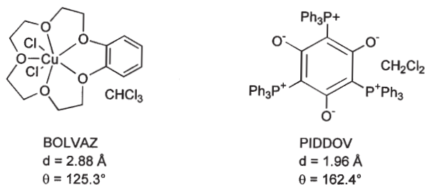
Scheme 7. Outlier refcodes in the CSD study of C-H...O hydrogen bonding in \text{CHCl}_3 and \text{CH}_2\text{Cl}_2 solvates
