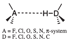
Fig. 5. Hydrogen bonds formed between an acidic hydrogen atom (D-H) and an acceptor (A)
