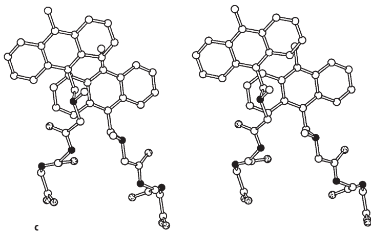
Fig. 3 c. Stereoview of packing in the alkylated sarcosylglycylglycine. In this and all subsequent figures oxygen atoms are stippled and nitrogen atoms filled circles
