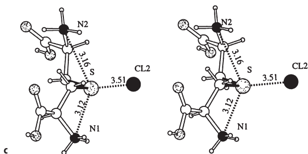
Fig. 5 c. Stereoview of the surroundings of C-S-C (filled bonds) in mesolanthionine dihydrochloride [111]. Note Cl - in C-S-C plane, N + perpendicular to it
