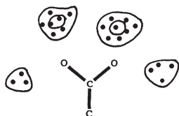
Fig. 1 a–d. Construction of a scatterplot of intermolecular interactions around a functional group [10]
