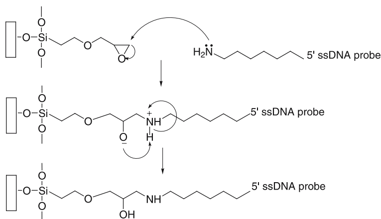
Fig. 7 Reaction of glycidoxypolypropyltrimethoxysilane with a 5'-amino-terminated single-strand DNA probe
