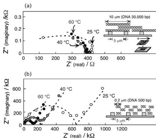
Fig. 13 Cole-Cole plots (10 Hz to 10 MHz frequencies) of alternating currents of the DNA aligned film placed perpendicular to the comb-type electrodes (5 μm distance). a The film prepared from the long DNA molecules (10 μm, 30 000 bps) and b the film prepared from the short DNA molecules (0.2 μm, 500 bps)
