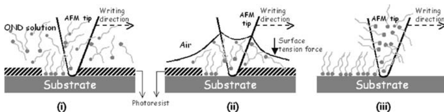
Fig. 22 Patterning of QND or DNA solutions by means of an AFM tip. (i) Nanografting, (ii) Meniscus-Force Nanografting, (iii) Dip-pen lithography
