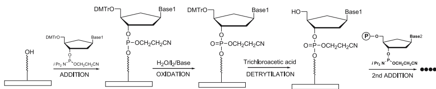
Fig. 19 Basic steps in a cycle of nucleotide addition by the phosphoramidite method in-situ synthesis using ink-jetting. DMTr = dimethoxytrityl group
