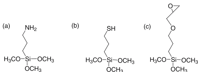
Fig. 6 Common silanizing agents to promote covalent DNA immobilization: a 3-aminopropyltrimethoxysilane (APS) b 3-mercaptopropyltrimethoxysilane (MPS) c 3-glycidopropyltrimethoxysilane (GPS)
