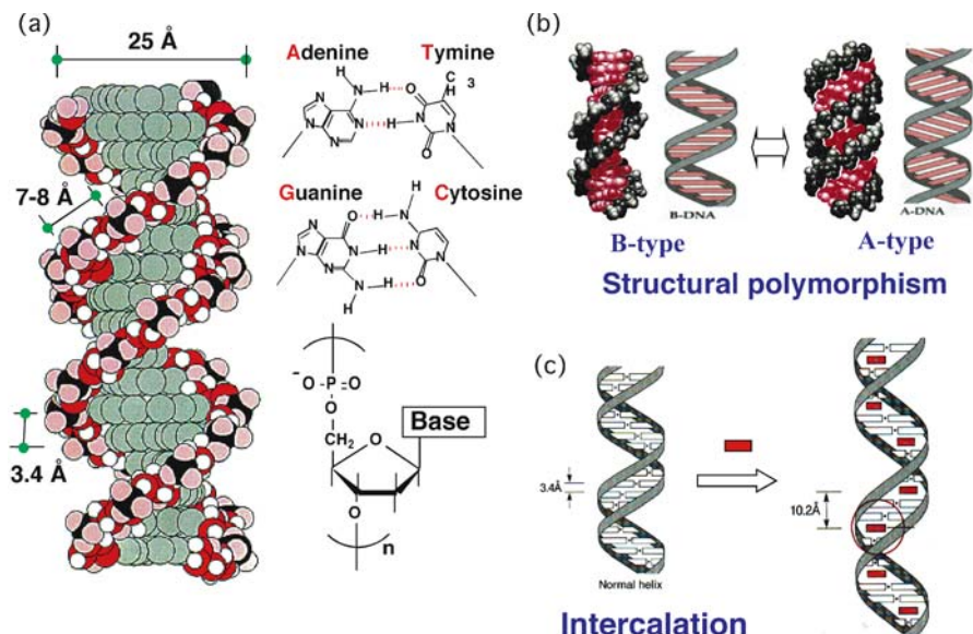
Fig. 1 a DNA structures, b polymorphism of DNA, and c intercalation of dye molecules into DNA
