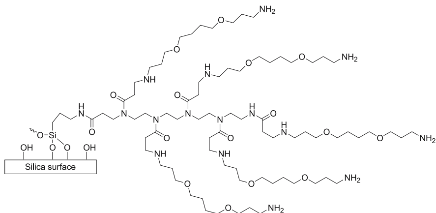
Fig. 11 In-situ synthesized dendrimeric structure prepared from an aminosilanized surface and multifunctional linkers [38]
