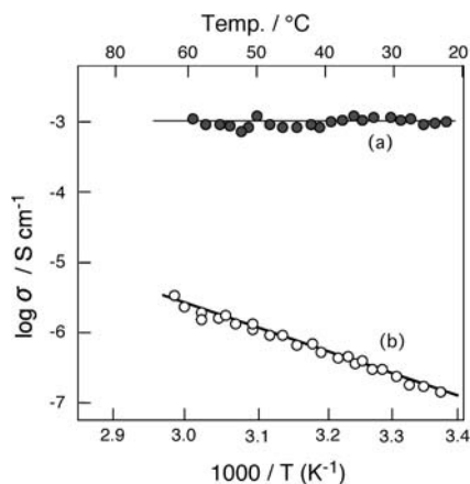
Fig. 14 Temperature dependence of alternating conductivities of a the film prepared from the long DNA molecules (10 μm, 30 000 bps) and b the film prepared from the short DNA molecules (0.2 μm, 500 bps)
