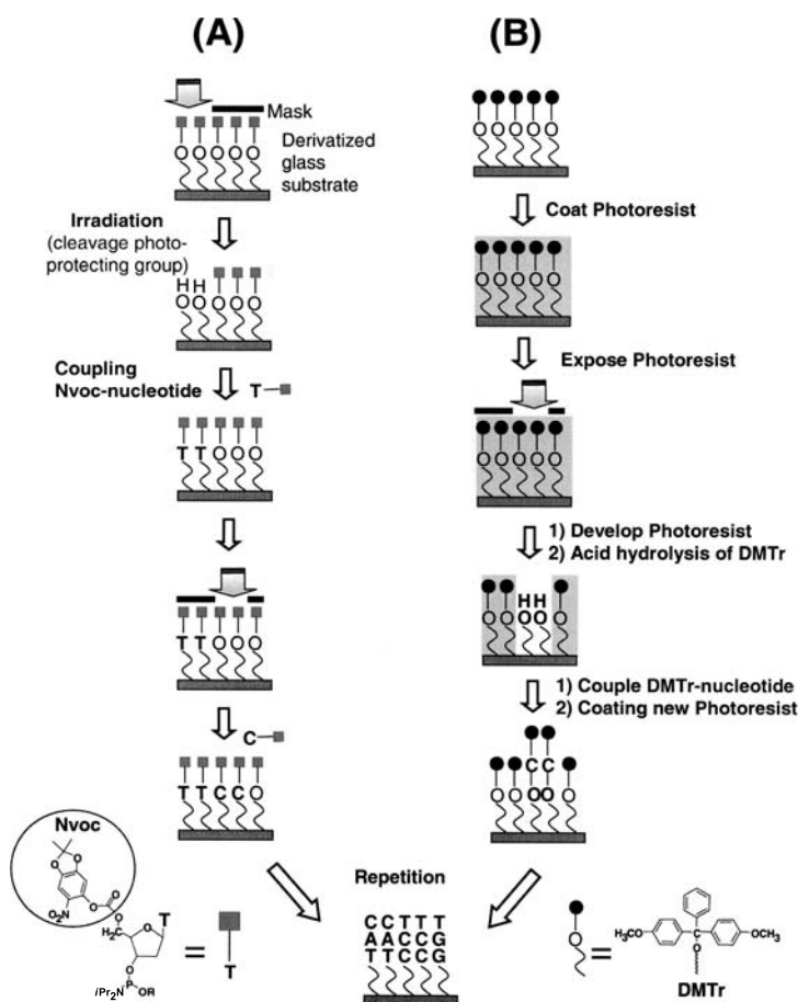
Fig. 18 Light directed OND synthesis onto substrates. a The patterning is mediated by photolabile groups (eg. Nitroveratryl, Nvoc) which protect the surface active groups. Light is directed through a mask to deprotect and activate selected sites, and protected nucleotides couple to the activated sites. The process is repeated, activating different sets of sites and coupling different bases allowing arbitrary DNA probes to be constructed at each site. In b the patterning is mediated by irradiation of a photoresist layer spin-coated onto the functionalized substrate. Irradiation through a mask removes the photoresist layer from selected places and allows coupling of nucleotides on those sites with surface functional groups
