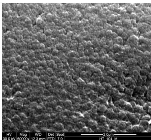
Fig. 8 ESEM image of the surface of a freshly prepared fractal composite sphere showing a cauliflower-like arrangement representing bundles of subunits of the last fractal generation (Fig. 7). By comparison with the surface image given in Fig. 6 it becomes evident that drying and ageing slightly affects the images of the composite samples
