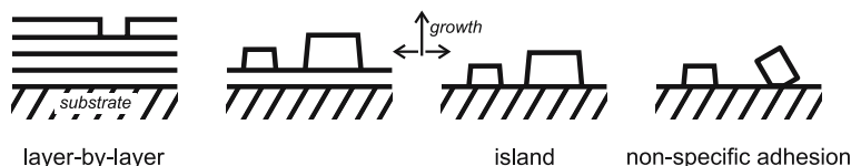
Fig. 4 Schematic representation of different epitaxial growth modes. The 3-D alignment of the over-growing phase relative to the substrate is primarily dependent on the matching of the two different lattices. The structural similarity is most pronounced in the layer-by-layer growth mode. (Adapted from [13])
