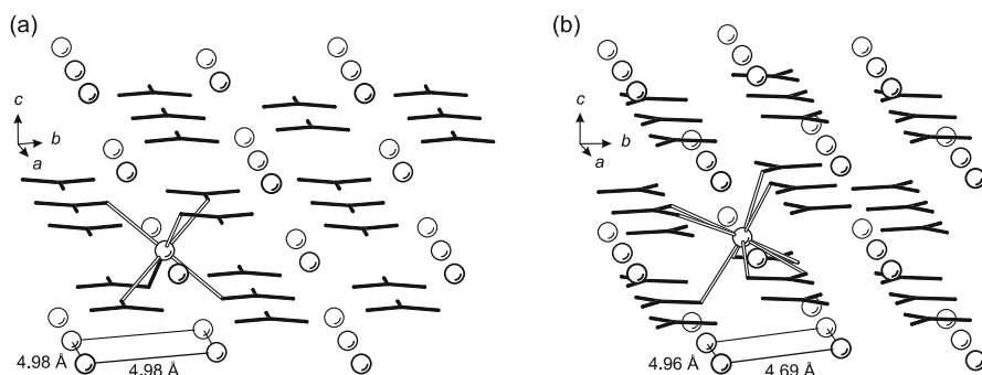
Fig. 2 Ion packing arrangement in the crystal structures of a calcite and b aragonite. The coordinative bonds between \text{CO}_3^{2-} anions (black sticks) and one of the \text{Ca}^{2+} ions (open circles) are emphasized with open lines. The minimum distances of \text{Ca}^{2+} ions in the ab planes for both crystal lattices are indicated at the bottom. (Reprinted from [18] with permission)
