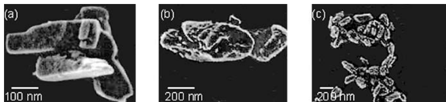
Fig. 3 FESEM of hemozoin purified from a Plasmodium falciparum , b Schistosoma mansoni , c Hemaoproteus columbae
