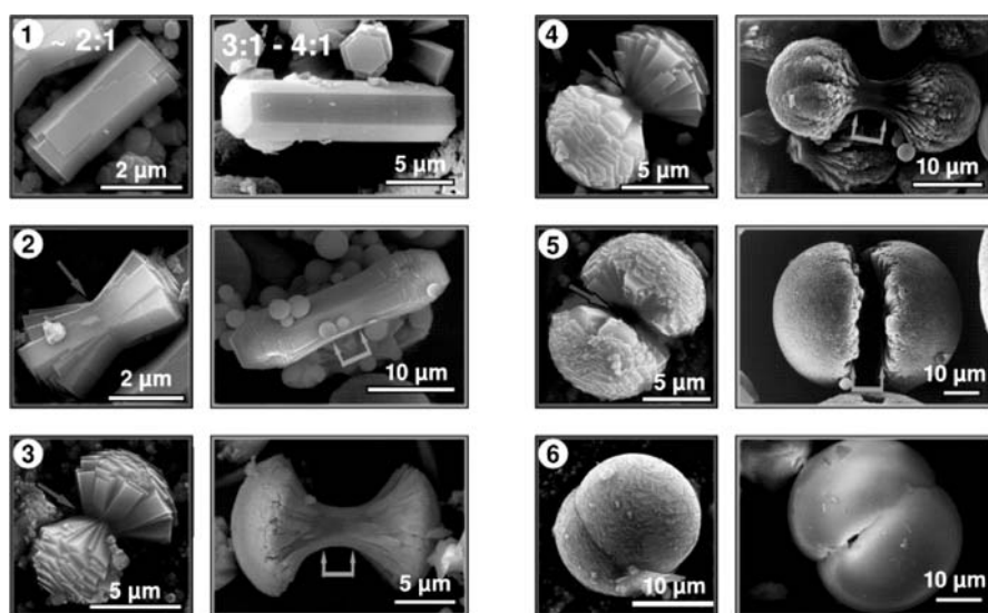
Fig. 10 SEM images illustrating subsequent states (1–6) of the morphogeneses of fluorapatite-gelatine nanocomposites for fan-like (vertical rows on the left-hand side) and fractal (vertical rows on the right-hand side) growth mechanisms [24]. The arrows indicate the growth plane and the “free bridge” respectively, see text for details
