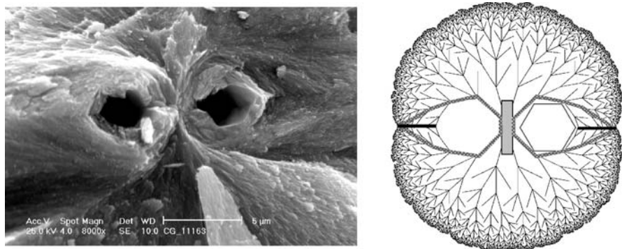
Fig. 13 Torus-shaped cavity around the seed in a closed sphere of the fractal morphogenesis. The SEM image ( left ) clearly shows the hexagonal cross section of the cavity which impressively supports the (modified: see text) 2D simulation model ( right )
