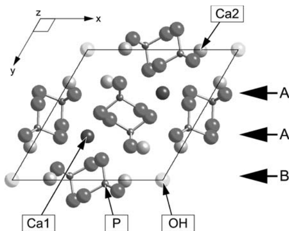
Fig. 15 HAp crystal structure observed along \langle 001 \rangle . The planes “A” and “B” are the possible positions where a HAp structure can be terminated
