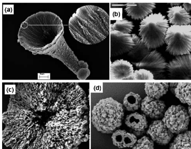
Fig. 21 Hollow and porous morphologies of \text{CaCO}_3 consisting of small units: a micro-trumpet [99], b shuttlecock [100], c porous microparticles synthesized with polyelectrolyte layer-by-layer assembly [101], d hollow particles consisted of the calcite rhombohedral subunits grown with DHBCs [58]. Reproduced from [58, 99–101] with permission of the American Chemical Society and the Royal Society of Chemistry
