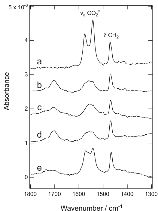
Fig. 10 IR transmission spectra of arachidic acid LB films soaked in various solutions: a SBF for 1 hour; b \text{CaCl}_2 solution for 1 hour; c \text{NaCl} solution for 1 hour; d \text{CaCl}_2 and \text{NaCl} solution for 1 hour; e \text{CaCl}_2 solution for 1 hour and subsequently in \text{K}_2\text{HPO}_4 solution for 1 hour. The spectra are offset for clarity. (Reproduced with permission from [45]. © 2000 Wiley)
