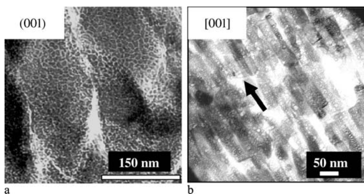
Fig. 26 Nano-structuring of the seeds of the fractal aggregates of fluorapatite-gelatine-nanocomposite. a TEM image of an ultra thin slice of a seed oriented parallel to [001] : the parallel arrangement of elongated subunits follows the principles of self-similarity. b TEM image of an ultra thin slice oriented perpendicular to [001] : the nano-structure with its grain boundaries corresponds to a hexagonal material
