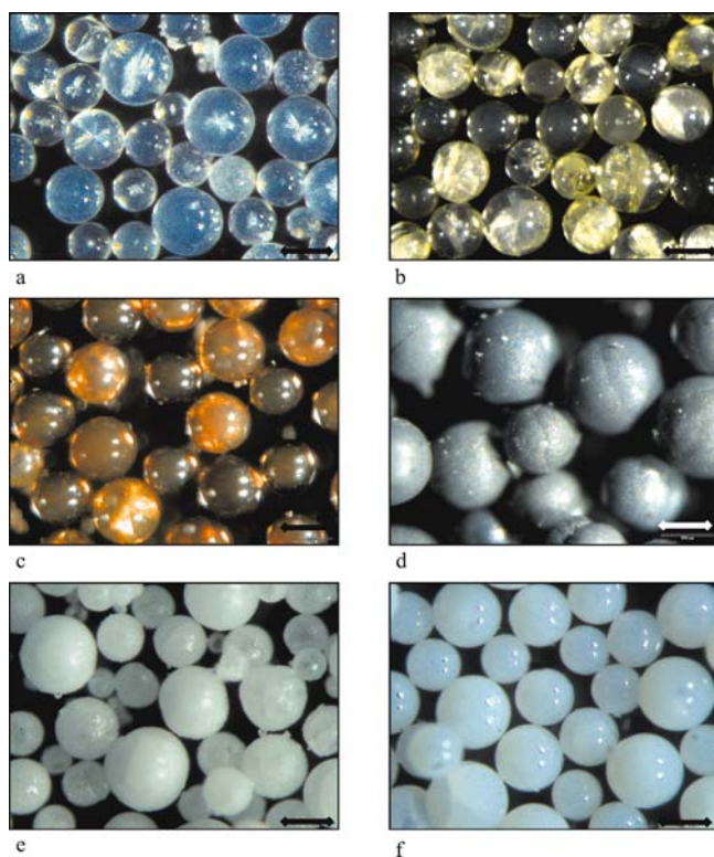
Fig. 20 Photographs of composite spheres heated to different temperatures under an optical microscope using a temperature increase of 30 °C/min. Scale bars in the lower right correspond to 100 µm: a room temperature, b 250 °C, c 400 °C, d 700 °C, e 1000 °C. The decomposition of the gelatine is accompanied by a color change from translucent over yellow to red , black and finally to white . f Treatment of the aggregates with boiling water for seven days leads to a loss of translucency
