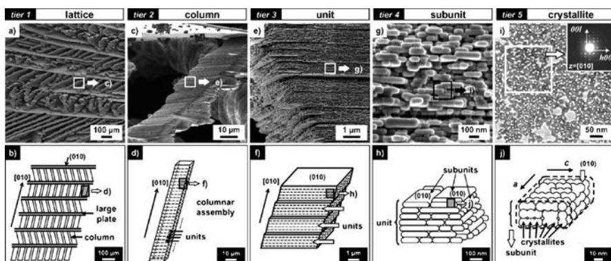
Fig. 25 Hierarchical architecture of K_2SO_4 grown with PAA: a, b the macroscopic lattice architecture (tier 1), c, d columns between plates (tier 2), e, f platy units in the columns (tier 3), g, h granular subunits inside of a unit (tier 4), and i, j crystallites with the same orientation in a subunit (tier 5). Reproduced from [113] with permission of Wiley
