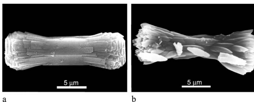
Fig. 45 SEM images of mature composite seeds showing the start of “splitting” a without an external field b with an applied external field (5000 V/1.4 cm)
