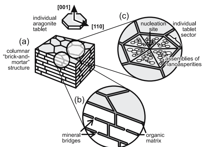
Fig. 7 Schematic illustration of the multiscale hierarchical structure of nacre: a 10 \mu\text{m} length scale, b , c 2 \mu\text{m} length scale, showing individual tablet features at a 200 nm length scale consisting of assemblies of nanoasperities. (Scheme redrawn after [55]). In “columnar” nacre, the tablets are relatively uniform in size and stacked vertically along the c -axis direction (with a slightly staggered arrangement laterally), thereby forming microlaminate sheets and tessellated bands. A domain structure has been found parallel to the c -axis direction consisting of 3–10 tablets with a -axes parallel to each other, while in the plane of the sheet, the a -axis orientation is variable
