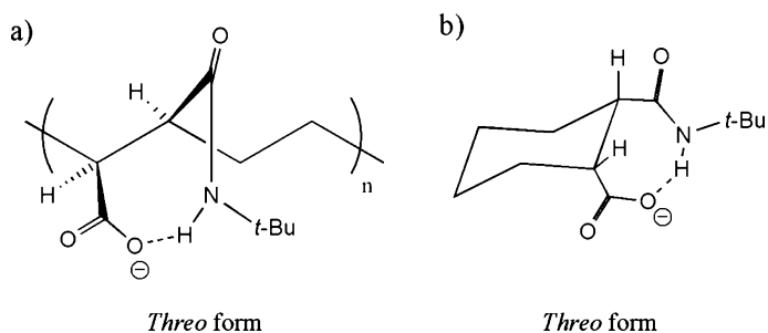
Fig. 17 a A possible structure of poly[1-carboxylate-2-( N - t -butylcarbamoyl)ethylene- alt -ethylene] in threo form and b a possible structure of ( S , R )-2-( N - t -butylcarbamoyl)cyclohexanecarboxylate in threo form
