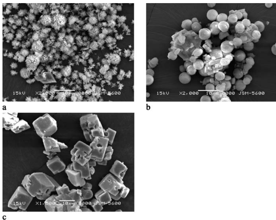
Fig. 8 Scanning electron micrographs of \text{CaCO}_3 from the products of run 1 (a), run 2 (b), and run 3 (c) in Table 1. (Reproduced with permission from [97]. Copyright 2004 The Chemical Society of Japan)
