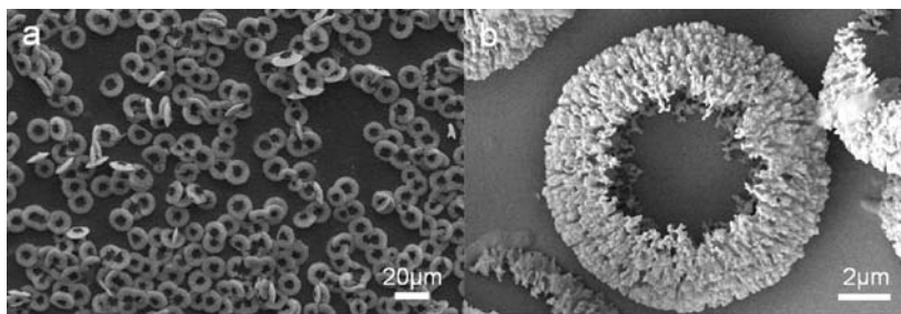
Fig. 7 SEM images of \text{CaCO}_3 microrings; 2.0\text{ g L}^{-1} PEG- b -PEIPA- C_{17} , 15 days, starting pH 4, [\text{CaCl}_2] = 20\text{ mM} . (Reproduced from [156], © 2006, American Chemical Society)
