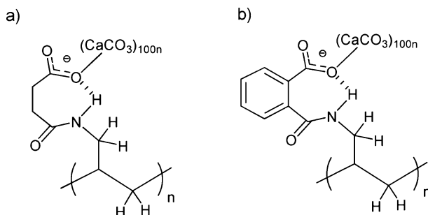
Fig. 19 Polycarboxylate/CaCO 3 composite with 7-membered ring NH \cdots O hydrogen bonds including a succinate and b phthalate in side chains
