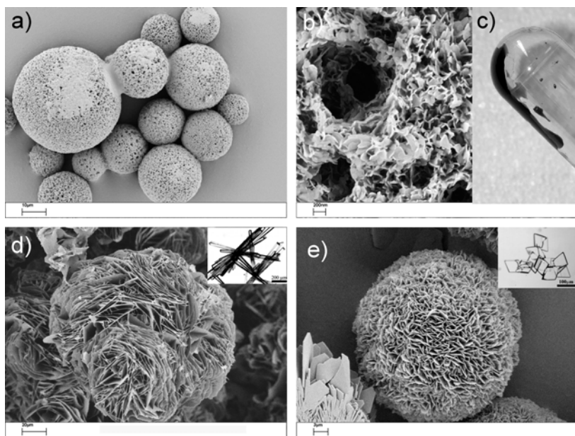
Fig. 12 a DL-Glutamic acid crystals obtained from a concentrated PILP precursor phase with PEI. b Zoom in of a showing the porous structure and the nanoplate building units. c Experimental proof of the liquid character of a DL-glutamic acid PILP phase after centrifugation and removal of the supernatant aqueous phase. d L-Histidine crystals obtained from a concentrated PILP precursor phase with PAA. e L-Lysine crystals obtained from a concentrated PILP precursor phase with PAA. The insets show the default crystals without additives. Scale bars represent a 10 \mu\text{m} , b 200 nm, d 20 \mu\text{m} , and e 3 \mu\text{m} . Figure reproduced from [141] with permission of Wiley
