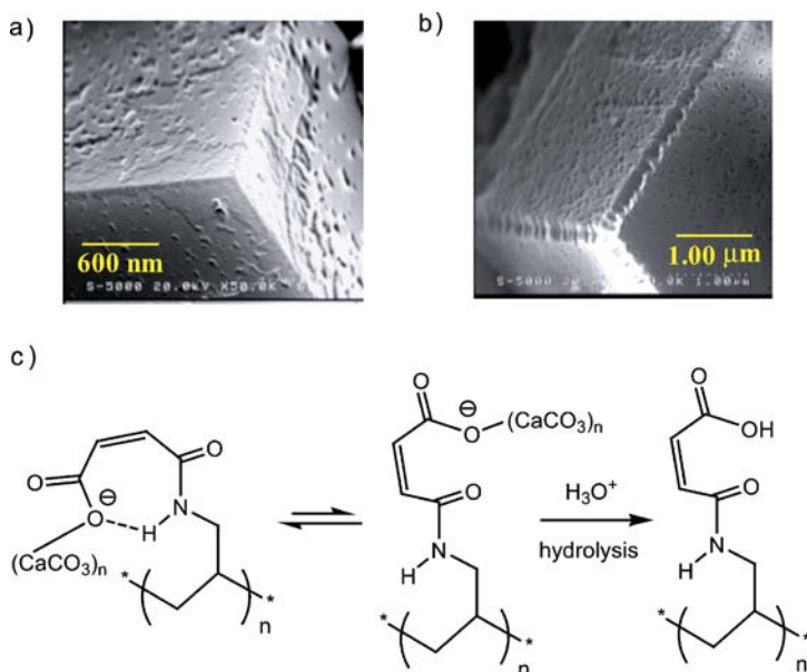
Fig. 26 FE/SEM images of \text{CaCO}_3 /poly[( Z )-3-allylcarbamoyl-2-propenate] composite a before washing with MeOH/water and b after the washing. c The schematic conformational change of poly[( Z )-3-allylcarbamoyl-2-propenate] on the surface of \text{CaCO}_3 composite
