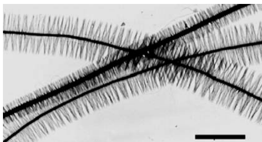
Fig. 30 TEM image of penniform BaWO 4 nanostructures obtained in the presence of 0.5 g L -1 PEO- b -PMAA after aging for 8 h in reverse micelles. Scale bar represents 5 \mu m. Reprinted in part from [357] with permission of the American Chemical Society
