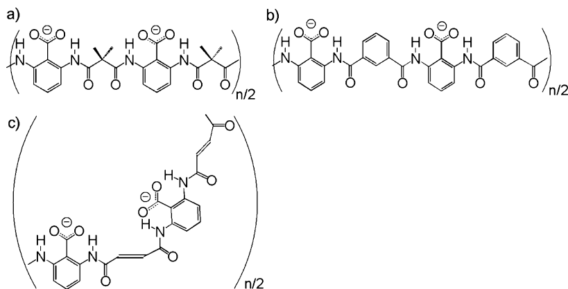
Fig. 13 Synthetic rigid polycarboxylates with intramolecular \text{NH} \cdots \text{O} hydrogen bonds. a \{\text{NHC}_6\text{H}_3(\text{COO}^-)\text{NHCOC}(\text{CH}_3)_2\text{CO}\}_n , b \{\text{NHC}_6\text{H}_3(\text{COO}^-)\text{NHCO-}m\text{-C}_6\text{H}_4\text{CO}\}_n , and c \{\text{NHC}_6\text{H}_3(\text{COO}^-)\text{NHCOCH}=\text{CHCO}\}_n
