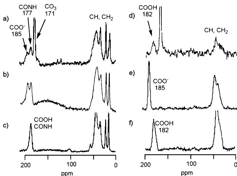
Fig. 15 Solid-state 13 C CP/MAS spectra of a CaCO 3 /poly(1-carboxylate-3- N - n -BuNHCO C 4 H 6 ) composite, b poly(1-carboxylate-3- N - n -BuNHCOC 4 H 6 Na salt), c poly(1-carboxyl-3- N - t -BuNHCOC 4 H 6 ), d CaCO 3 /poly(acrylate) composite, e poly(acrylate Na salt), and f poly(acrylic acid) at 303 K
