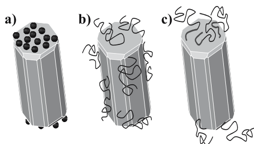
Fig. 19 Face-selective adsorption of ions or low molar mass additives ( a ), steric particle stabilization by polymers ( b ), and face-selective adsorption and particle stabilization by DHBC ( c ). Figure reproduced from [57] with permission of the Royal Society of Chemistry
