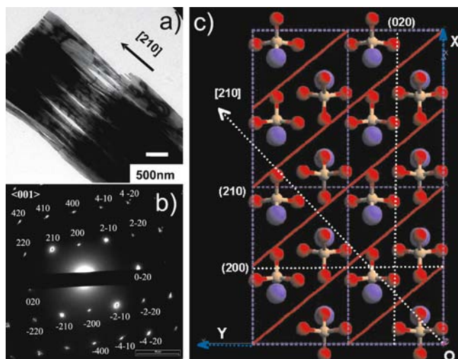
Fig. 25 a TEM image of highly ordered \text{BaCrO}_4 nanofibers obtained in the presence of PEO- b -PMAA- \text{PO}_3\text{H}_2 , pH 5. b Electron diffraction pattern taken along the [001] zone, showing that the fiber bundles are well-crystallized single crystals and elongated along (210) . c Plot of the \text{BaCrO}_4 crystal structure as calculated with the Cerius 2 software viewed perpendicular to the (210) axis (indicated by white dashed arrow ). Blue = Ba, red = O, light brown = C. The red lines are (210) faces. a,b reprinted from [110] and c from [297] with permission of Wiley
