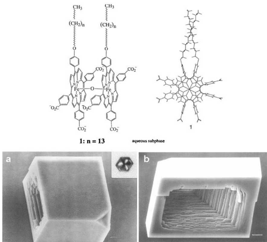
Fig. 13 Top : Molecular structure of the \mu -oxo iron(III) porphyrin dimer. Bottom : SEM images of calcite crystals obtained from nucleation under 1 ( a,b ). a Image of a single calcite crystal showing the truncated corner and cavity on a distal \{10.4\} plane, obtained by the “dipping” method. Inset : An in situ optical micrograph of a calcite crystal nucleated under 1 , viewed from above. b View of the rectangular projections and a terraced gallery on adjoining \{10.4\} planes distal to the truncated corner. The scale bar represents 5 \mu\text{m} . (Reproduced from [198], © 1997, American Chemical Society)
