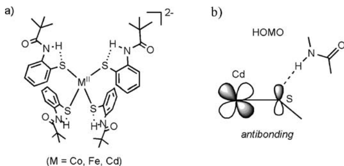
Fig. 2 Molecular structure of a [\text{M}^{\text{II}}(\text{S}-t\text{-BuCONHC}_6\text{H}_4)_4]^{2-} (M = Co, Fe, Cd) with intramolecular \text{NH} \cdots \text{S} hydrogen bond and b antibonding interaction of Cd–S in HOMO of [\text{Cd}^{\text{II}}(\text{S}-t\text{-BuCONHC}_6\text{H}_4)_4]^{2-} affected by amide NH
