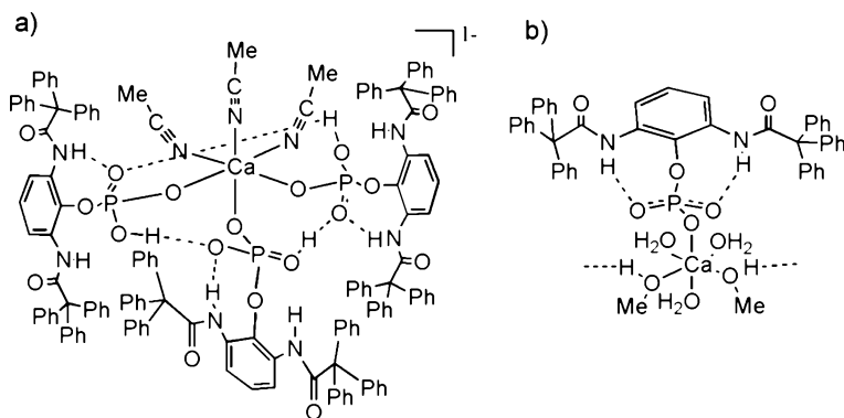
Fig. 9 Molecular structures of a (\text{NMe}_4)[\text{Ca}^{\text{II}}\{\text{O}_2\text{P}(\text{OH})\text{OC}_6\text{H}_3\text{-2,6-(NHCOCPh}_3)_2\}_3(\text{N} \equiv \text{CMe})_3] and b a phosphate dianion, [\text{Ca}^{\text{II}}\{\text{O}_3\text{POC}_6\text{H}_3\text{-2,6-(NHCOCPh}_3)_2\}(\text{H}_2\text{O})_3(\text{MeOH})_2]
