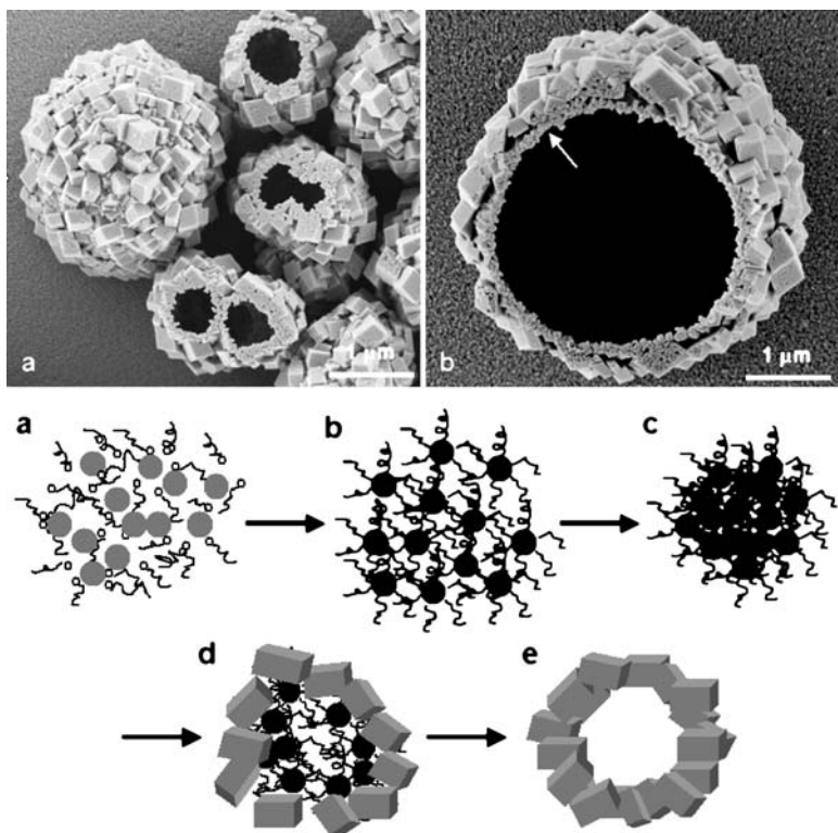
Fig. 27 Top: SEM images of \text{CaCO}_3 particles grown on a glass slip in the early reaction stage, PEO- b -PMAA, [\text{CaCl}_2] = 10 \text{ mM} , 1 \text{ g L}^{-1} , 5 h. a \text{CaCO}_3 particles with either spherical or hollow structures. b Zoom showing the calcite rhombohedral subunits grown on the surface of the hollow structure and the inner part consisting of tiny primary nanocrystals with a grain size of about 320 nm as indicated by the arrow (sacrificial vaterite template). Bottom: Proposed formation mechanism of the calcite hollow spheres: a polymer-stabilized amorphous nanoparticles; b Formation of spherical vaterite precursors; c aggregation of the vaterite nanoparticles; d vaterite–calcite transformation starting on the outer sphere of the particles; e formation of calcite hollow spheres under consumption of the sacrificial vaterite precursors. Reproduced in part from [61] with permission of the American Chemical Society
