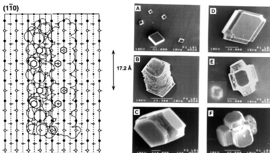
Fig. 3 Left: The footprint of two \alpha -helical peptide (CBP1) molecules binding to the (110) prism faces of calcite. The filled circles are \text{Ca}^{2+} ions, and open circles are \text{CO}_3^{2-} ions. Large circles are ions in the plane of the surface and small circles are 1.28 Å behind this plane. The hexagons indicate that peptide carboxylate ions occupy \text{CO}_3^{2-} sites on the corrugated surface. Right: SEM micrographs showing the effect of CBP1 on the growth of calcite crystals: a Calcite seed crystals showing typical rhombohedral morphology. b Elongated calcite crystals formed from seed crystals at 3 °C in saturated \text{Ca}(\text{HCO}_3)_2 containing ca. 0.2 mM CBP1, showing expression of new surfaces corresponding to the prism faces and rhombohedral (104) caps; growth is along the c -axis, which extends through the vertices of the end caps. c “Repair” and re-expression of rhombohedral surfaces when crystals from b are allowed to grow in saturated \text{Ca}(\text{HCO}_3)_2 after removal of CBP1 solution. d,e Respective earlier and later stages of growth of calcite crystals from rhombohedral seed crystals at 25 °C in saturated \text{Ca}(\text{HCO}_3)_2 containing ca. 0.2 mM CBP1, showing epitaxial growth from the rhombohedral surfaces. e inset: Fluorescence micrograph of epitaxial studded calcite crystals grown under similar conditions in the presence of fluorescein-labeled CBP1; the dark spot in the center corresponds to a (104) face, indicating that the peptide is binding to the newly expressed surfaces and not (104). f “Repair” and re-expression of rhombohedral surfaces when crystals from e are allowed to grow in saturated \text{Ca}(\text{HCO}_3)_2 after removal of CBP1. Reproduced in part from [92] with permission of the American Chemical Society
