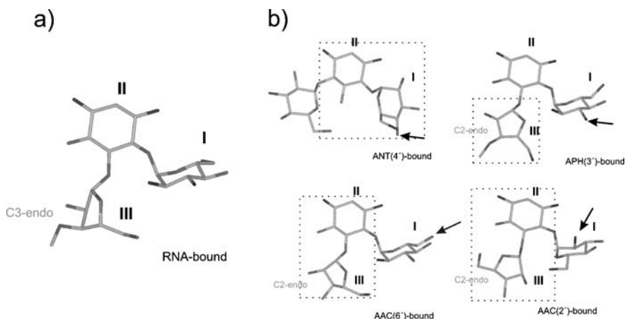
Fig. 7 Schematic representation of the conformational differences ( highlighted with a dotted box ) exhibited by aminoglycosides in the binding pockets of RNA ( a ) and some of the enzymes involved in bacterial resistance ( b ). The glucose, 2-deoxy-streptamine and ribose units are numbered as I, II and III respectively
