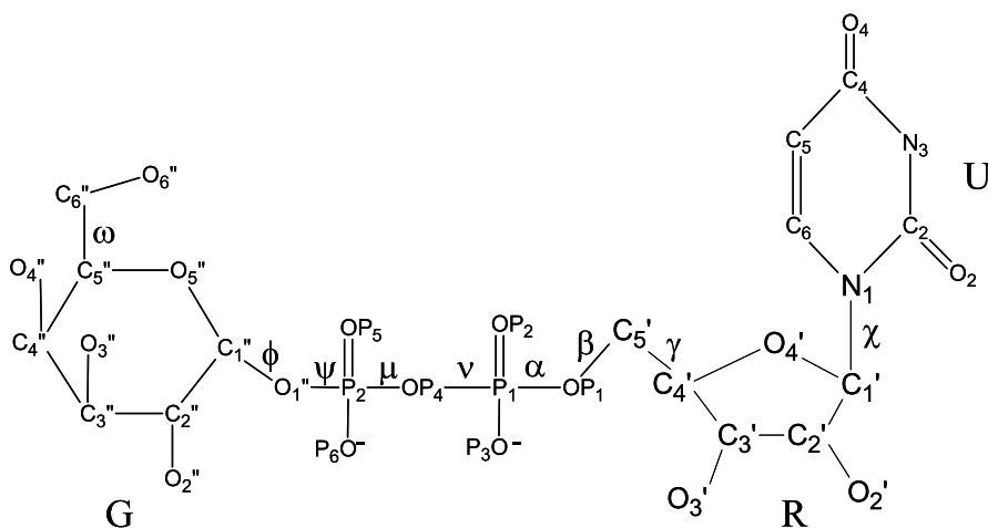
Fig. 8 Structure of UDP-Gal with labeling of the residues ( G galactose, R ribose, U uracil) and torsion angles. Reprinted with permission from [69] (supporting information); © 2004, American Chemical Society
