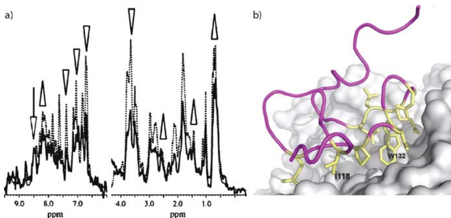
Fig. 4 Third receptor fragment V3 of VLDLR binding to HRV2 as monitored by STD NMR. a Dotted reference spectrum is overlaid with the corresponding STD NMR spectrum (taken from [57]). This data was recorded on a 500 MHz spectrometer with 500-fold excess of V3 over HRV2. Up-arrows highlight resonances with a large relative saturation transfer. down-arrows indicate resonances that received less relative saturation. b The complex as derived from a cocrystal structure (pdbcode: 1V9U) [28]. Amino acid side chains from V3 closer than 5.0 Å to the virus ( white ) are highlighted in yellow . The only aromatic amino acid close to the viral shell is W132 and the only methyl group in a 5.0 Å radius around the virus originates from I118. It is hypothesized that the observed saturation transfer is mainly due to these two amino acids
