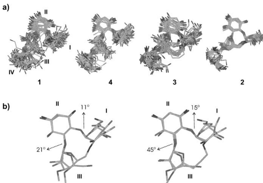
Fig. 10 a MD-tar ensembles of conformers for 2–4. The experimental ensemble corresponding to 1 in the free state ( left ) is shown for comparison. b Structures representative of the main conformational families present in solution for neomycin-B derivatives 2 ( left ) and 3 ( right ) superimposed on the X-Ray structure of paromomycin in the complex with ribosomal RNA, according to X-Ray data. The maximum \Phi/\Psi deviations (for each glycosidic linkage) is shown. Unit IV is omitted for simplicity
