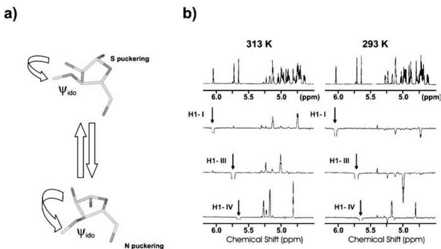
Fig. 3 a 1 : 3 syn-diaxial interactions established by OH2 III and OH5 III with the vicinal OH3 III group are dependent on the ring III conformation. b Dependency exhibited by the intrasidue NOEs on temperature for the different sugar units. Selective NOEs obtained upon inversion of the three anomeric protons at 313 K ( left ) and 293 K ( right )
