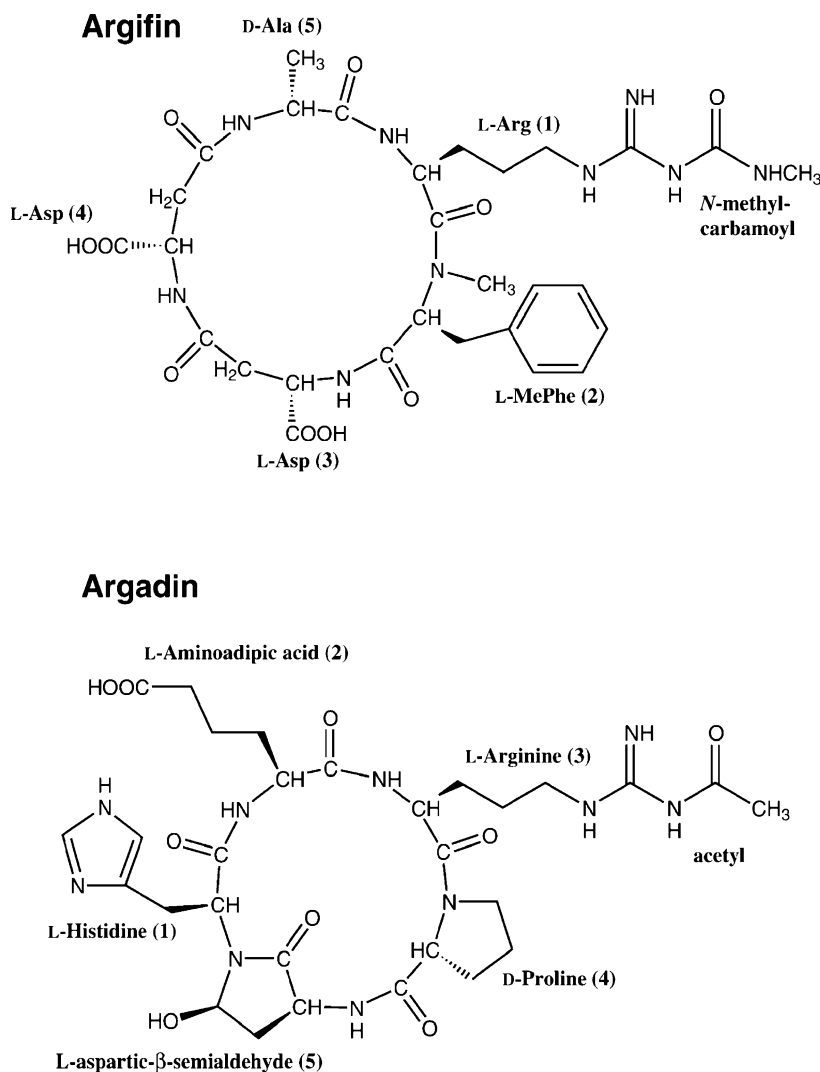
Fig. 13 The chemical structures of argifin and argadin. Reproduced with permission from [170]. © 2005 Elsevier Science
