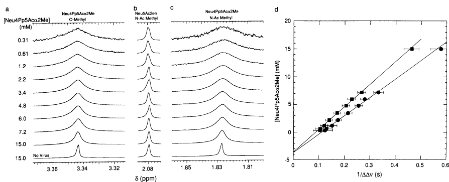
Fig. 1 ^1\text{H} NMR titration of Neu4PpAc2Me in the presence of 3 mg mL ^{-1} Influenza (H3N2) virus [37]. Two ligand resonances are observed: (a) O-methyl and (b) N-Ac methyl. The N-Ac methyl resonance of the neuraminidase inhibitor Neu5Ac2en (c) was used as a reference to calculate \Delta\Delta\nu = (\Delta\nu_{\text{Neu4PpAc2Me}} - \Delta\nu_{\text{Neu5Ac2en}})_{\text{virus}} - (\Delta\nu_{\text{Neu4PpAc2Me}} - \Delta\nu_{\text{Neu5Ac2en}})_{\text{no virus}} . d Linear regression analysis of titration of N-Ac methyl (●) and 2-O-methyl of Neu4PpAc2Me (■), which yield -K_D (y-intercept). The error in broadening was estimated using the square root of the signal-to-noise ratio or the digital resolution, whichever was higher. The data were acquired at 500 MHz. (With permission of Virology.)
