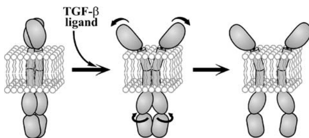
Fig. 5 Possible motions of the type II receptors during interaction with the TGF- \beta ligand. Binding of the ligand to the T \beta RII receptor homodimer induces rotation and swinging of the extracellular domains, which are translated through the transmembrane parts into rearrangements of intracellular domains by means of a “flexible rotation” mechanism, finally causing dissolution of the dimer and spatial separation of the receptor monomers
