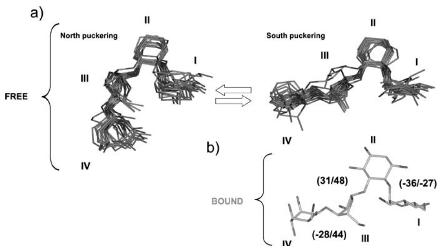
Fig. 5 a Neomycin-B conformational families characterized by “N” (left) and “S” (right) ribose (ring III) puckering obtained from the MD-tar calculations. The global shape of neomycin-B is extremely dependent on the precise puckering of this unit. Only the skeleton carbon and oxygen atoms are shown for clarity. b Structure of the neomycin-B related antibiotic paromomycin bound to the A-site. The \Phi/\Psi values for the three glycosidic linkages are indicated
