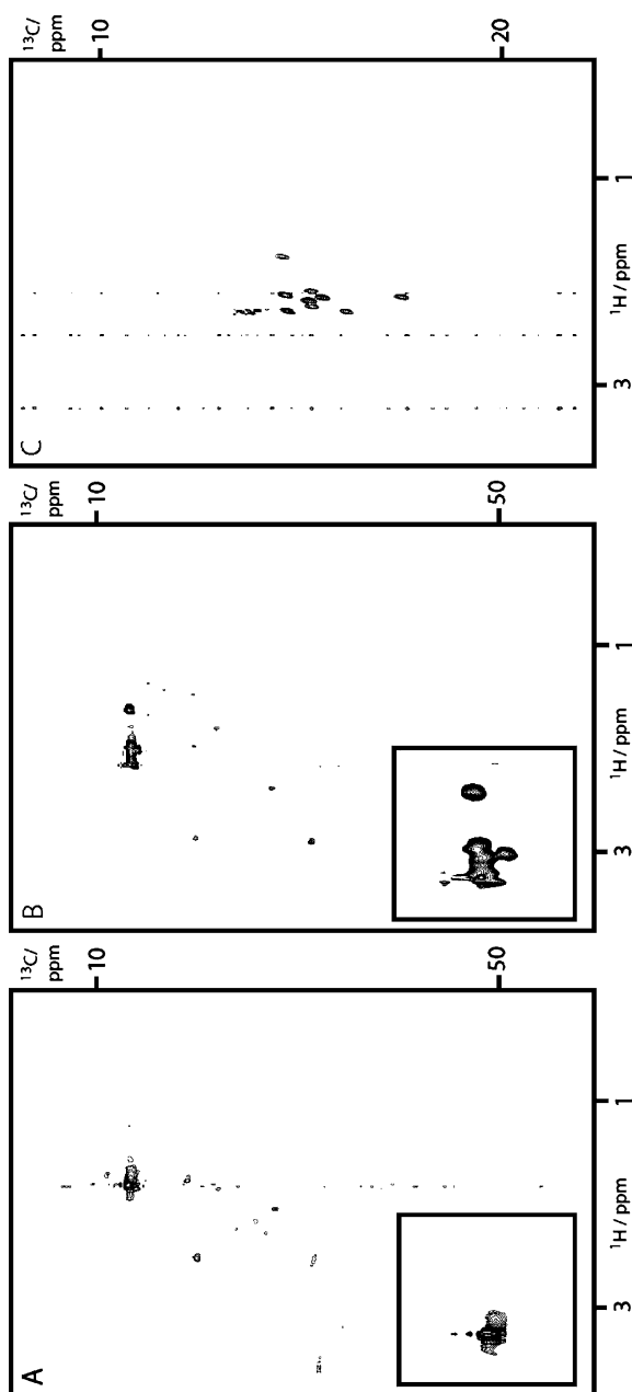
Fig. 4 Comparison of background levels in ^{13}\text{C} , ^1\text{H} -HSQC spectra of bacterial samples grown on ^{13}\text{C} -methyl group labeled methionine without over-expression (A) and with over-expression of calmodulin (B). The spectrum in C was measured with a smaller spectral width as the spectrum in B. Only the free methionine and the nine methionine resonances of calmodulin are visible. Reprinted with permission from Serber et al., 2004
