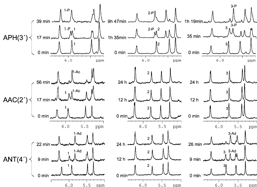
Fig. 12 Time evolution (at pH 7.0 and 310 K) of neomycin-B (1, left), derivative 2 (middle) and derivative 3 (right) at 100 \mu M concentration in the presence of ATP or AcCoA (100 \mu M), after addition of 0.2 \mu M ANT(4') (lower part), AAC(2') (middle) or APH(3') (upper part) followed by 1-D NMR. 1-Ad and 3-Ad stand for the adenylated derivatives 1 and 3, respectively. 1-Ac stands for the acetylated derivative 1. 1-P, 2-P and 3-P stand for the phosphorylated derivatives 1, 2 and 3, respectively
