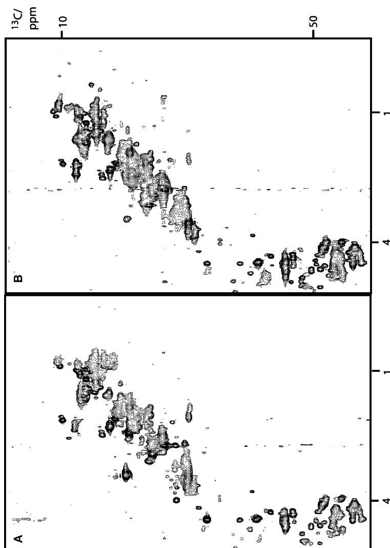
Fig. 3 Sections of two ^{13}\text{C},^1\text{H} -HSQC spectra taken from a bacterial sample grown on minimal medium containing ^{13}\text{C} -labeled glucose with (A) and without (B) overexpression of calmodulin. Reprinted with permission from Serber et al., 2004
