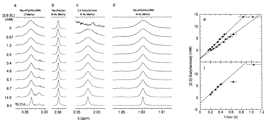
Fig. 2 ^1\text{H} NMR titration of \alpha(2,6) sialyllactose using Neu4Pp5Ac \alpha 2Me as a reporter ligand [37]. While Neu4Pp5Ac \alpha 2Me was present at a constant concentration of 1 mM, \alpha(2,6) sialyllactose was titrated into the solution in presence of the 2 mg mL ^{-1} H3N2 Influenza virus. A decrease in line broadening of the O-methyl (a) and N-Ac methyl (d) resonances of Neu4Pp5Ac \alpha 2Me can be observed when the concentration of \alpha(2,6) sialyllactose is increased. To calculate \Delta\Delta\nu , the N-Ac methyl resonance of the Neu5Ac2en (b) is used. c N-Ac methyl resonances of \alpha(2,6) sialyllactose. Linear regression analysis of e N-Ac methyl (●) and 2-O-methyl (■) of Neu4Pp5Ac \alpha 2Me, and f 2-O-methyl (▲) of \alpha(2,6) sialyllactose. The known K_{\text{D}}(\text{Neu4Pp5Ac}\alpha 2\text{Me}) = 3.6 mM of the reporter ligand was used to derive K_{\text{D}}(\alpha(2,6)\text{sialyllactose}) by following the equation: y-intercept = -K_{\text{D}}(\alpha(2,6)\text{sialyllactose})(1 + [\text{Neu4Pp5Ac}\alpha 2\text{Me}]/K_{\text{D}}(\text{Neu4Pp5Ac}\alpha 2\text{Me})) . (With permission of Virology.)
