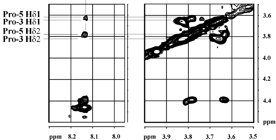
Fig. 9 TrNOESY and QUIET-trNOESY spectra of the peptide DRPVVPY in the presence of the antibody SA-3. A Regions of a trNOESY spectrum ( \tau_m = 200 ms) showing Val-4 HN-Pro-3,-5 H \delta cross-peaks and Pro-3,-5 H \delta -H \delta cross-peaks. B Corresponding regions of a QUIET-trNOESY spectrum ( \tau_m = 200 ms) with inversion of 0.75 ppm wide bands centered at 4.15 ppm and 8.1 ppm; within the intersection of the quiet bands (quiet window), the Val HN-Pro-5 H \delta cross-peaks are still present, while the Val HN-Pro-3 H \delta_2 cross-peak is absent, indicating cancellation due to spin diffusion. Reproduced with permission from [125]. © 2002 American Chemical Society
