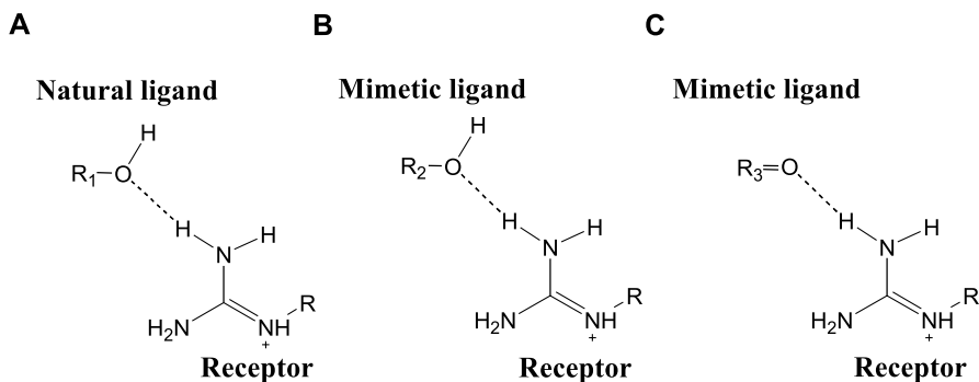
Scheme 1 Examples of structural mimicry
