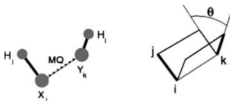
Fig. 1 Cross-correlated relaxation: Interaction between magnetic moments are dependent on the angle between them. This interaction is only present for large proteins or protein-ligand complexes
