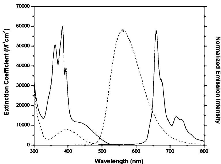
Fig. 8 Absorption ( left ) and emission ( right ) spectra of the bis-(pyrenylacetylide) platinum complex 13 ( solid lines ) and of Pt(dbbpy)(-C≡C-Ph) 2 for comparison ( dotted lines ) in deoxygenated CH 2 Cl 2 at room temperature; \lambda_{\text{ex}} = 480 nm. Reprinted with permission from [32]. © (2003) American Chemical Society
