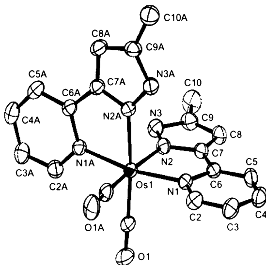
Fig. 2 X-ray structure of [\text{Os}(\text{fppz})_2(\text{CO})_2] [26]
