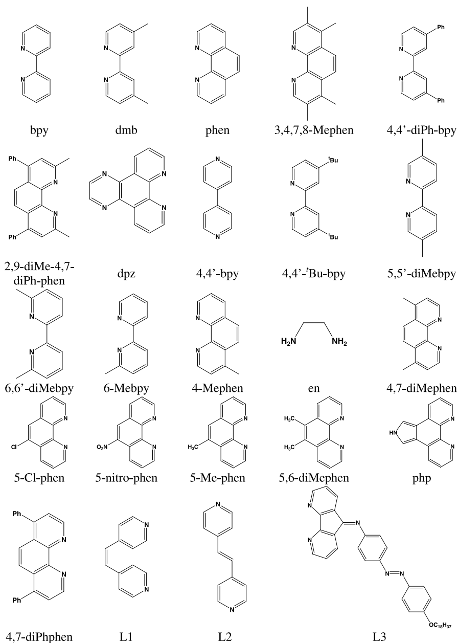
Fig. 5 Structures of ligands with acronyms and L1–L3
