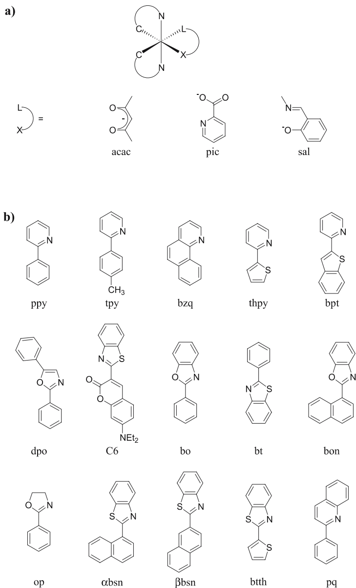
Fig. 5 a (XL) ligands of neutral (C^N)_2Ir(LX) complexes of Table 3; b (C^N) ligands of the neutral (C^N)_2Ir(LX) complexes of Table 3
