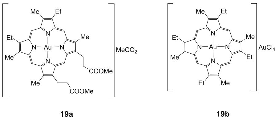
Fig. 25 Structure of 19a and 19b
