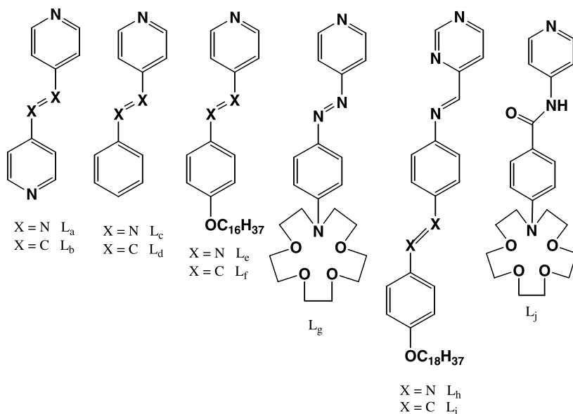
Fig. 16 Azo, ethylenic and crown ligands
