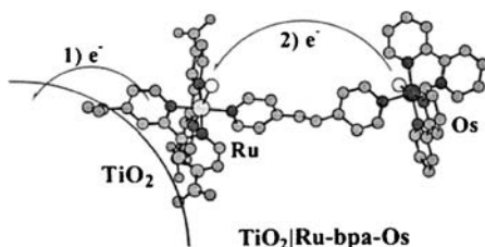
Fig. 20 Photoinduced charge injection into \text{TiO}_2 and subsequent hole migration to the Os(II) center in [(\text{dcb})_2\text{Ru}(\text{Cl})(\text{bpa})\text{Os}(\text{Cl})(\text{bpy})_2]^{2+} [116]
