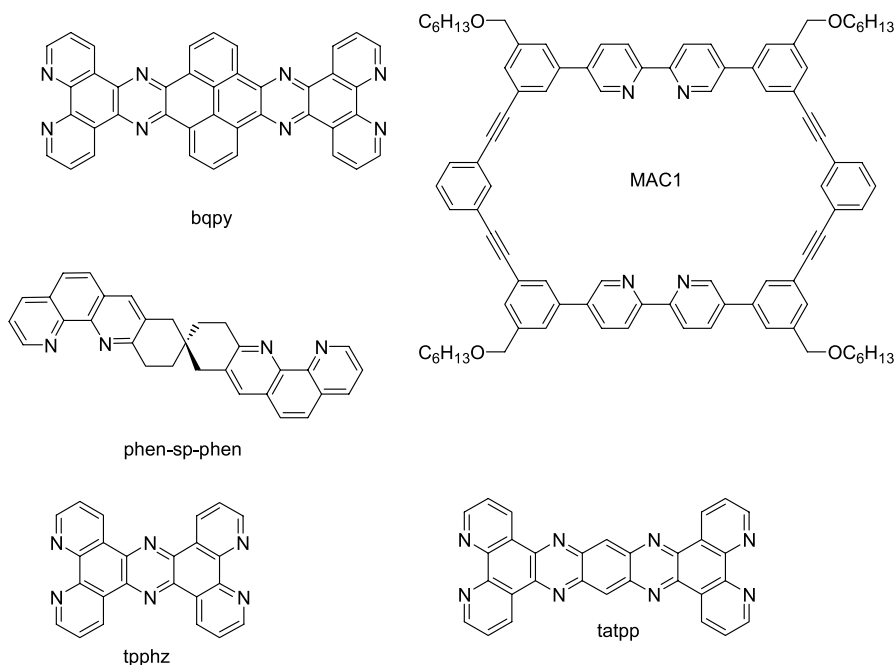
Scheme 2 Structures of bridging ligands
