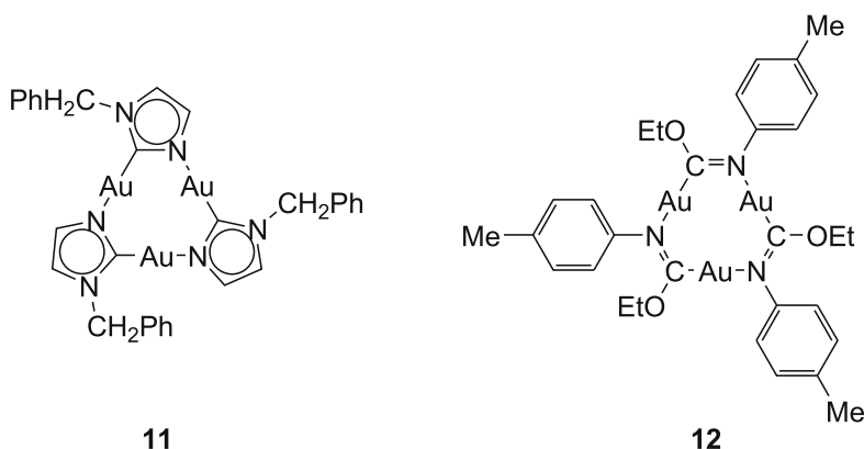
Fig. 15 Structure of the trinuclear gold(I) complexes 11 and 12
