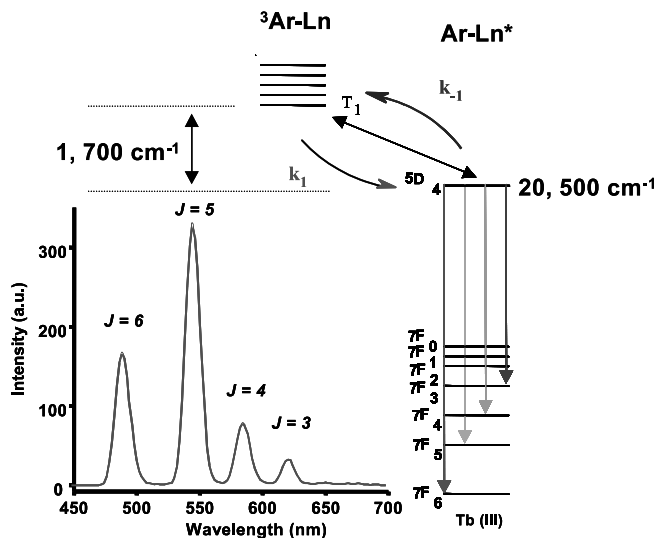
Fig. 1 Illustration of energy transfer to the lanthanide ion in sensitisation process for Tb(III), from triplet state of the antenna and the corresponding emission spectra for Tb(III)
