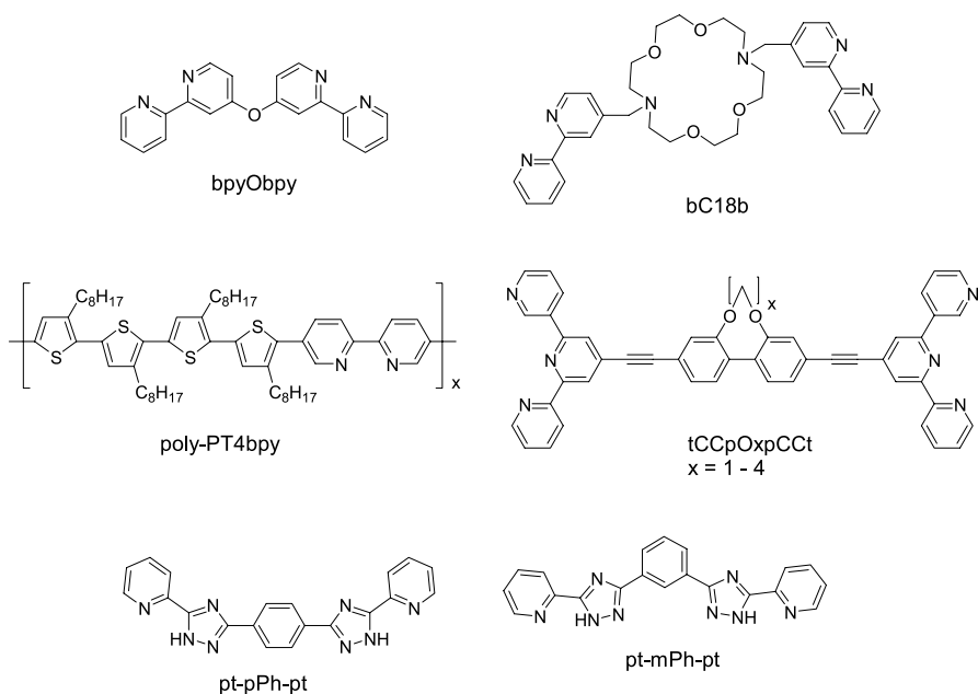
Scheme 5 Structures of bridging ligands
