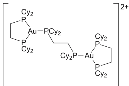
Fig. 3 Structure of the complex cation of [(\mu\text{-dcpe})\{\text{Au}(\text{dcpe})\}_2](\text{PF}_6)_2
