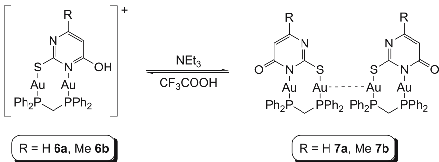
Fig. 10 Acid-base controlled interconversion of 6 and 7
