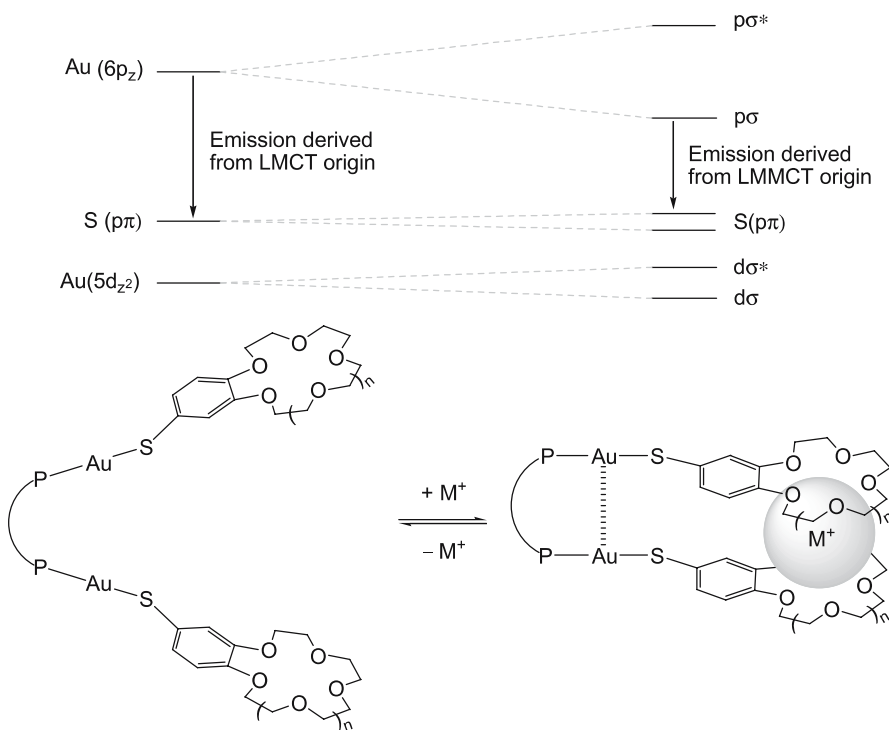
Fig. 7 Red shift in emission energy of binuclear gold(I) thiolate complexes via metal-ion encapsulation
