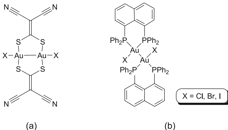
Fig. 19 Luminescent binuclear gold(II) complexes
