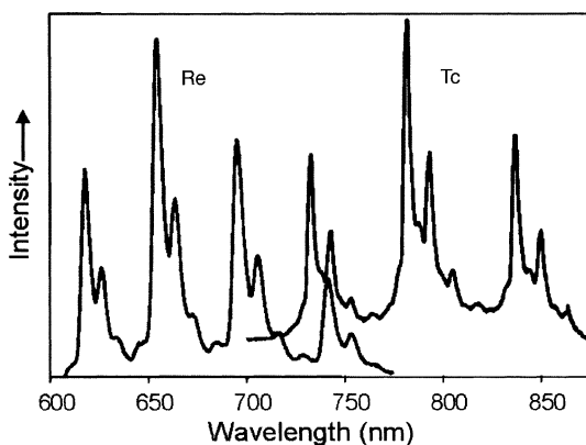
Fig. 4 Structure on the low-temperature emission spectra of [\text{MO}_2(\text{pic})_2]\text{BPh}_4 . Left spectrum is for \text{M}=\text{Re} , right for \text{M}=\text{Tc}
