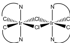
Scheme 2 2\text{IrCl}_3 \cdot n\text{H}_2\text{O} + 4(\text{C}^\wedge\text{NCH}) \rightarrow [(\text{C}^\wedge\text{N})_2\text{Ir}(\mu - \text{Cl})_2\text{Ir}(\text{C}^\wedge\text{N})_2] + 4\text{HCl} + n\text{H}_2\text{O}
