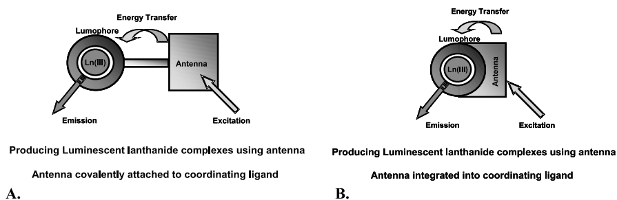
Scheme 4 Two common methods ( A and B ) of incorporating antenna into coordinating ligands
