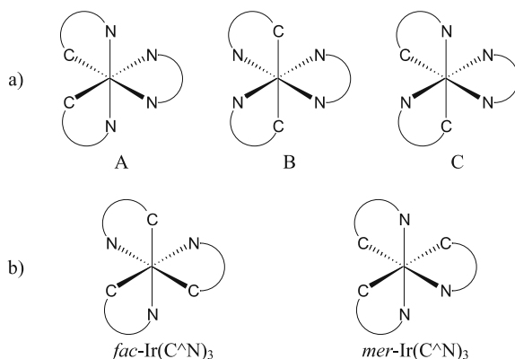
Fig. 4 Geometrical isomers: a A, B, C for \text{Ir}(\text{ppy})_2(\text{bpy})^+ and b fac - \text{Ir}(\text{C}^{\wedge}\text{N})_3 and mer - \text{Ir}(\text{C}^{\wedge}\text{N})_3
