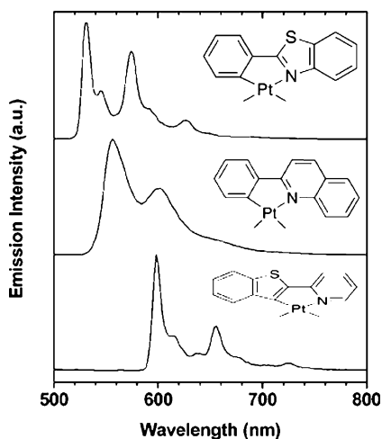
Fig. 20 From top to bottom: Emission spectra of Pt(bt)(dpm), Pt(pq)(dpm), and Pt(btp)(acac), in MeTHF at 77 K. The O ^ O-chelated \beta -diketone ligand is omitted from the structures shown. Reprinted with permission from [109]. © (2002) American Chemical Society
