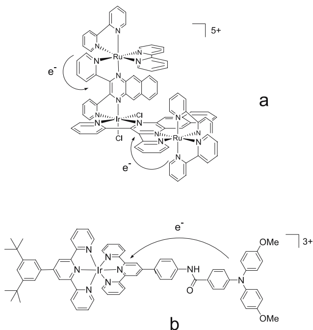
Fig. 26 Schematic structures of arrays, see text; arrows denote electron transfer
