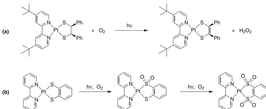
Scheme 2 Photo-oxidation of (a) Pt(dbbpy)(dpdt) leading to the corresponding dithiolene complex [48]; (b) Pt(bpy)(bdt) leading sequentially to the sulfinate and disulfinate complexes [22]
