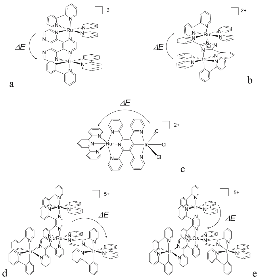
Fig. 22 Schematic structures of polynuclear complexes, see text; arrows denote energy transfer
