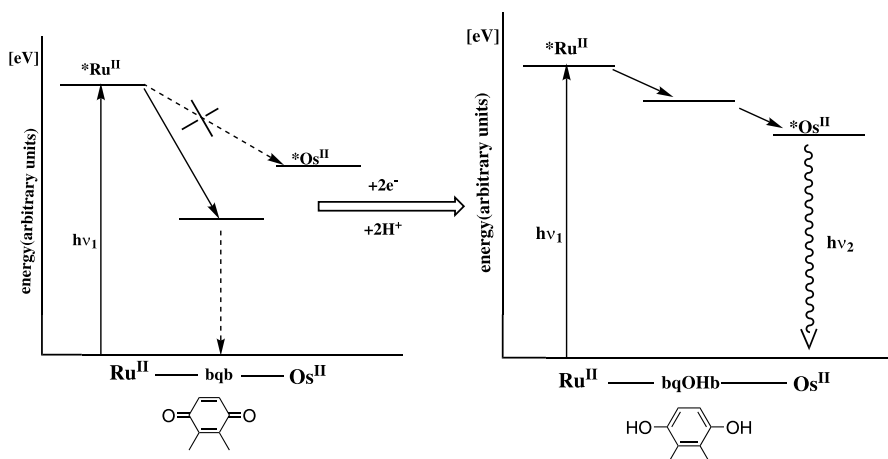
Fig. 9 Energy level diagram indicating redox control of Os(II) complex luminescence [51]
