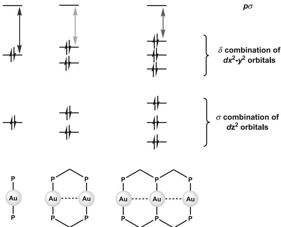
Fig. 1 Schematic molecular orbital diagram showing the effect of aurophilic contacts on the HOMO-LUMO energy gap of gold(I) phosphine complexes
