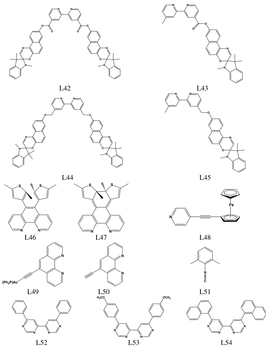
Fig. 8 Structures of ligands L42–L54
