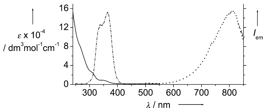
Fig. 5 Electronic absorption (—), emission (···) (excitation at 365 nm) and excitation (– · – · –) (monitored at 810 nm) spectra of 1 in dichloromethane solution at 298 K [29]
