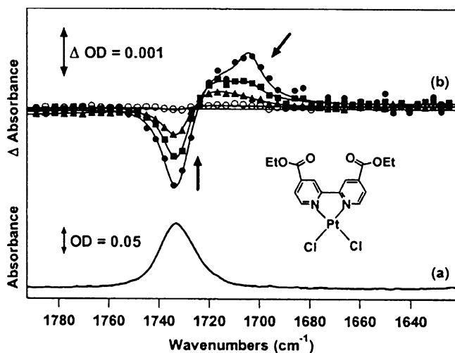
Fig. 6 a Ground-state IR spectrum of \text{Pt}(4,4'-(\text{EtCO}_2)_2\text{-bpy})\text{Cl}_2 in \text{CH}_2\text{Cl}_2 . b TRIR spectra obtained at 1.5 ps (solid circles), 4 ps (squares), 11 ps (triangles) and 50 ps (open circles) after excitation at 400 nm (150 fs pulse). Solid lines represent curve-fitted spectra and arrows indicate movement of the bands with increasing time delay following excitation. Reprinted from [15] by permission of the Royal Society of Chemistry
