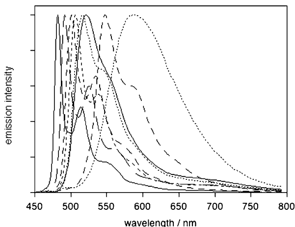
Fig. 23 Emission spectra of N^C^N complexes 49 in \text{CH}_2\text{Cl}_2 ( 10^{-5} M), RT, \lambda_{\text{ex}} = 400 nm. From left to right: R = -\text{CO}_2\text{Me} , H, mesityl, 2-pyridyl, 4-tolyl, 4-biphenyl, 2-thienyl, 4-(dimethyl-amino)phenyl
