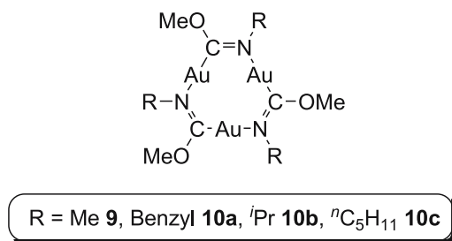
Fig. 14 Solvoluminescent and polymorphic trinuclear gold(I) complex 9 and its related counterparts 10a–c
