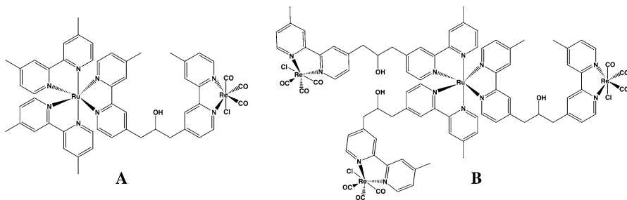
Fig. 20 Multimetallic carbon dioxide reduction photocatalysts
