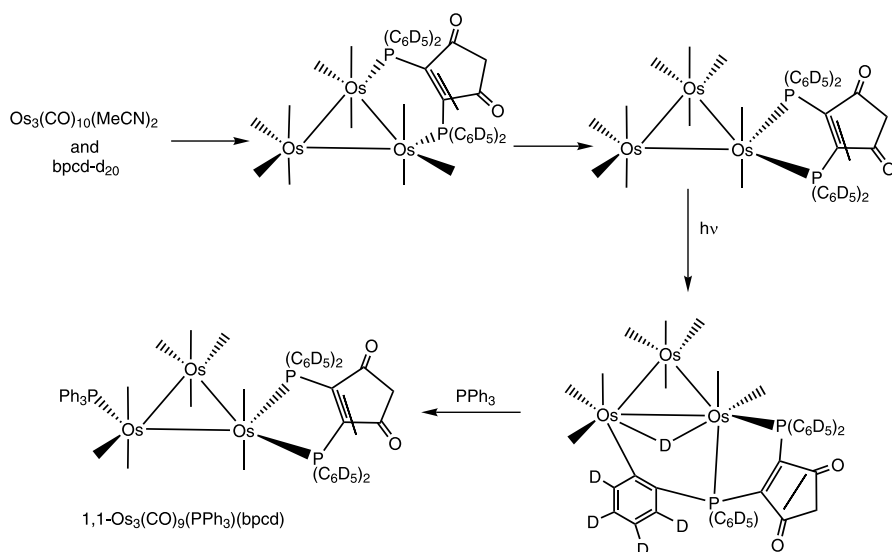
Fig. 17 Products from ultraviolet photolysis of the diphosphine complex [\text{Os}_3(\text{CO})_{10}(\text{bpcd})] [100]
