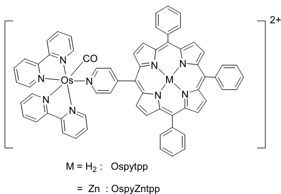
Fig. 7 Os(II) bipyridyl carbonyl complex covalently linked to both free base and Zn(II) tetraphenylporphyrin [45]
