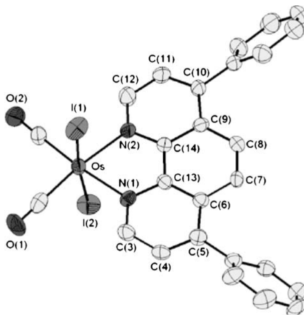
Fig. 3 X-ray structure of [\text{Os}(\text{CO})_2(\text{I})_2(\text{dpphen})] [28]
