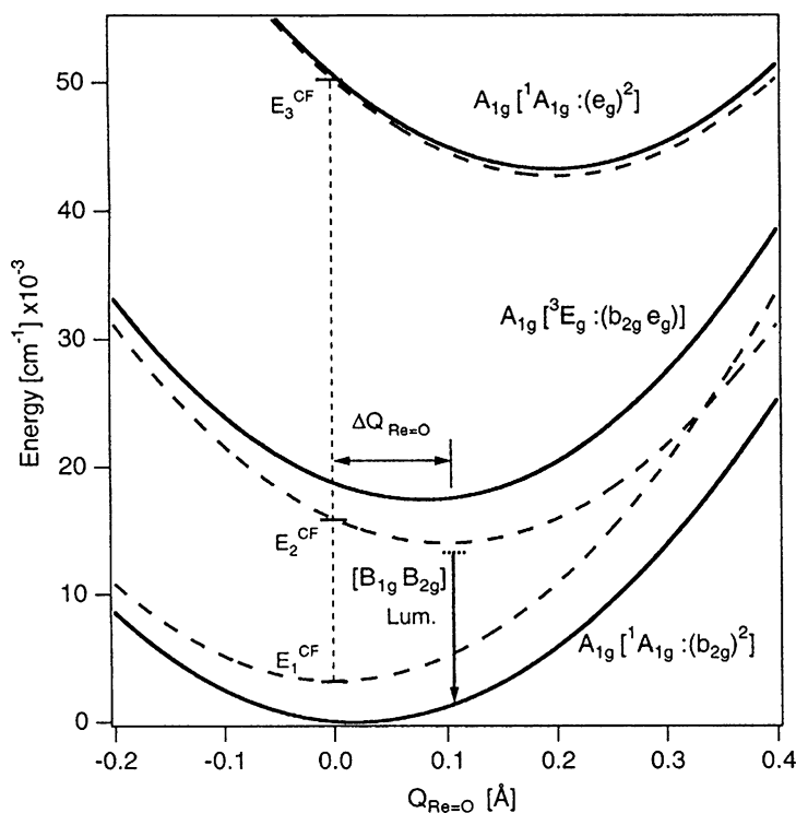
Fig. 2 The model of coupled potential energy surfaces used to explain the vibronic spectral features in Re dioxo complexes. Solid and dashed lines represent adiabatic and diabatic surfaces, respectively. The lowest adiabatic surface corresponds to the electronic ground state used to calculate the luminescence spectra. The crystal field energies for all three A_{1g} states are given along the vertical dashed line
