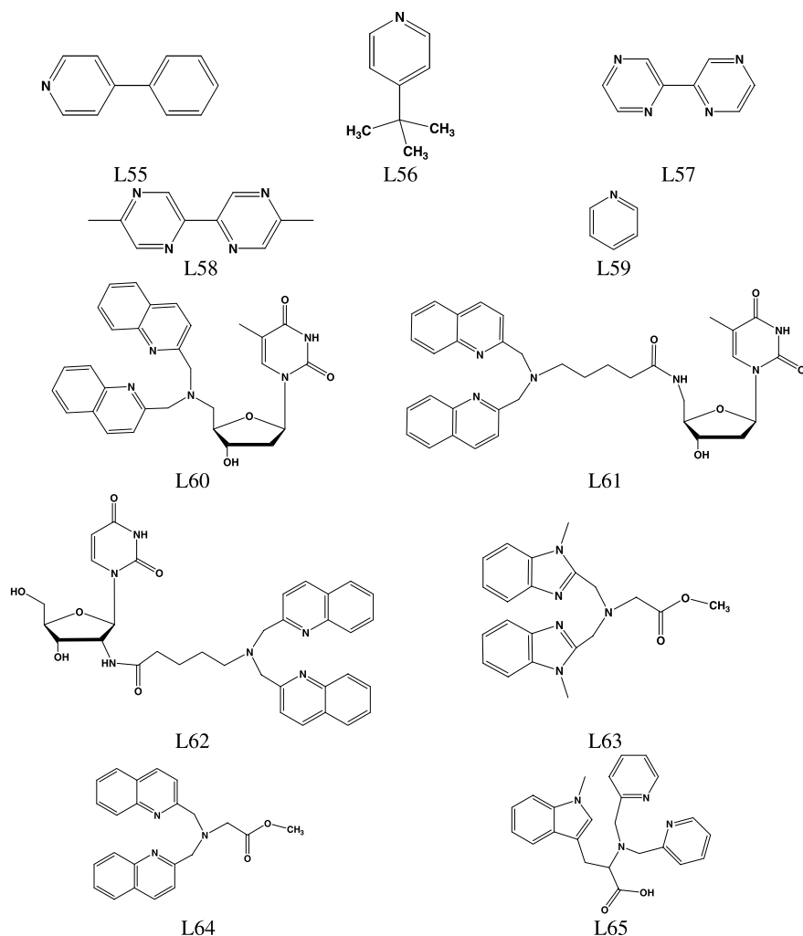
Fig. 9 Structures of ligands L55–L65
