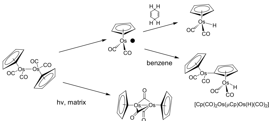
Fig. 16 Photoreactivity of [\text{Cp}_2\text{Os}_2(\text{CO})_4] in frozen matrices and solution [97, 98]
