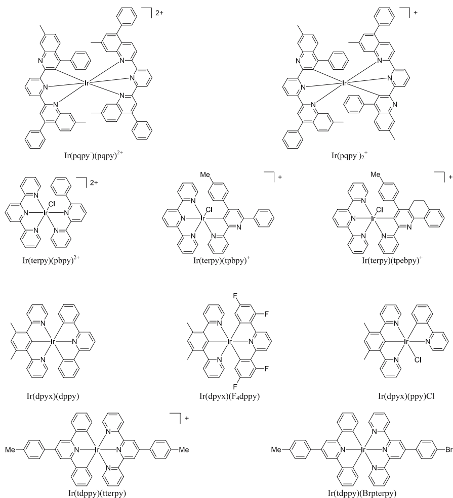
Fig. 18 Schematic structures of cyclometalated bis-terdentate complexes; the two terdentate planar systems are roughly perpendicular to each other
