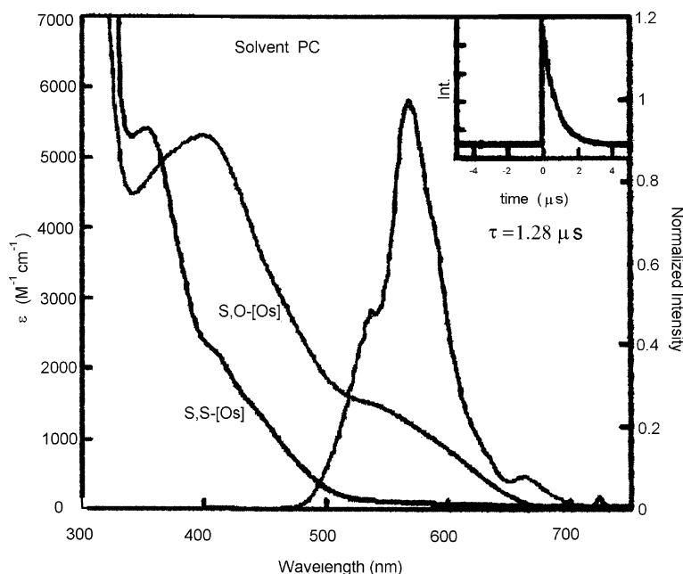
Fig. 4 Absorption and luminescence spectra of [\text{Os}(\text{bpy})_2(\text{DMSO})_2]^{2+} . Spectra shown are for the starting S,S bound bis-DMSO and the photoproduct S,O bound bis-DMSO. The inset shows the luminescence decay of the S,S complex [30]
