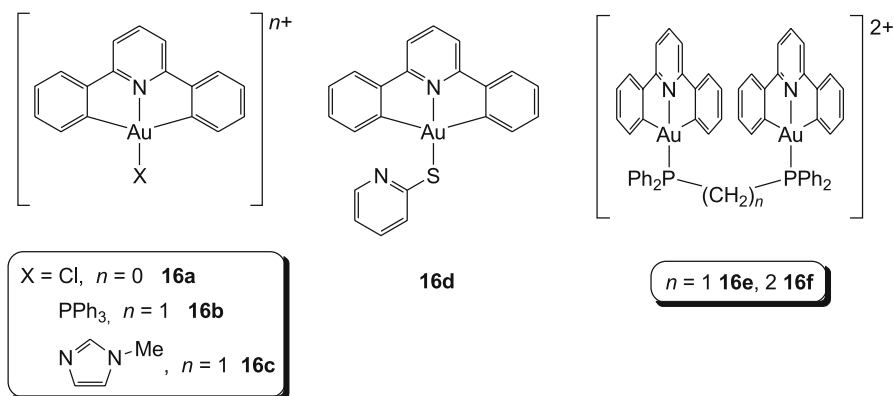
Fig. 22 Structure of the bis-cyclometallated gold(III) complexes 16a–f
