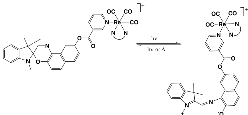
A. Ring-opening, spirooxazines
