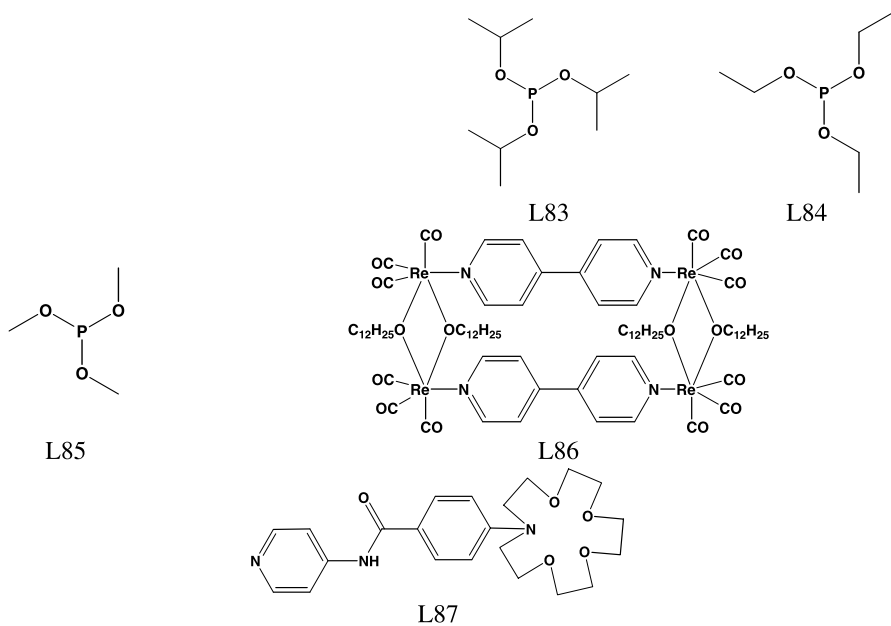
Fig. 12 Structures of ligands L83–L87
