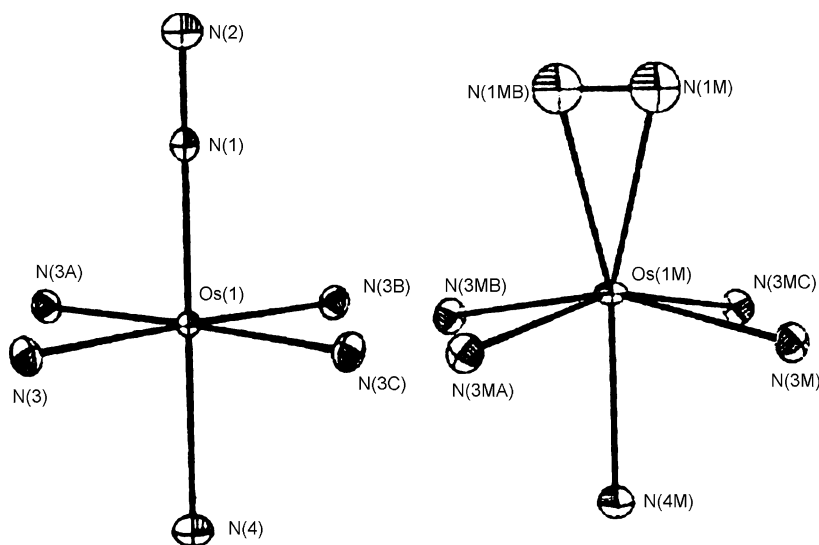
Fig. 5 X-ray structures of end-on and side-bound \text{N}_2 in [\text{Os}(\text{NH}_3)_5(\text{N}_2)]^{2+} [37]
