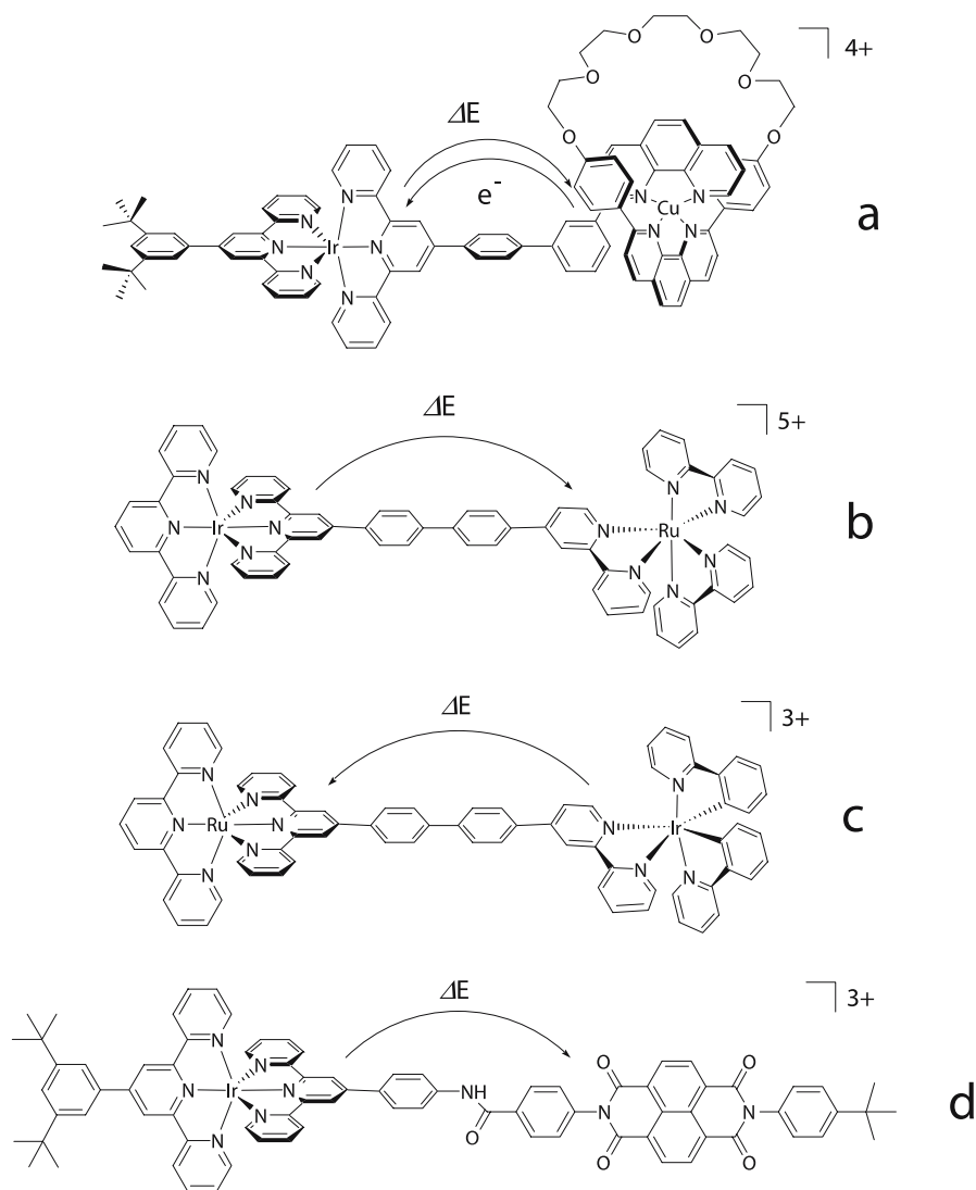
Fig. 25 Schematic structures of arrays, see text; arrows denote energy transfer
