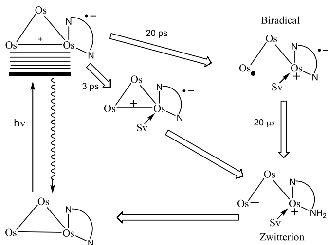
Fig. 15 Formation of zwitterions and biradicals from the diimine clusters [\text{Os}_3(\text{CO})_{10}(\text{LL})] (LL = diimine ligand) [93, 94]
