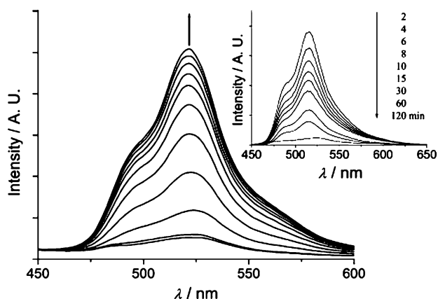
Fig. 9 Growth of the emission from a thin film of \text{Pt}(\text{dbbpy})(-\text{C}\equiv\text{C}-4\text{-py})_2 upon exposure to \text{N}_2 saturated with \text{CH}_2\text{Cl}_2 vapor ( \lambda_{\text{ex}} = 350 \text{ nm} , \text{N}_2 flow rate = 12 \text{ mL min}^{-1} , interval between spectra = 2 min). The inset shows the emission spectral traces for this film upon removal of the \text{CH}_2\text{Cl}_2 vapor ( \text{N}_2 flow rate = 90 \text{ mL min}^{-1} ). Reprinted with permission from [37]. © (2003) Wiley-VCH
