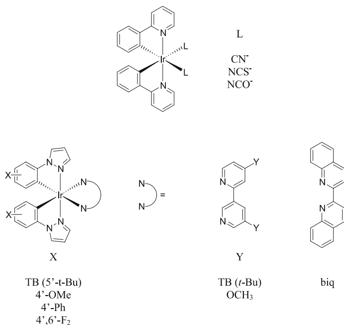
Fig. 10 Mono-anionic [57] and mono-cationic [58] complexes of Table 8
