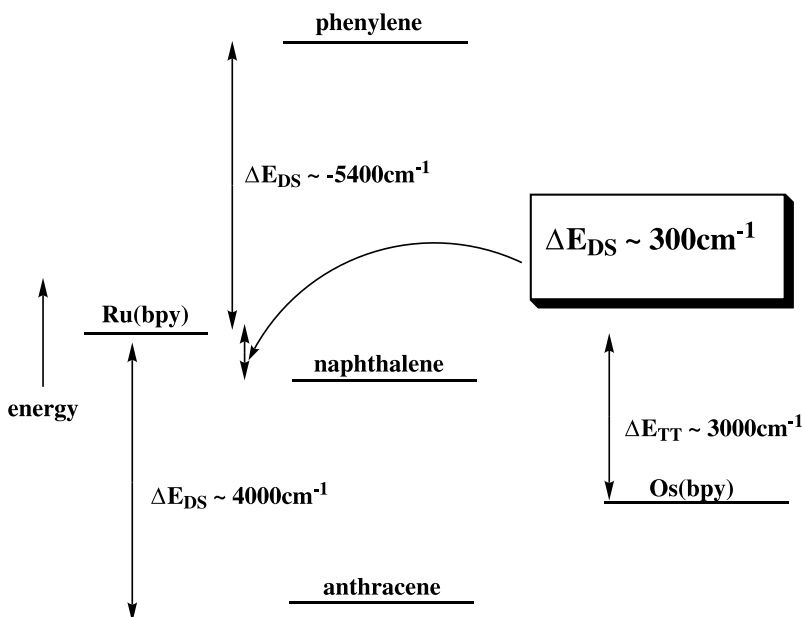
Fig. 10 State diagram for a Ru-aromatic hydrocarbon-Os complex bridge ( E_{DS} = the energy gap between the donor and the spacer in the bridging ligand) [56]
