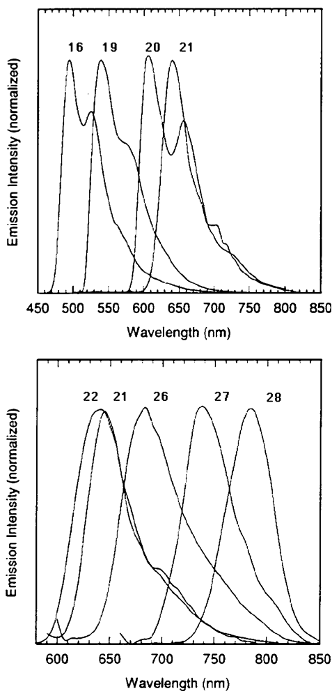
Fig. 10 Charge-transfer-to-diimine emission bands of the dbbpy series of complexes 16–21 with varying dithiolate ( top ), and the toluenedithiolate series 21–28 with varying diimine ( bottom ). The spectra were recorded in frozen butyronitrile at 77 K; their intensities have been normalized. Reprinted with permission from [43]. © (1996) American Chemical Society
