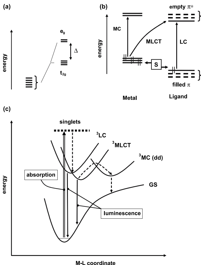
Fig. 3 a d orbitals in octahedral field; b orbital description of MC, MLCT, and LC transitions; S is a substituent group capable of exerting electron withdrawing or releasing effects (resulting in stabilization or destabilization, respectively, of the energy level of the filled d and \pi orbitals); c electronic transitions involving MC, MLCT, and LC excited states; the MC levels are not emissive
