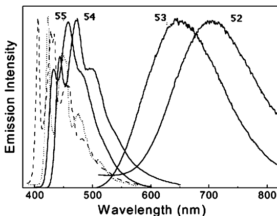
Fig. 25 Emission spectra of the N^C^N coordinated complexes 52–55 at 77 K in ethanol-methanol (4 : 1) glassy solution; the spectra of 4-phenylpyridine ( dotted line ) and 4,4'-bipyridine ( dashed line ) under the same conditions are also shown. Reprinted with permission from [142]. © (2004) American Chemical Society
