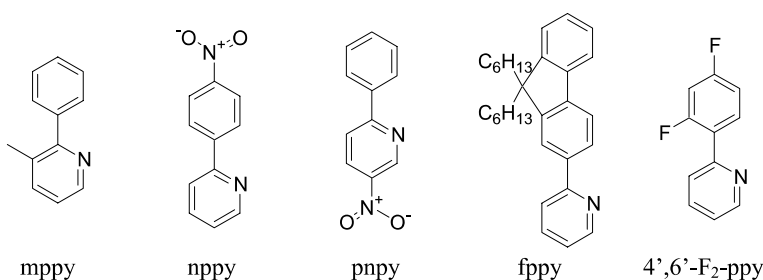
Fig. 20 Terminal ligands employed in binuclear homometallic complexes
