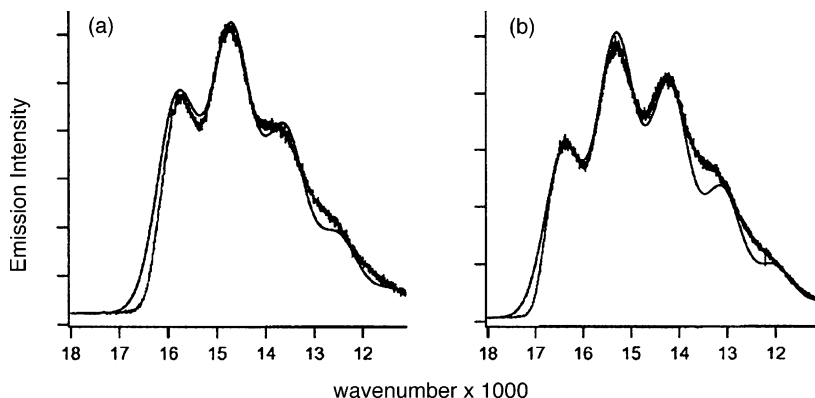
Fig. 3 Experimental ( thick noisy line ) and calculated ( fitted solid line ) emission spectra for ReNCl 2 (PCy 3 ) 2 (a) and ReNBr 2 (PCy 3 ) 2 . The fitted line is consistent with a lengthening of the ReN bond in the excited state of ca. 0.08–0.09 Å
