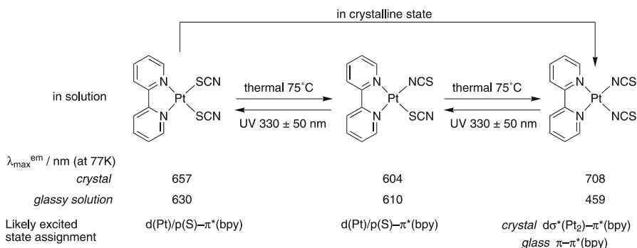
Scheme 1 Linkage isomers of bis(thiocyanate)(2,2'-bipyridine)platinum(II), their interconversion, and their emission maxima and excited states at 77 K. Based on data from [48]
