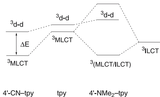
Fig. 16 Schematic of the trends in excited-state energies in [\text{Pt}(4'\text{-R-tpy})\text{Cl}]^+ complexes, showing the mixing of the ILCT state for the amino-substituted complex. \Delta E represents the barrier to deactivation via a ^3\text{d-d} state. Reproduced from data in [65] with permission from Elsevier
