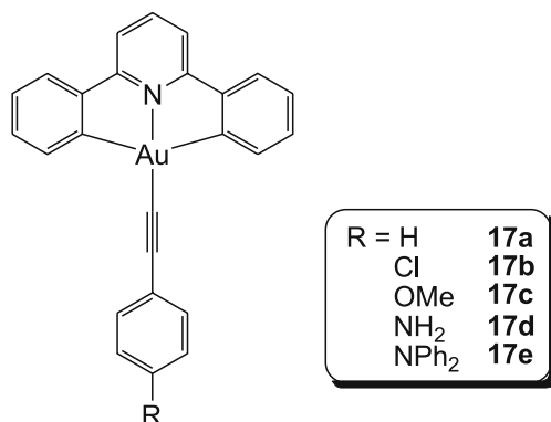
Fig. 23 Structure of the bis-cyclometallated gold(III) alkynyl complexes 17a–e
