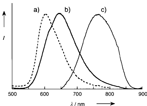
Fig. 14 Luminescence spectra of [\text{Pt}(\text{bpy})(2\text{-pyS})]_2 at room temperature: (a) the anti isomer, (b) the light-red form of the syn isomer, and (c) the dark-red (solvated) form of the syn isomer. See Fig. 13 for corresponding structures. Reprinted with permission from [54]. © (2002) Wiley-VCH
