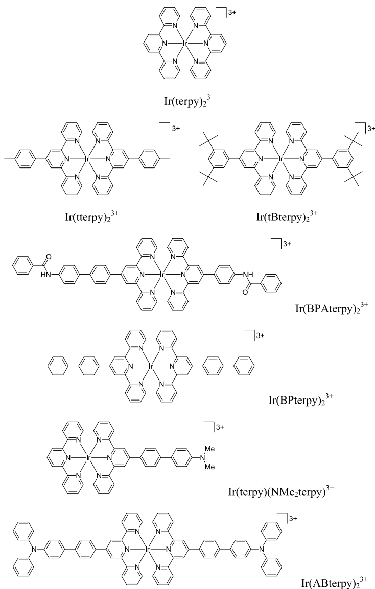
Fig. 16 Schematic structures of bis-terdentate complexes; the two terdentate planar systems are roughly perpendicular each other
