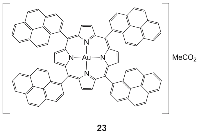
Fig. 29 Structure of the pyrene-functionalized gold(III) porphyrin complex 23
