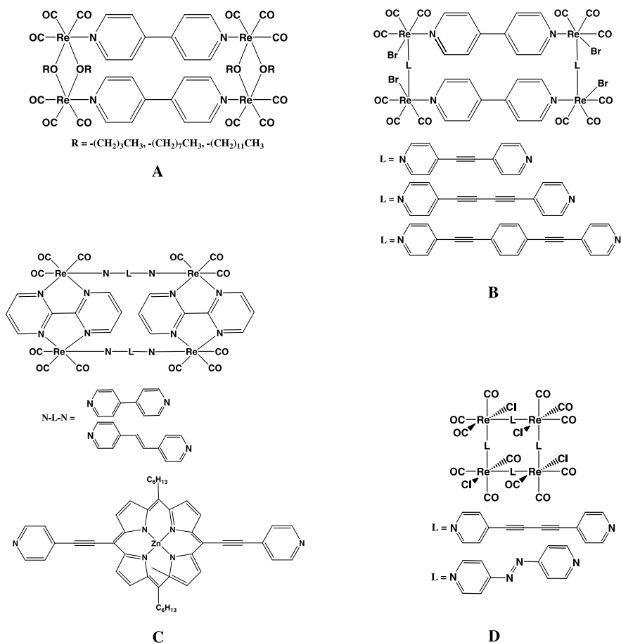
Fig. 18 Squares, Rectangles, Triangles
