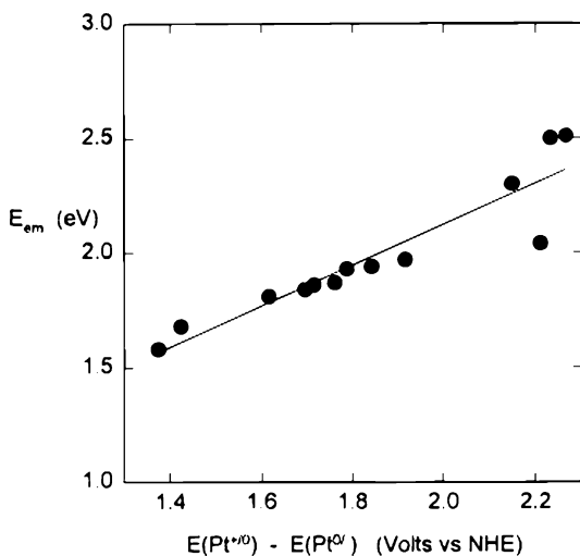
Fig. 12 Plot of emission energy (from 77 K butyronitrile spectra) against the difference between the ground state oxidation and reduction potentials for 16–29, and the linear least-squares fit. Reprinted with permission from [43]. © (1996) American Chemical Society
