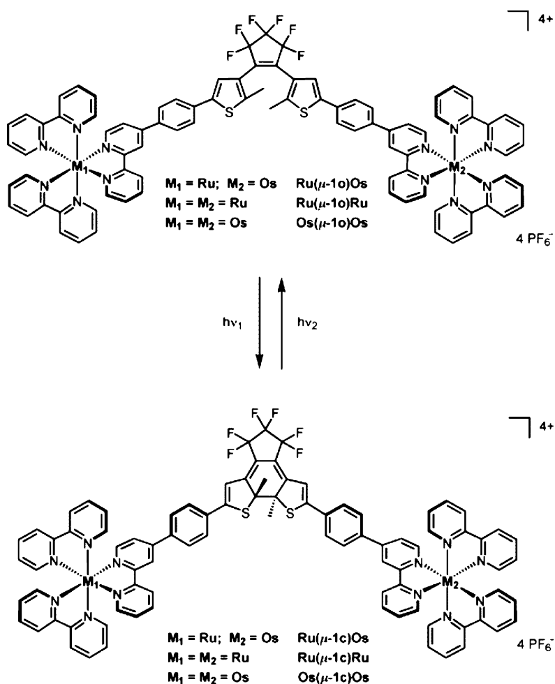
Fig. 11 Photocyclization of dithienylethene bridged bimetallic complexes [76, 77]
