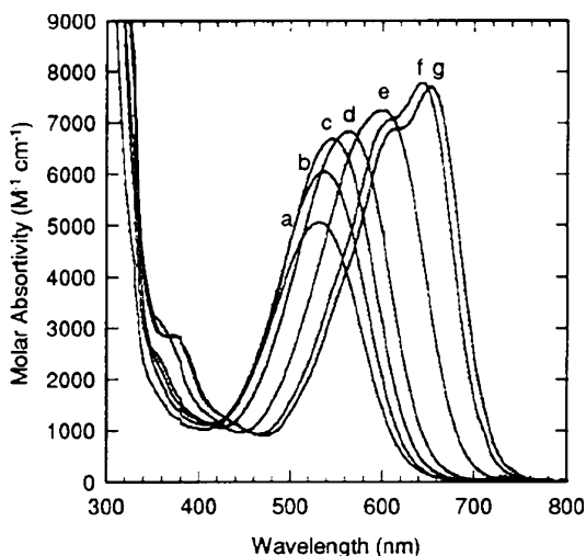
Fig. 11 Charge-transfer-to-diimine absorption band for 21 in (a) \text{CH}_3\text{CN} , (b) \text{DMSO} , (c) \text{DMF} , (d) \text{THF} , (e) \text{CH}_2\text{Cl}_2 , (f) \text{C}_6\text{H}_6 , and (g) \text{C}_6\text{H}_5\text{CH}_3 . Reprinted with permission from [43]. © (1996) American Chemical Society
