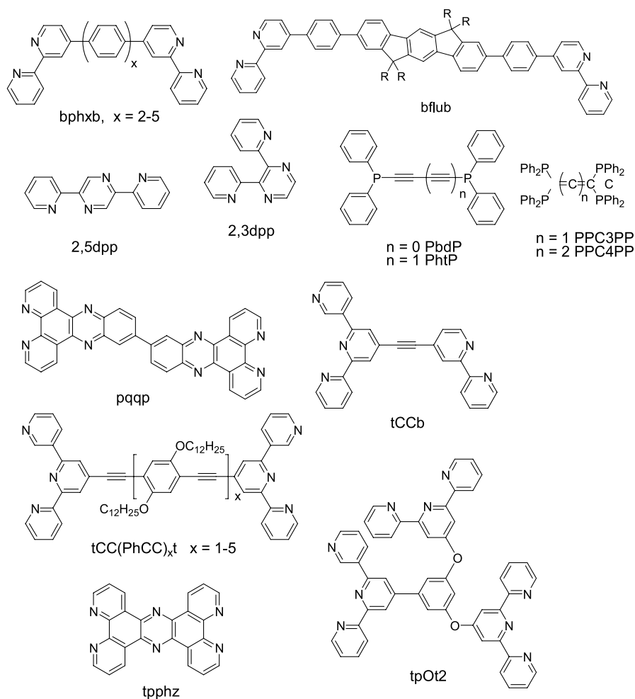
Scheme 4 Structures of bridging ligands
