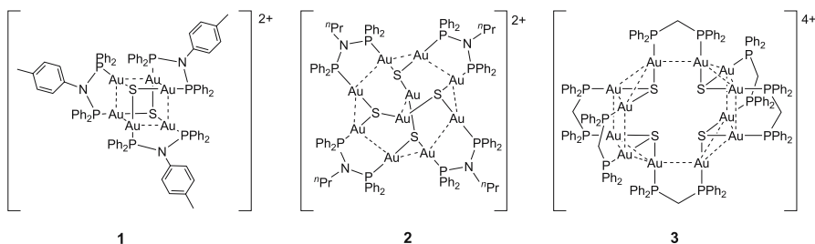
Fig. 4 Luminescent high-nuclearity gold(I) sulfido complexes 1–3
