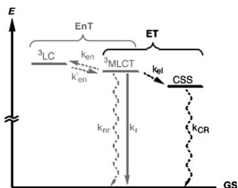
Fig. 6 State diagram for the complexes [(\text{mpt})\text{Os}(\text{tppydN})]^{2+} and [(\text{mpt})\text{Os}(\text{tpyMpydN})]^{2+} indicating the existence of a ligand centered state that provides an energy transfer path that competes with electron transfer (EnT = energy transfer; ET = electron transfer; CSS = charge separated state; CR = charge recombination) [42]
