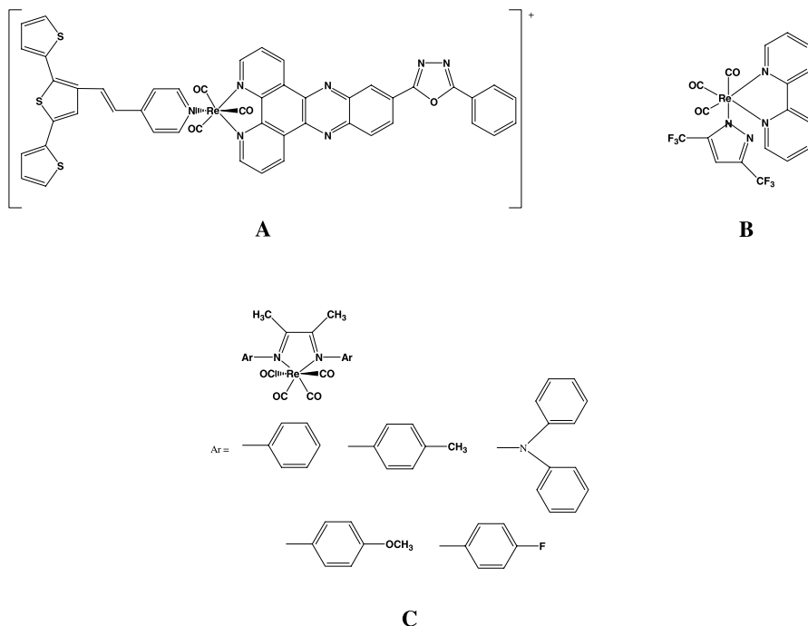
Fig. 24 OLED molecules
