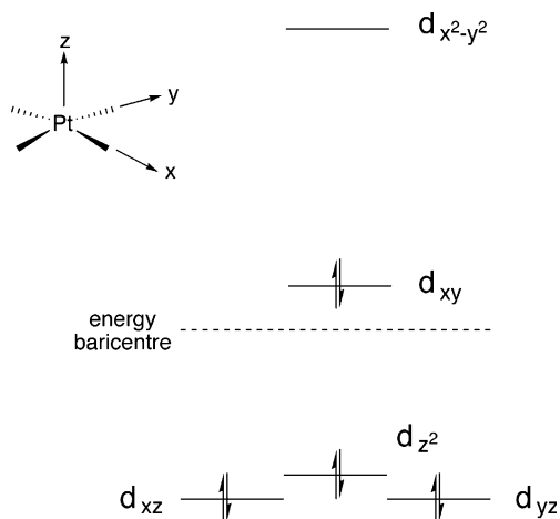
Fig. 1 Simple ligand field-splitting diagram for metal d orbitals in a square planar complex. By convention, the z axis is perpendicular to the plane of the complex and the M – L bonds lie along the x and y axes. Note that the exact ordering of the lower energy levels depends on the ligand set (e.g., relative importance of \sigma - and \pi -effects) but the d_{x^2-y^2} is always unequivocally the highest
