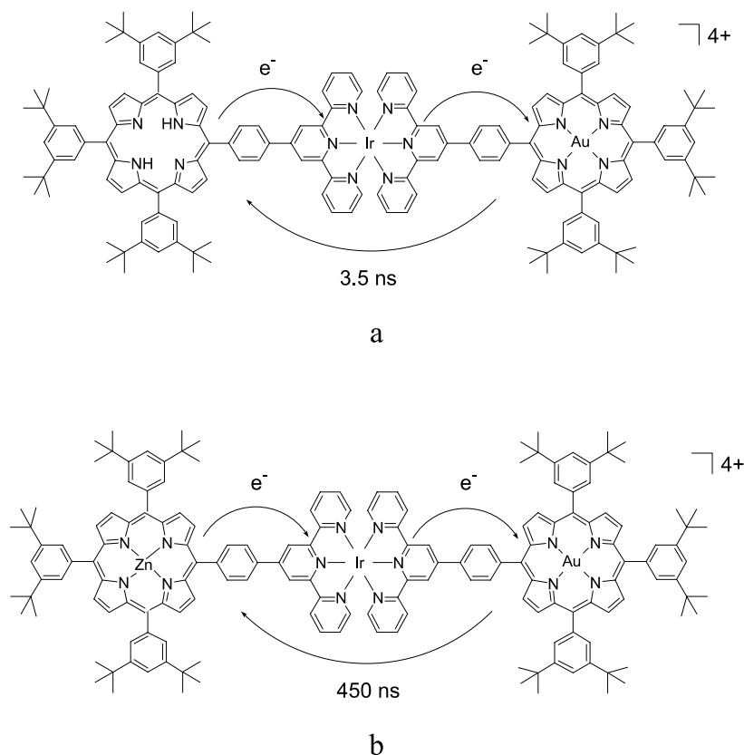
Fig. 27 Schematic structures of arrays, see text; arrows denote electron transfer
