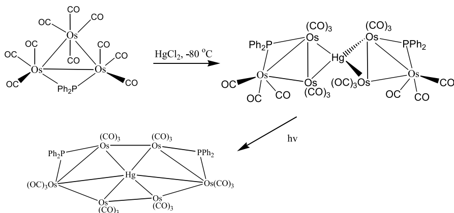
Fig. 18 Photoreaction of the photoproduct of [\text{Os}_3(\text{CO})_{10}(\mu\text{-PPh}_2)] with \text{Hg}^{2+} to yield a cyclic heptametallic complex [102]
