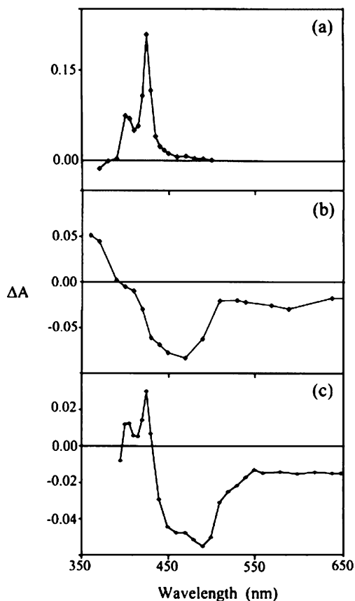
Fig. 12 Nanosecond transient absorption spectra of the AN2bpy ligand (a), [Os(bpy)_3]^{2+} (b), and [Os(AN2bpy)_3]^{2+} (c) [85]
