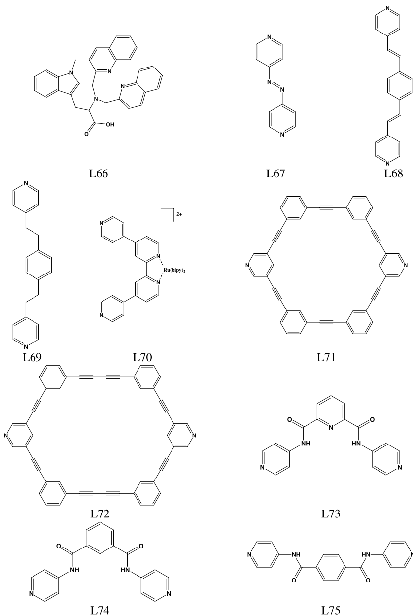
Fig. 10 Structures of ligands L66–L75
