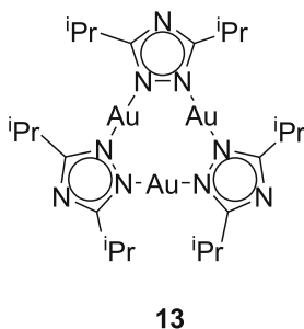
Fig. 16 Structure of the trinuclear gold(I) triazolate complex 13
