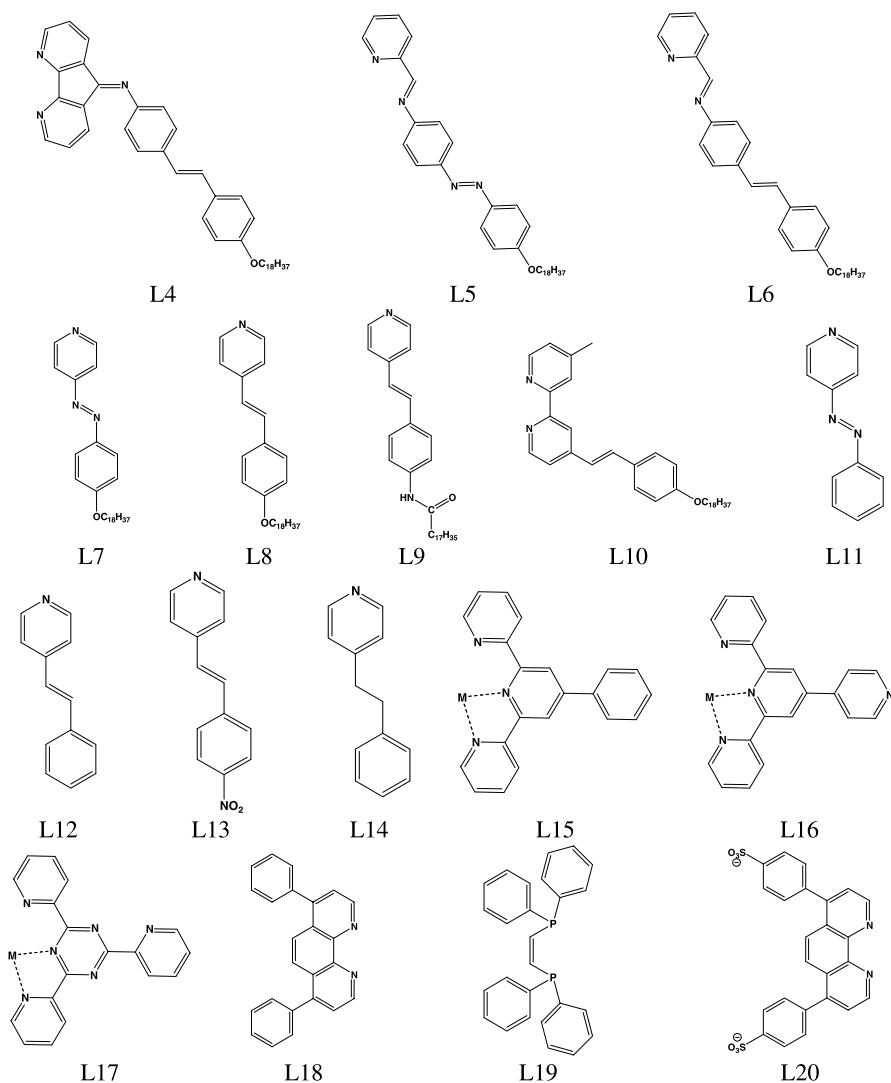
Fig. 6 Structures of ligands L4–L20
