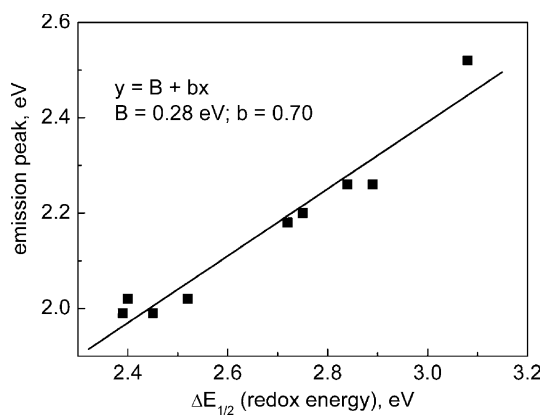
Fig. 11 Correlation between redox and emission energies, Eq. 3, for the series of cationic complexes of Table 8
