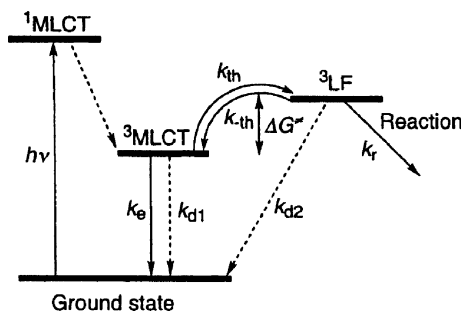
Scheme 1 Jablonski diagram for the dissociative, activated loss of the ligand trans to \text{PR}_3 in fac - [\text{Re}(\text{bpy})(\text{CO})_3(\text{PR}_3)]^+ complexes
