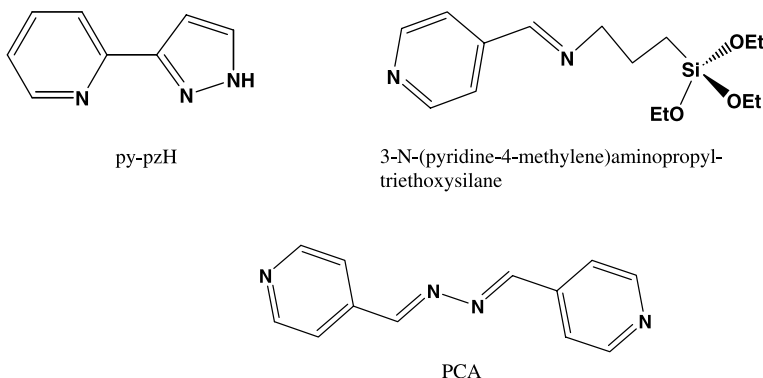
Fig. 25 Proton sensor ligands
