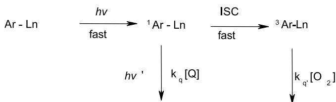
Scheme 2 Initial steps of sensitisation process – the antenna excitation
