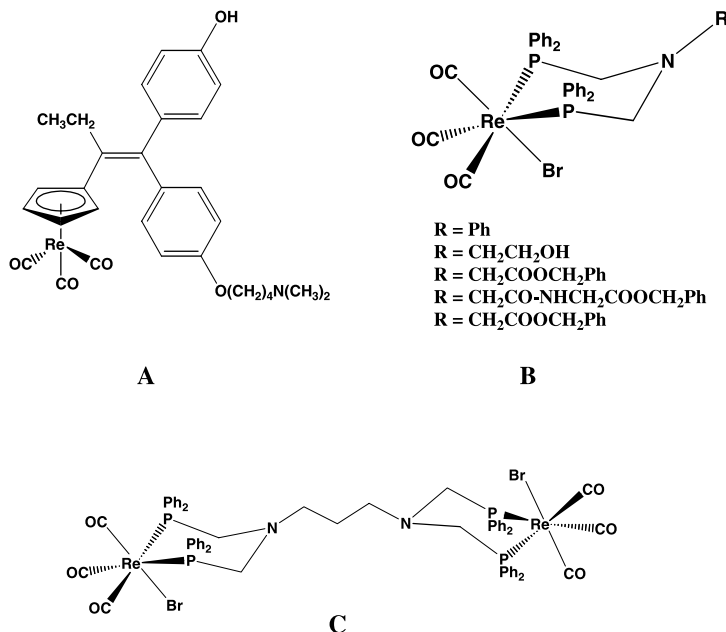
Fig. 23 Rhenium Complexes used in Cancer Studies
