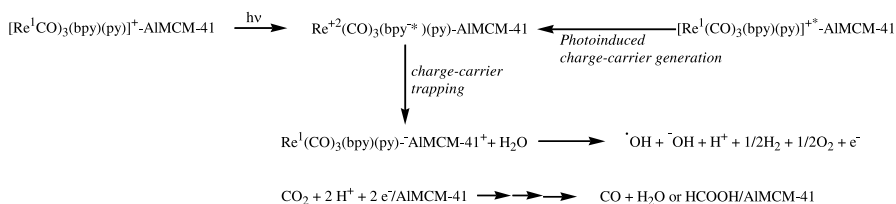
Scheme 5 Photocatalytic activation mechanism of \text{CO}_2 under visible light irradiation using [\text{Re}(\text{CO})_3(\text{bpy})(\text{py})]^+
