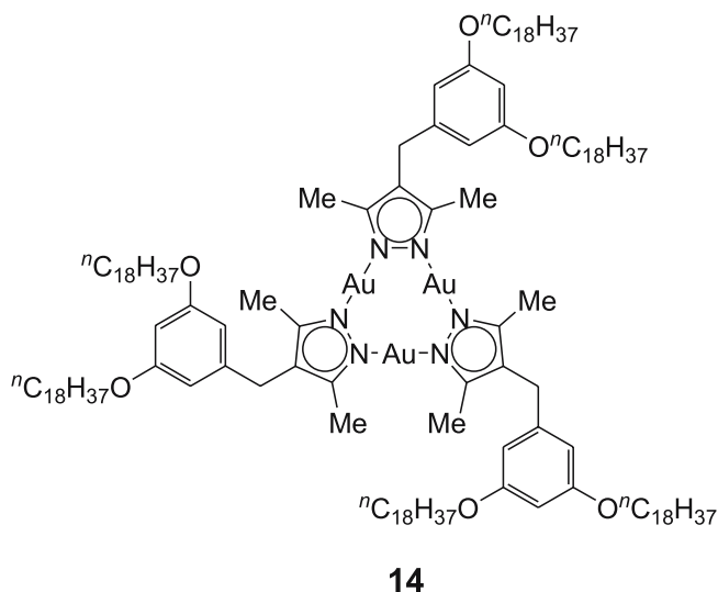
Fig. 17 Phosphorescent trinuclear gold(I) organogel
