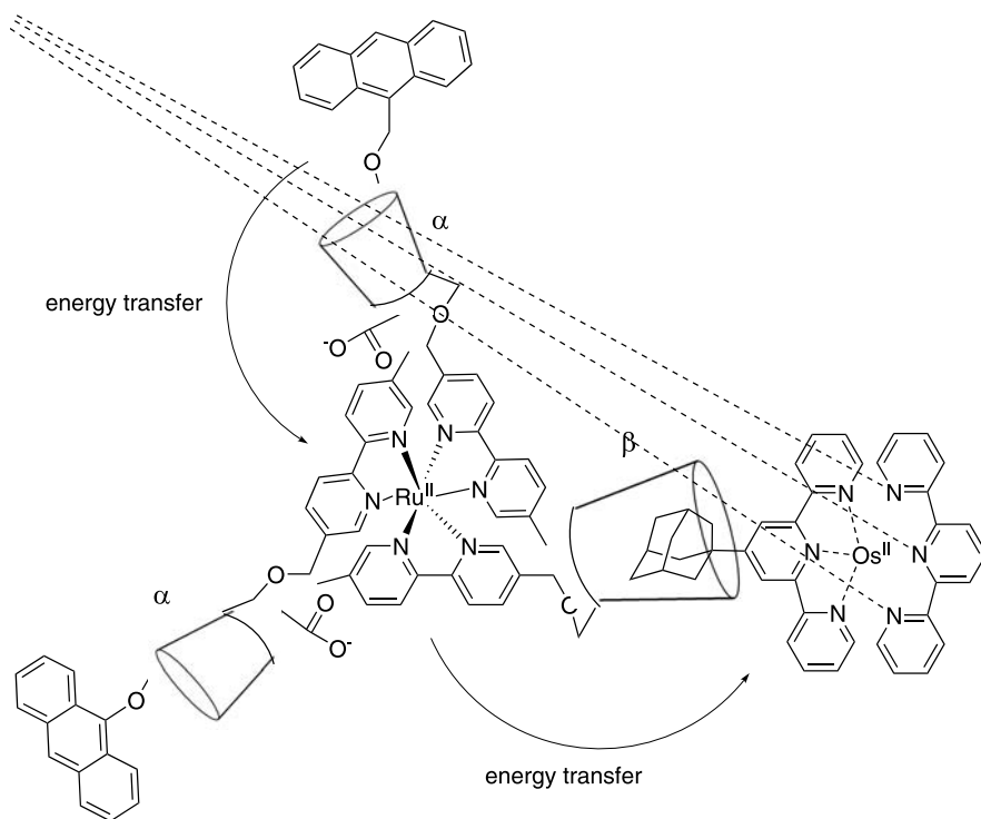
Fig. 14 Energy transfer cascade in self-assembling anthracene–Ru complex–Os complex light harvesting array linked by cyclodextrins [88]
