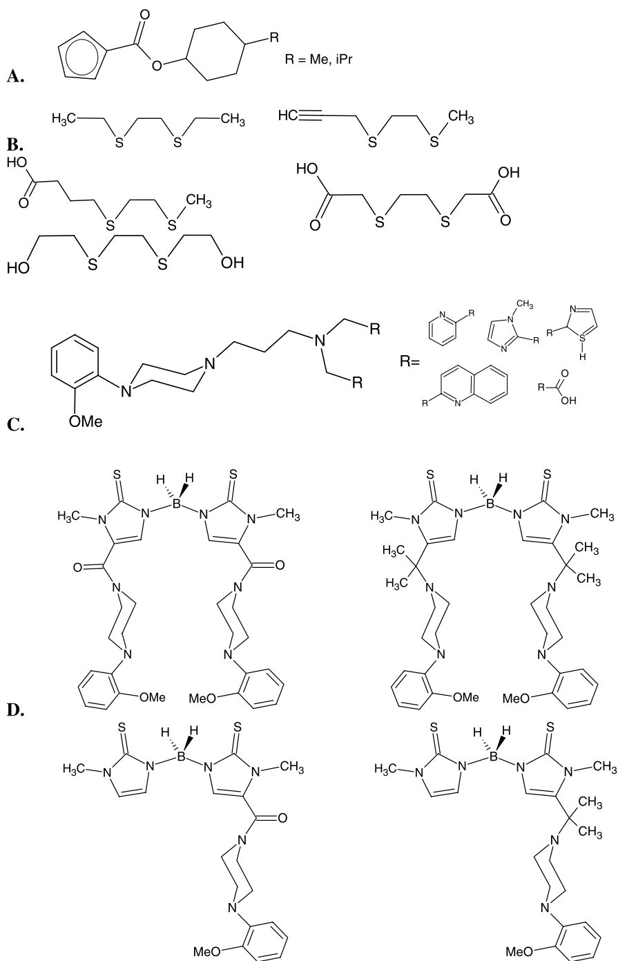
Fig. 22 Ligands bonded to the \{\text{Re}(\text{CO})_3\}^+ unit
