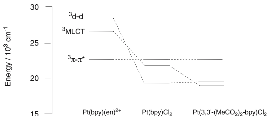
Fig. 5 Estimates of the energies of the low-lying triplet ligand-centred ( \pi-\pi^* ), charge-transfer (MLCT) and metal-centred (d-d) excited states of three platinum(II) bipyridyl complexes. Reproduced from data in [10] with permission. © (1993) American Chemical Society
