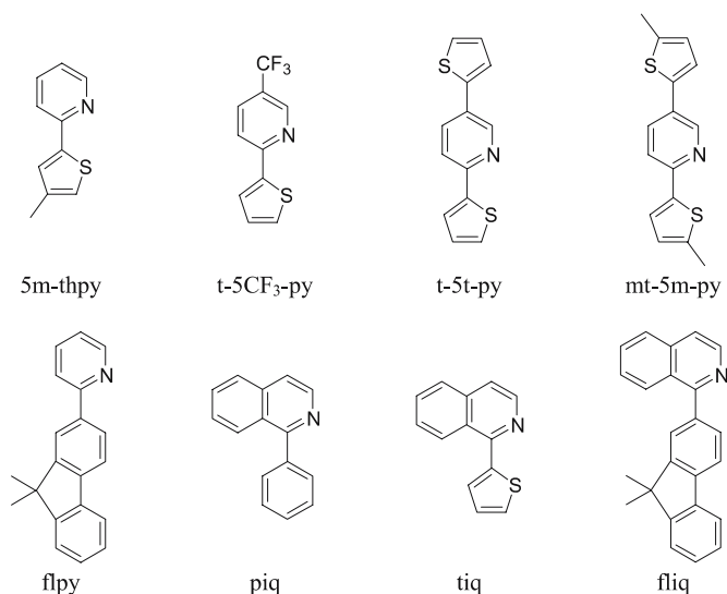
Fig. 6 (C ^ N) ligands of the neutral homoleptic Ir(C ^ N) 3 complexes of Table 4
