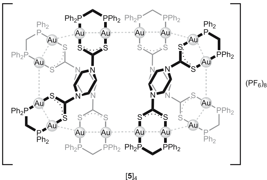
Fig. 9 Chiral Au 16 aggregate [5] 4 via self-assembly process
