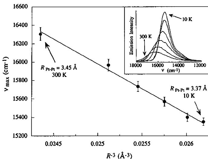
Fig. 4 Emission peak energy ( \nu_{\max} ) of the red form of \text{Pt}(\text{bpy})\text{Cl}_2 1 as a function of the inverse cube of the Pt–Pt separation R [10]. The data were obtained from variable temperature X-ray crystallography. The solid line is the linear fit to the equation: \nu_{\max} = 29.5(55) \times 10^3 - 5.4(3) \times 10^5 R^{-3} . The inset , adapted from reference [1], shows six emission spectra at different temperatures: 300, 200, 150, 100, 50 and 10 K. Reprinted with permission from [11]. © (1996) American Chemical Society
