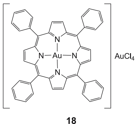
Fig. 24 Structure of the gold(III) porphyrin complex 18
