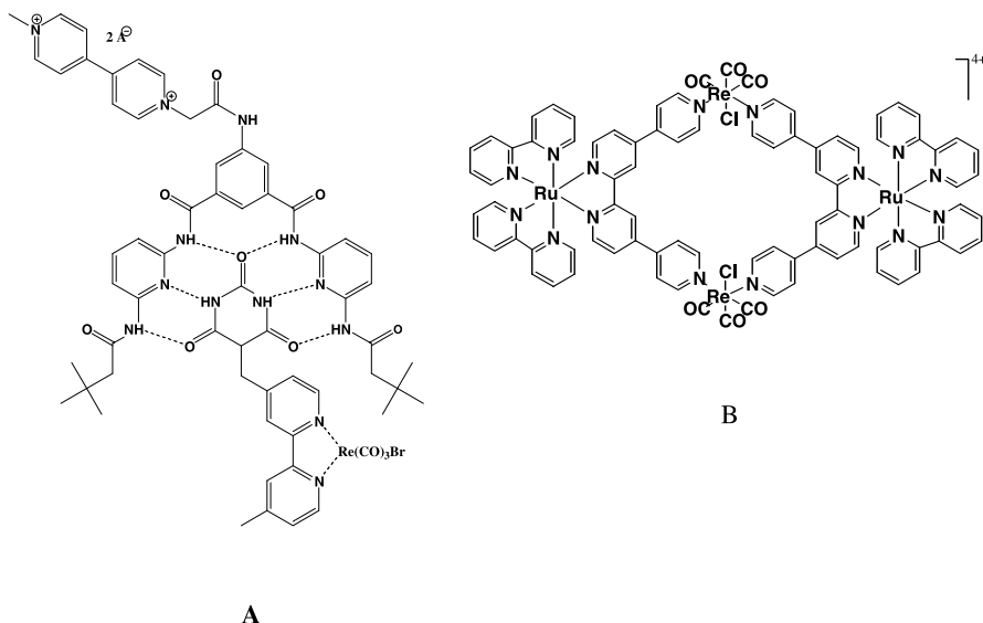
Fig. 19 Host-guest molecules
