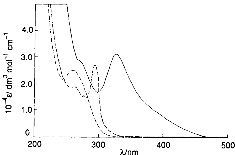
Fig. 2 Electronic absorption spectra of [\text{Au}(\text{PPh}_3)_2]\text{OTf} (— · — · — ·), [\text{Au}_2(\text{dppm})_2](\text{OTf})_2 (---) and [\text{Au}_3(\text{dmpm})_2](\text{SCN})_3 (—) in MeCN at room temperature [16]
