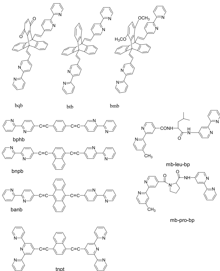
Scheme 3 Structures of bridging ligands
