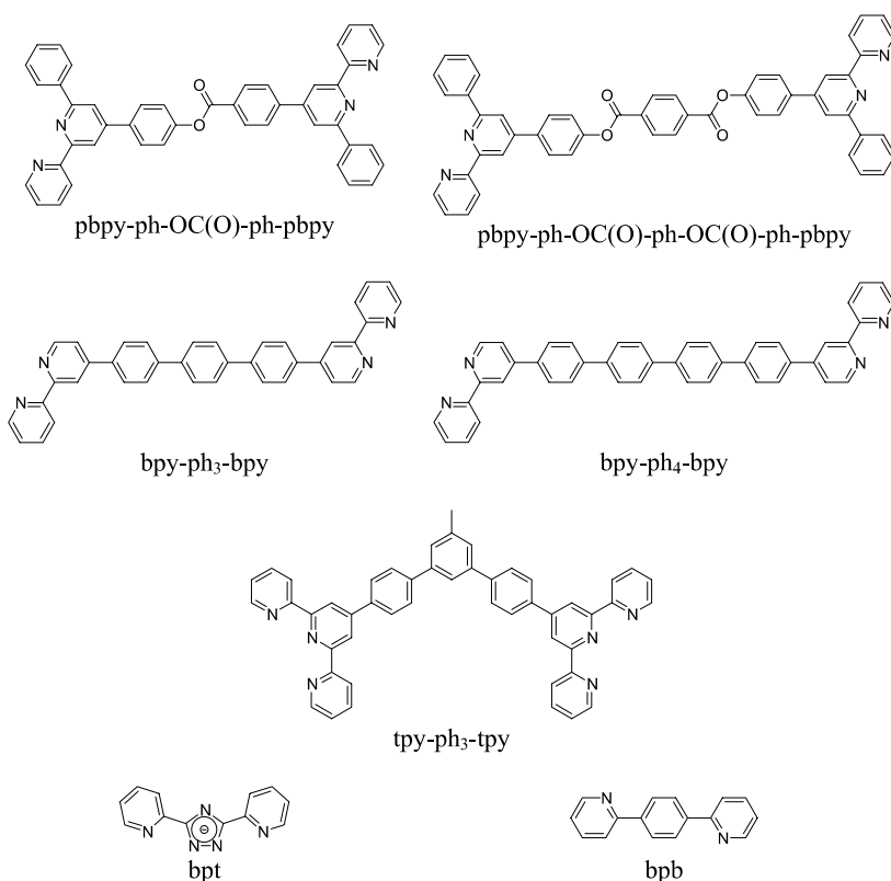
Fig. 21 Bridging ligands employed in binuclear homometallic complexes
