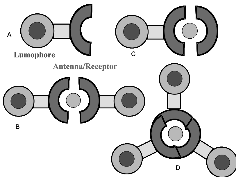
Scheme 6 The various self-assembly structures possible for simple f-d mixed coordination based compounds
