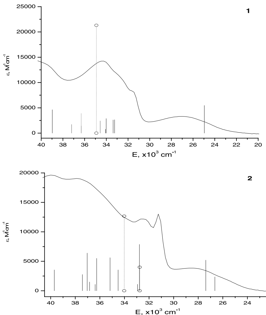
Fig. 14 Experimental absorption spectra of 1, [\text{Re}(\text{bpy})(\text{CO})_3\text{Cl}] , and 2, [\text{Re}(\text{bpy})(\text{CO})_3(\text{py})]^+ , and calculated singlet excited-states. The excited states are shown as vertical bars with height equal to the extinction coefficient. Black = MLLCT, green = LLCT, blue = \pi \rightarrow \pi^* , red = MCDCT, orange = \text{Re}_d , \text{CNx} \rightarrow \text{Re}_s mixed excited-state (with permission from ACS)
