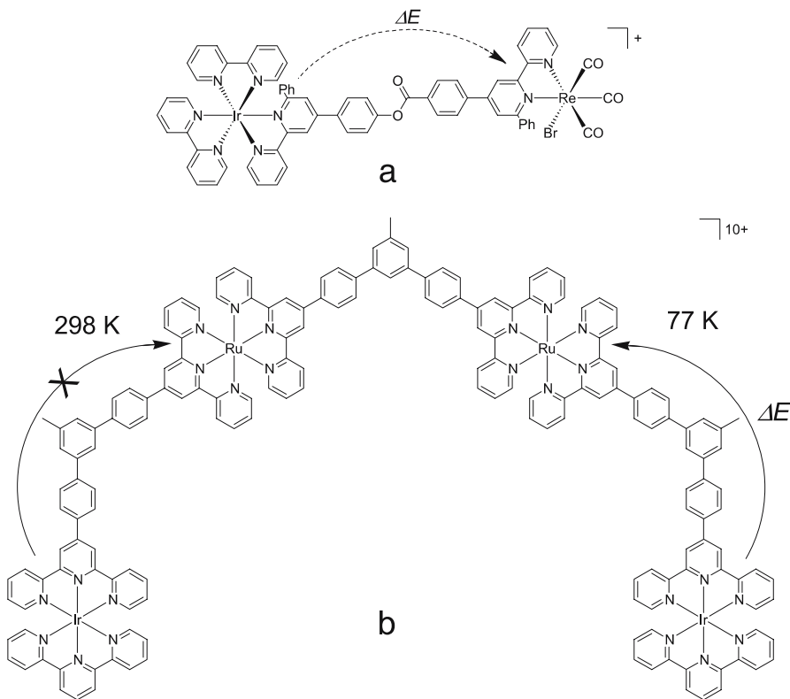
Fig. 23 Schematic structures of polynuclear complexes, see text; arrows denote energy transfer
