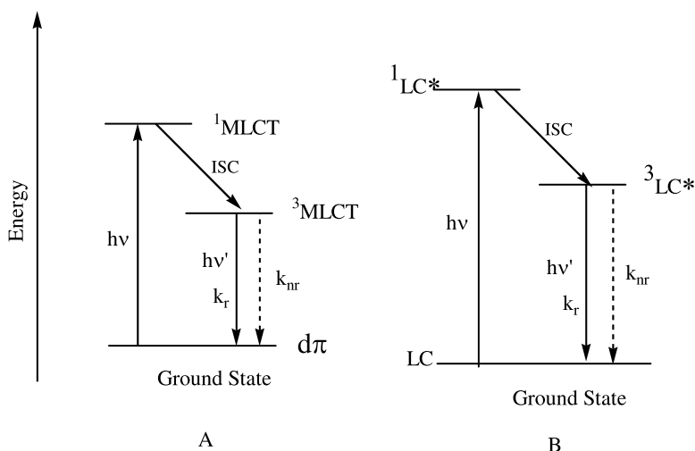
Fig. 13 Jablonski Diagrams for [\text{Re}(\text{diimine})(\text{CO})_3\text{L}] Complexes: A MLCT Model; B Ligand-Centered Model
