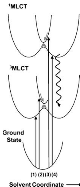
Fig. 1 Potential energy surfaces of the 1 MLCT and 3 MLCT states of [Os(bpy) 3 ] 2+ for a model in which the excitation can be localized on a single bipyridine [16]
