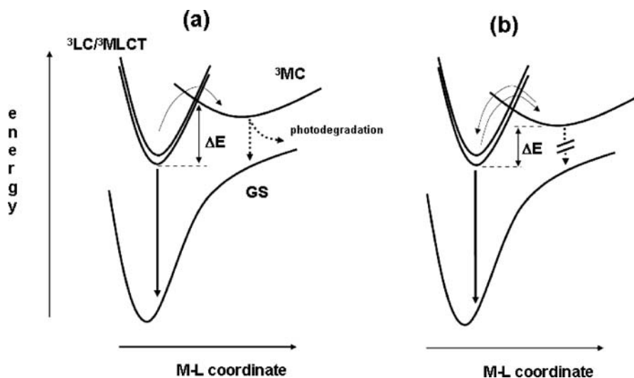
Fig. 19 Expected limiting kinetic cases for deactivation of the luminescent ^3\text{LC}/^3\text{MLCT} levels in Ir(III)-complexes, see text. Adapted from refs [3, 98]
