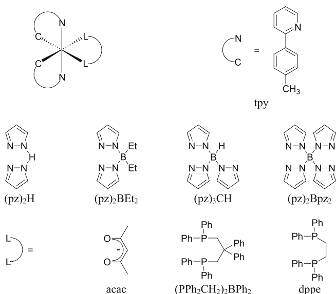
Fig. 7 Ligands of complexes of Table 6
