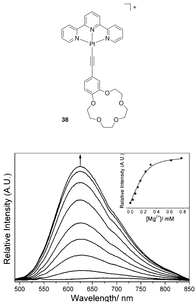
Fig. 18 Growth of emission of 38 in MeCN ( 2.5 \times 10^{-4} M) upon addition of increasing amounts of \text{Mg}(\text{ClO}_4)_2 . Inset shows relative intensity at 625 nm vs. [\text{Mg}^{2+}] (squares) and the 1 : 1 fit (line). Reprinted from [93] by permission of the Royal Society of Chemistry
