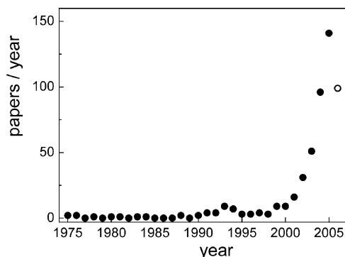
Fig. 2 Representative number of papers ( full points ) dealing with the luminescence of iridium(III) complexes in the indicated years; updating is set at August 2006 ( empty point )
