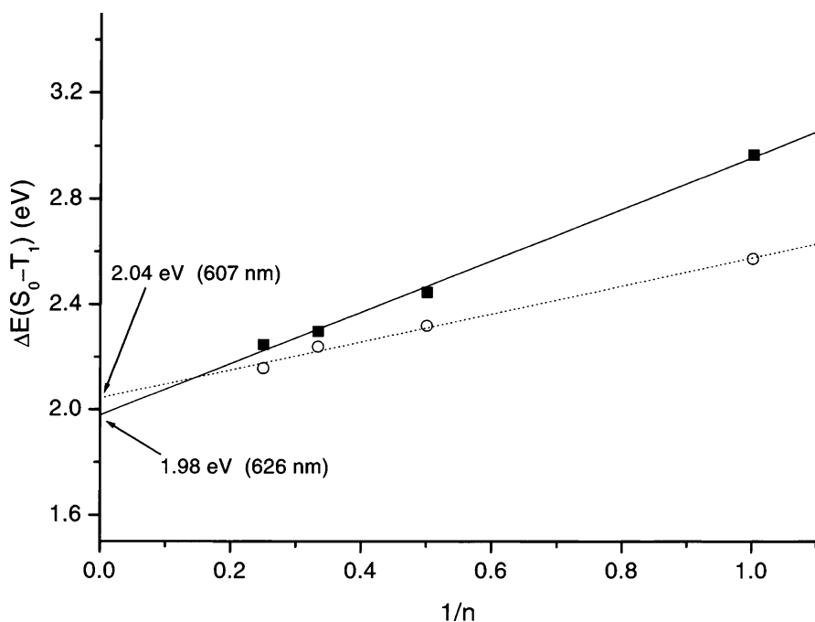
Fig. 11 Plot of \Delta E(\text{S}_0-\text{T}_1) against 1/n in mononuclear [(\text{Cy}_3\text{P})\text{Au}\{(\text{C}\equiv\text{C}-\text{C}_6\text{H}_4)_{n-1}\text{C}\equiv\text{CPh}\}] (■) and binuclear [(\text{Cy}_3\text{P})\text{Au}\{(\text{C}\equiv\text{C}-\text{C}_6\text{H}_4)_n\text{C}\equiv\text{C}\}\text{Au}(\text{PCy}_3)] (○) complexes [92]
