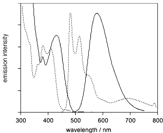
Fig. 24 Emission and excitation spectra of 49 , where R = -\text{C}_6\text{H}_4\text{-NMe}_2 (solid lines), in \text{CH}_2\text{Cl}_2 at RT ( 6 \times 10^{-5} M), and of the same solution after addition of trifluoroacetic acid (dotted lines)
