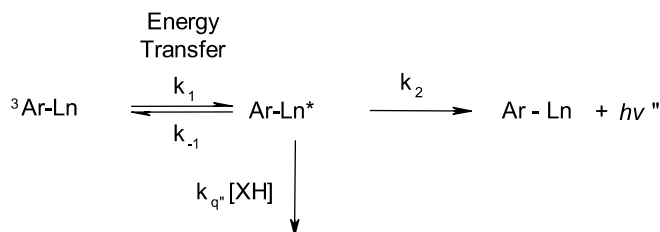
Scheme 3 Final steps of sensitisation process – lanthanide luminescence
