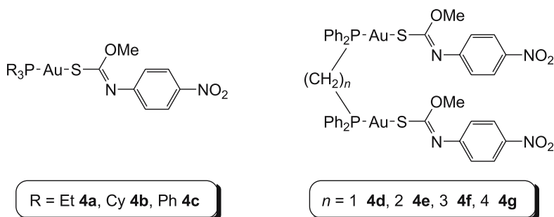
Fig. 8 Gold(I) complexes 4a–g with thiolate ligand bearing donor-acceptor functionalities
