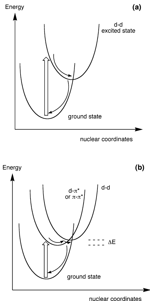
Fig. 2 a Illustrating the displacement of the potential energy surface for the d-d excited state in a square planar d^8 complex, formed by population of the d_{x^2-y^2} orbital, compared to the ground state. b Even though other excited states (e.g., d-\pi^* or \pi-\pi^* ) may lie at lower energies, the d-d excited state can provide a thermally activated non-radiative decay pathway. Thick arrows represent absorption of light; thin ones indicate vibrational relaxation and non-radiative decay
