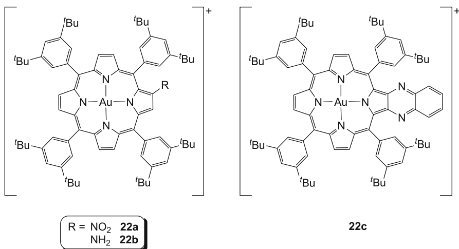
Fig. 28 Structure of 22a–c
