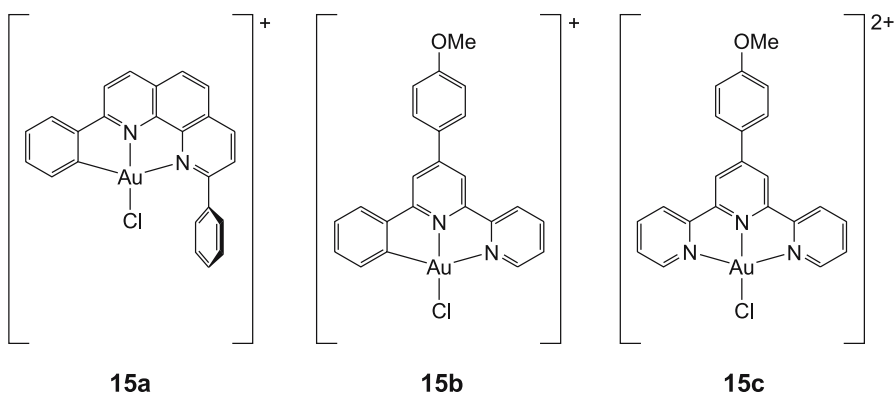
Fig. 21 Structure of the cyclometallated chlorogold(III) complexes 15a–b , and the related terpyridyl counterpart 15c
