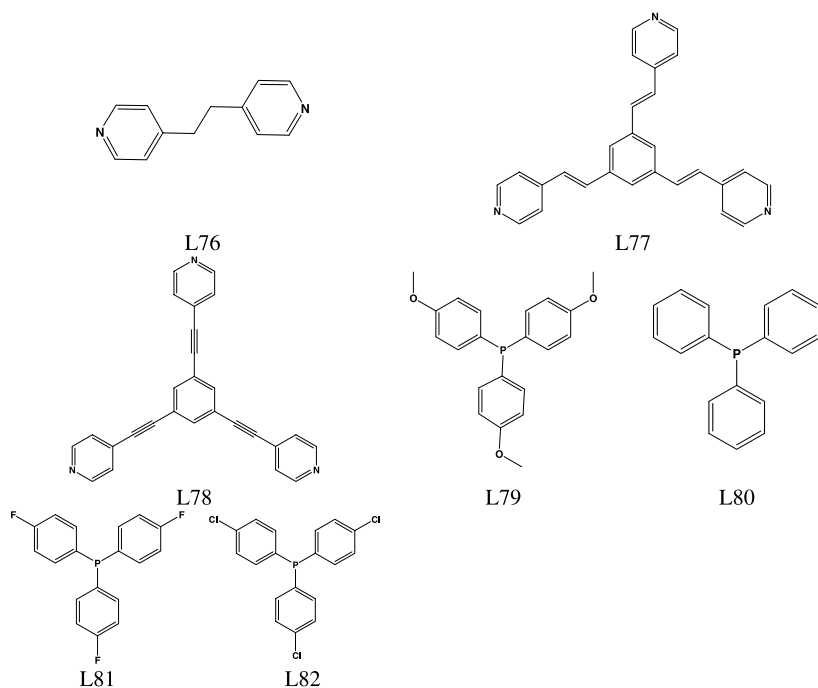
Fig. 11 Structures of ligands L76–L82
