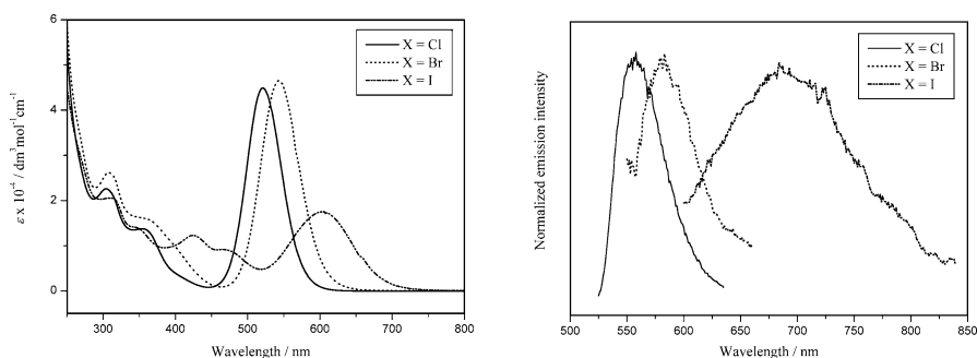
Fig. 20 Electronic absorption spectra in dichloromethane at 298 K ( left ) and normalized emission spectra in solvent glass at 77 K ( right ) for [\{\text{Au}(\text{dppn})\text{X}\}_2](\text{PF}_6)_2 (X = Cl, Br, I) [132]
