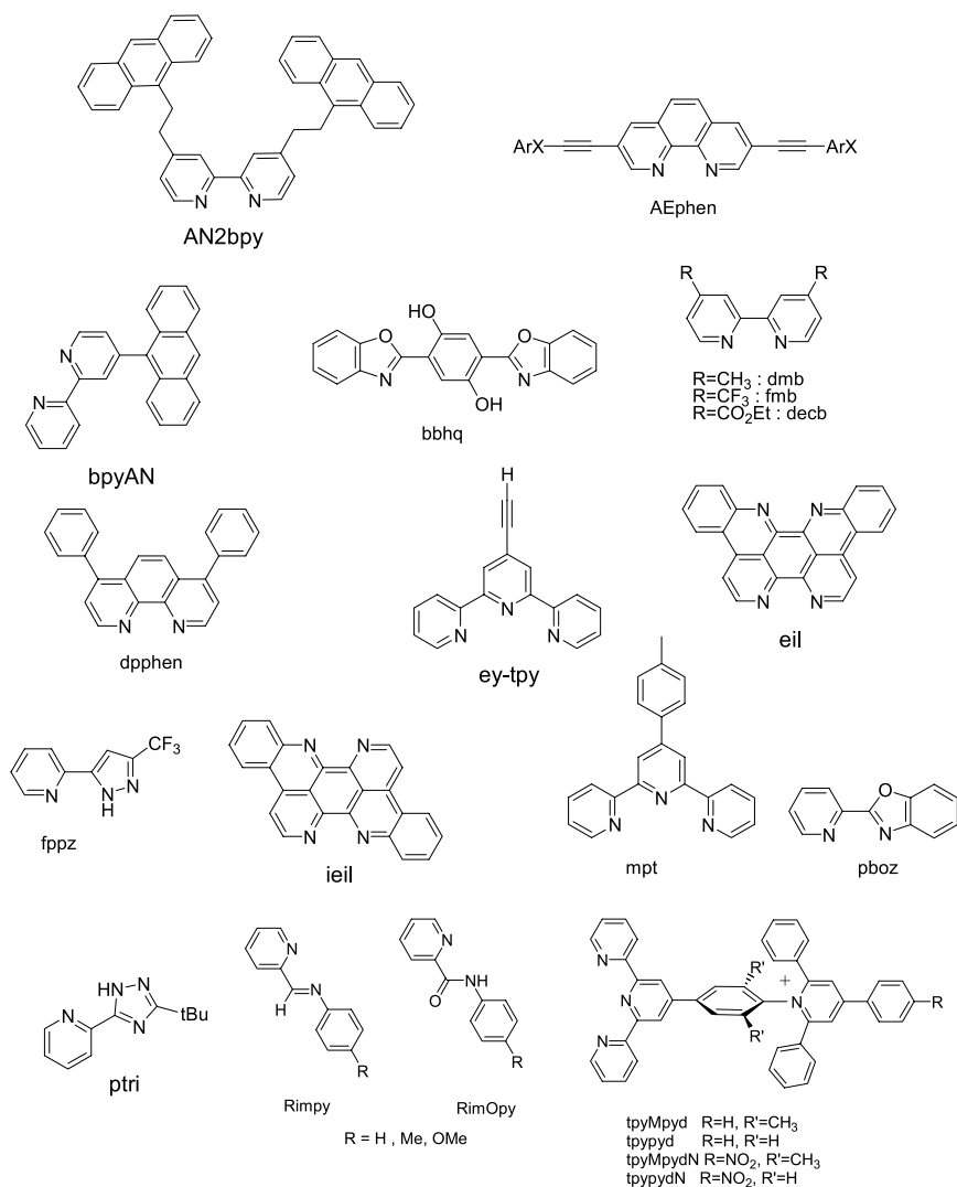
Scheme 1 Structures of simple ligands used
