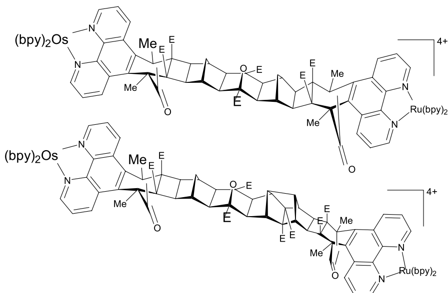
Fig. 8 Rigidly bridged Ru diimine donor/Os diimine acceptor [47]
