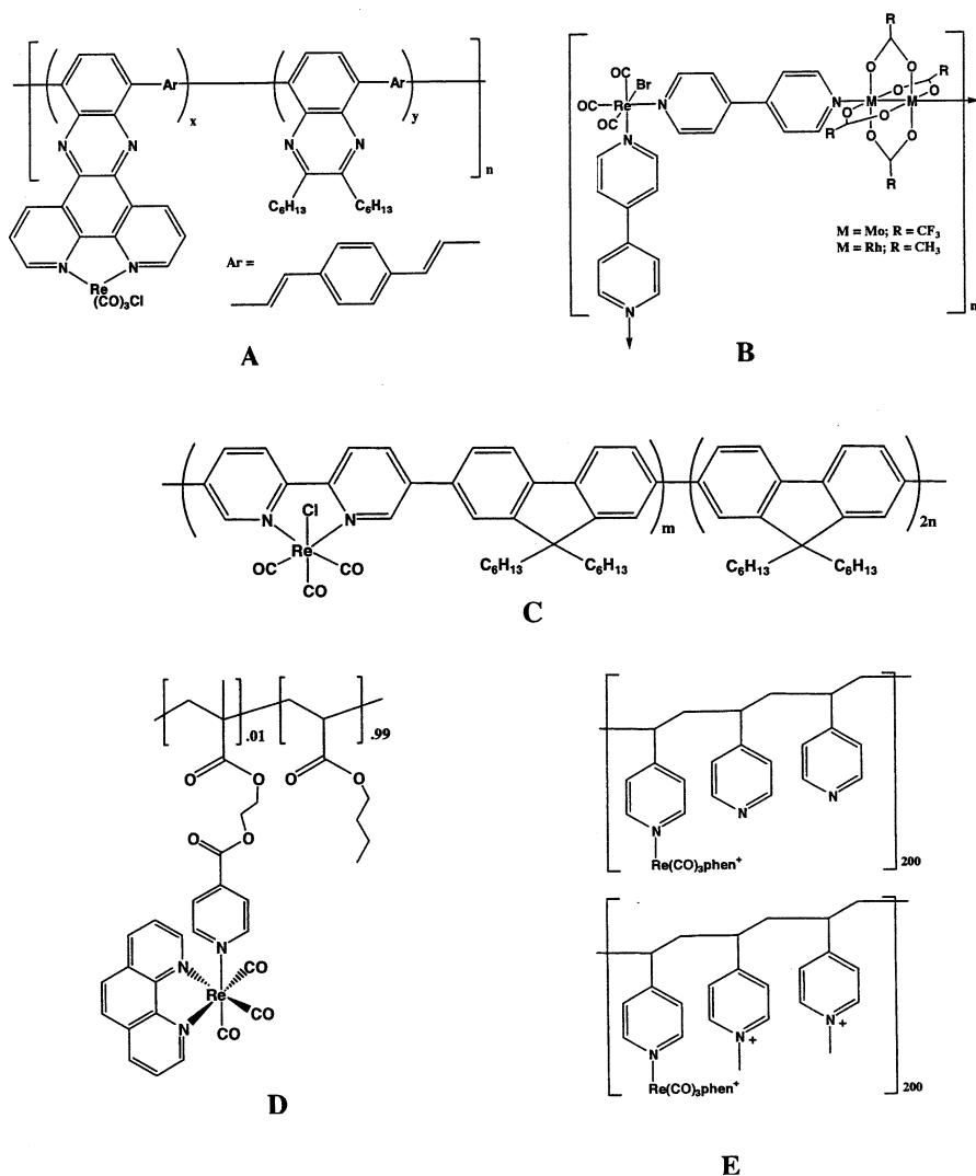
Fig. 17 Polymers incorporating rhenium into their structures
