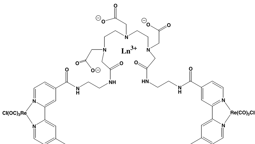
Fig. 27 Lanthanide sensor
