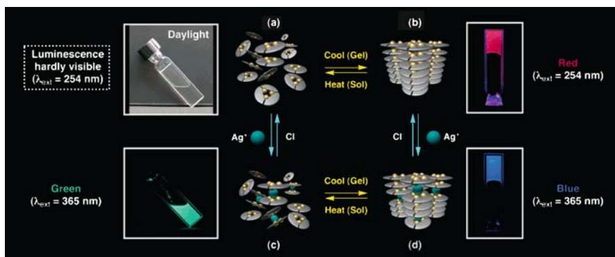
Fig. 18 Luminescence profiles of 14 in hexane. Pictures and schematic self-assembling structures of (a) sol, (b) gel, (c) sol containing \text{AgOTf} (0.01 equiv.), and (d) gel containing \text{AgOTf} (0.01 equiv.) [123]
