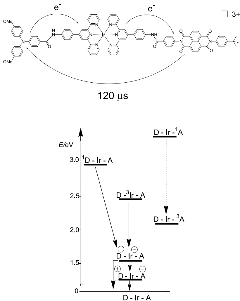
Fig. 28 Upper panel: schematic structure of a D-Ir-A triad (see text), arrows denote electron transfer steps. Lower panel: energy level diagram and elementary reactions (see text)
