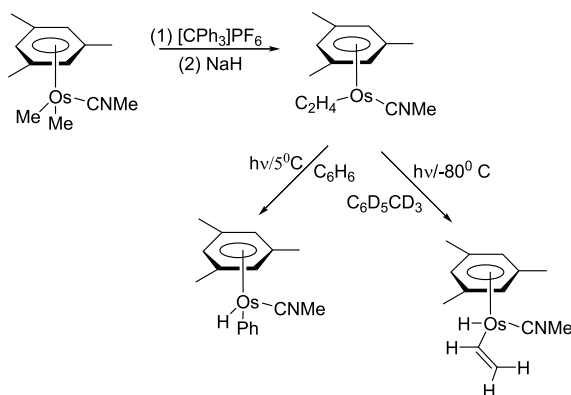
Fig. 19 C – H insertion into [(\text{mes})\text{Os}(\text{C}_2\text{H}_4)(\text{CH}_3\text{CN})] following photolysis in benzene solution [103]
