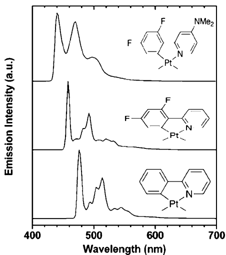
Fig. 19 From bottom to top: Emission spectra of Pt(ppy)(dpm), Pt(46dfppy)(dpm), and Pt(46dfp-4dmapy)(dpm), in MeTHF at 77 K. In the partial structures shown, the O ^ O-chelated dpm ligand has been omitted. Reprinted with permission from [109]. © (2002) American Chemical Society
