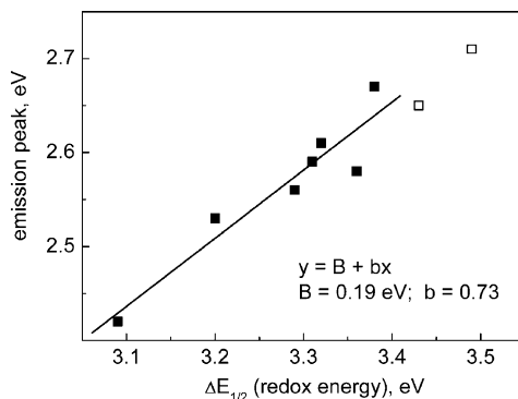
Fig. 8 Correlation between redox and emission energies, Eq. 3, for the series of Table 6. Empty points are for the 3 LC emitters (tpy) 2 Ir(PPh 2 CH 2 ) 2 BPh 2 and (tpy) 2 Ir(dppe) (CF 3 SO 3 ) [36]
