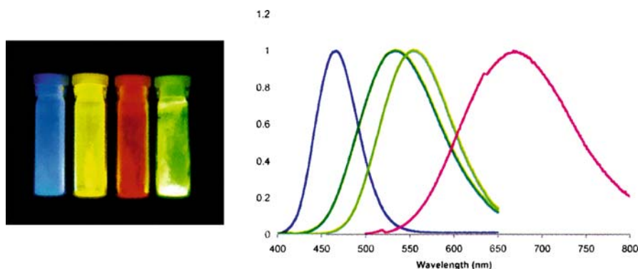
Fig. 6 Photo of the solid-state emission from [E\{Au_3(dppy)\}_3Ag](BF_4)_2 ( E = O, S, Se ) and [S\{Au_3(Me-dppy)\}_3Ag](BF_4)_2 from left to right ( \lambda_{ex} = 365 nm) (left), and the normalized emission spectra of [E\{Au_3(dppy)\}_3Ag](BF_4)_2 ( E = O (blue), S (green), Se (red)) and [S\{Au_3(Me-dppy)\}_3Ag](BF_4)_2 (dark green) in the solid state at room temperature (right) [38]
