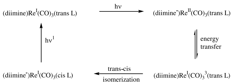
Scheme 3 Photoinduced cis-trans isomerization of complexes with C = N linkages
