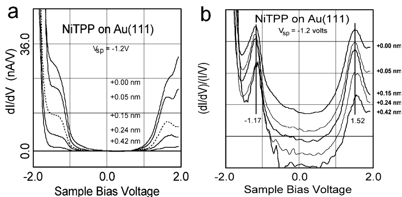
Fig. 8 OMTS dI/dV -V (a) and d\ln I/d\ln V (b) curves acquired from a NiTPP monolayer at -1.2 V sample bias and varying tip–sample distance. A different constant was added to each data set in (b) to allow them to be better distinguished. The distances given are relative to the closest tip–sample separation (-1.2 V, 2.0 nA)
