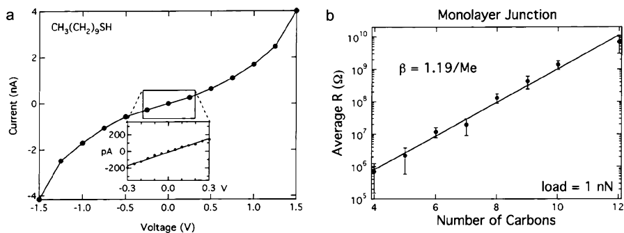
Fig. 2 a A typical I - V trace for a decanethiol SAM. The inset shows the nearly linear behaviour at low voltages. b Semilog plot of the alkanethiol junction resistance as a function of chain length. Reprinted with permission from [27]. © 2001 American Chemical Society
