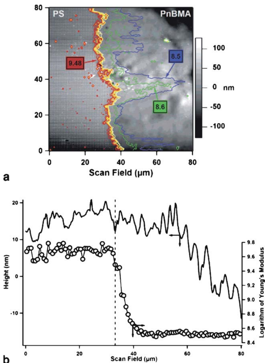
Fig. 22 a Topographic image (gray scale) of the model blend at the interface at 57.4 °C and superimposed profiles of \log(E) = 9.48 (dark red line), down to \log(E) = 9 (light yellow line), in steps of 0.08 (lines of increasing brightness, very close to each other and bunched together at the interface). Also the profiles of \log(E) = 8.6 (green line) and of \log(E) = 8.5 (blue line) are shown. b Line profile of the topography (referred to left axis) and of \log(E) (referred to the right axis) of the model blend across the interface. It can be seen that there is no discontinuity in the topography at the interface and also that the topography does not influence the determined Young's modulus. (Reprinted with permission from [121]. © (2006) American Chemical Society)
