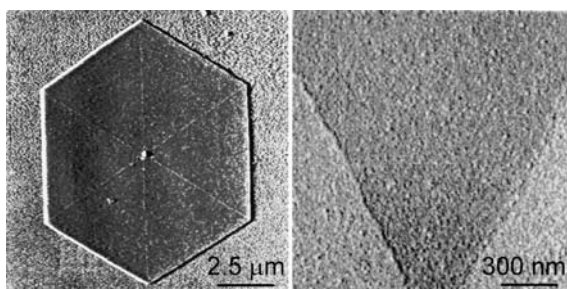
Fig. 35 Lamellar crystals of poly(oxyethylene) with clearly resolved chain fold domains at the surface of the lamellae defined by the diagonals and the edges of the crystals. The frictional force within the domains, obtained in AFM experiments, was found to depend on the relative scan direction. (Reprinted from [180] with permission from Elsevier. © (1994) Elsevier)
