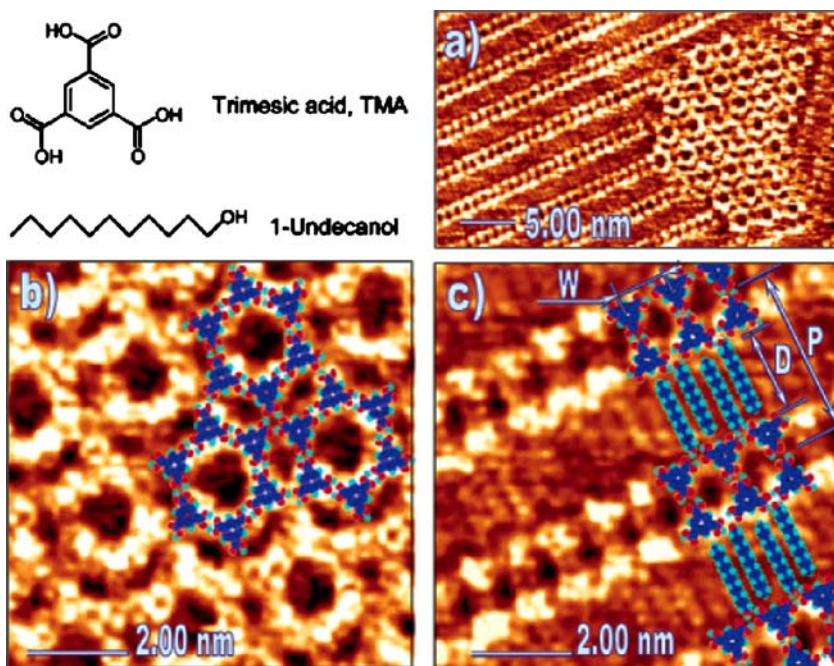
Fig. 12 a STM images of SAMNs formed by deposition of 1-undecanol and TMA from a heptanoic acid solution on HOPG. b TMA flower pattern with molecular model. c TMA linear pattern with molecular model. V_s = -0.8 V, I_t = 150 pA. Reprinted with permission from [62]. © (2006) American Chemical Society
