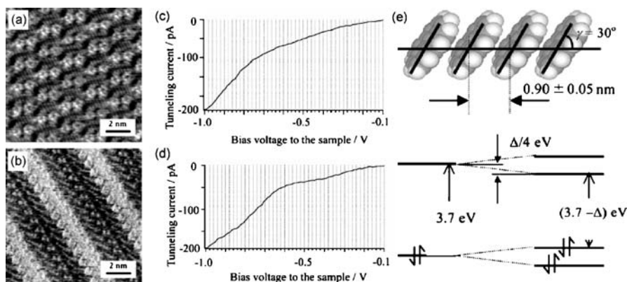
Fig. 28 STM images of 1-pyrenehexadecanoic acid (a) ( 11 \times 11 nm 2 ) and 1-pyrenehexadecanoic acid-4,4-dipyridyl (b) ( 11 \times 11 nm 2 ) monolayers at the 1-phenyloctane/graphite interface. Imaging condition was I = 0.15 nA, V = 0.80 V and I = 0.13 nA, V = 1.00 V, respectively. c,d I–V curves taken above the isolated pyrene unit within the one-component monolayers and the \pi -stacked pyrene units within the two-component monolayers, respectively. e Schematic structural model of the \pi -stacking of pyrene units and energy diagrams of the HOMO and LUMO levels for isolated and \pi -stacked pyrene units
