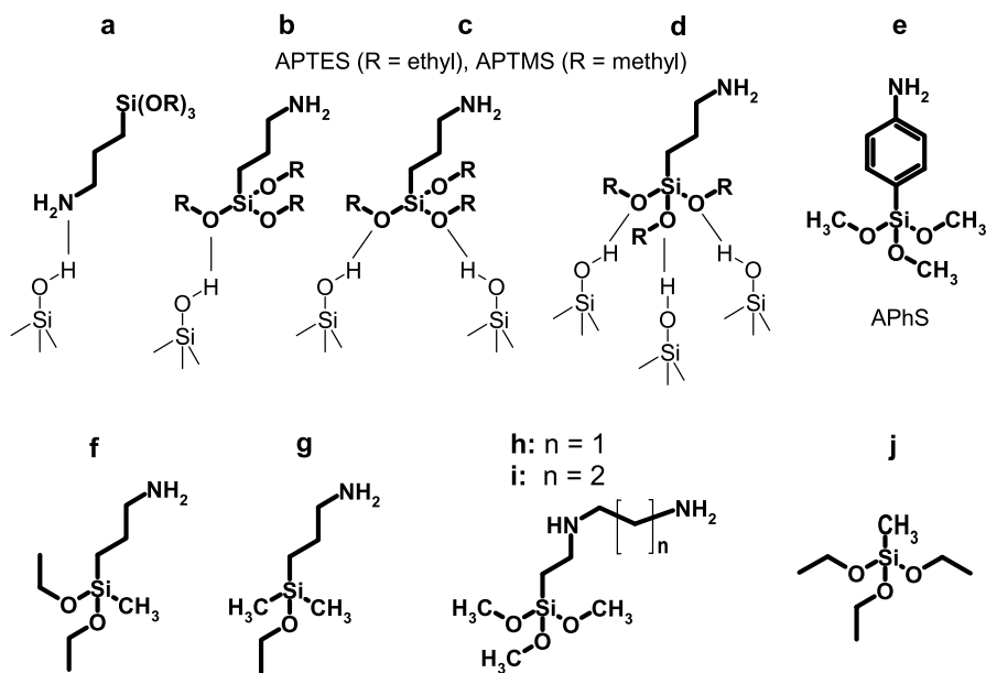
Fig. 6 Aminosilanes (a–i) and methyltriethoxysilane (j, for adjustment of low amino group surface densities in gas phase silanization [50, 133]). Hydrogen-bonding of APTES and APTMS to silicon dioxide surfaces, initially via their amino function (a), and after “flipping” [124, 134] via their alkoxy groups (b–d, reproduced from [135] with permission). APhS (e) and the diamines shown in h and i also possess three reactive methoxy groups, whereas 3-aminopropyl-methyl-diethoxysilane (f) or 3-aminopropyl-dimethyl-ethoxysilane (g) contain two or a single reactive ethoxy function only
