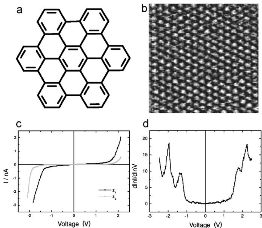
Fig. 16 a Chemical structure of hexabenzocoronene. b Constant height STM image of a double layer of hexabenzocoronene on Au(100). (Image size is 100\text{ nm} \times 100\text{ nm} , V = 0.65\text{ V} , I = 0.05\text{ nA} .) c I–V curves at two different tip–sample distances measured on the same site with a tungsten tip. The distance z_2 is nominally 0.25\text{ nm} larger. The separation z_1 is determined by the tunneling parameters I = 0.05\text{ nA} and V = 0.7\text{ V} . d Normalized differential conductance curve calculated from an I–V curve obtained at 0.2\text{ nA}/-1.5\text{ V} with a gold tip
