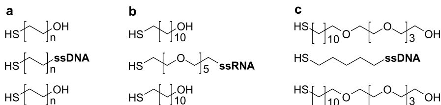
Fig. 22 Chemisorption of mixed SAMs of 5'-mercaptoalkyl-ssDNA (a, c) [164] or 5'-mercapto-PEG-ssRNA (b) [174] with various \omega -mercaptoalkanols on gold-coated AFM tips and supports [164, 174], and adjustment of optimal lateral DNA density with a 50 : 1 mixture of spacer and ssDNA in phosphate buffer (c) [175]
