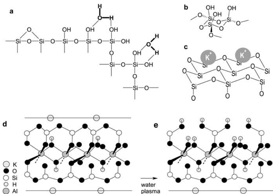
Fig. 3 Chemical structure of the silicon dioxide layer as formed on the surface of silicon or silicon nitride tips/chip under atmospheric conditions (a) and ideal surface structure of SiO 2 (b). In contrast, to SiO 2 , the surface of freshly cleaved mica (c) does not contain reactive silanol groups but electrostatically bound K + ions which can be exchanged for H 3 O + or divalent cations from aqueous solution. d Mica is a phyllosilicate in which two layers of condensed silicic acid are strongly held together by a layer of aluminum hydroxide. These trilayers are stacked and weakly held together by layers of K + ions which constitute predetermined fracture plains. e Water plasma activation partially fragments the silicate layer and generates reactive silanol groups. Parts d and e are reproduced from [129] with permission
