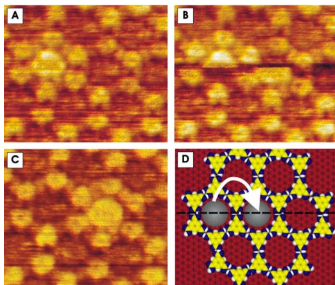
Fig. 5 STM images ( A–C 4.6 \times 4.6 \text{ nm}^2 ). A Single \text{C}_{60} molecule on a TMA network; B manipulation step: after half the molecule was scanned, the current was switched from 70 to 150 pA; C final result of the manipulation with the molecule moved into the adjacent cavity. D Illustration of the manipulation experiment. Reprinted with permission from [51]. © (2004) American Chemical Society
