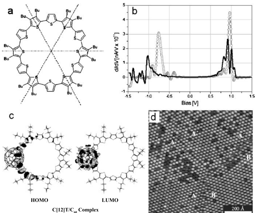
Fig. 25 a Molecular model of C[12]T. b Differential conductance ( dI/dV ) versus bias voltage (V) measured on top of a C[12]T-macrocycle (circles) and a C[12]T-C 60 complex (solid line). c Calculated molecular orbitals of complexed C[12]T molecule derived from an energy-minimized geometry. d STM image of C[12]T-C 60 complexes, including some non-complexed macrocycles
