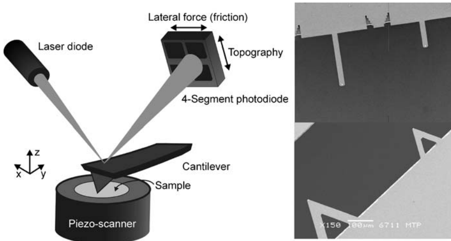
Fig. 6 Left : Schematic diagram of contact mode AFM; right : SEM images of single beam and V-shaped cantilevers
