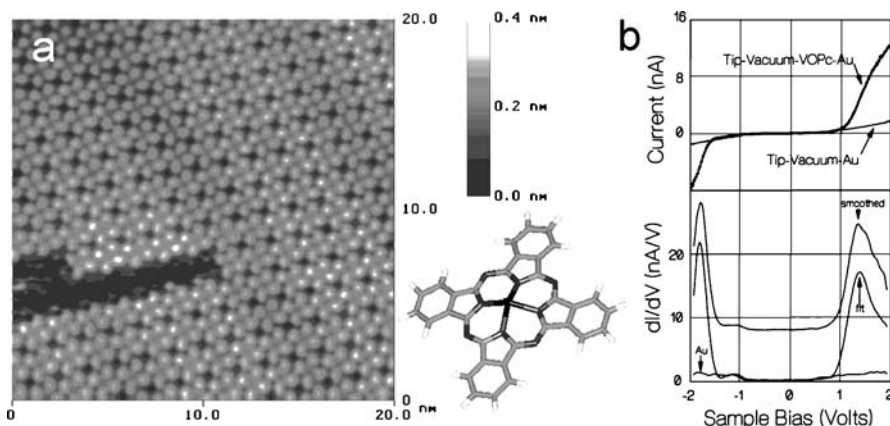
Fig. 10 a High-resolution STM image of a VOPc monolayer on Au(111). The image was acquired at 600 mV sample bias and 300 pA. A model of the VOPc molecule is shown in the lower right. b Area averaged I–V curves and generated dI/dV–V. The dI/dV–V was generated in two ways: the I–V curve was fit by a polynomial and the exact derivative of the polynomial was taken (indicated as fit), or the raw I–V data was smoothed and then a numerical derivative was taken (indicated as smoothed)
