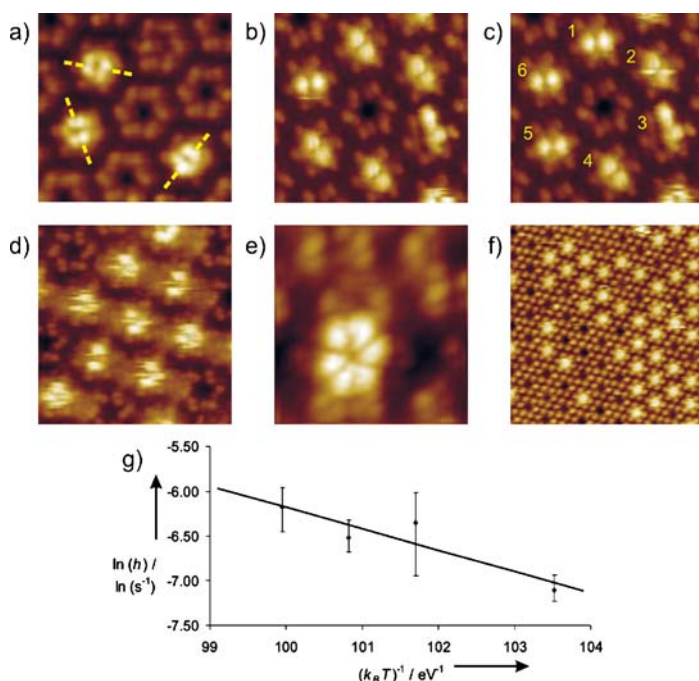
Fig. 33 a–f STM images of the porphyrin network ( I_t = 20 pA, V_s = -1.5 V). Sample coverage 10% (a–c) and 30–40% (a–f). a 77 K, 10.2 \times 10.2 nm 2 , b and c 112 K ( 7.4 \times 7.4 nm 2 ); d 115 K, 8.8 \times 8.8 nm 2 , e 150 K, 3.0 \times 3.0 nm 2 , f RT, 29.9 \times 29.9 nm 2 . g Arrhenius plot for the determination of the activation energy needed to switch between two neighboring positions. Reprinted with permission from [88]. © (2007) Wiley
