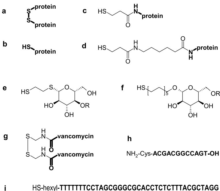
Fig. 21 Direct chemisorption onto gold-coated tips and/or supports of proteins or peptides via endogenous disulfides ( a ) [36, 76, 78, 94, 169] or thiols ( b ) [57, 110] or artificially introduced thiol groups ( c ) [170] and d [73]). The same strategy was used for chemisorption of carbohydrates with \omega -mercaptoalkyl groups ( e ) [69, 70] and f [166, 171]), of vancomycin-cystamin ( g ) [163], of a peptide nucleic acid with an N-terminal cysteine ( h ) [172], and of 5'-thiohexyl-ssDNA with a hairpin loop sequence ( i ) [106]
