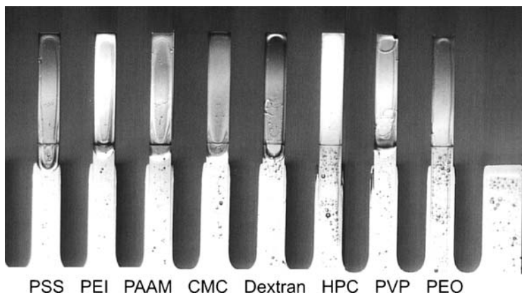
Fig. 7 Optical microscopy image of a polymer-coated microcantilever array for application as an artificial nose for solvents. The pitch between microcantilevers is 250 micron
