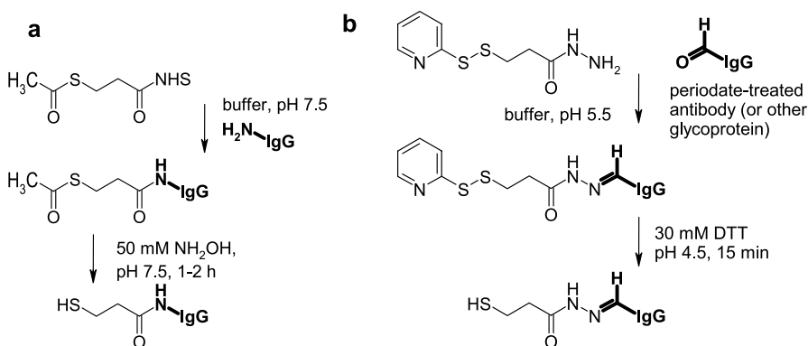
Fig. 11 Artificial introduction of thiol residues on antibody, either with SATP ( a ) [46, 145] or with pyridyldithiopropionic acid hydrazide ( b ) [147] and mild cleavage with DTT at pH 4.5 [148] in order to leave the disulfides in the protein structure intact
