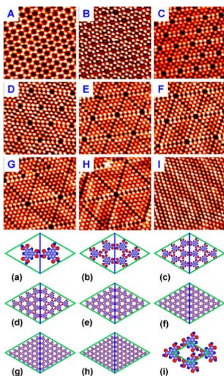
Fig. 14 Coverage induced evolution of TMA self-assembling structures on Au(111)-(22√3). Image size: 16.5 × 16.5 nm 2 . Reprinted with permission from [66]. © (2007) American Chemical Society
