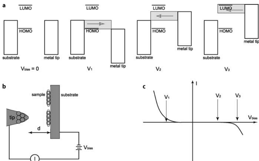
Fig. 1 Schematic diagram of orbital mediated tunneling spectroscopy and the STM/STS setup. In this example, the HOMO of the adsorbed molecule is closer to the Fermi level of the substrate than the LUMO. V is the applied tip bias. The arrow indicates the current flow. At positive tip bias (or negative sample bias) electrons tunnel from filled states of the substrate into the tip. At negative tip bias (or positive sample bias) electrons tunnel from the tip into empty states of the substrate. At certain potentials, the molecular orbitals may mediate the tunneling process. A resulting asymmetric I - V plot is shown in (c). The asymmetry is due to the asymmetric position of the molecular frontier orbitals versus the Fermi level of the substrate combined with the asymmetric position of the molecule in the tunneling gap. dI/dV - V spectroscopy typically reveals peaks if molecular orbitals are involved. For examples, see text
