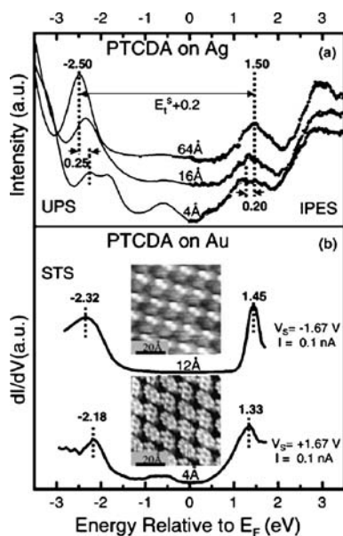
Fig. 5 Composite UPS/IPES spectra as a function of PTCDA thickness on Ag ( a ) and STS spectra recorded for a monolayer ( bottom ) and a 2–3 molecular layer ( top ) film of PTCDA deposited on Au (111). The corresponding STM images are also shown
