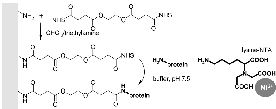
Fig. 15 Use of a short homobifunctional crosslinker to attach underivatized protein [117] or lysine-NTA [14] to aminofunctionalized mica
