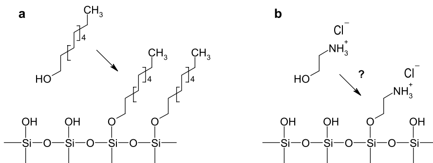
Fig. 8 Esterification of a glass surface (condensed silicic acid with embedded Na + counterions) with a perfect SAM of dodecanol at high temperature [118] and putative mechanism of AFM tip aminofunctionalization with ethanolamine hydrochloride in DMSO [44, 55]
