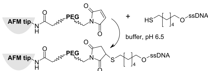
Fig. 13 Tethering of 5'-thiohexyl-ssDNA to aminofunctionalized tip via maleimide-PEG-NHS [40, 51, 60, 61] or a short heterobifunctional linker with a maleimide and NHS-ester function [134]
