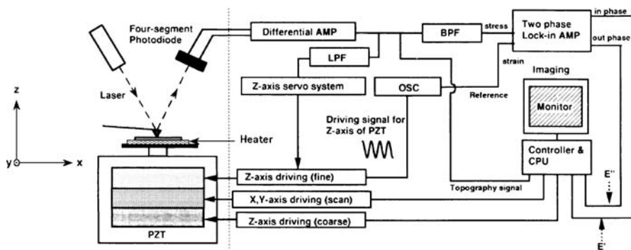
Fig. 15 Schematic of scanning viscoelasticity microscopy used for imaging of dynamic viscoelasticity by AFM. (Reprinted with permission from [97]. © (1994) American Chemical Society)
