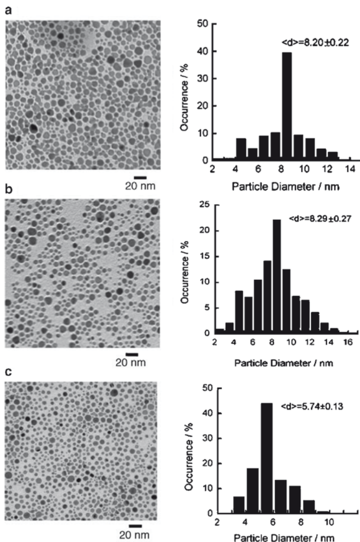
Fig. 8 TEM images and size distribution of Ag(0) nanoparticles obtained by chemical reduction of the Ag-ILs with NaBH 4 . a [Ag(eth-hex-en) 2 ] 2 NO 3 *0.3 H 2 O liquid. b [Ag(eth-hex-en) 2 ] 2 NO 3 *5 H 2 O. c [Ag(eth-hex-en) 2 ] 2 NO 3 *0.3 H 2 O + eth-hex-en (molar ratio = 1:1). Image adapted from [181]. Image Copyright Wiley-VCH (2008)
