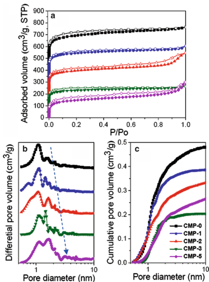
Fig. 8 Gas sorption characterization data for series of CMP polymers [19]. \text{N}_2 adsorption-desorption isotherms measured at 77.3 K (a), adsorption branch is labelled with filled symbols . For clarity, the isotherms of CMP-0, CMP-1, CMP-2, and CMP-3 were shifted vertically by 400, 300, 200, and 100 \text{cm}^3 \text{g}^{-1} , respectively. NL-DFT pore size distribution curves, (b); the dashed arrow indicates the shift to larger average pore size in this series. Cumulative pore volume curve calculated by application of NL-DFT, (c)
