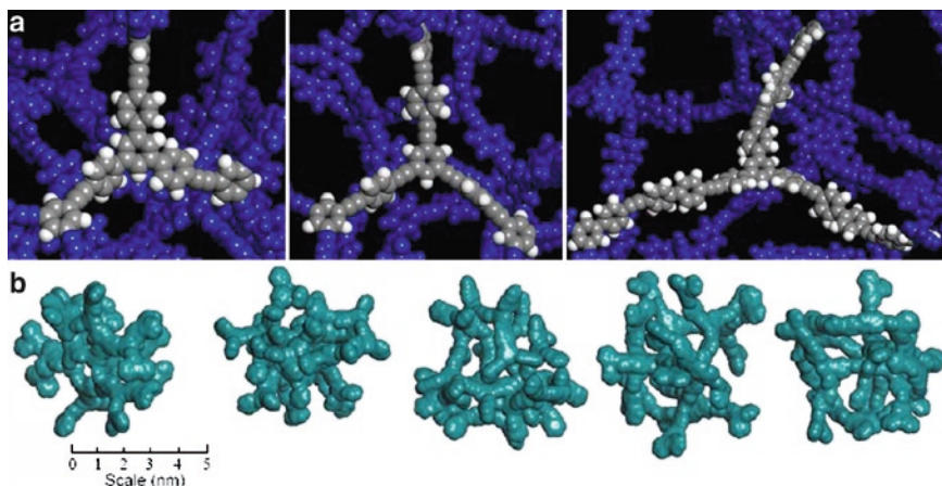
Fig. 9 Atomistic simulations for PAE networks with different strut lengths [19]. Node-strut topology for simulated network fragments for CMP-0 (left), CMP-1 (centre), and CMP-5 (right), (a). Atomistic simulations of network fragments for CMP-0, CMP-1, CMP-2, CMP-3, and CMP-5 (left to right), (b). A solvent accessible surface is shown (in green) in each case (solvent diameter=0.182 nm)
