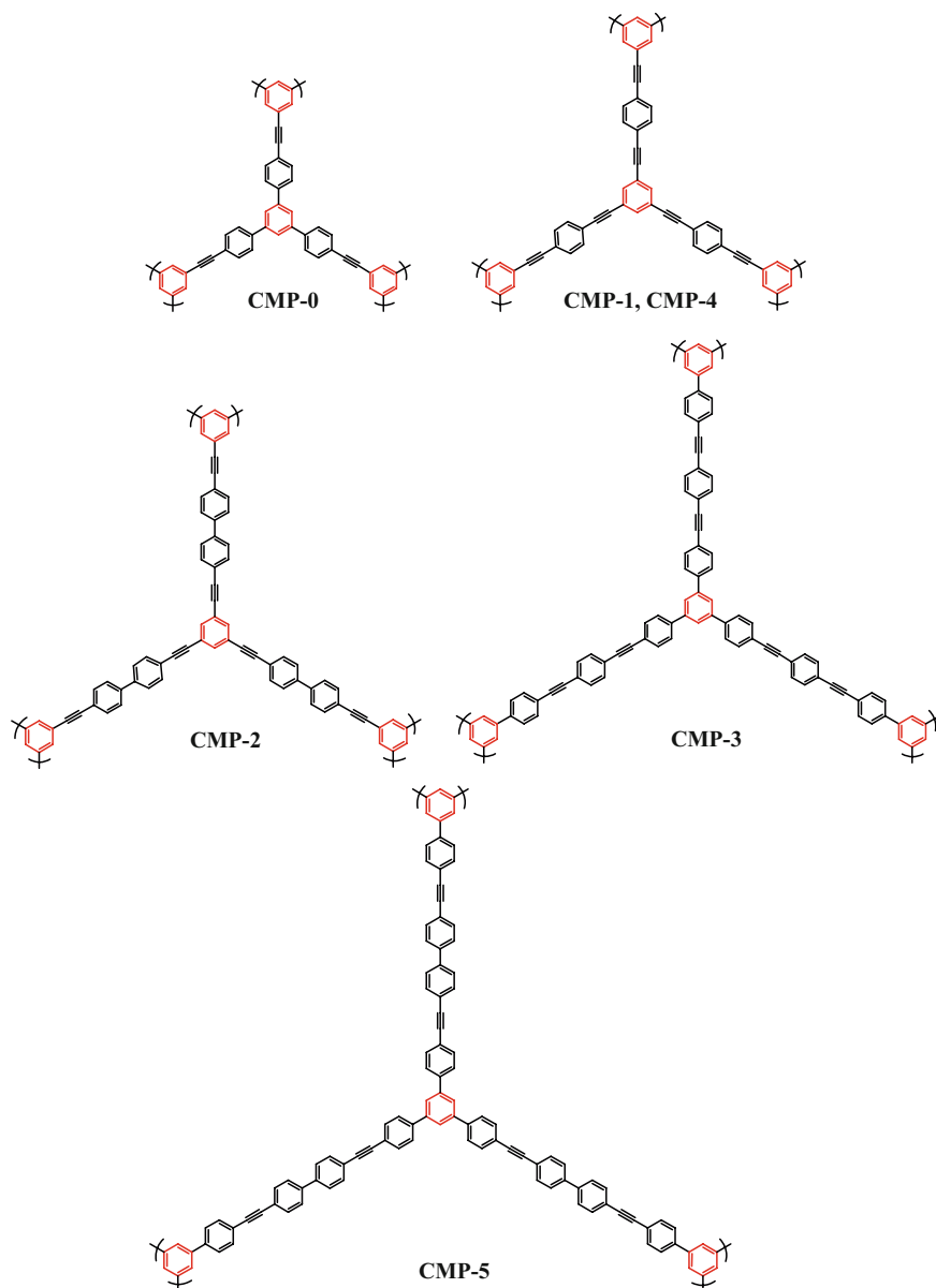
Fig. 7 “Node-strut” topology for series of CMPs networks produced by Sonagashira–Hagihara cross-coupling chemistry [19]. The benzene “nodes” are shown in red . The total number of ethyne plus benzene links per “strut” increases in increments of one from two (CMP-0) to six (CMP-5) in this series of samples. It should be stressed that these are simple representations of the repeat unit structures for the networks. The actual three-dimensional materials have more complex structures and include both terminal alkyne and halogen end groups (see also molecular simulations, Fig. 9)
