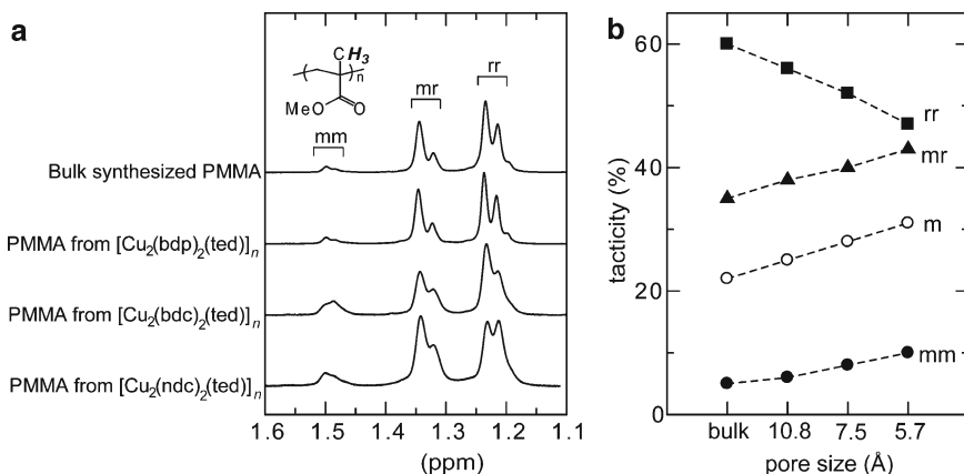
Fig. 6 (a) ^1\text{H} NMR spectra of Poly(methyl methacrylate) (PMMA) obtained from the nanochannels of [\text{Cu}_2(\text{L})_2(\text{ted})]_n and the bulk condition in nitrobenzene- d_5 at 110^\circ\text{C} . (b) Plot of nanochannel size effect on tacticity of PMMA
