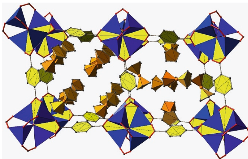
Fig. 3 Cut-out of the crystal structure [60] of the inclusion compound ferrocene 7 @MOF-5
