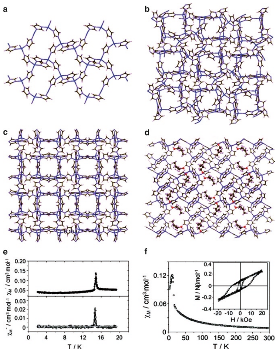
Fig. 16 Views and magnetic properties of the open-framework coordination polymers based on cobalt imidazoles. (a) Evacuated [\text{Co}(\text{im})_2] \cdot 0.5\text{Ch} . (b) [\text{Co}(\text{im})_2]_4 . (c) [\text{Co}(\text{im})_2]_2 . (d) [\text{Co}_5(\text{im})_{10} \cdot 0.4\text{Mb}]_5 . (e) Plots of temperature dependence of ac susceptibility obtained at 0.1 Oe field for [\text{Co}(\text{im})_2] \cdot 0.5\text{Ch} . A peak appears at 15 K, which is indicative of the ferromagnetic character of this compound. (f) Plot of the thermal evolution of the \chi_M for [\text{Co}(\text{im})_2]_2 at 10 kOe field. The inset shows the hysteresis loop at 1.8 K ( \square ) and 5.0 K ( \circ ). (Co, blue; O, red; C, brown; N, violet; H, white. Solvent guest molecules in (d) are represented as spheres) Reprinted from ref 168 [Tian YQ, Cai C-X, Ren X-M, Duan C-Y, Xu Y, Gao S, You X-Z, "The Silica-Like Extended Polymorphism of Cobalt(II) Imidazolate Three-Dimensional Frameworks: X-ray Single-Crystal Structures and Magnetic Properties" (2003) Chem Eur J 9:5673]. Copyright Wiley-VCH Verlag GmbH & Co. KGaA. Reproduced with permission
