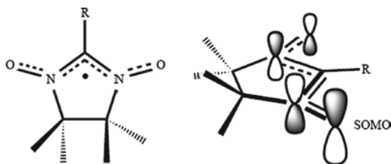
Fig. 4 General chemical structure of the family of \alpha -nitronyl nitroxides and a representation of their singly occupied molecular orbitals (SOMO). Reprinted from ref. 55 [Amabilino DB, Cirujeda J, Veciana J, “Crystal architectures of organic molecular-based magnets”, (1999) Phil Trans R Soc Lond A 357:2873] by permission of The Royal Society, Copyright 1999
