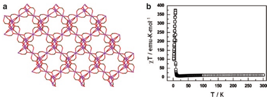
Fig. 9 (a) Structure of evacuated [Mn 3 (1) 6 ] showing the 1-D channels. (Mn, purple; O, red; C, brown). (b) Temperature dependence of the \chi \cdot T product for an applied magnetic field of 100 Oe. Reproduced from ref. 82 by permission of The Royal Society of Chemistry. http://dx.doi.org/10.1039/b314221c
