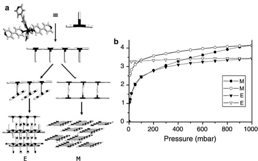
Fig. 19 (a) View of the structures of [\text{Ni}_2(\text{NO}_3)_4(4,4'\text{-bipyridine})_3]_\infty ; forms E and M. (b) Hysteretic \text{H}_2 adsorption-desorption at 77 K [187]. Reproduced by kind permission of the authors
