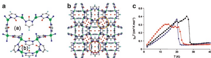
Fig. 24 Structure and magnetic properties for [\text{Cu}(\text{F-pymo})_2(\text{H}_2\text{O})_{1.25}]_n (a) Metallacalix[8]arenes (a) and metallacalix[4]arenes (b) cyclic motifs. (b) Gismondine-like framework (guest water molecules are represented as red spheres). (c) \chi_M \cdot T versus temperature for as-synthesized (blue), activated (red) and \text{CO}_2 -loaded (black) materials. Reprinted with permission from ref 212. Copyright 2008, American Chemical Society
