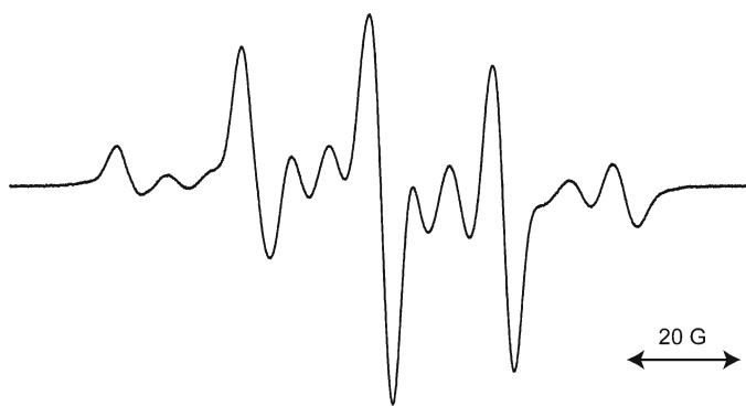
Fig. 9 ESR spectrum for propagating radical of Poly(methyl methacrylate) (PMMA) in the nanochannel of [\text{Zn}_2(\text{bdc})_2(\text{ted})]_n
