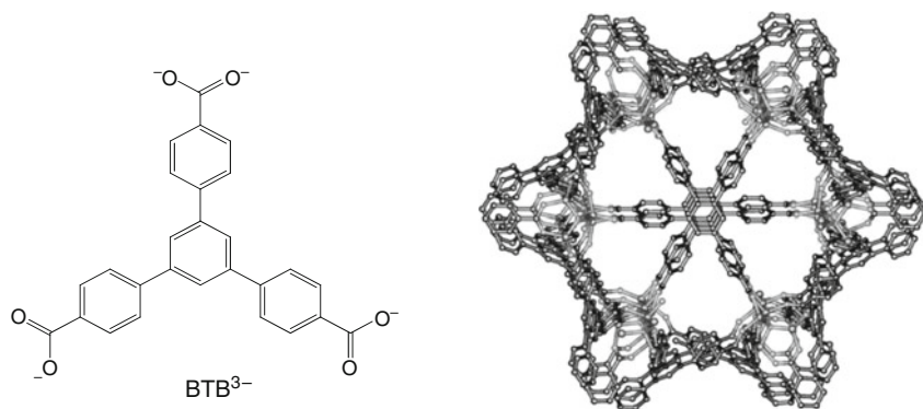
Fig. 4 View of the linker \text{BTB}^{3-} and the structure of MOF-177 [100]. Reproduced by kind permission of the authors
