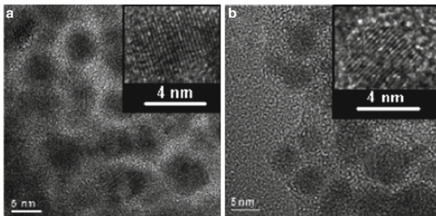
Fig. 21 HRTEM images of Ag nanoparticles formed by immersion of [\text{Ni}(\text{cyclam})]_2[\text{BPTC}] \cdot 2n \text{H}_2\text{O} in the EtOH solution of \text{AgNO}_3 ( 1.3 \times 10^{-1} \text{ M} ) at room temperature (a) for 5 min and (b) for 16 h [90]. Copyright Wiley-VCH Verlag GmbH & Co. KGaA. Reproduced with permission
