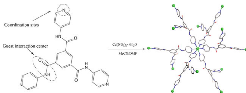
Scheme 7 Synthetic scheme for MOFs that contain amide groups in the bridging ligands
