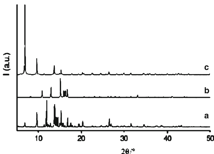
Fig. 4 Powder X-ray diffractograms of (a) [\text{Ru}(\text{cod})(\text{cot})]@ \text{MOF-5} , (b) [\text{Ru}(\text{cod})(\text{cot})] and (c) MOF-5. Reproduced with permission from [64]. Copyright 2008 American Chemical Society
