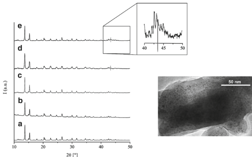
Fig. 16 Powder X-ray diffraction patterns of (a) pure, activated MOF-5, (b) [CpCu(PMe 3 )]@MOF-5, (c) [CpCu(CN'Bu)]@MOF-5, (d) Cu@MOF-5 (derived from [CpCu(PMe 3 )]@MOF-5) (e) Cu@MOF-5 (derived from [CpCu(CN'Bu)]@MOF-5). TEM image of Cu@MOF-5 (derived from [CpCu(PMe 3 )]@MOF-5). Reproduced with permission [80]. Copyright 2008 American Chemical Society
