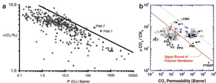
Fig. 14 Robeson plot showing high \text{O}_2/\text{N}_2 separation selectivities for PIM-1 and PIM-7, (a) [77]. Relation between \text{CO}_2 permeability and \text{CO}_2/\text{CH}_4 selectivity of thermally rearranged polyimides, (b) [78]
