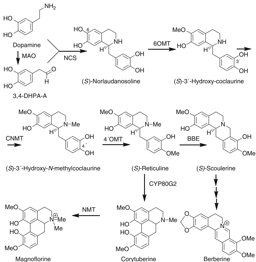
Fig. 18 Reconstructed isoquinoline alkaloid biosynthetic pathway in microbes ( E. coli and S. cerevisiae ) [120]. Accession numbers of the genes can be taken from Gene Bank. (3,4-DHPA-A 3,4-dihydroxyphenylacetaldehyde; NCS norcoclaurine synthase; 6OMT 6-O-methyltransferase; CNMT coclaurine-N-methyltransferase; 4'OMT 4'-O-methyltransferase; BBE berberine bridge enzyme; NMT N-methyltransferase)
