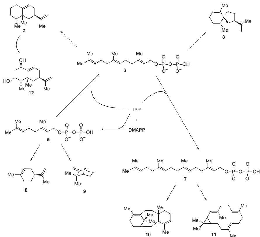
Fig. 2 Biosynthetic route to terpenes. Geranyl diphosphate (5); farnesyl diphosphate (6); geranylgeranyl diphosphate (7); (–)-limonene (8); (–)-camphene (9); taxadiene (10); casbene (11); capsiadiol (12). IPP = isopentenyl diphosphate, DMAPP = dimethylallyl diphosphate
