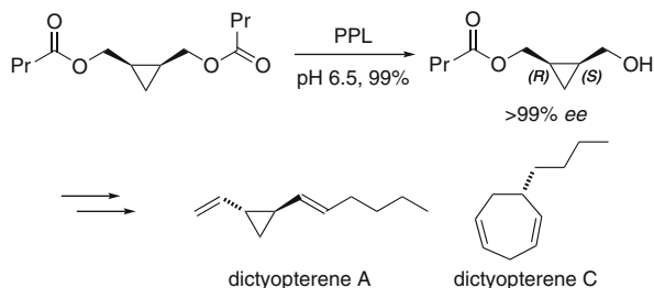
Fig. 2 Chemoenzymatic synthesis of dictyopterene A and C
