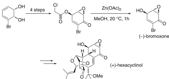
Fig. 30 Chemoenzymatic access to epoxyquinols
