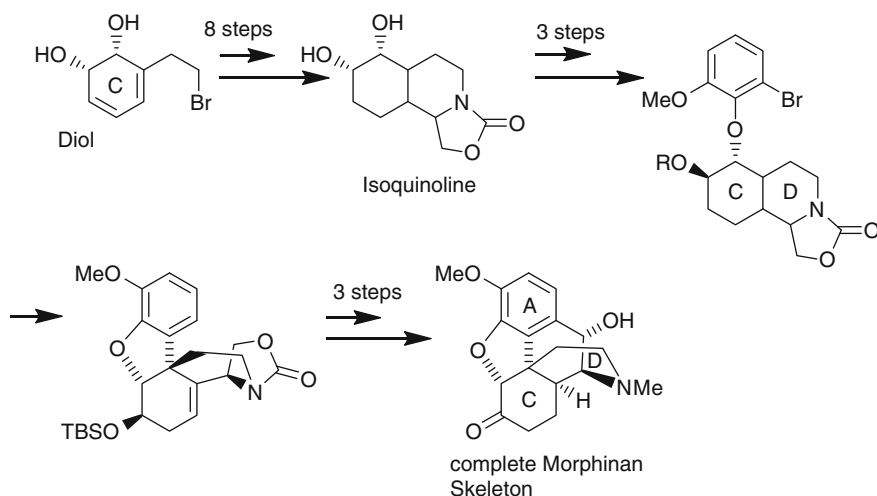
Fig. 20 Fourteen-step synthesis of the complete morphinan skeleton of morphine and codeine, starting with the enzymatically formed diol providing ring C of the carbon frame work of these alkaloids [129, 130]
