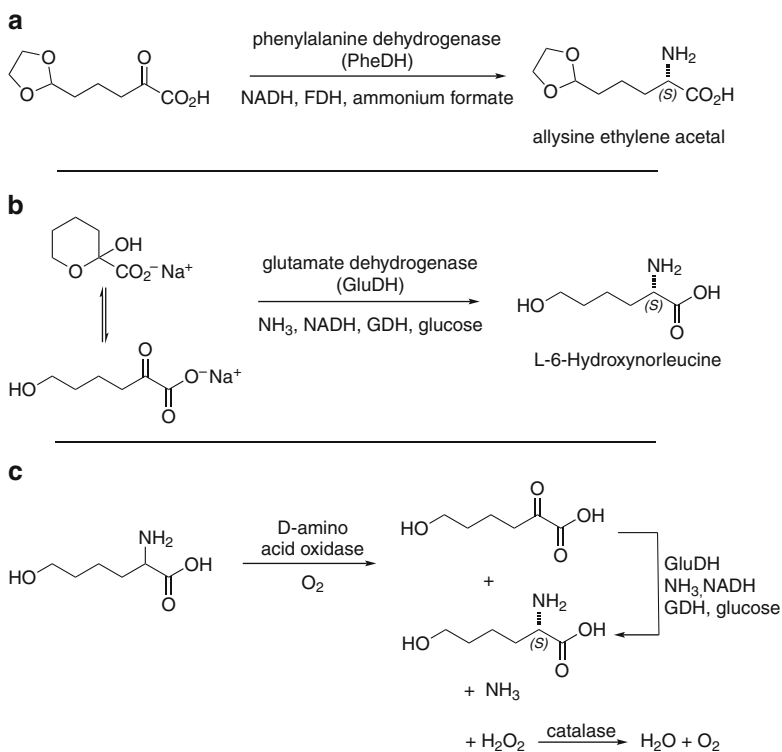
Fig. 21 Enzymatic synthesis of unnatural amino acids as building blocks for omapatrilat. (a–c) Enzymatic approaches to 6-oxonorleucine analogs
