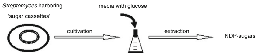
Fig. 2 Chemo- and bioenzymatic strategies toward NDP-sugars
