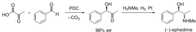
Fig. 42 Chemoenzymatic synthesis of (–)-ephedrine
