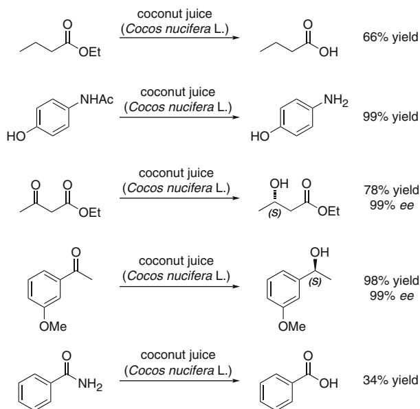
Fig. 1 Enzymatic reactions catalyzed by coconut juice ( Cocos nucifera )
