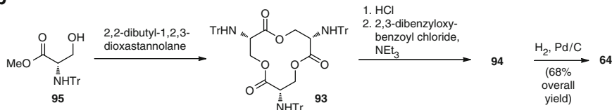
Fig. 16 Chemical syntheses of 64 via (a) the first and (b) the currently most efficient organotin template strategies
