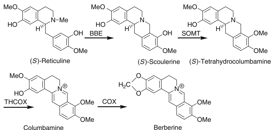
Fig. 17 Sequential enzymatic formation of berberine from (S)-reticuline (BBE berberine bridge enzyme; SOMT scoulerine O-methyltransferase; THCOX tetrahydrocolumbamine oxidase; COX columbamine oxidase)
