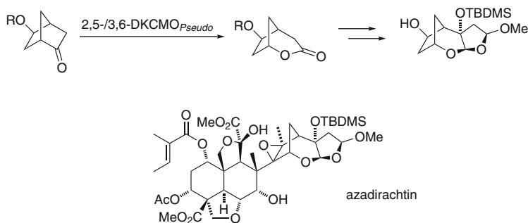
Fig. 26 Chemoenzymatic approach to azadirachtin
