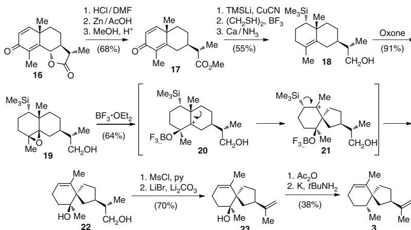
Fig. 5 Synthetic route to (–)-premnaspirodiene ( 3 )
