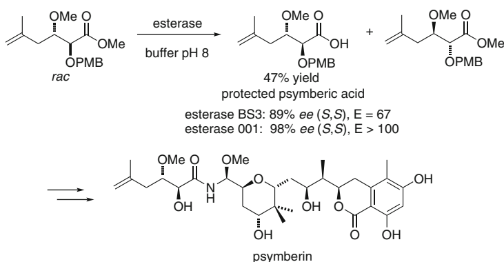
Fig. 7 Chemoenzymatic synthesis of PMB-protected psymberic acid
