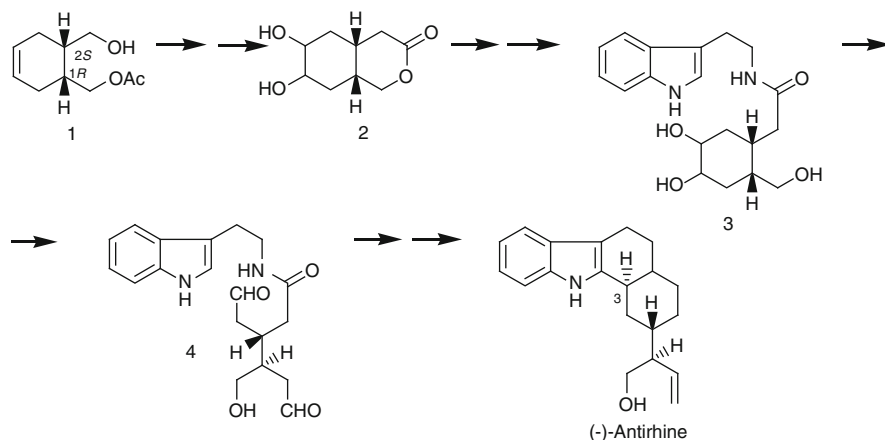
Fig. 11 Complete synthesis of the major alkaloid (–)-antirrhine known from the plant Antirrhoea putaminosa (except for formation of 1, all other reaction steps were not enzyme-catalysed)
