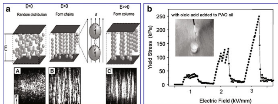
Fig. 2 Working principle of GERF. (a) GERF stays in liquid state when no electric field ( E ) is applied, begins to form chains under a moderate field of 500 V/mm, and then grows into columns as electric field increases. (b) Yield stress of hydrocarbon oil-based GERF with oleic acid additive, as function of applied electric field [33]
