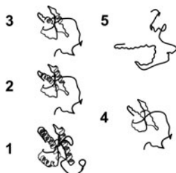
Fig. 4 Proposed intermediate states during the unfolding of PrP 90-231 . Schematic showing the intermediate states of PrP as measured by NMR, starting from natively folded monomer (1) and progressing into the unfolded state (5). Reproduced from [65] with permission from the author and the journal Biochemistry
