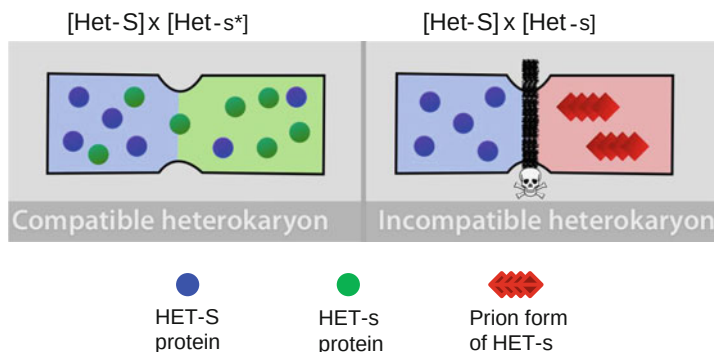
Fig. 3 [Het-s] prion-regulated heterokaryon incompatibility in Podospira anserina . The fungal hyphae expressing the HET-S protein (designated [Het-S]) are only able to fuse with hyphae expressing the soluble form of the HET-s protein (designated [Het-s*]) if HET-s is in the non-prion form of this protein. If the hyphae do express the prion form of HET-s (designated [Het-s]) then hyphal fusion triggers a lethal reaction at the point of contact, thereby preventing mixing of the cytoplasmic components of the two hyphal types
