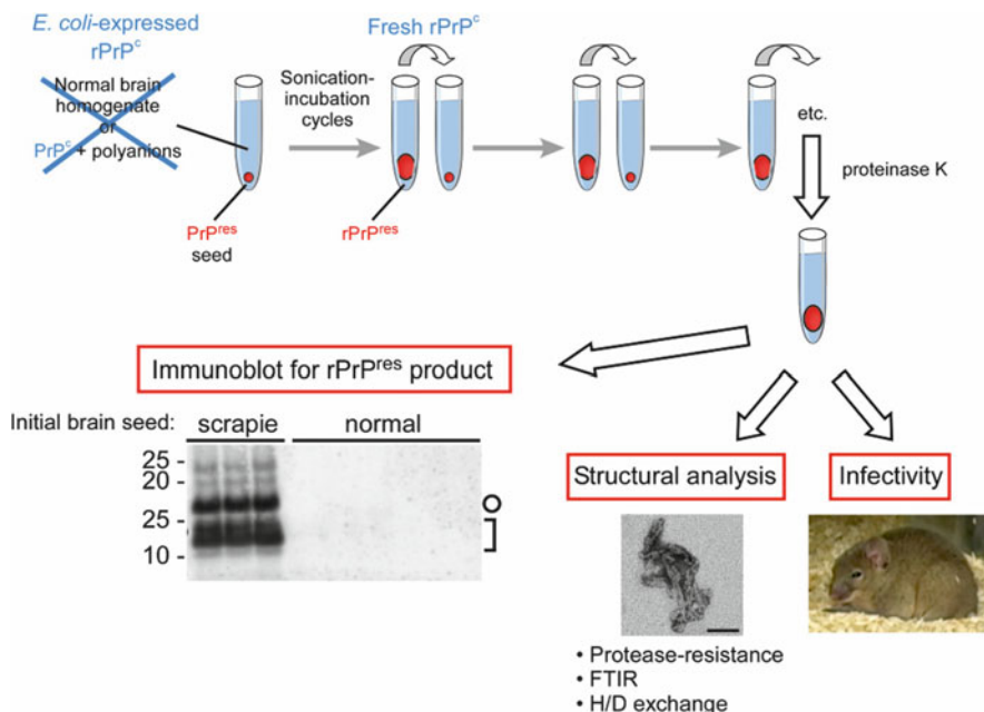
Fig. 1 Summary of the biochemical, structural and biological studies on recombinant-PMCA (r-PMCA) products. Immunoblot and electron microscopy image adapted from [26]
