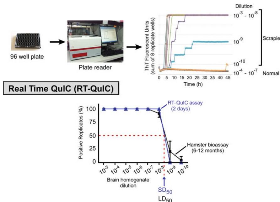
Fig. 3 Diagram of Real Time QuIC RT-QuIC and comparison of end-point dilution titrations of scrapie brain homogenate by RT-QuIC with animal bioassay. ( Top panel ) RT-QuIC analysis of normal and scrapie brain homogenate (BH) dilutions using hamster (90–231) rPrP C as a substrate. ( Bottom panel ) Comparison of hamster brain homogenate end point dilution titrations by RT-QuIC and animal bioassay. The Spearman–Kärber estimate of the SD 50 (i.e., seeding dose giving sufficient Thioflavin T fluorescence in half of the replicate wells) per 2 \mu L of neat brain tissue is indicated. Graphs adapted from [55]
