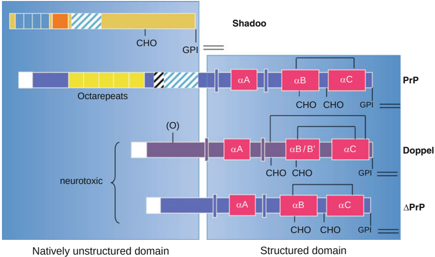
Fig. 1 Domain structure of the PrP protein family. Sho, PrP, Dpl, and internally deleted forms of PrP, noted here, generically, as ΔPrP are shown. The proteins are organized around natively unstructured and \alpha -helical structured domains. The exact boundaries between the domains are approximate. The central hydrophobic tract is indicated by blue diagonal shading (see also Fig. 4). For the Sho protein the blue shaded rectangles indicate degenerate arginine-glycine-glycine (RGG) repeats. The orange shaded rectangle encompasses a different type of arginine-rich tract of the general form RVRVRPAPR. White boxes in PrP and Dpl indicate an N-terminal tract of charged residues. The diagonally shaded box with black stripes indicates a second type of charged patch. CHO indicates N-linked carbohydrates. Disulfide linkages are shown by black lines . Alpha helices are shown as crimson boxes ( \alpha A , \alpha B , and \alpha C ) while narrower boxes denote \beta -strands. GPI denotes the glycosylphosphatidyl inositol anchor
