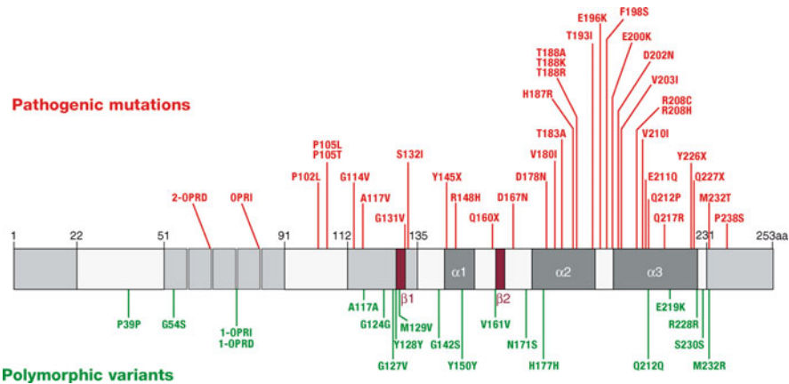
Fig. 1 Diagram of the human prion protein gene showing the octapeptide repeat region (51–91), regions of predicted secondary structure [designated α (helical) or β (sheet)], pathogenic or likely pathogenic mutations (above in red), non-synonymous polymorphisms and synonymous polymorphisms (below in green)
