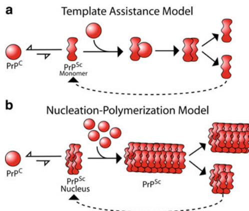
Fig. 5 Models of prion replication. (a) The template assistance model predicts that a PrP Sc monomer is more stable than PrP C , but is kinetically inaccessible. In the rare event that a PrP Sc monomer is created spontaneously (or provided exogenously), it can template the misfolding of another PrP C molecule by direct interaction. The dashed line shows that the newly created PrP Sc monomer can act as another seed to formation of PrP Sc . (b) The nucleation polymerization model predicts that barrier to prion protein conversion is the formation of a nucleus in which the protein adopts a PrP Sc -like structure. The formation of such a low order aggregate is not favored; however, once it has formed, polymerization from a pool of PrP C molecules can take place efficiently. Fragmentation of the polymer increases the number of ends for the recruitment of PrP C monomers
