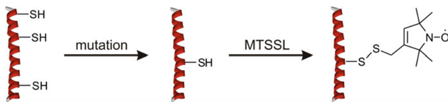
Fig. 5 Scheme of site directed spin labeling (MTSSL: Methanethiosulfonate Spin Label)
