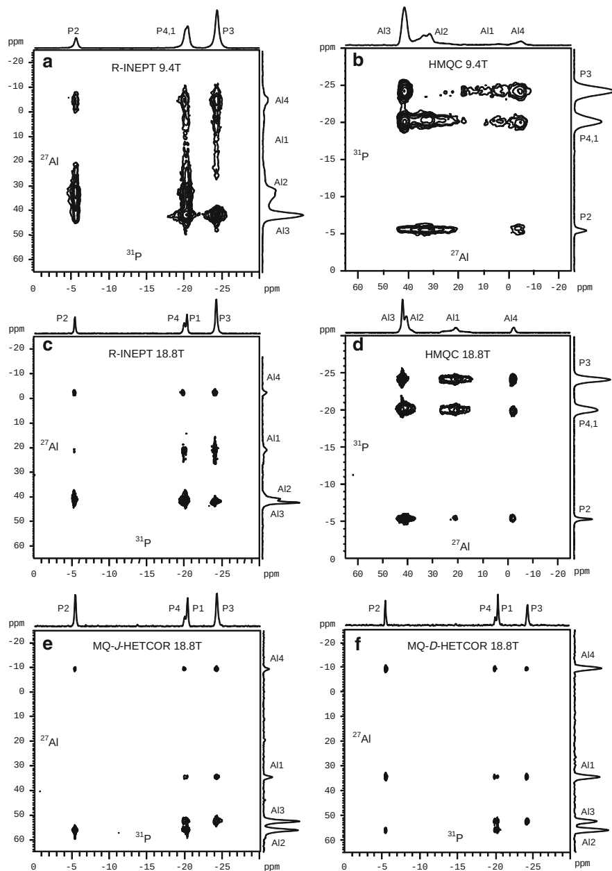
Fig. 20 2D HETCOR spectra of \text{AlPO}_4\text{-14} : (a) ^{27}\text{Al} \rightarrow ^{31}\text{P} R-INEPT at 9.4 T, (b) ^{27}\text{Al}\{^{31}\text{P}\} HMQC at 9.4 T, (c) ^{27}\text{Al} \rightarrow ^{31}\text{P} R-INEPT at 18.8 T, (d) ^{27}\text{Al}\{^{31}\text{P}\} HMQC at 18.8 T, (e) ^{27}\text{Al} \rightarrow ^{31}\text{P} SPAM-MQ-J-HETCOR with R-INEPT at 18.8 T, and (f) ^{27}\text{Al} \rightarrow ^{31}\text{P} SPAM-MQ-D-HETCOR obtained using cross-polarization at 18.8 T. The total experimental times were 5 h (a), 5 h (b), 2 h (c), 2 h (d), 10 h (e) and 7 h (f). (Reproduced with permission from [235])
