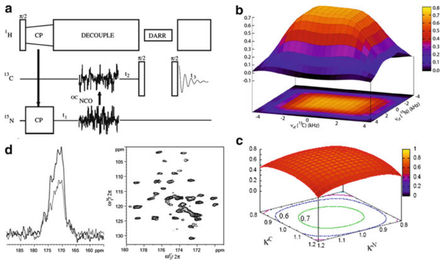
Fig. 11 (a) 2D NCO experiment with optimal control element inserted for ^{15}\text{N} \rightarrow ^{13}\text{C}' transfer. Transfer efficiencies for the ^{\text{OCNCO}} experiment optimized for 12 kHz spinning speed as function of (b) resonance offsets for ^{13}\text{C}' and ^{15}\text{N} and (c) rf inhomogeneity/adjustment in terms of scaling factors on the nominal rf field strengths for ^{13}\text{C} and ^{15}\text{N} . (d) Experimental ^{\text{OCNCO}} 2D spectrum of uniformly ^{13}\text{C} , ^{15}\text{N} -labeled ubiquitin with the projections to the left comparing ^{\text{OCNCO}} experiment ( most intense ) and DCP ( less intense ) based NCO experiments [reproduced with permission from [161] (a, d) and [164] (c)]
