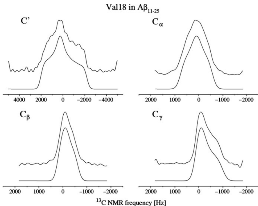
Fig. 11 ROCSA spectra for Val-18 of A\beta_{11-25} fibrils. The C' spectrum was measured at 9.39 T under a MAS frequency of 20 kHz. The other spectra were measured at 14.09 T under the frequency of 11 kHz. Upper traces are experimental spectra. Lower traces are best-fit simulations for one-spin system. The rf carrier frequency is at 0 Hz. (Figure and caption adapted from [158]. Copyright [2003], American Institute of Physics)
