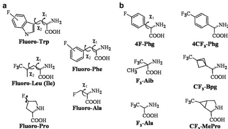
Fig. 3 Important ^{19}\text{F} -labelled amino acids. (a) Compounds that are iso -stereic to native amino acids can be incorporated into proteins biosynthetically, but they possess too many degrees of torsional freedom to be useful for ssNMR structure analysis. (b) In these artificial amino acids the ^{19}\text{F} -reporter group is rigidly attached to the peptide backbone. They can be incorporated by solid-phase peptide synthesis, but some problems can arise due to racemisation (4F-Phg, 4CF 3 -Phg), steric hindrance of coupling (F 3 -Aib) or HF elimination (fluoro-Ala, F 3 -Ala). 4F-Phg is additionally problematic due to an ambiguity of the side-chain rotamer. The preferred ^{19}\text{F} -labels for ssNMR structure analysis are CF 3 -Bpg and CF 3 -Phg (as suitable substitutes for Leu, Ile, Met, Val and Ala), as well as F 3 -Aib and CF 3 -MePro
