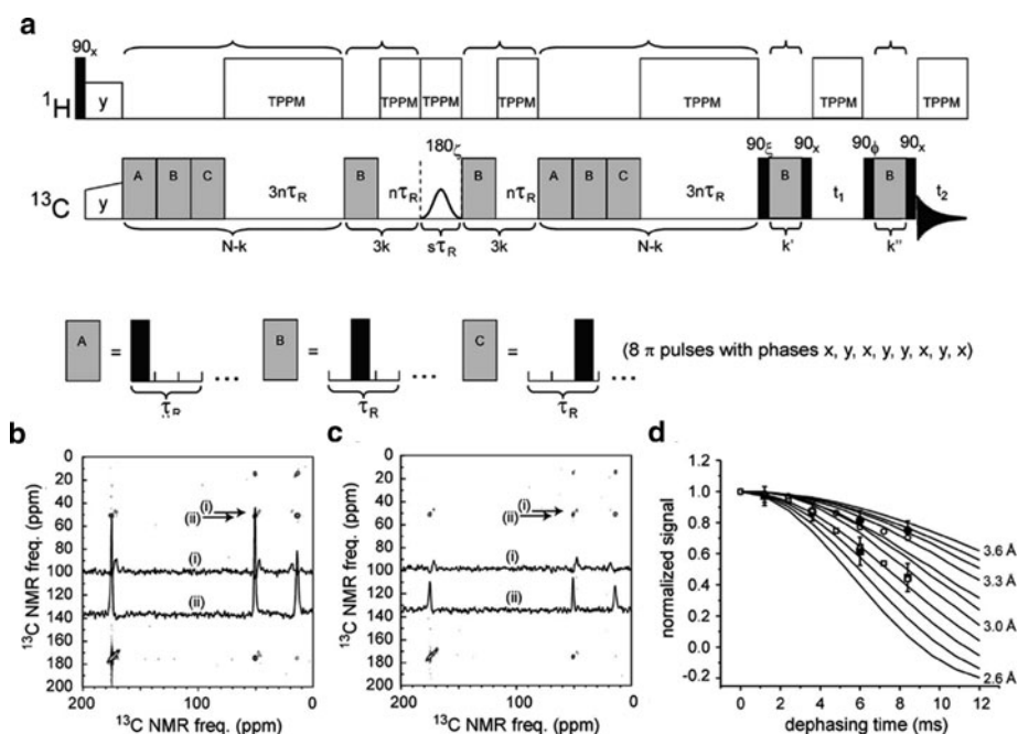
Fig. 9 (a) Constant-time frequency-selective pulse sequence used for indirect measurement of ^{13}\text{C}' - ^{13}\text{C}' distances in MB(i + 4)EK with uniformly ^{15}\text{N} , ^{13}\text{C} -labeled L-alanine at Ala9 and Ala10. The 2D spectra in (b) and (c) and the extracted data points in (d) show that the dephasing is more rapid, with hence a shorter internuclear distance, for ^{13}\text{C}' nuclei in the helical conformation (represented by squares ) than for those in the non-helical conformation (represented by circles ) (reproduced from [149] with permission)
