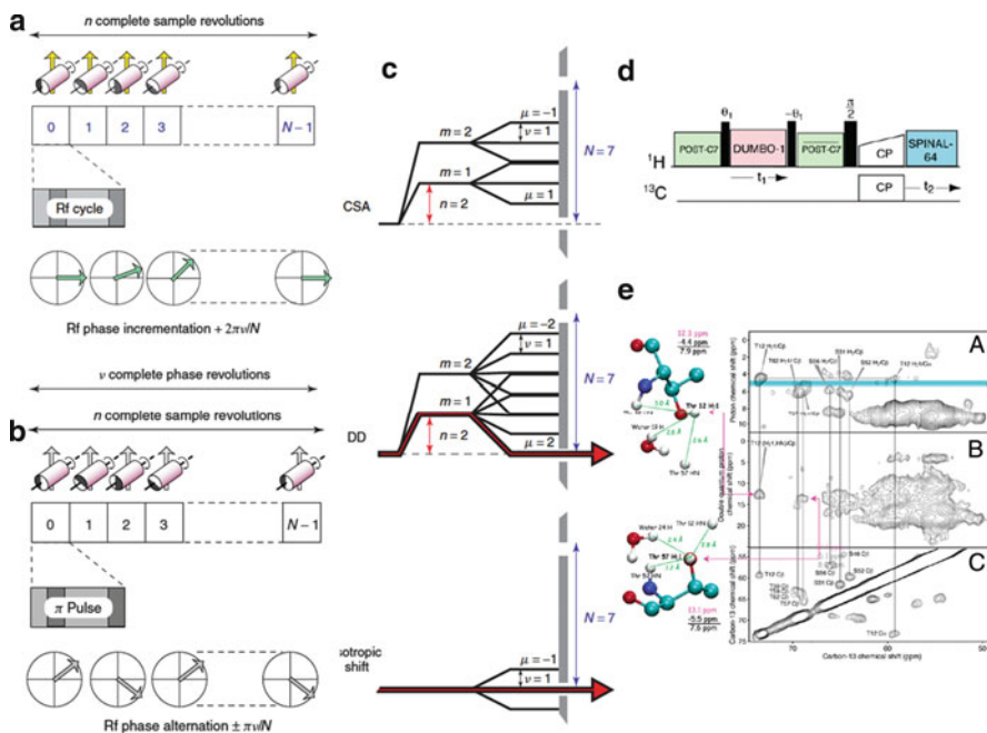
Fig. 5 Symmetry-based dipolar recoupling illustrated in terms of pulse sequences for the CN_n^v (a) and RN_n^v (b) pulse sequences, a spin-space selection diagram for the C7_2 symmetry (c) (reproduced from [118] with permission). Application of POST- C7_2 [31] as an element in a ^1\text{H} - ^{13}\text{C} double-quantum vs ^{13}\text{C} chemical shift correlation experiment (d) used as elements (B panel) in a study of water binding to polycrystalline proteins (reproduced from [119] with permission)
