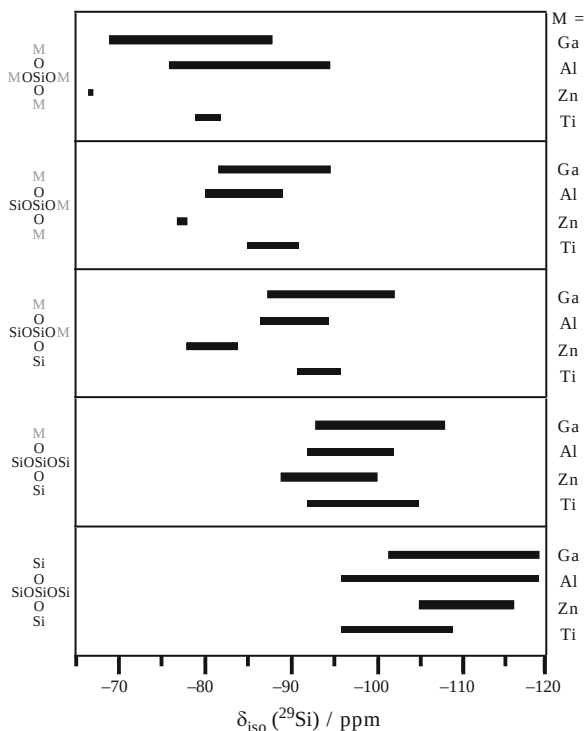
Fig. 1 ^{29}\text{Si} chemical shift scales for tetrahedral \text{Si}(n\text{M}) units in zeolites; data for Al were adapted from [24] for a large variety of zeolites, data for other substitutions are taken from: Ga: zeolites A, X, Y, L, sodalite, offretite, mazzite, ZSM-5 [21], TNU-1, TNU-4, sodalite, ZSM-5 [48], beta [49–52], paulingite [53], and natrolite [54]; Zn: VPI-7, VPI-9, \text{Na}_2\text{ZnSiO}_4 , kkalovite, \text{K}_2\text{ZnSi}_4\text{O}_{10} [55], sodalite [56], RUB-17, VPI-7 [57, 58]; Ti: ETS-4, natisite, sphene, lorenzenite, \text{Na}_2\text{TiSi}_2\text{O}_7 , \text{Ba}_2\text{TiSi}_2\text{O}_8 (fresnoite), benitoite, \text{K}_2\text{TiSi}_3\text{O}_9 , narsarsukite, \text{Cs}_2\text{TiSi}_6\text{O}_{15} , \text{CsTiSi}_2\text{O}_{6.5} [59], ETS-10 [60, 61], AV-11 [62], AM-18 [63], JLU-1 [64], penkvelkisite [65], nenadkevichite [66]
