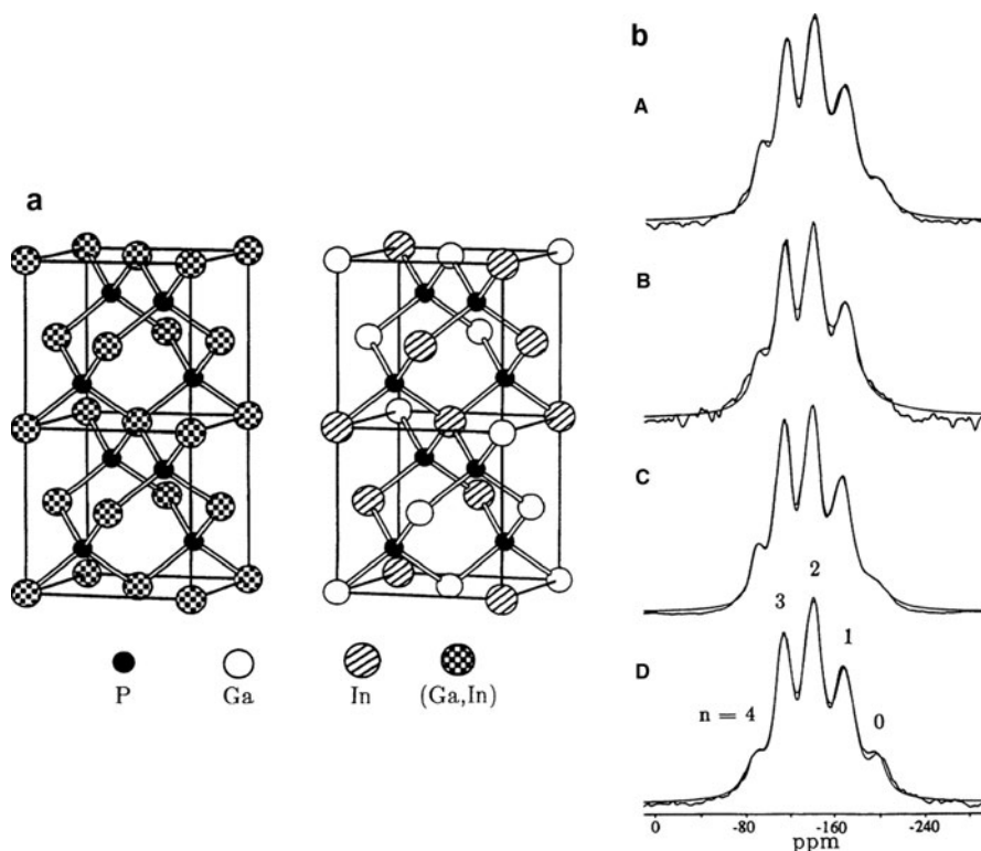
Fig. 5 (a) Random ( left ) and fully ordered ( right ) \text{Ga}_{0.5}\text{In}_{0.5}\text{P} structures. (b) ^{31}\text{P} MAS-NMR spectra of four different \text{Ga}_{0.5}\text{In}_{0.5}\text{P} films A–D and least-squares fit. Reprinted with permission from [146]. Copyright 1992 by the American Physical Society
