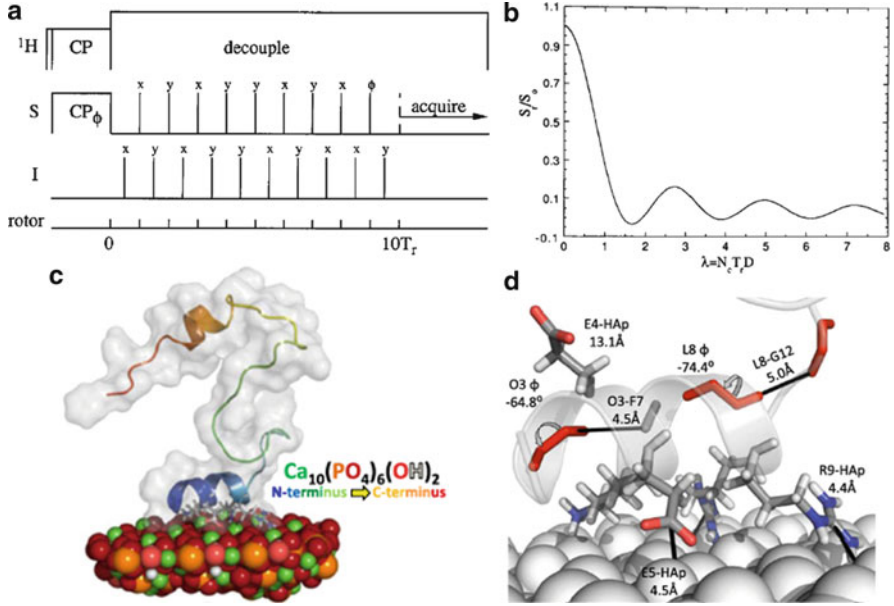
Fig. 1 (a) REDOR experiment and (b) typical REDOR dephasing curve (D designates the dipole–dipole coupling, \tau_r the rotor period, and N_c the number of rotor cycles for the REDOR experiment) (reproduced from [78] with permission). (c, d) REDOR based determination of statherin binding to a hydroxyapatite surface (reproduced from [79] with permission)
