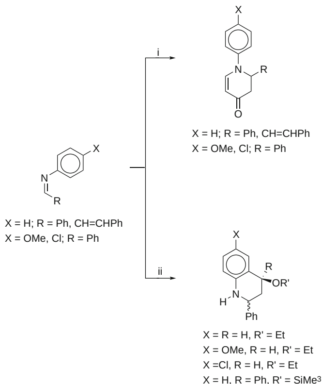
Scheme 15 Aza Diels–Alder reactions catalyzed by Bi(OTf)_3 \cdot xH_2O . Reaction conditions: (i) 1, CH_3OCH = C(OSiMe_3)Me , Bi(OTf)_3 \cdot xH_2O (0.05–0.1 eq.); 2, H_2O . (ii) 1, HC(OEt) = CH_2 or PhC(OSiMe_3) = CH_2 , Bi(OTf)_3 \cdot xH_2O (0.05–0.1 eq.); 2, H_2O
