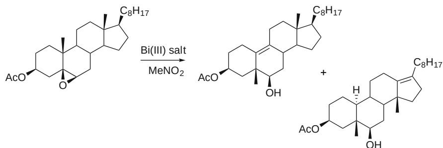
Scheme 31 Bismuth(III) salt-catalyzed rearrangement of 5 \beta ,6 \beta -epoxycholestan-3 \beta -yl acetate using MeNO 2 as solvent
