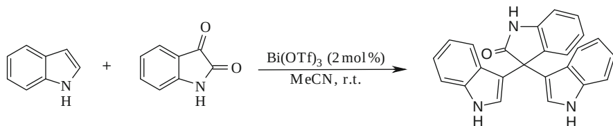
Fig. 12 Reaction of indole with isatin to form 3,3-di(3-indolyl)oxindole
