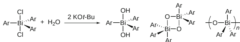
Scheme 1 Synthesis of organobismuth(V) reagents
