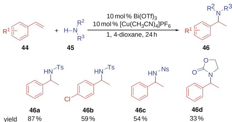
Scheme 34 \text{Bi}(\text{OTf})_3 -catalyzed hydroamination of styrenes
