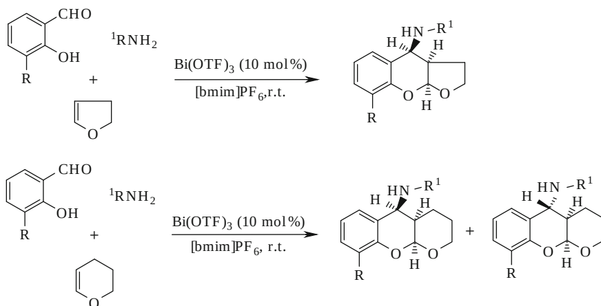
Fig. 24 Synthesis of cis -fused pyano- and furanobenzopyran
