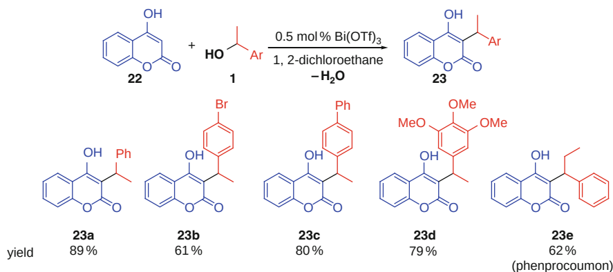
Scheme 19 Bi(OTf) 3 -catalyzed synthesis of novel warfarin derivatives
