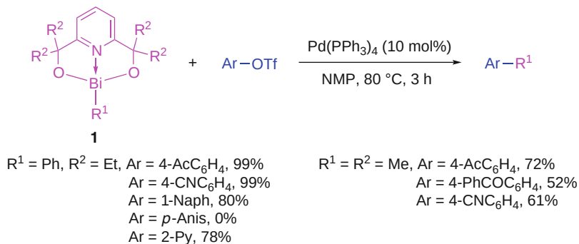
Scheme 28 Cross-coupling reaction of organobismuth alkoxides with aryl triflates
