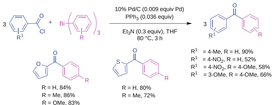
Scheme 23 Cross-coupling reaction of Ar 3 Bi with acid chlorides using Pd/C system
