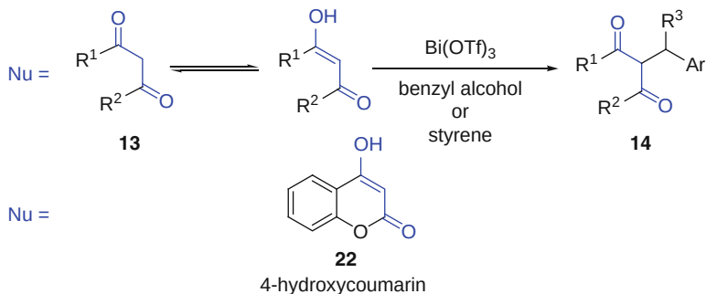
Scheme 18 Structural similarities between acetylacetonate and 4-hydroxycoumarin
