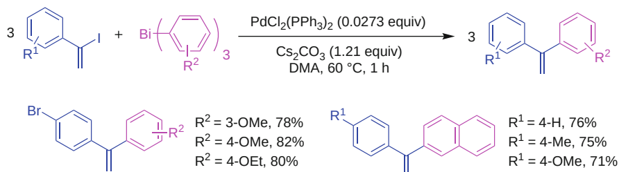
Scheme 41 Cross-coupling reaction of Ar 3 Bi with 1-iodovinylbenzenes
