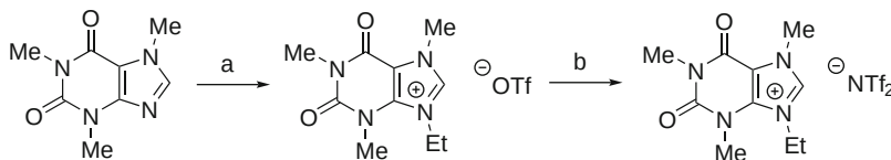
Scheme 4 Preparation of 1,3,7-trimethyl-9-ethylxanthiniumbis(trifluoromethanesulfonyl) amide [\text{CafEt}][\text{NTf}_2] . Reagents and conditions: (a) \text{EtOTf} (1.2 eq.), \text{PhNO}_2 , 100^\circ\text{C} , 16 h; (b) \text{LiNTf}_2 (1 eq.), acetone, room temperature
