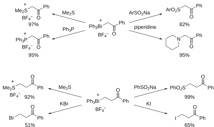
Scheme 12 Reactions of 2-oxoalkyl- and 3-oxoalkyl-triphenylbismuthonium salts with hetero nucleophiles [33–35]
