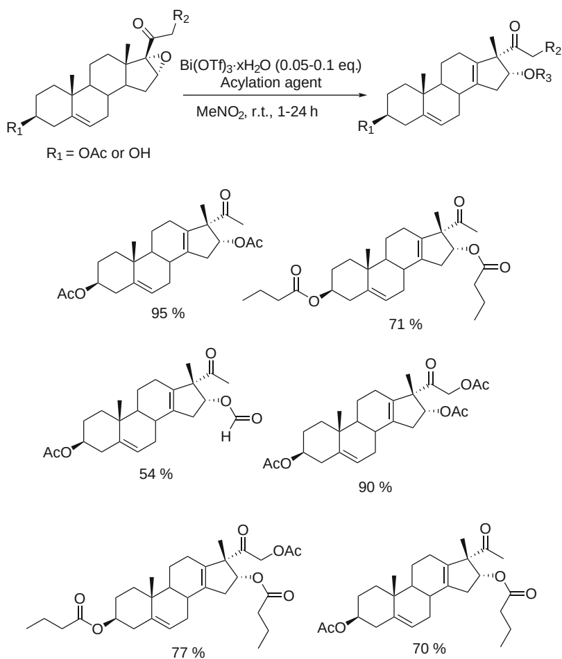
Scheme 36 \text{Bi}(\text{OTf})_3 \cdot x\text{H}_2\text{O} -catalyzed rearrangement of 16\alpha,17\alpha -epoxy-20-oxosteroids in the presence of an acylation agent
