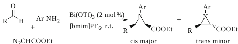
Fig. 26 Synthesis of cis -aziridine carboxylates
