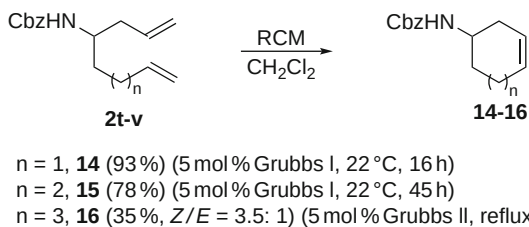
Scheme 4 Ring-closing metathesis of terminal dienes
