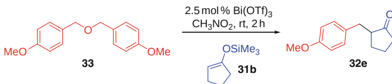
Scheme 25 Dibenzyloxy compounds as the putative reactive precursors for the benzylation of silyl enol ethers
