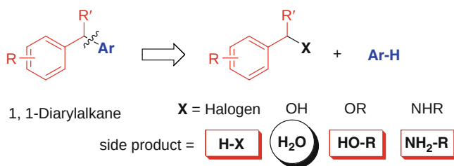
Scheme 3 Retrosynthetic analysis of 1,1-diaryllkanes
