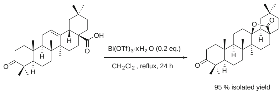
Scheme 42 \text{Bi(OTf)}_3 \cdot x\text{H}_2\text{O} -promoted lactonization of oleanonic acid
