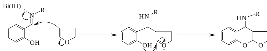
Fig. 25 Mechanism of formation of furanobenzopyran
