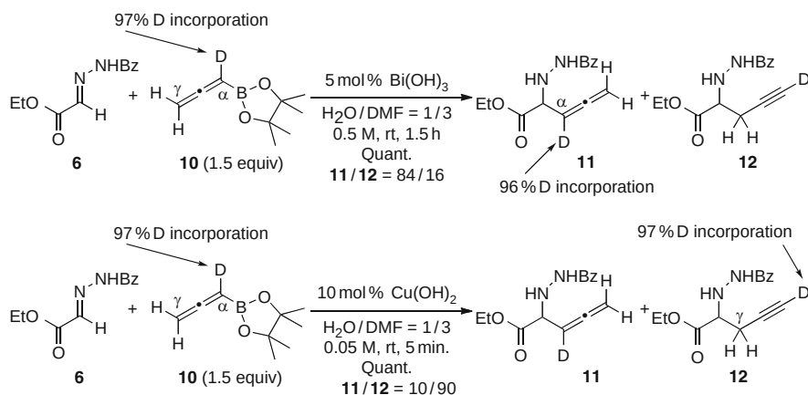
Scheme 4 Deuterium-labeling experiments
