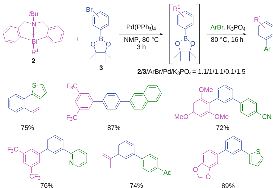
Scheme 36 One-pot multicoupling reaction using azabismocines and bromophenylboronates
