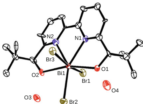
Fig. 1 Ortep drawing of the X-ray crystal structure of [\text{BiBr}_3 \cdot 2] \cdot (\text{H}_2\text{O})_2 \cdot \text{DME} . DME is omitted for clarity
