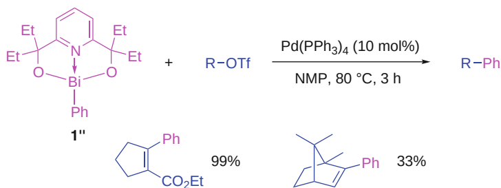
Scheme 39 Cross-coupling reaction of phenylbismuth alkoxide with alkenyl triflates
