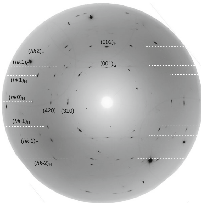
Fig. 15 2D diffraction pattern from a quasi-single-crystal of Sc-II at 48 GPa. The relative spacing of the layers of reflections from the host (hkl)_H and guest (hkl)_G structures (compare to Fig. 14), and the presence of the (001) guest reflection confirms the guest structure to be C-centred
