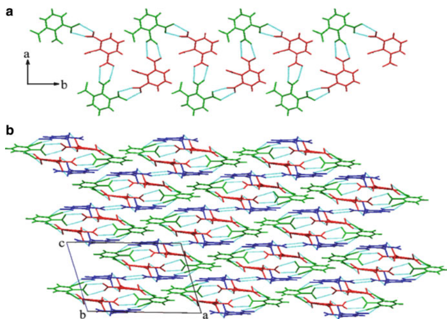
Fig. 14 Crystal structure of BTCA , with the three crystallographically independent molecules displayed in different colours (A, green; B, blue; C, red): (a) a hydrogen-bonded chain of A and C molecules viewed approximately along the c -axis, and (b) the complete crystal structure viewed along the b -axis (the AC chains run into the page, with adjacent AC chains cross-linked by hydrogen bonding to B molecules)
