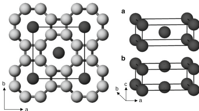
Fig. 12 The composite incommensurate structure of Sc-II, as viewed down the c axis. The eight-atom host framework is shown in grey , and the 1D guest chains are shown in black . The insets show perspective views of (a) the body-centred guest structure of Fujihisa et al. and (b) the C-centred guest structure of McMahon et al. The crystallographic axes are labelled
