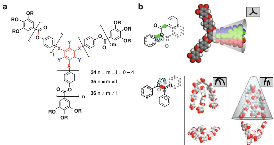
Fig. 8 General structure of semi-flexible oligobenzoate Hekates 34–36 . (a) These stars may consist of three identical arms ( 34 ) or two ( 35 ) or three ( 36 ) different arms. Thereby the length ( n, m, l ), the peripheral chains ( R', R'', R''' ), the linking groups X (OOC, COO, CONH) to the core and the substituents Y (H, I) can be adjusted. (b) Borderline conformers – star-shaped, E -shaped and cone-shaped conformers – for a non-symmetric oligobenzoate scaffold ( X = \text{OOC} ). They can be created by rotation about the C–O single bond within the carboxy linking group to the core
