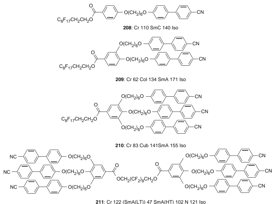
Fig. 69 Examples of oligomesogens incorporating semiperfluorinated chains ( T^{\circ} C) [364–366]
