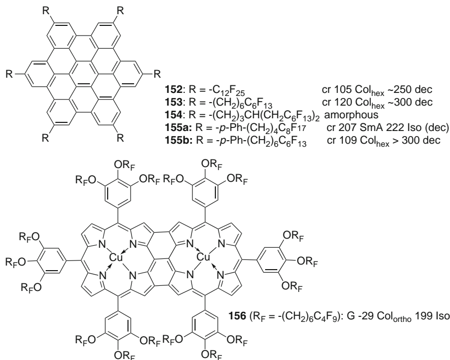
Fig. 42 Effect of chain fluorination on the LC phases of peri-hexabenzocoronene based mesogens (compounds 152–155 ) [274–276] and the fused metalloporphyrin dimer 156 ( T^\circ C); G = glassy state, \text{Col}_{\text{ortho}} = orthorhombic phase [277]
