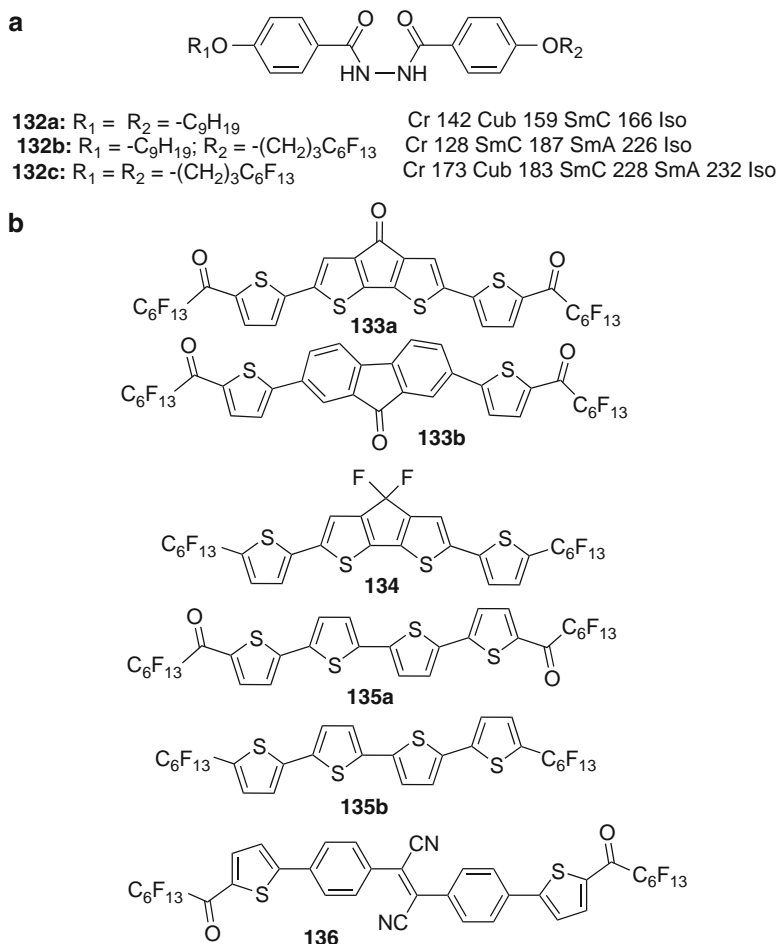
Fig. 35 Examples of (a) mesogenic dibenzoylhydrazines 132a–c ( T_i^\circ C) [122] and (b) thiophene based \pi -conjugated aromatics [250–255]
