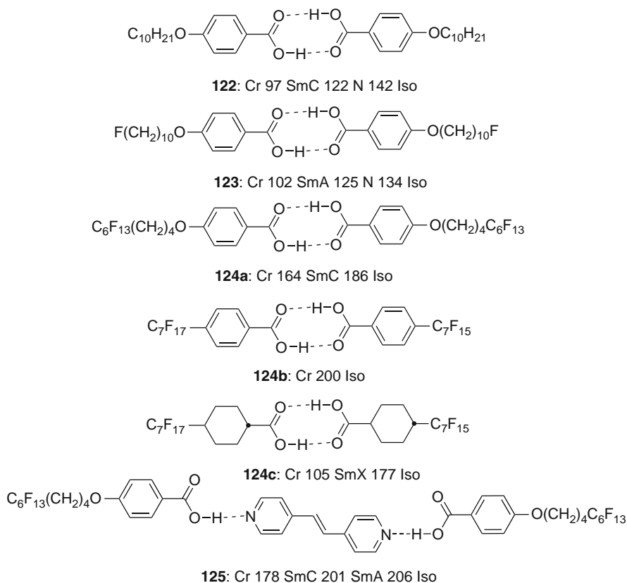
Fig. 33 Examples of supramolecular rod-like mesogens formed by self assembly of fluorinated benzoic acid and a trans -4- R_F -cyclohexane carboxylic acid ( T^\circ C) [120, 122]
