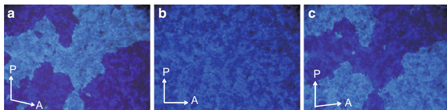
Fig. 2 Polarizing optical micrographs in the B4 phase of bent-core LC. Under crossed polarizers, texture with bluish color is observable ( middle ). By decrossing polarizers, two brighter and darker domains are observable ( right and left ). The brightness is interchanged by decrossing polarizers to counter senses [11]
