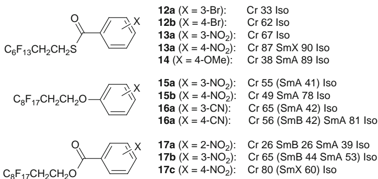
Fig. 9 Comparison of selected examples of compounds combining one semiperfluorinated chain with a benzene ring, showing the effects of substituent type and position ( T^{\circ}\text{C} ) [113, 115, 117, 120]
