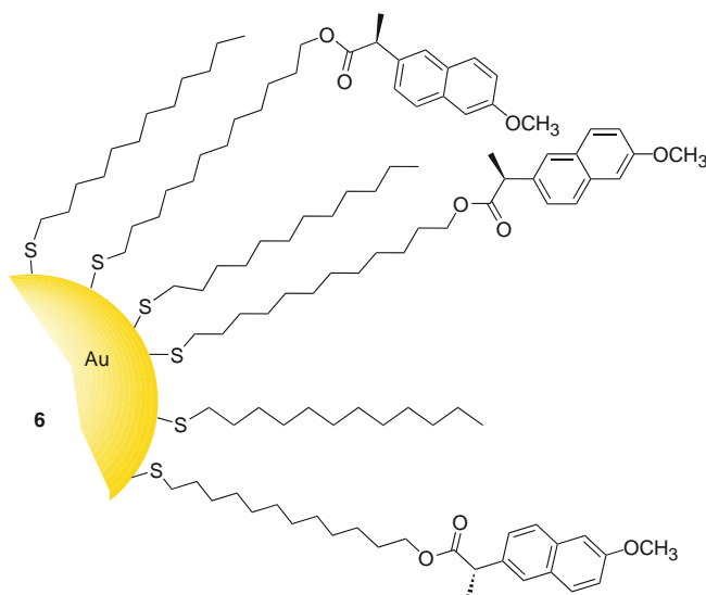
Fig. 11 Mixed monolayer alkylthiol-capped gold nanoparticle end-functionalized with (S)-naproxen chiral dopant moieties [349, 365, 366]
