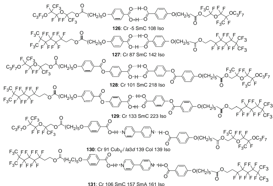
Fig. 34 Examples of supramolecular rod-like mesogens formed by self assembly of branched fluorinated benzoic acid into dimers and their 4,4'-bipyridine complexes ( T^{\circ}\text{C} ) [166]
