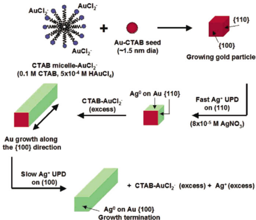
Scheme 3 Nanorod growth mechanism in the presence of \text{Ag}^+ ions [170]. (Copyright © 2006, American Chemical Society)
