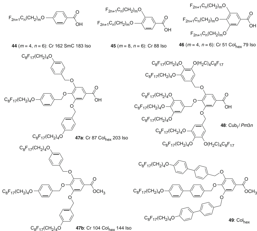
Fig. 16 Representative examples of semiperfluorinated benzoic acids and methyl benzoates with fluorinated chains ( T^\circ\text{C} ) [126, 133, 134, 136, 144–146]
