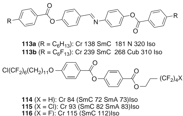
Fig. 31 Selected examples of rod-like mesogens with semiperfluorinated chains at both ends and the effect of modification of one chain end ( T^\circ\text{C} ) [202, 203]
