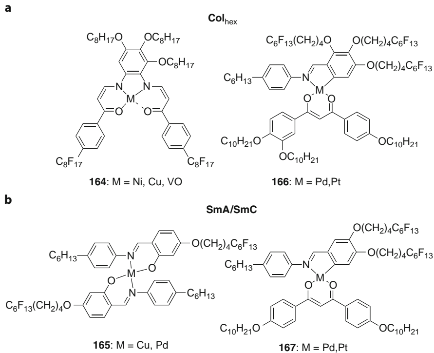
Fig. 44 Representative fluoros metallomesogens with disc-like and board-like shape ( T^\circ C) [40, 41, 294]
