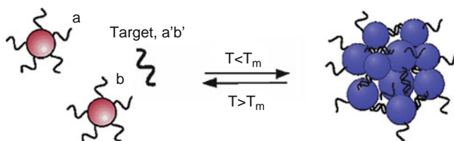
Fig. 29 Two families of gold nanoparticles are functionalized with different non-complementary DNA sequences a and b . The strands are designed to recognize a single target sequence a'b' , which then assembles the particles into clusters. Reproduced with permission from [127]
