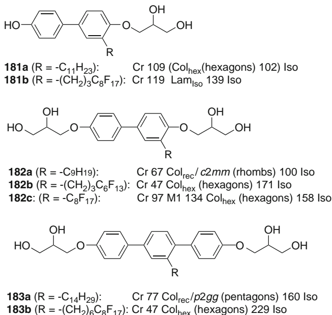
Fig. 51 Examples of T-shaped bolaamphiphiles with non-polar lateral R_F/R_H -chains showing the effect of fluorination on mesophase types and transition temperatures ( T^\circ C) [316–318, Lehmann A, Prehm M, Tschierske C, unpublished results, 319]
