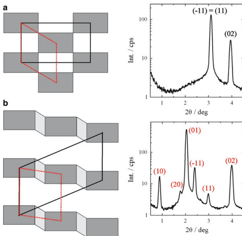
Fig. 3 Left: Schematic models of 2D modulated structures; dark regions are filled with the aromatic parts of molecules. The possible choices of the primitive ( dotted red ) and the body centered ( solid black ) crystallographic unit cells are shown for both phases. Right: The corresponding XRD patterns. (a) B1-type phase: the layer fragments are only displaced and there are no connecting regions of different density. XRD signals are indexed assuming the body centered unit cell. (b) B1rev-type phase: layer fragments are connected by defects in which the electron density is lower than in the blocks. XRD Miller indices are given assuming the primitive unit cell. Note that the position of the main, most intensive signal in the X-ray pattern of the B1 and B1rev phase is much different despite the similar sizes of the blocks
