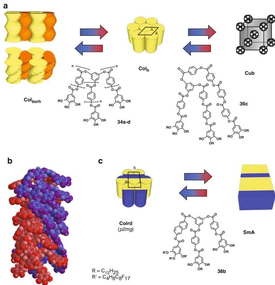
Fig. 10 Different LC structures formed from \text{C}_3 -symmetric or non- \text{C}_3 -symmetric oligobenzoate Hekates. (a) 3D ordered mesophases based on an undulated columnar topology of helical stacks as proposed for E -shaped oligobenzoates 34a–d in the soft crystal and thermotropic LC phases ( left ) and their transition to the hexagonal phase ( \text{Col}_{\text{h}} ). Formation of the micellar cubic mesophase in the series of folded non-symmetric mesogens (e.g. 36c ) and the transformation to the hexagonal phase ( right ). (b) Model of the helical packing of E -shaped oligobenzoate scaffolds of 34a . (c) 2D columnar mesophase ( \text{Col}_{\text{rd}} rectangular columnar) in the rare plane group p2mg and the transition to the lamellar structure ( \text{SmA} ) for a mesogen 38b containing semi-perfluorinated chains. Copyright Wiley-VCH Verlag GmbH & Co. KGaA. Reproduced with permission from reference [2]
