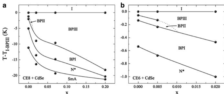
Fig. 12 (a) Reduced temperature T - T_{I-BPIII} vs x_{CdSe} phase diagram for CE8 + CdSe mixtures obtained from cooling runs by a.c. colorimetry. T_{I-BPIII} was found to be a weak function of x . (b) T - T_{I-BPIII} vs x_{CdSe} plot for CE6 + CdSe mixtures obtained from heating runs by adiabatic scanning calorimetry. For clarity the data in both diagrams are plotted vs the T_{I-BPIII} [428]. (Copyright © 2010, The American Physical Society)
