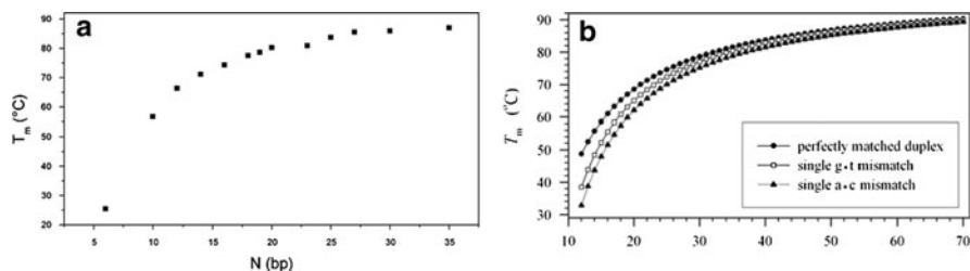
Fig. 4 Dependence of DNA melting temperature T_m on duplex length N . (a) Experimental data from [6], obtained for [\text{Na}^+] = 1\text{ M} . The saturation is already approached for N = 35 . (b) Calculated behavior for the same conditions of (a), based on NN parameters. Reproduced with permission from [8]
