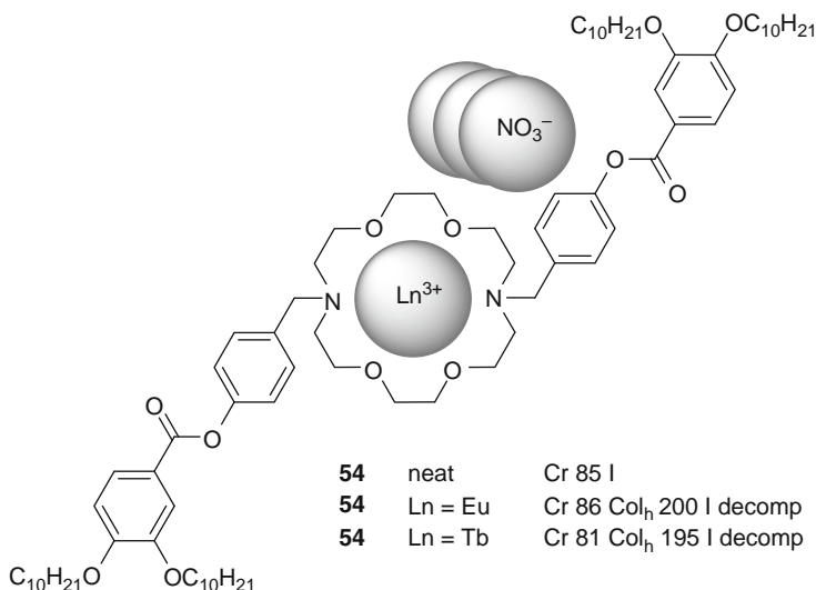
Scheme 30 Complexation of lanthanide salts by 54
