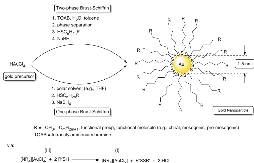
Scheme 1 The one- and two-phase Brust–Schiffrin method for the synthesis of thiol-capped gold nanoparticles, and the first step of the reaction prior to the reduction step with \text{NaBH}_4 [63]
