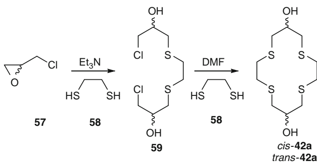
Scheme 31 Synthesis of crown thioether 42a
