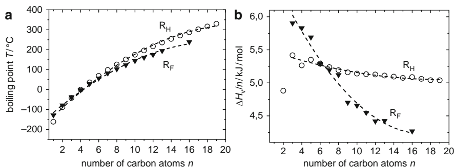
Fig. 4 (a) Boiling points and (b) vaporization enthalpies, normalized to the chain length ( \Delta H_v/n ), for n -alkanes and n -perfluoroalkanes depending on the chain length n , based on values from [75]
