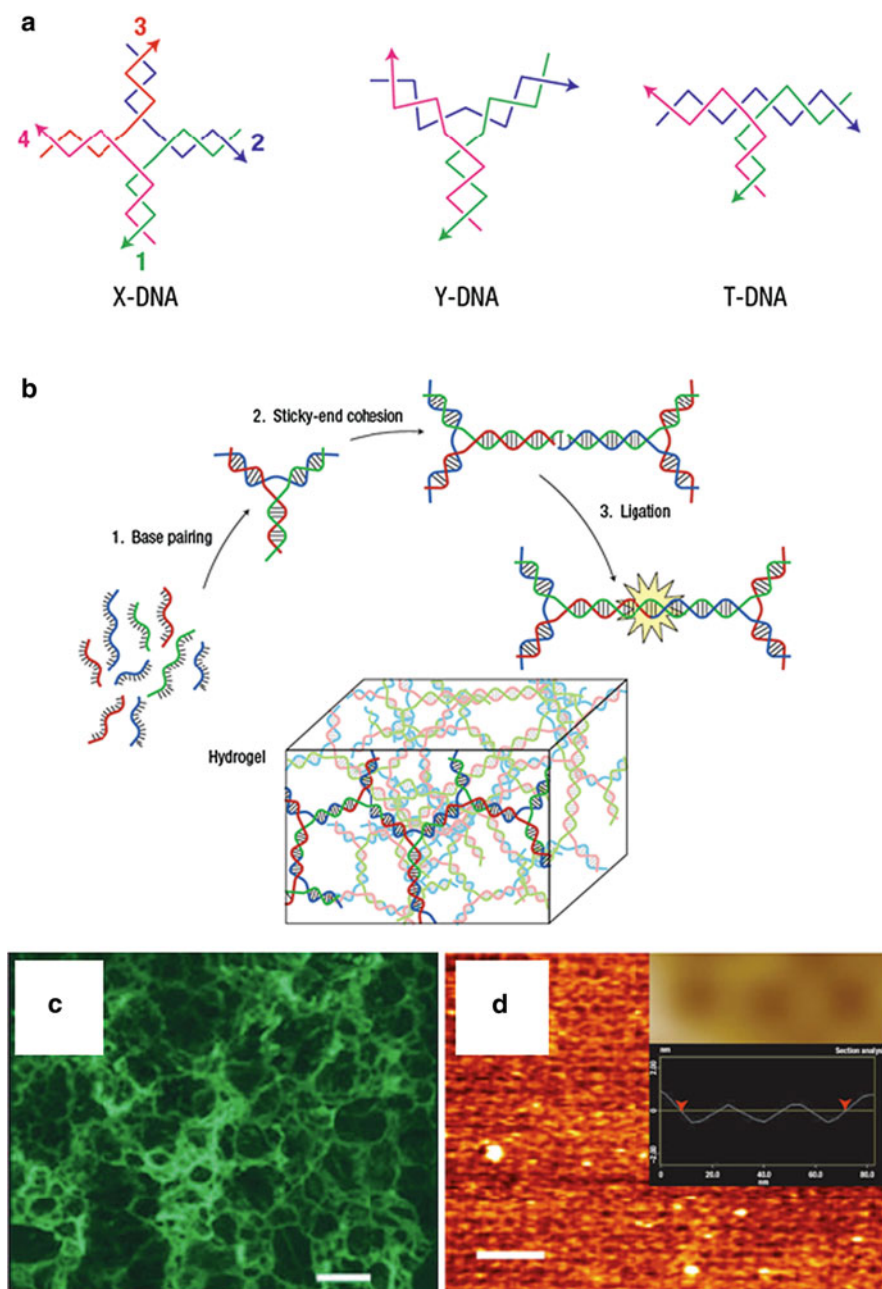
Fig. 28 (a) Various branched DNA structures with sticky ends. (b) Schematic representation of the aggregation of branched monomers and of their ligation into hydrogel networks. (c) Confocal microscopy image of swollen DNA hydrogel obtained from X-DNA structure in (a). Scale bar is 200 \mu\text{m} . (d) AFM image of X-DNA gel (scale bar is 200 nm). The inset shows an enlarged portion of the image with hydrogel pores visible. (a, c, d) reproduced with permission from [123], (b) from [124]
