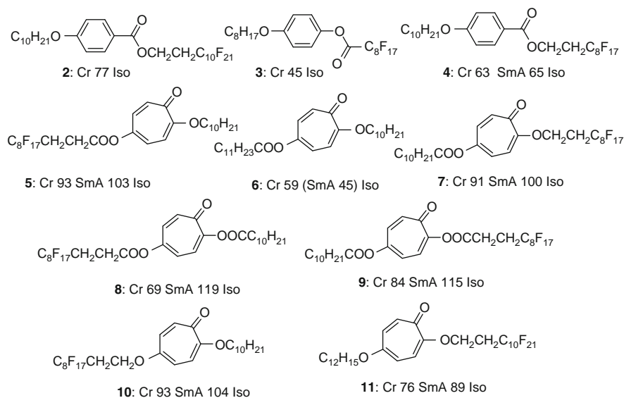
Fig. 8 Examples of mesogenic and potentially mesogenic molecules incorporating only one ring ( T_m /°C) [115, 116]
