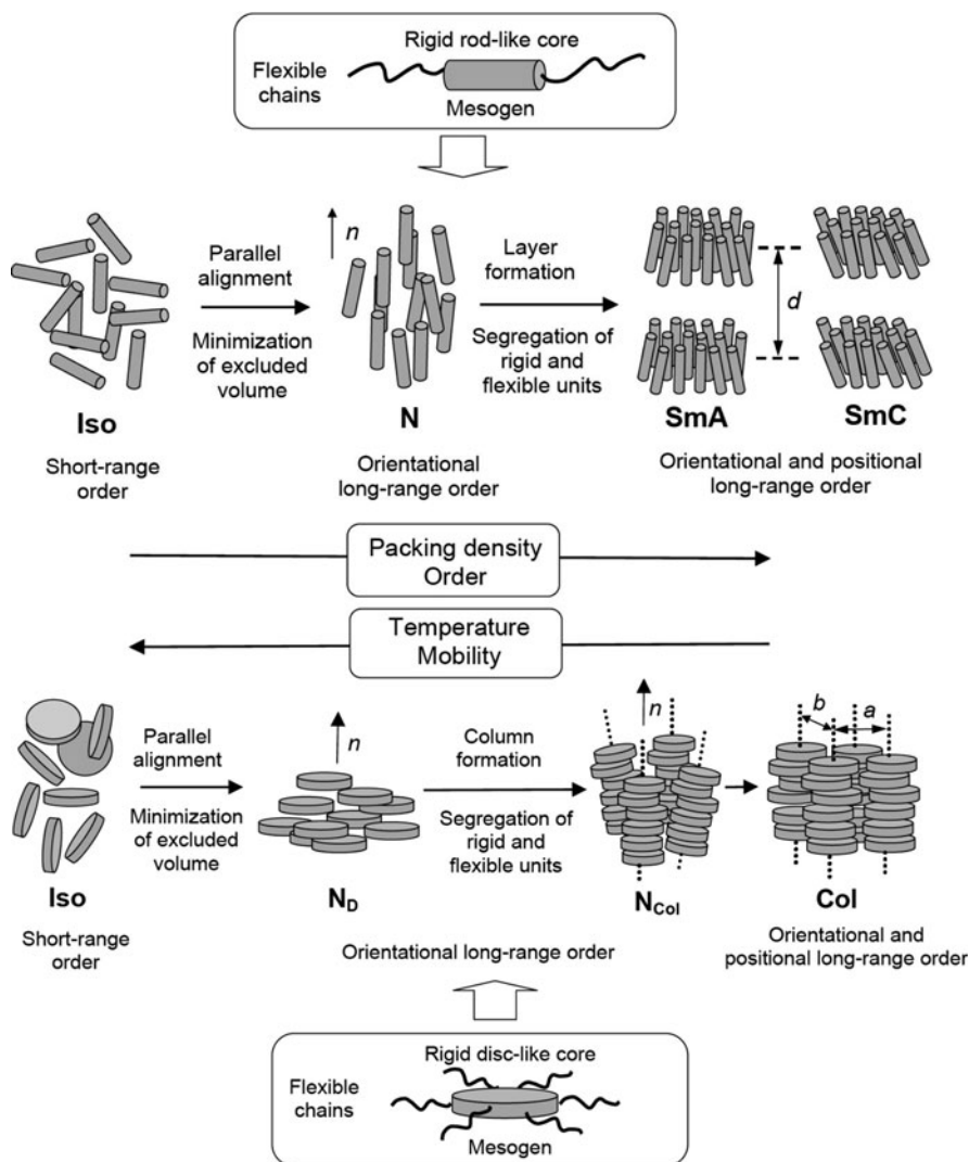
Fig. 1 Organization of rod-like molecules ( top ) and disc-like molecules ( bottom ) in LC phases (for clarity the alkyl chains are not shown in the models of the phase structures). Abbreviations: Iso isotropic liquid state; N nematic LC phase; SmA smectic A phase, SmC smectic C phase (tilted), Col columnar phase [8]
