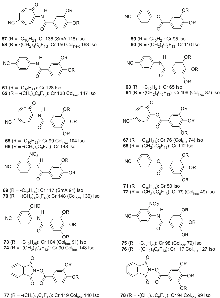
Fig. 18 Examples of short rod-like molecule with two or three semiperfluorinated chains ( T^\circ\text{C} ). [121, 152]
