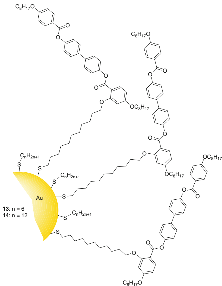
Fig. 19 Gold nanoparticles 13 and 14 capped with a mixed monolayer of hexanethiol ( 13 ) or dedecanethiol ( 14 ) and a lateral substituted nematic liquid crystal thiol attached in a side-on fashion (thiol ratio: \sim 1:1 ) [540, 541]
