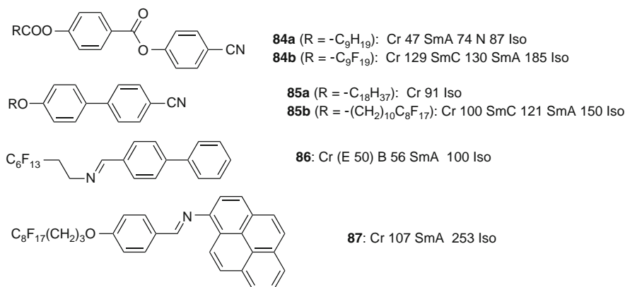
Fig. 23 Selected examples of rod-like molecules with one linear semiperfluorinated chain ( T^\circ C) [163–165]
