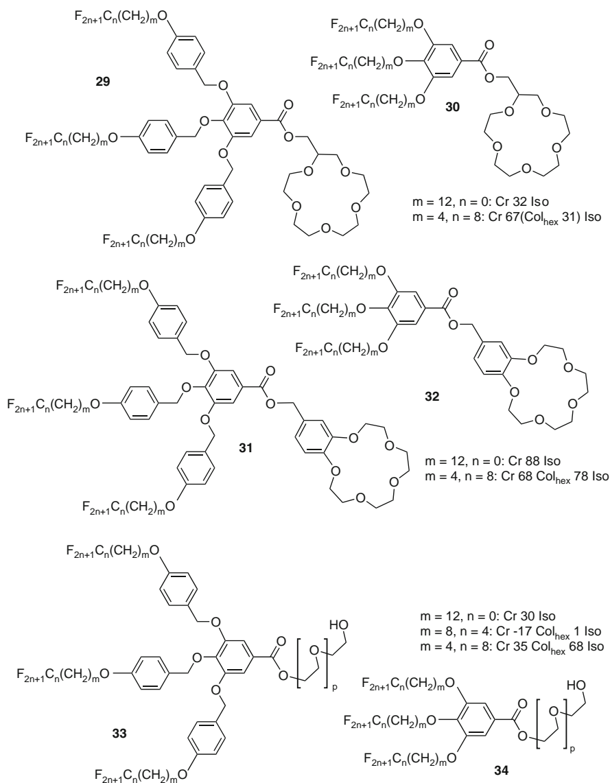
Fig. 12 Selected examples of taper shaped crown ethers and polyethers with three fluorinated chains ( T^{\circ}C ); data refer to compounds 30 , 32 and 34 [132–135]
