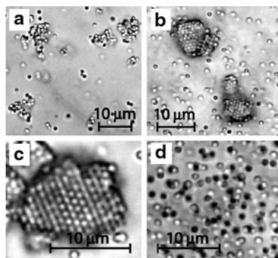
Fig. 36 Self-assembly of DNA-coated colloids observed in optical microscopy. (a) Fractal-like aggregates of microspheres with 14,000 DNA molecules per each sphere. (b, c) Similar colloids with 3,700 DNA/sphere form small crystals. (d) Upon heating by only 2°C, the crystallites and the aggregates both melt into monomers. Adapted with permission from [153]
