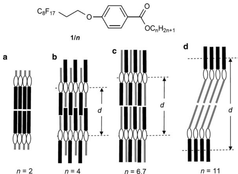
Fig. 7 Compounds 1/n and schematics of their fundamental organization in distinct crystal structures depending on alkyl chain length; R_F = black, R_H = gray, additionally, there is the possibility of tilting which is not considered in all cases [94]
