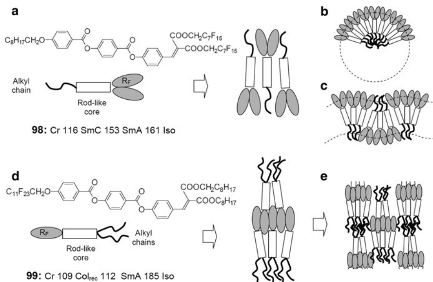
Fig. 28 (a,d) Influence of the position of the fluorinated chain(s) and the hydrocarbon chain(s) on the packing behavior of the tricatena compounds 98 and 99 ( T^\circ\text{C} ) and (b,c,e) different possible packing modes [194]
