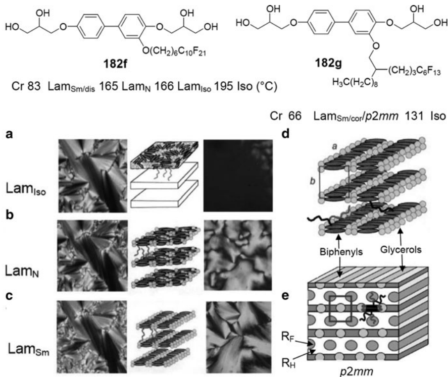
Fig. 57 Lam-phases (a–c) as formed by compound 182f with a linear lateral R_F -chain and (d,e) Lam_{Sm/cor}/p2mm phase as formed by compound 182g with a branched lateral chain: (a) Lam_{iso} phase = lamellar phase without order in the layers; (b–d) in these Lam-phases the rod-like aromatic cores are organized on average parallel to the layer planes; (b) Lam_N (lamellar nematic phase) = lamellar phase with only orientational order in the layers and between layers; (c) Lam_{Sm/dis} (lamellar smectic phase) = lamellar phase with orientational and positional order in the layers and only orientational order between the layers, a sliding of the layers with respect to each other is possible; (d,e) in the correlated Lam_{Sm/cor} phase there is also positional order between the layers and a p2mm -lattice is formed [8, 316, 317, 320–322]. (a–c) Reproduced with permission [321], copyright 2002, American Chemical Society (ACS)
