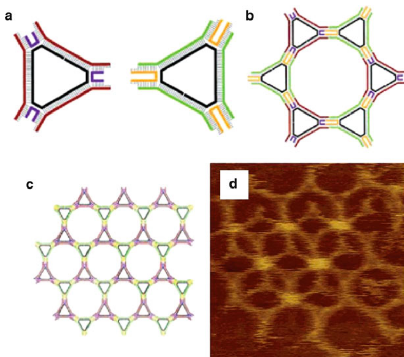
Fig. 14 Interacting triangular tiles. (a) Sequences are designed so to assemble in two different triangular tiles with complementary sticky ends. (b) Six connected triangles form hexagonal units, which (c) create a two-dimensional crystal. (d) AFM image (edge size is 133 nm) of two overlapped hexagonal tilings. Adapted with permission from [69]
