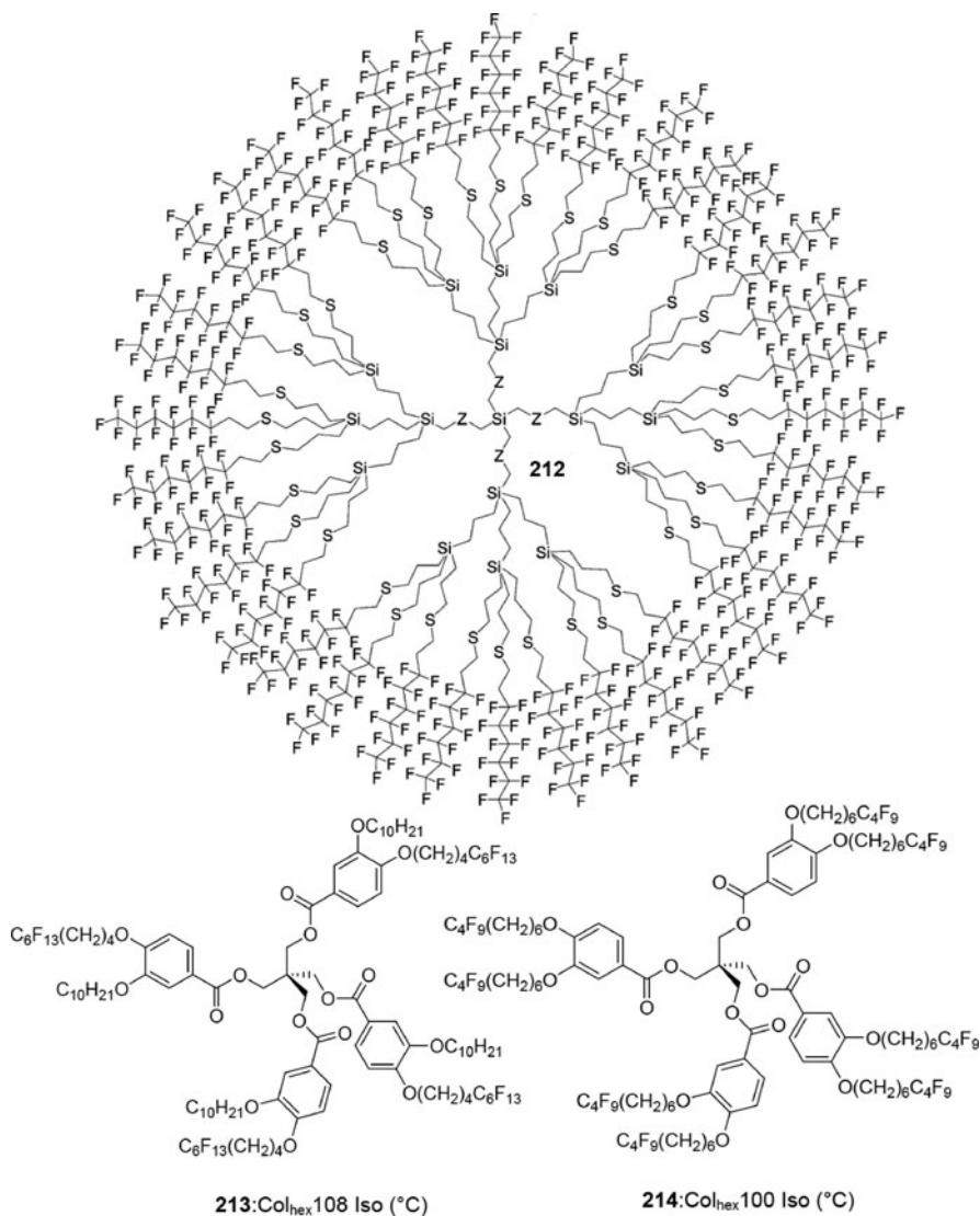
Fig. 70 Carbosilane based dendrimer ( 212 , Z = \text{CH}_2 ) and pentaerythritol tetrabenzoates 213 and 214 with \text{R}_\text{F} -chains at the periphery [138, 141, 373]
