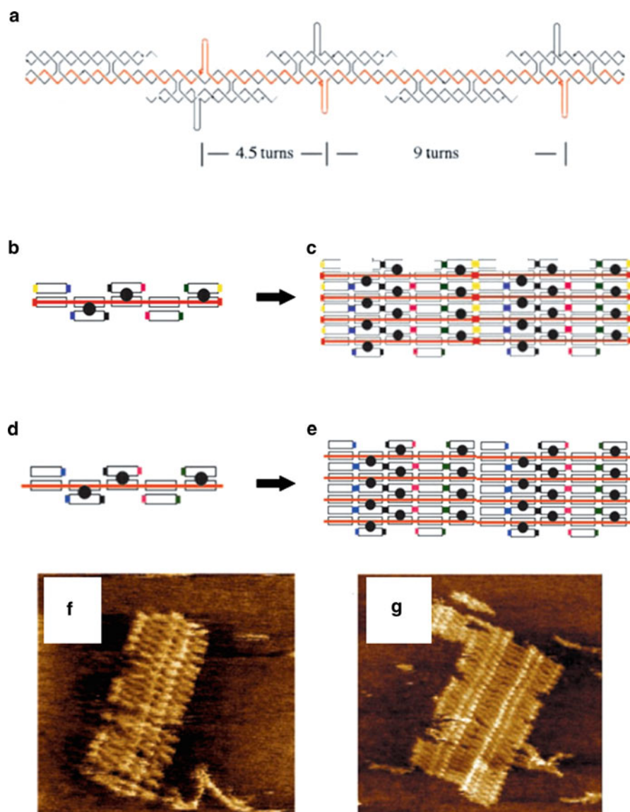
Fig. 19 (a) Tile structure proposed in [79], with a scaffold sequence (red) connected to shorter satellite strands through WC pairing and DX, with or without protruding hairpins. (b, d) Schematic illustration of the tile in (a), with black dots representing hairpins and colored caps representing sticky ends. The tiles form layers through sticky end pairing and can aggregate end-to-end, either through sticky ends (c) or blunt-end stacking (e). (f, g) AFM images corresponding respectively to (c) and (e). Image size is 250 nm (f) and 400 nm (g). Adapted with permission from [79]
