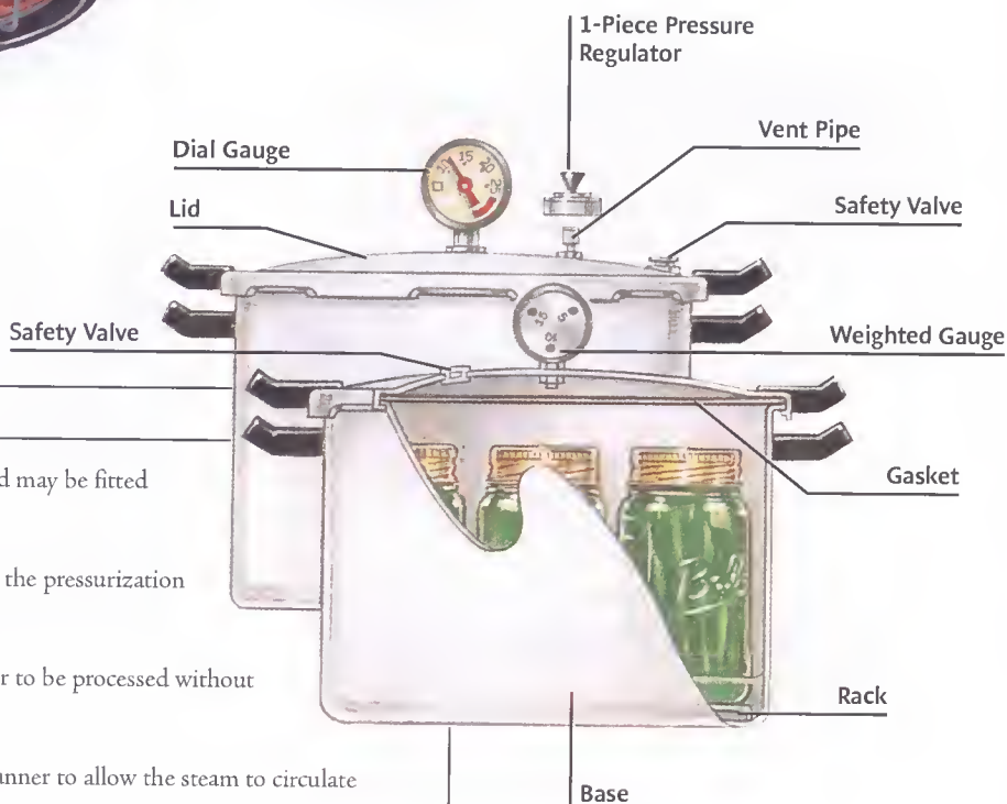
figure 5 | Steam-Pressure Canner Features
