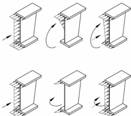
Figure 6.3.7 Stress Distribution
