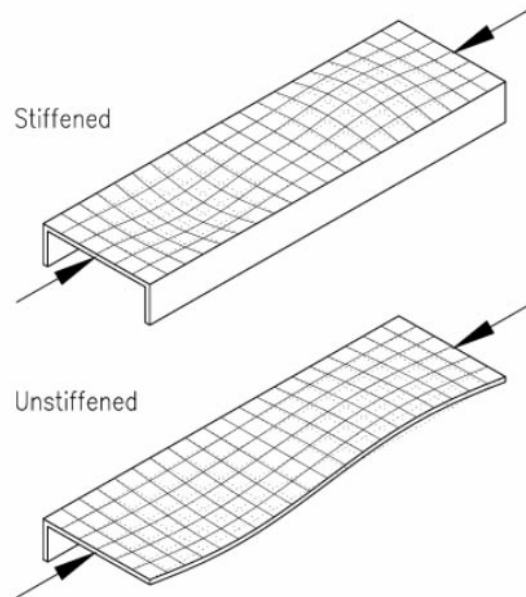
Figure 6.3.4 Buckled Unstiffened Element
