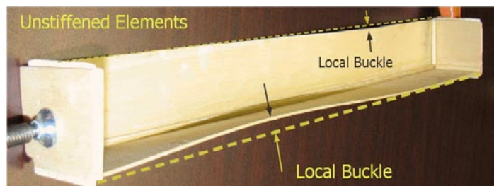
Figure 6.3.4 Buckled Unstiffened Element
