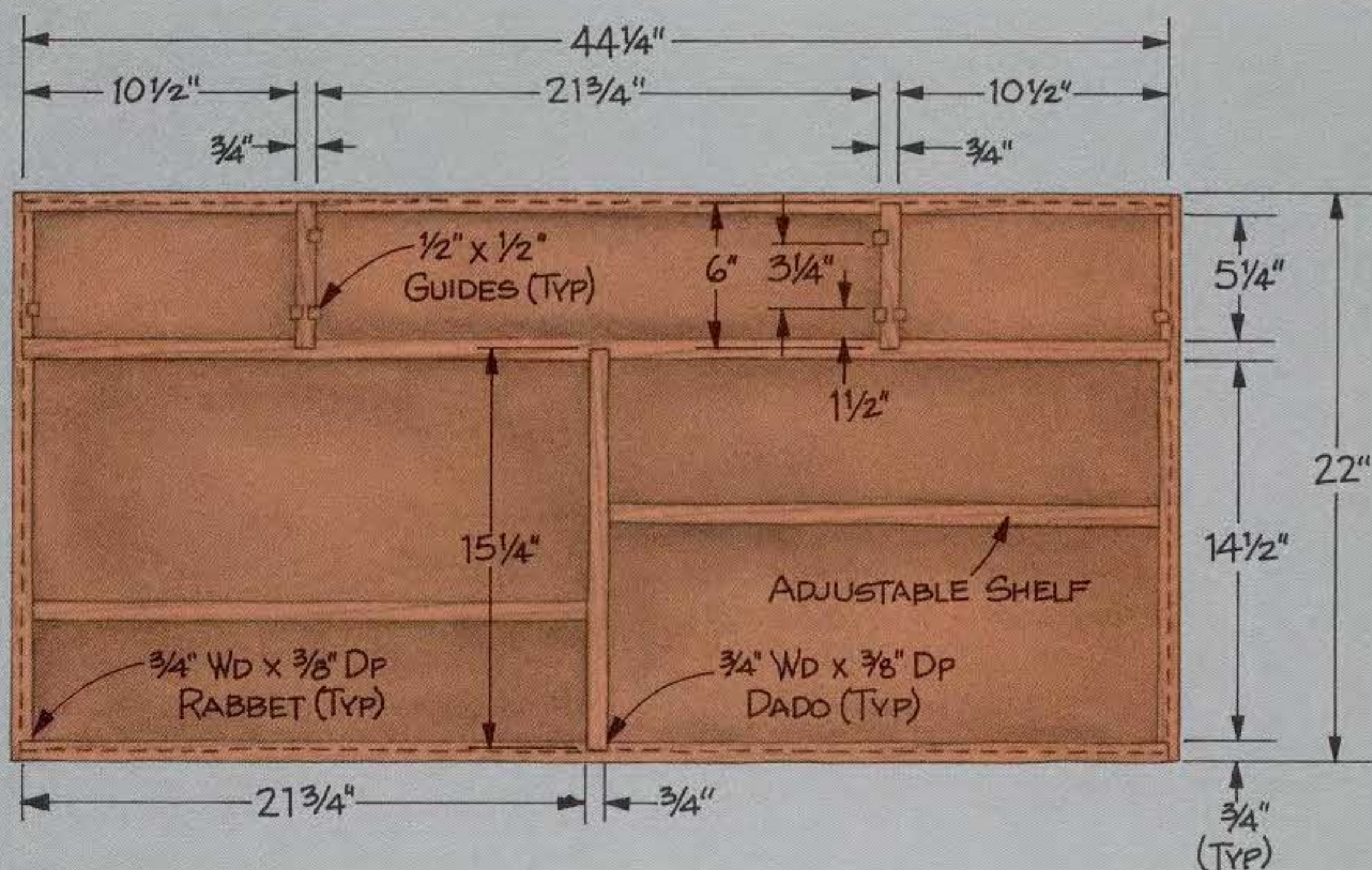
CASE LAYOUT
