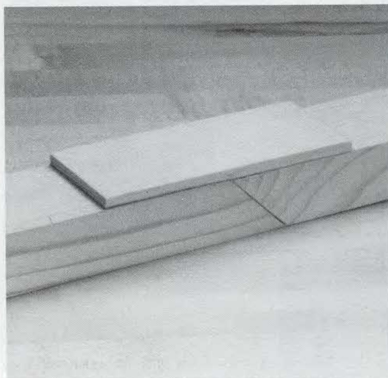
4-1 Because scarf joints are glued end grain to end grain, they are inherently weak. This one has been reinforced with a rectangular glue block that straddles the joint. Note that the grain of the glue block is parallel to that of the adjoining members, and runs across the joint.
