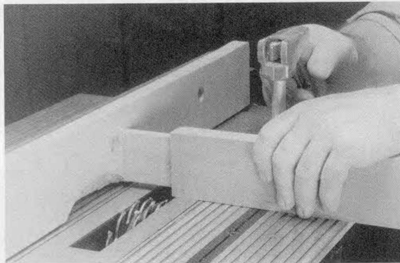
5-16 You can also use a miter gauge to guide the workpiece when cutting a tenon with a dado cutter. This setup allows you to make much longer tenons, since you aren't limited by the diameter of the cutter. It's also easier to cut shoulders and cheeks on all four sides of a tenon. The disadvantage is that you usually must make several passes to cut each tenon side.
