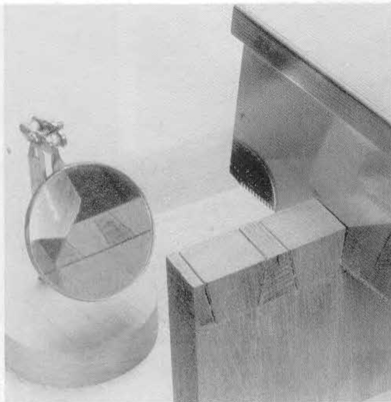
6-13 As you cut the cheeks, you must monitor both sides of the board, making sure the saw follows both sets of layout lines. You can do this with a great deal of head bobbing, or you can use the Third Eye (see page 31) to keep watch on the side of the board facing away from you.
