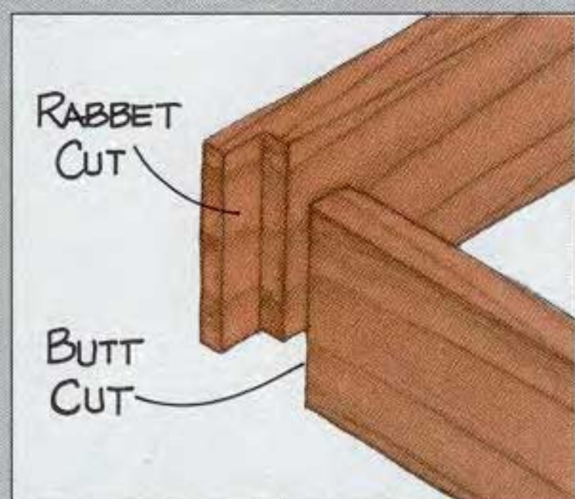
RABBET JOINT
