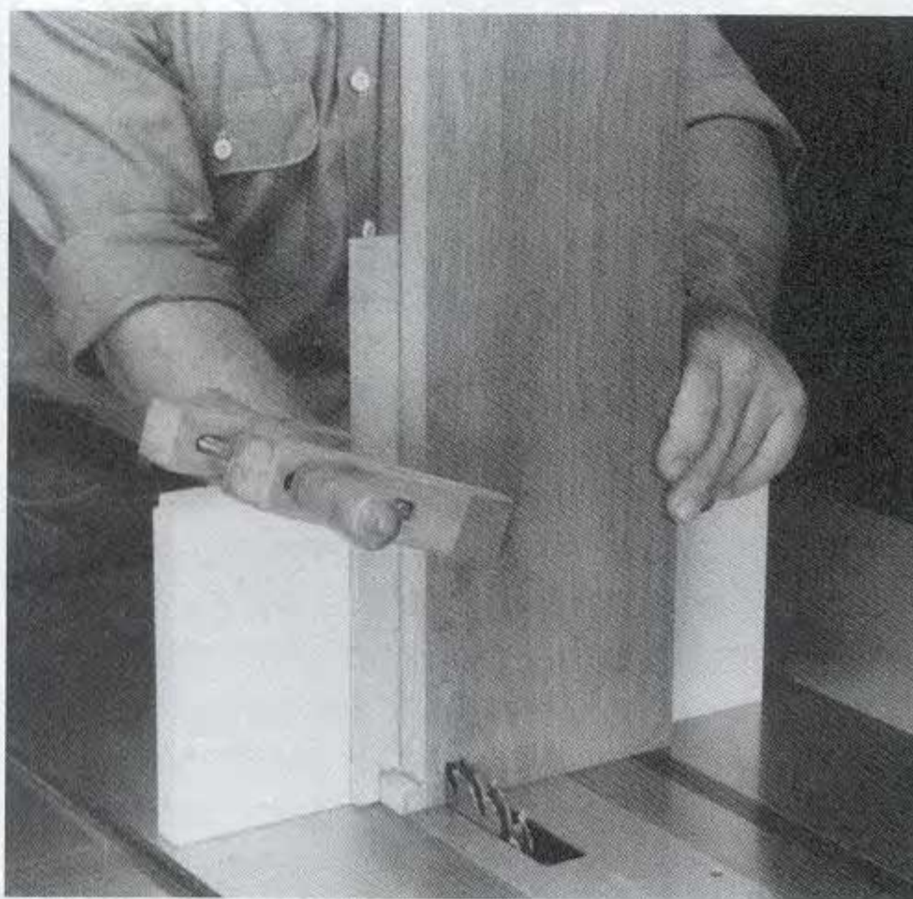
6-3 Place the first adjoining board end down against the face of the jig and slide it to one side until the edge butts against the stop. Clamp the board to the jig to prevent it from moving. Turn the saw on and slide the board forward, cutting the first notch. Note: To prevent tear-out, always back up the board with a scrap.
