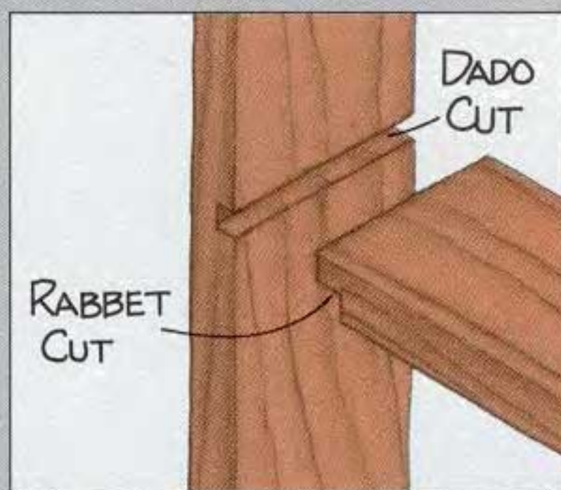
DADO-AND-RABBET JOINT
