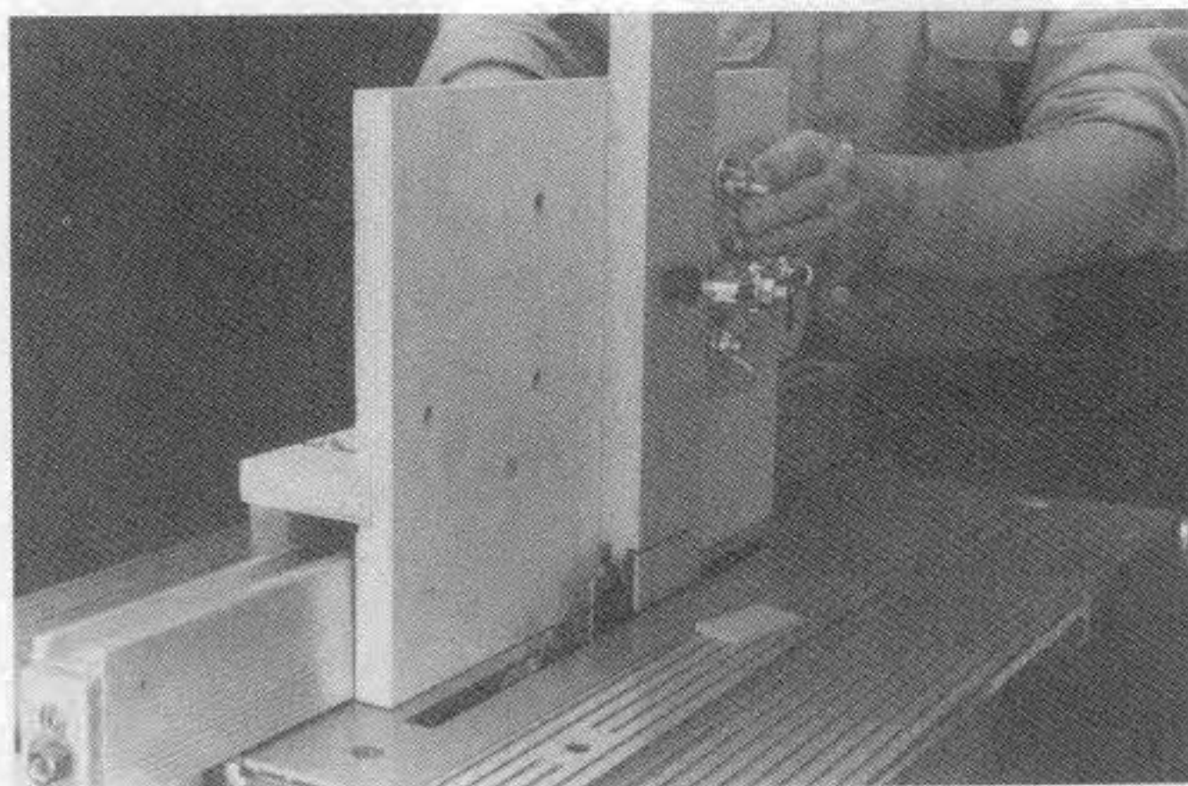
5-14 Next, cut the cheeks, using a tenoning jig to hold the stock as you slide the jig along the fence. Test fit the tenon in its mortise. If it's too tight , move the fence closer to the blade — this will shave a little more stock from the tenon. If it's too loose , move the fence farther away — this will make the tenon thicker.
