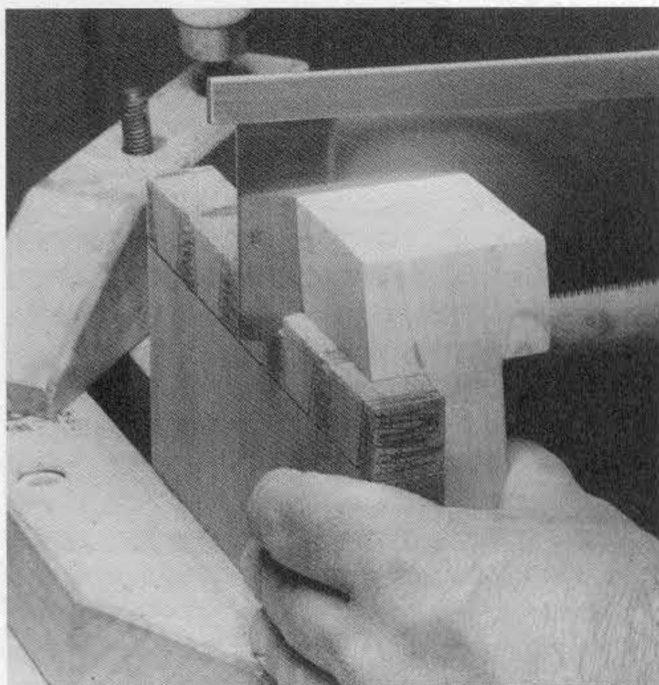
6-12 Using a dovetail saw or a dozuki saw, cut the sloping cheeks down to the baseline. If you wish, use the Slope Gauge as shown to help start the cut. You can also use the Chisel Guide (see page 90) to hold the board as you cut it.
