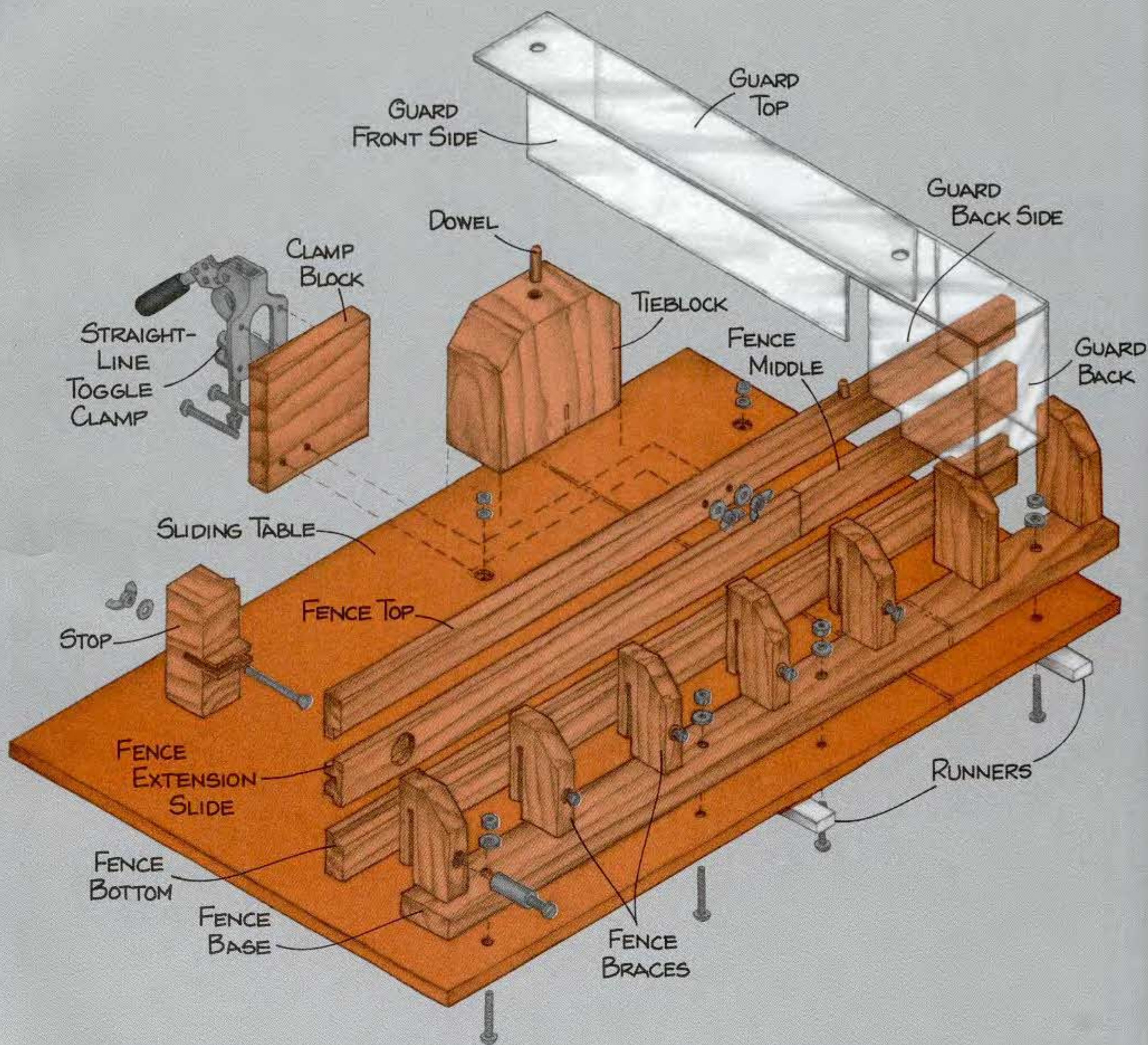
EXPLODED VIEW
