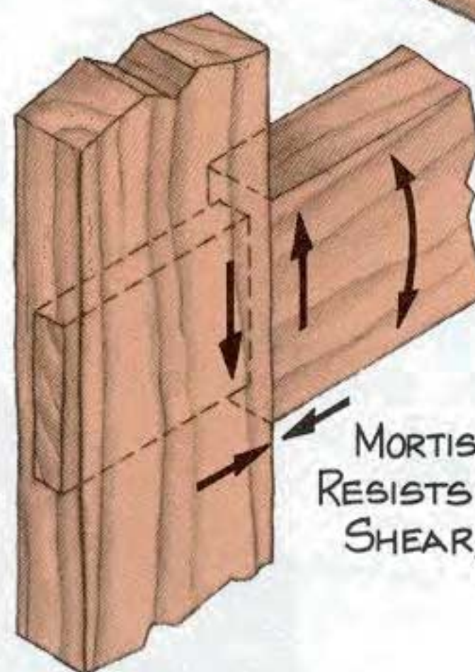
1-4 Even before a butt joint is glued or fastened, it will withstand compression, but any amount of tension, shear, or racking will pull it apart. A mortise-and-tenon joint, on the other hand, will resist compression, shear, and racking. Only tension can pull it apart before it's secured.
