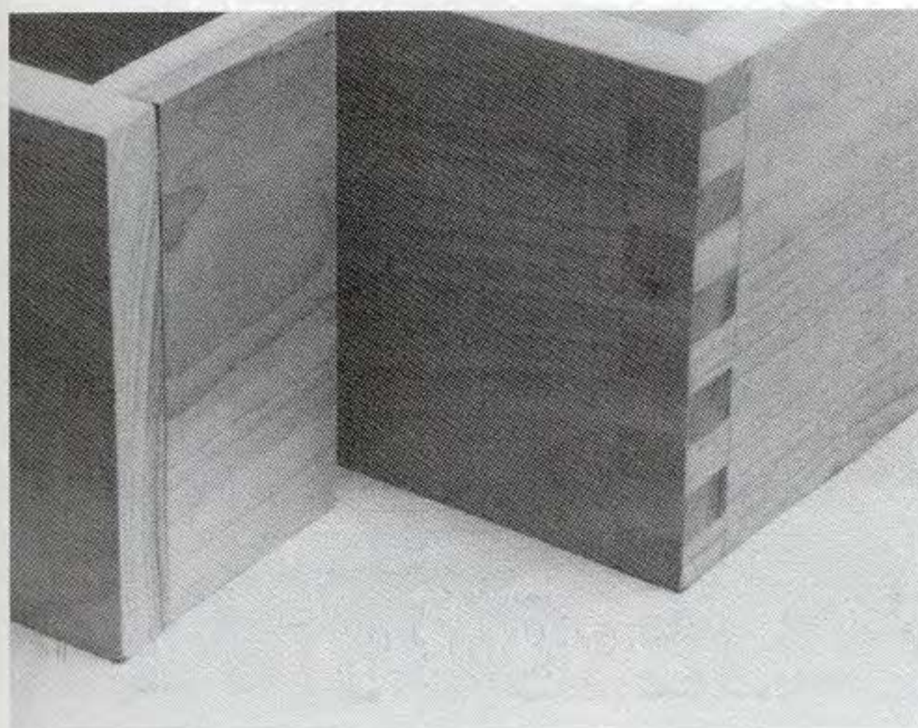
1-8 The adjoining members of both the butt joint (left) and the box joint (right) are precisely the same size. However, the fitted fingers of the box joint offer more gluing surface than the flat surfaces of the butt joint. Consequently, the box joint is much stronger.
