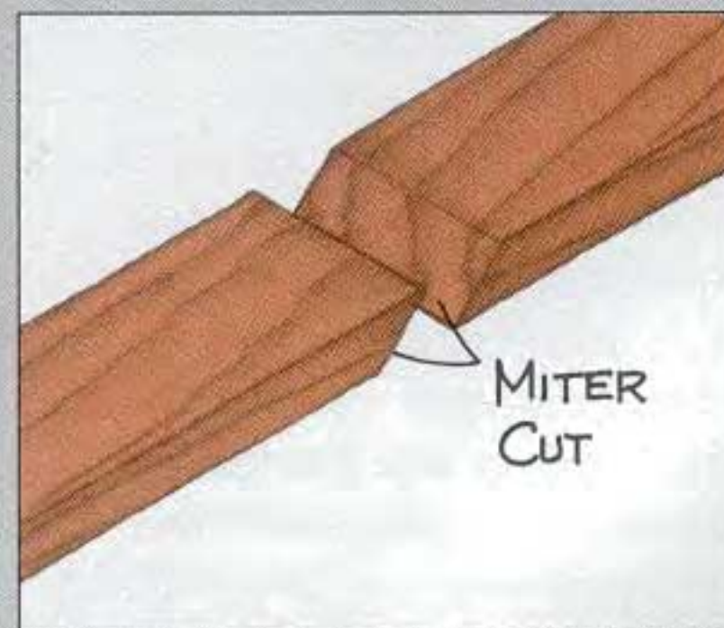
SCARF JOINT
