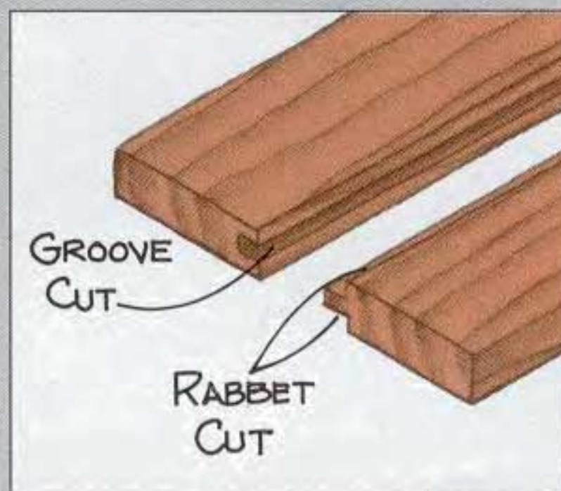
TONGUE-AND-GROOVE JOINT
