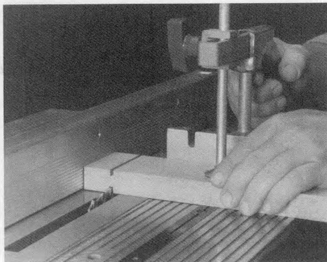
5-13 To cut a tenon with an ordinary table saw blade, first cut the shoulders. Guide the stock with a miter gauge. If you wish, use the fence to position the stock on the gauge.
