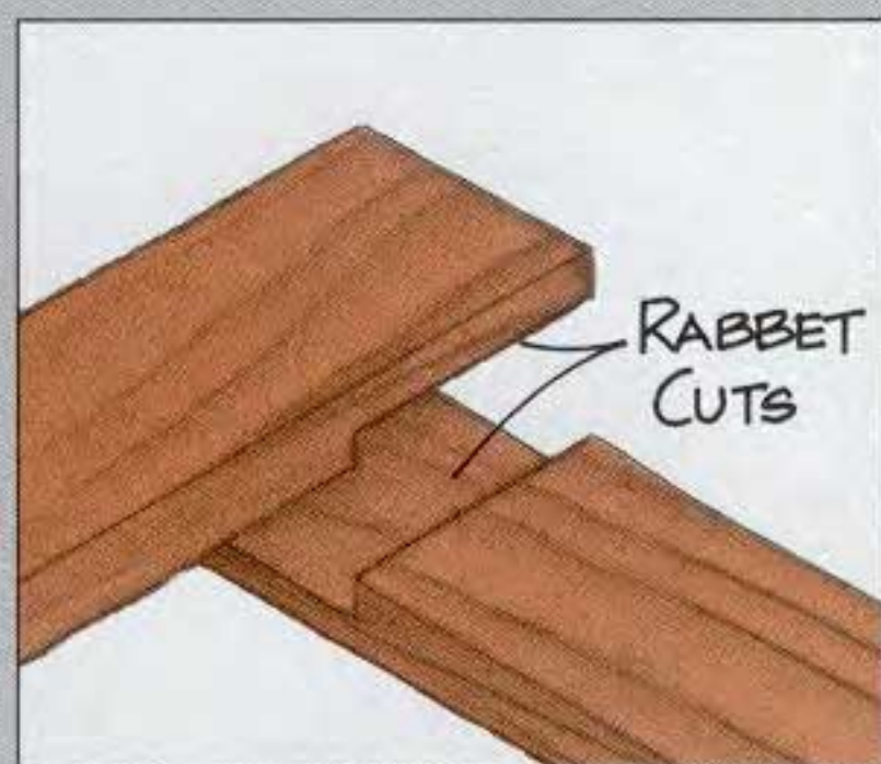
LAP JOINT
