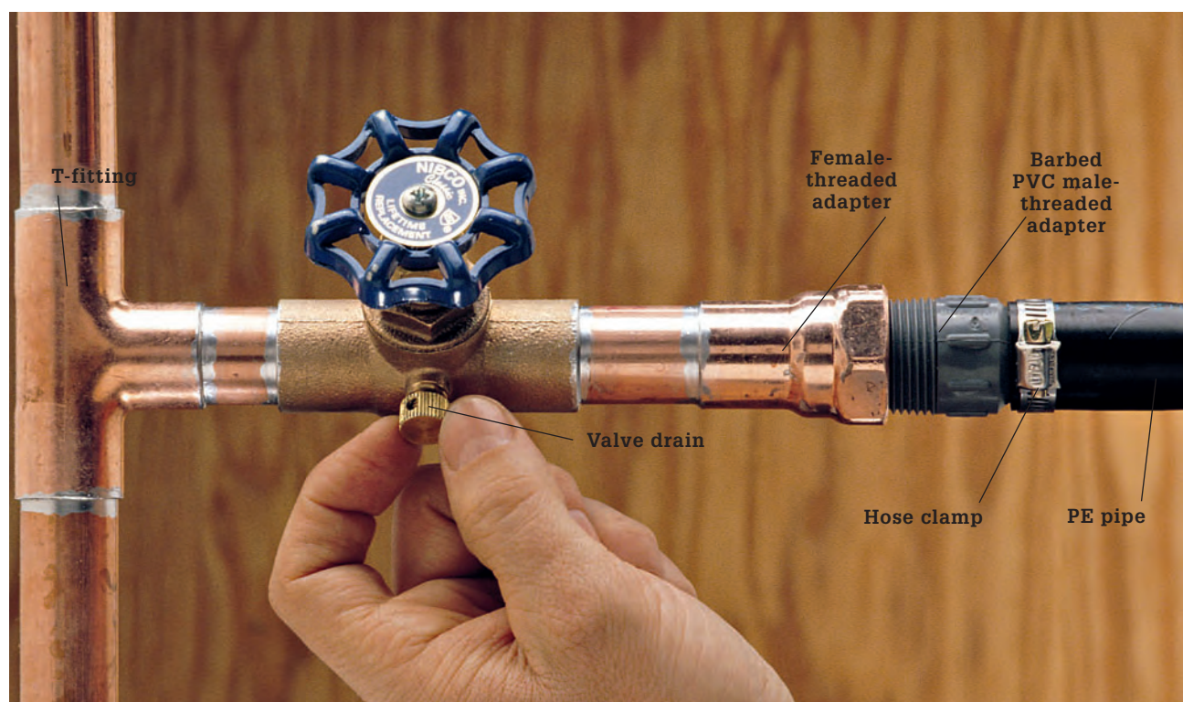
Connect lengths of PE pipe with a barbed PVC fitting. Secure the connection with stainless steel hose clamps.
