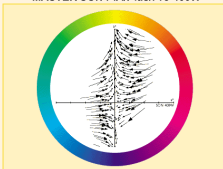
MASTER SON PIA/Plus/Pro 400W
