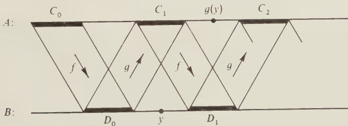
Fig. 39. The Schröder-Bernstein theorem.
