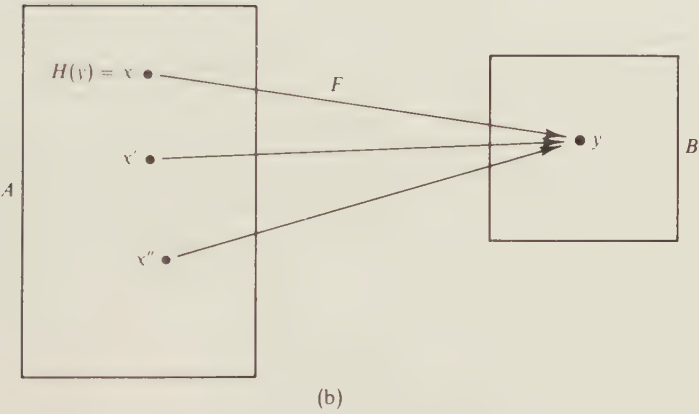
Fig. 10. The proof of Theorem 3J. In part (a), make G(x) = a for x \in B - \text{ran } F . In part (b), H(y) is the chosen x for which F(x) = y .
