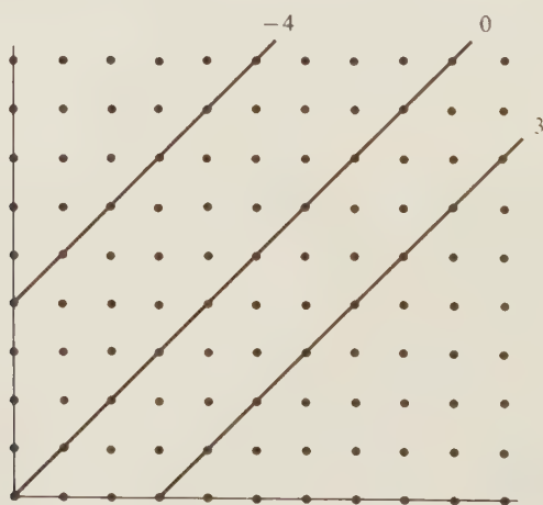
Fig. 20. An integer is a line in \omega \times \omega .
