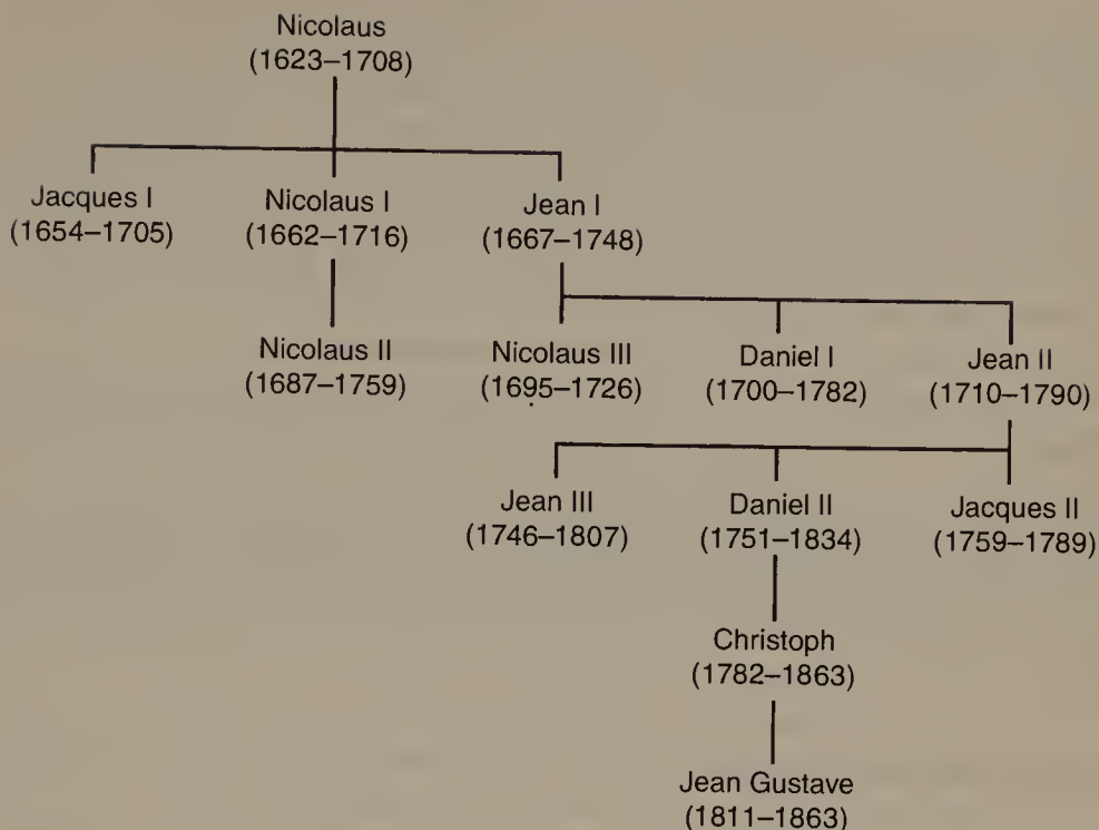
The mathematical Bernoullis: a genealogical chart
