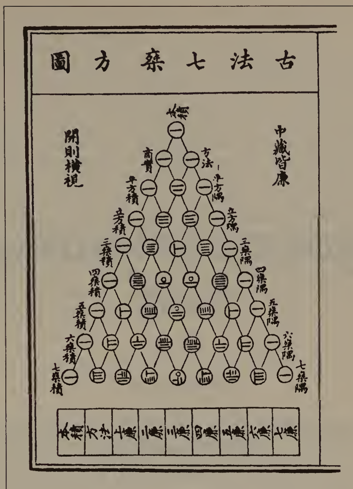
The “Pascal” triangle, as depicted in 1303 at the front of Zhu Shijie’s Jade Mirror . It is titled “The Old Method Chart of the Seven Multiplying Squares” and tabulates the binomial coefficients up to the eighth power. (Reproduced from J. Needham 1959, Vol. 3, p. 135.)
