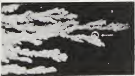
FIGURE 4.15: Linear displacement of oil by water at oil-water viscosity ratio 80 in a three-dimensional porous medium. Q —total volume injected, R —‘recovery’ volume, expressed as percentages of total pore volume (van Meurs, 1957; van Meurs and van der Poel, 1958).
