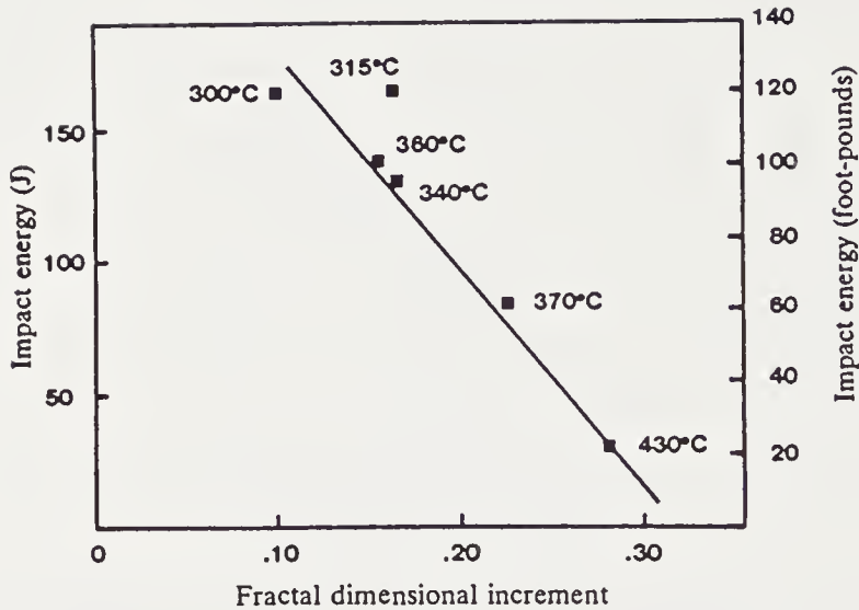
FIGURE 14.4: The relation between the observed surface fractal dimension D and the impact energy required to fracture a series of 300-Grade Maraging steel samples heat-treated at various temperatures (Mandelbrot et al., 1984).
