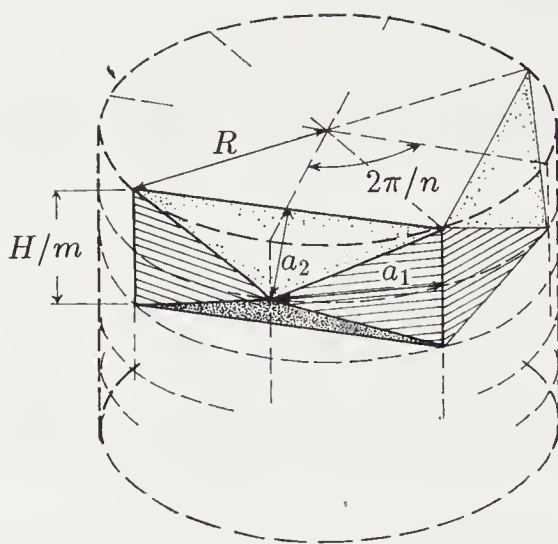
FIGURE 2.4: The vertical surface of a cylinder of radius R and height H is 2\pi RH . The surface is approximated by a triangulation as illustrated.
