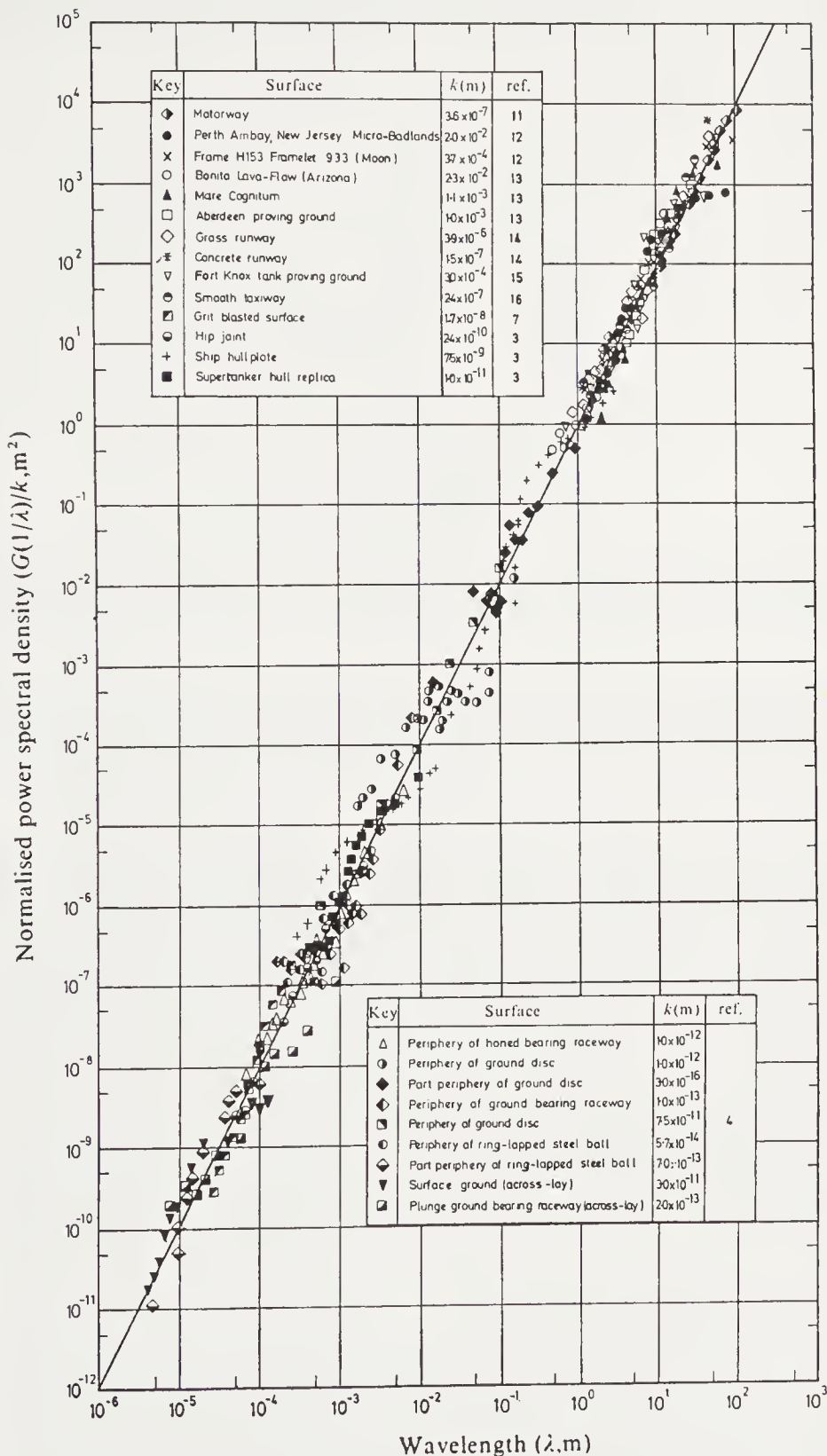
FIGURE 14.1: Scaled surface spectral power \frac{1}{k}G(1/\lambda) versus surface height wavelength \lambda for different systems (Sayles and Thomas, 1978a).
