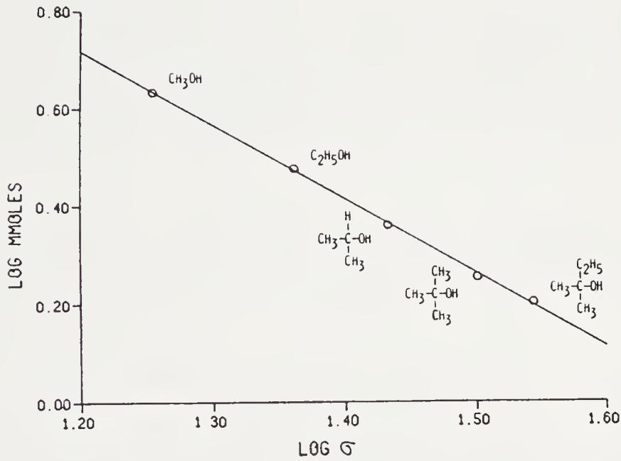
FIGURE 14.6: Measured monolayer mole numbers n on porous silica gel as a function of molecule cross-section \sigma ( \text{\AA}^2 ). D = 3.02 \pm 0.06 (Pfeifer et al., 1984).
