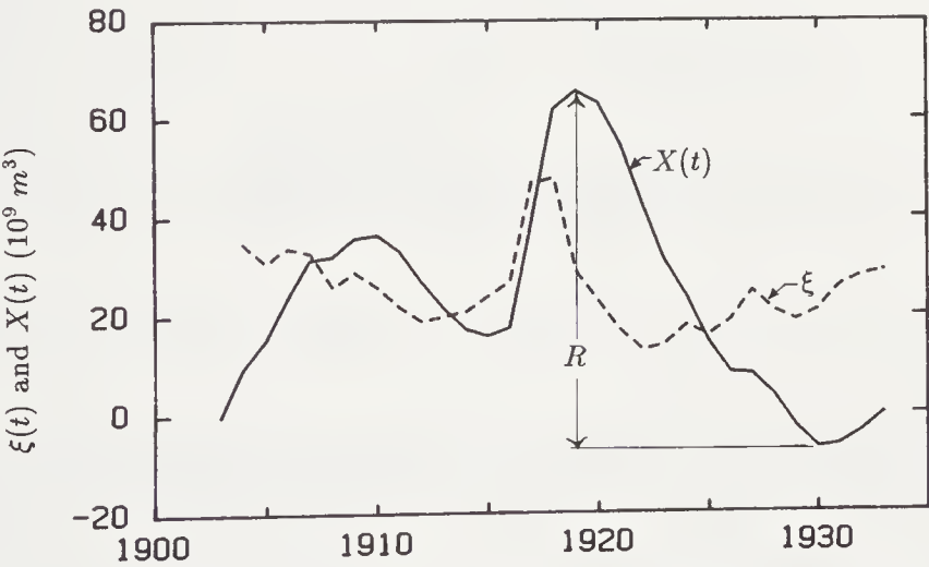
FIGURE 8.3: Lake Albert accumulated departures from the mean discharge X(t) for the first 30 years. The range is indicated by R (after Hurst et al., 1965).
