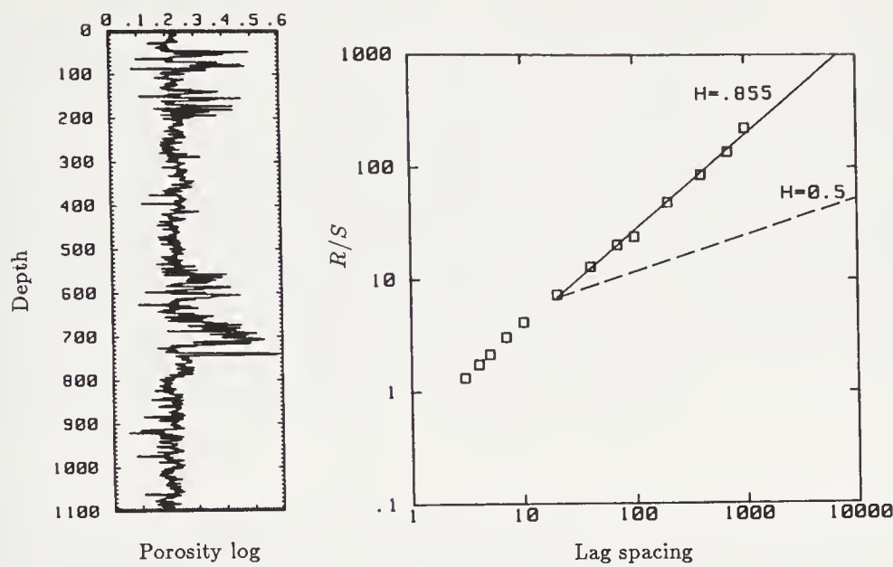
FIGURE 8.11: Porosity as a function of depth (feet) measured using a well log (left figure). R/S as a function of lag for the porosity data (right figure). The trend line is a fit with H = 0.855 . The broken line is the slope for a statistically independent process (Hewett, 1986).
