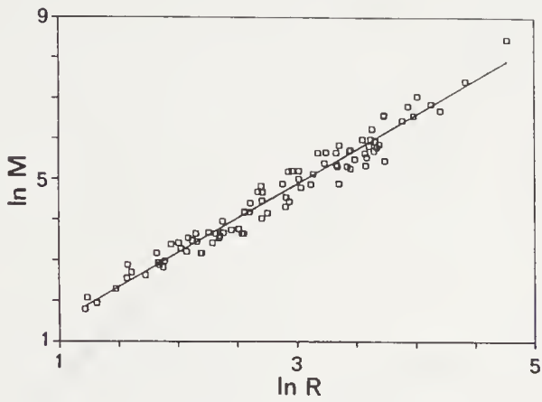
FIGURE 3.7: Variation of the mass as a function of size for gold colloid aggregates. The mass is in units of a single particle mass and the size is scaled by units of the particle diameter. The line corresponds to a fractal dimension D = 1.7 \pm 0.1 (Weitz and Huang, 1984).
