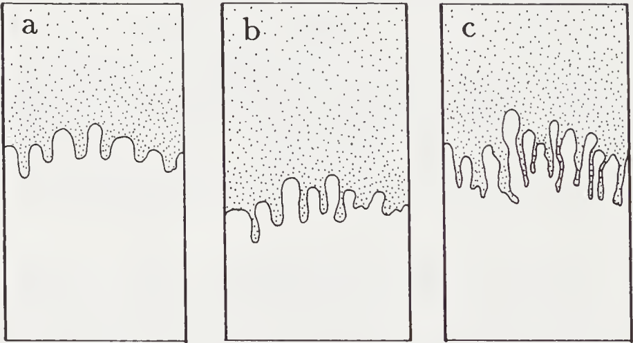
FIGURE 4.4: Water-glycerol solution (dark), \mu_1 = 0.552 poise, \rho_1 = 1.21 g/cm 3 , displacing oil, \mu_2 = 1.39 poise, \rho_2 = 0.877 g/cm 3 . The system is tilted an angle of 44^\circ 25' . The bulk interfacial tension is \sigma = 33 dyne/cm, and the oil wets the walls. The critical velocity is U_c = 0.23 cm/s. (a) U = 0.41 cm/s, \lambda_m = 3.5 cm, observed \lambda = 3.5 cm. (b) U = 0.87 cm/s, \lambda_m = 2.6 cm, observed \lambda = 2.4 cm. (c) U = 1.66 cm/s, \lambda_m = 1.6 cm, observed \lambda = 1.7 cm (Chuoque et al., 1959).
