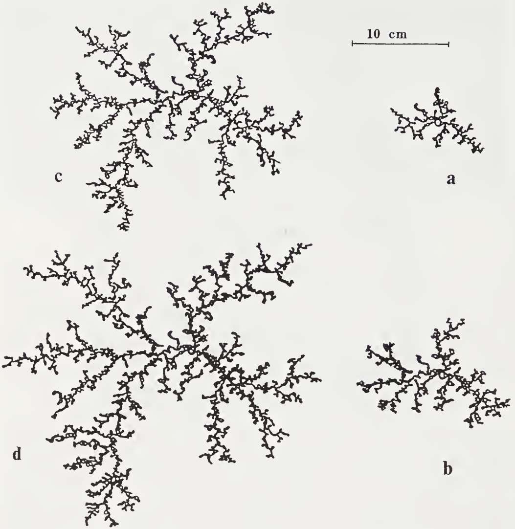
FIGURE 4.7: Fingers of air (black) displacing liquid epoxy in a two-dimensional porous medium consisting of 1.6-mm glass spheres in a monolayer between two glass plates 40 cm in diameter. The center of injection is near the center of the structure. (a) t = 2 s after the start of injection. (b) t = 3.9 s. (c) t = 17.2 s. (d) t = 19.1 s. The capillary number is Ca = 0.04 (Måløy et al., 1985a,b).
