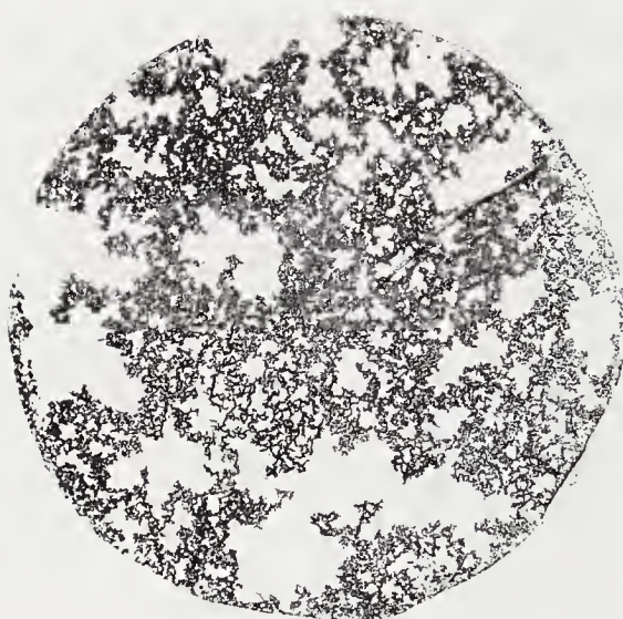
FIGURE 7.21: Air (black) displacing glycerol (white) at very low capillary numbers Ca \simeq 10^{-5} , in a two-dimensional model consisting of a layer of randomly packed glass spheres 1 mm in diameter. The fractal dimension of the cluster of invading of air is D \simeq 1.84 (Måløy et al., 1987b).
