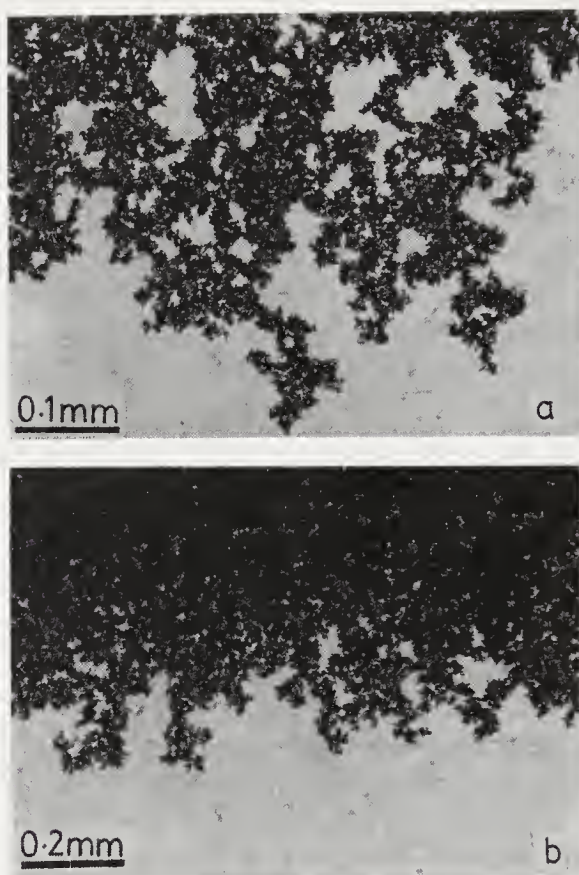
FIGURE 7.25: The drying front in a thin layer of silica spheres. Drained porosity appears dark in the transmitted light image. (a) Portion of the drying front. (b) In the lower-magnification image it is evident that the front is stable (Shaw, 1987).
