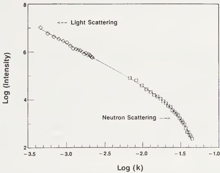
FIGURE 3.8: Light scattering and small-angle neutron scattering from gold colloid clusters, formed by diffusion-limited aggregation, plotted as a function of the scattering wave vector k = \frac{4\pi}{\lambda} \sin \theta (in units of \text{\AA}^{-1} ). The line represents the theoretical fit corresponding to D \simeq 1.79 (Weitz et al., 1985).
