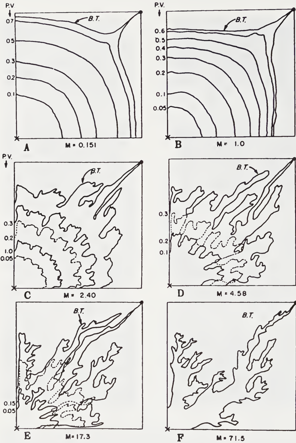
FIGURE 4.16: Displacement fronts for different mobility ratios, M , and injected pore volumes, P.V. , until breakthrough, B.T. (Habermann, 1960).
