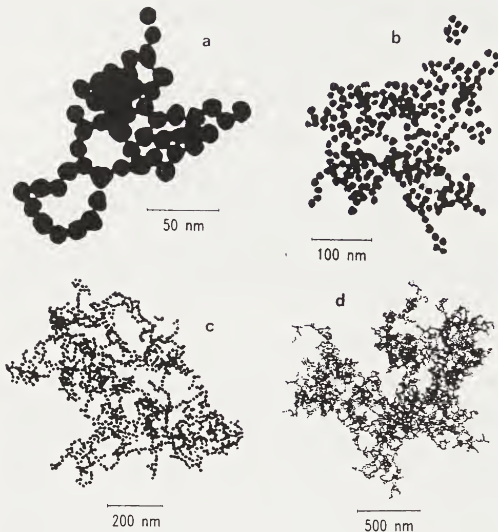
FIGURE 3.6: Transmission electron micrographs of gold clusters of different sizes (Weitz and Huang, 1984).
