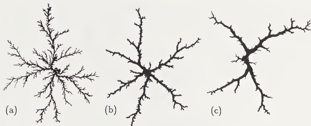
FIGURE 4.10: Photographs of two-dimensional patterns resulting from chemical dissolution of porous plaster by the radial flow of water at different injection rates: (a) 48 \text{ cm}^3/\text{h} ; (b) 4 \text{ cm}^3/\text{h} ; (c) 2 \text{ cm}^3/\text{h} (Daccord, 1987).
