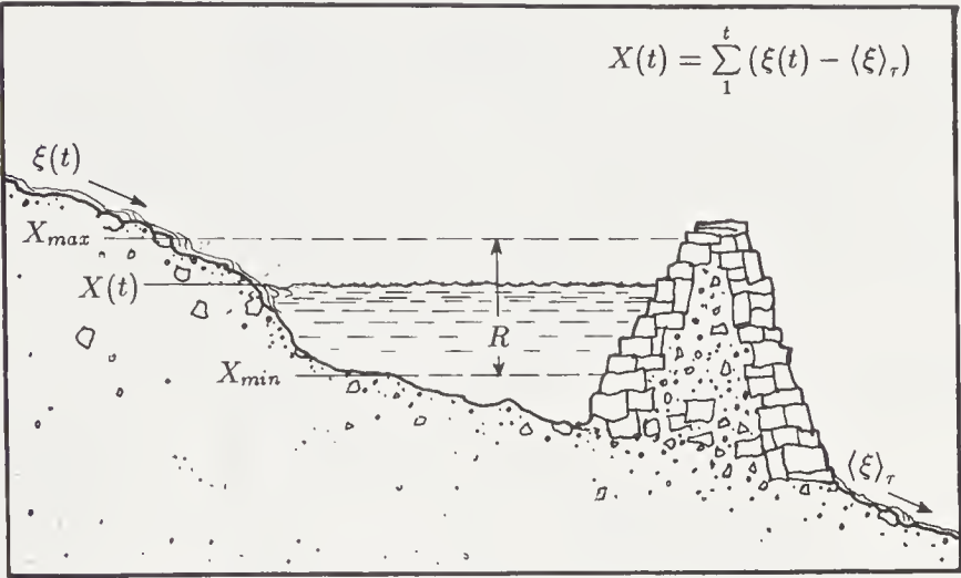
FIGURE 8.2: Sketch of a reservoir with an influx of \xi(t) , and an average discharge \langle \xi \rangle_\tau . The accumulated difference between influx and regulated outflow is X(t) . The range, R , is the difference between the maximum and minimum contents of the reservoir.
