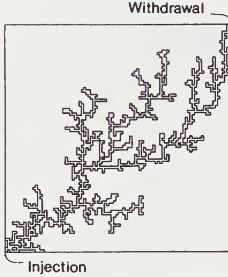
FIGURE 4.11: Simulation of the displacement front at breakthrough for one quarter of a five-spot well pattern. The driving fluid has infinite mobility (Paterson, 1984).
