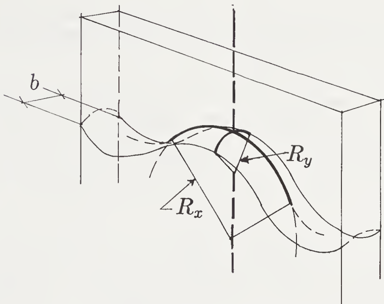
FIGURE 4.2: Geometry of the fluid–fluid interface.
