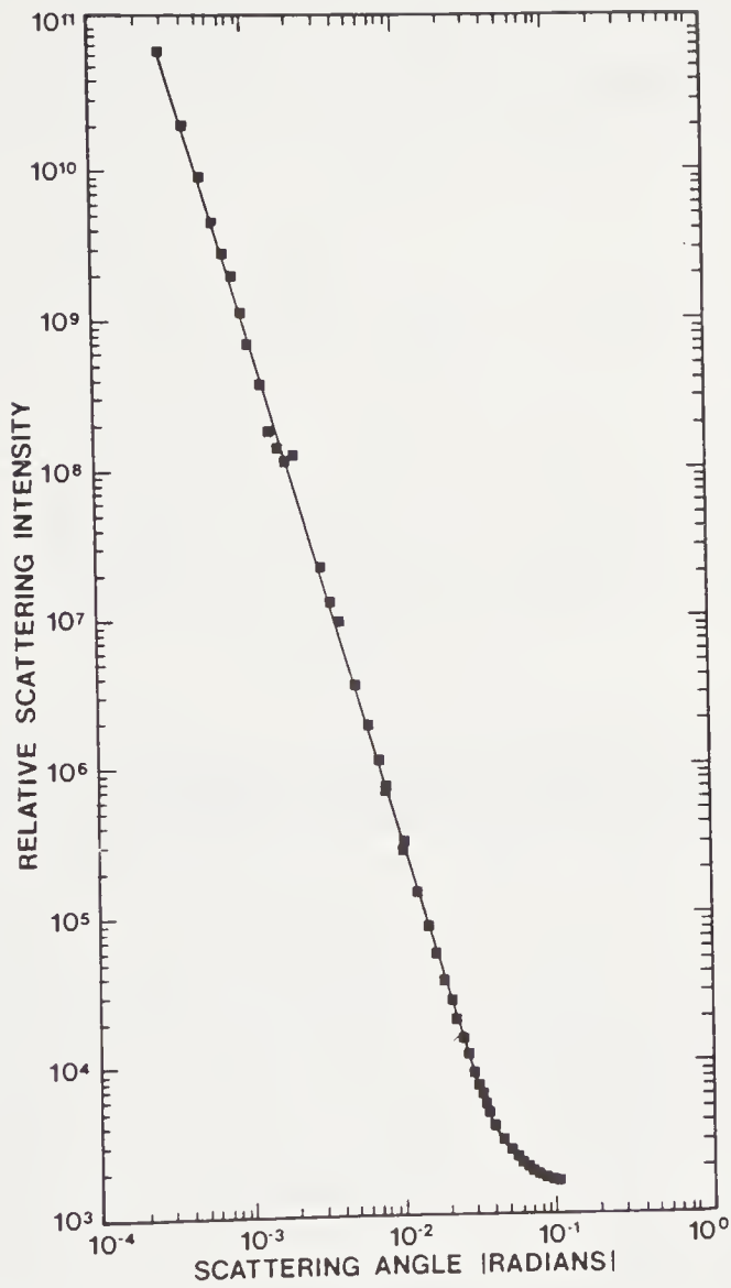
FIGURE 14.9: X-ray scattering intensity as a function of angle for Beulah lignite (Bale and Schmidt, 1984).
