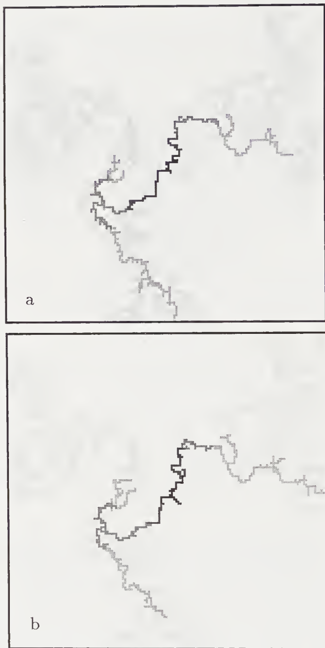
FIGURE 7.14: (a) Air displacing glycerol at a high capillary number on the percolation cluster shown in figure 7.13. (b) The results of numerical simulation of fluid displacement on the same percolation cluster. The different shades of gray represent pores invaded by air observed at successive time steps. The number of pores invaded by air is 30 (black), 86, 213 and finally at breakthrough 605 light gray, for both the experiment and the simulation. The backbone is shown in very light gray color. A color version of this figure is included in the insert that follows the Contents. (Oxaal et al., 1987).
