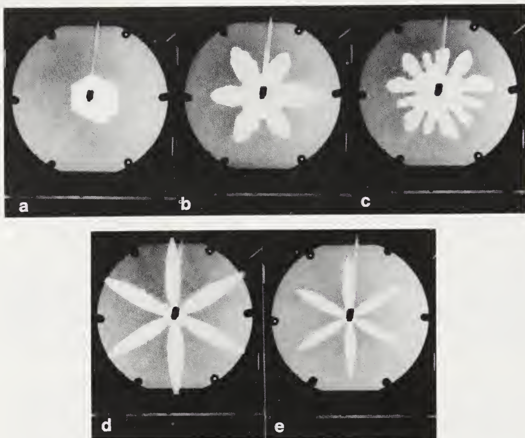
FIGURE 4.6: The various morphologies observed in the Hele-Shaw experiment with anisotropy. The cell is 25 cm across. Glycerol (black) is displaced by air (white) injected at the center. The anisotropy of the cell is \alpha = b_1/b_0 = 0.3 . The sequence of figures corresponds to increasing driving pressure. (a) Faceted growth. (b) Surface tension dendrites (with careful inspection it is possible to observe that the dendrite tips are pointed at an angle of 30^\circ to the ruling of the grooves). (c) Tip splitting growth (in a larger and more regular cell they assume that this would correspond to a dense-branching growth). (d) Kinetic dendrites (the needle crystals grow parallel to the ruled channels). (e) Kinetic dendrites at higher pressure (Ben-Jacob et al., 1985).
