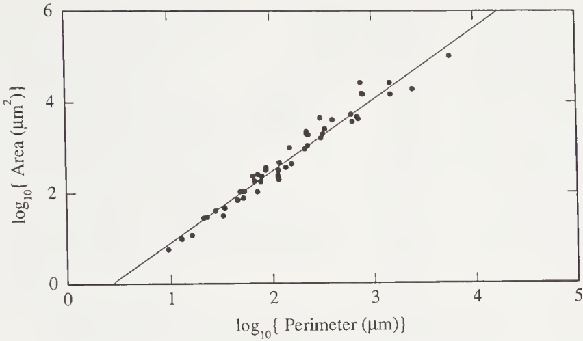
FIGURE 14.3: The perimeter-area relation for the fracture surface of 300-Grade Maraging steel. The line is a fit of A \sim L^{2/D'} with D' = 1.28 (Mandelbrot et al., 1984).
