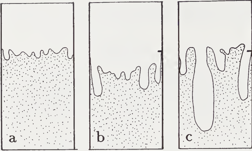
FIGURE 4.3: Viscous fingering in a vertical cell where air displaces glycerol (dark) from the top and downwards. U = 0.1 cm/s and \lambda_c = 1.2 cm. (a) Early stage with observed average \lambda \simeq 2.2 cm. (b) Later stage: Fingers tend to space themselves. (c) Late stage: Longer fingers inhibit the growth of neighbors (Saffman and Taylor, 1958).
