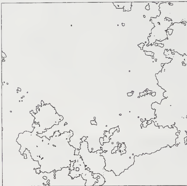
FIGURE 13.12: The coastline of the H = 0.7 landscape shown in figure 13.11. The coastline is self-similar with a fractal dimension D = 2 - H = 1.3 (Boger et al., 1987).
