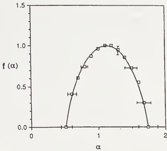
FIGURE 6.5: The multifractal spectrum for one-dimensional sections through the dissipation field in several fully developed turbulent flows (grid turbulence, wake of a circular cylinder, boundary layer, atmospheric turbulence). The symbols correspond to the experimental mean and the continuous curve is the f(\alpha) curve for the binomial multiplicative process with p = 0.7 (Meneveau and Sreenivasan, 1987).
