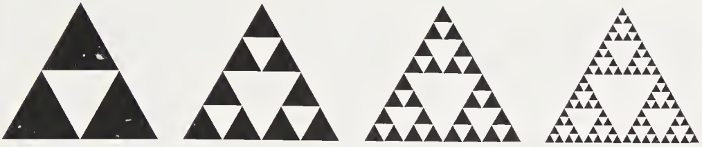
FIGURE 2.15: Construction of the triangular Sierpinski gasket. The initiator is a filled triangle. The generator eliminates a central triangle as shown. The fourth generation of the prefractal is shown to the right. The fractal curve obtained in the limit of an infinite number of generations has the fractal dimension D = \ln 3 / \ln 2 = 1.58 \dots
