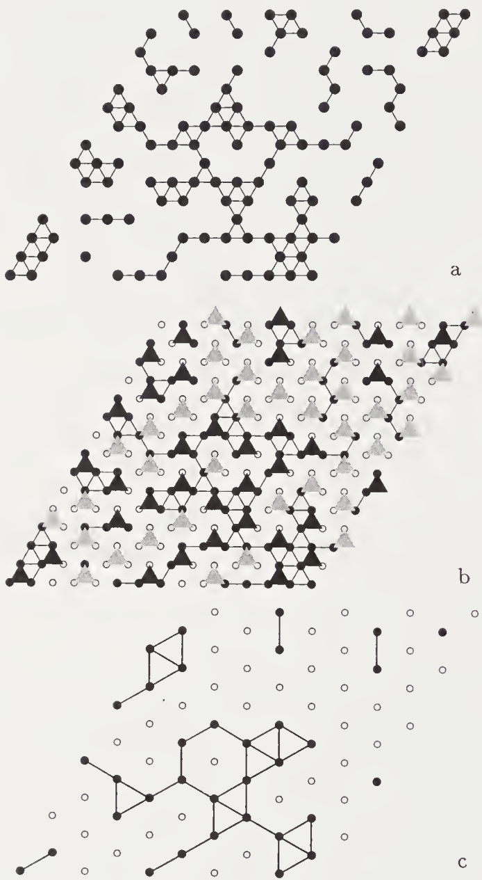
FIGURE 7.7: (a) Clusters at p_c on a triangular lattice. (b) Coarse-graining of the triangular lattice by a factor b = \sqrt{3} . Occupied sites are shown as filled circles and open sites are shown as open circles. Groups of three sites are blocked as indicated by the shaded triangles. If a majority of the sites belonging to a triangle are occupied then the triangle is shaded dark. (c) The coarse-grained percolation lattice where filled sites correspond to dark triangles in (b).
