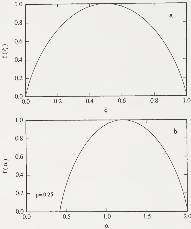
FIGURE 6.4: Fractal subsets of the measure generated by a binomial multiplicative process with p = 0.25 . (a) The fractal dimension of subsets \mathcal{S}_\xi of the interval that contain points x having a fraction \xi of zeros in the binary expansion of x , as a function of \xi . (b) The fractal dimension of subsets \mathcal{S}_\alpha having a Lipschitz-Hölder exponent \alpha , as a function of \alpha .
