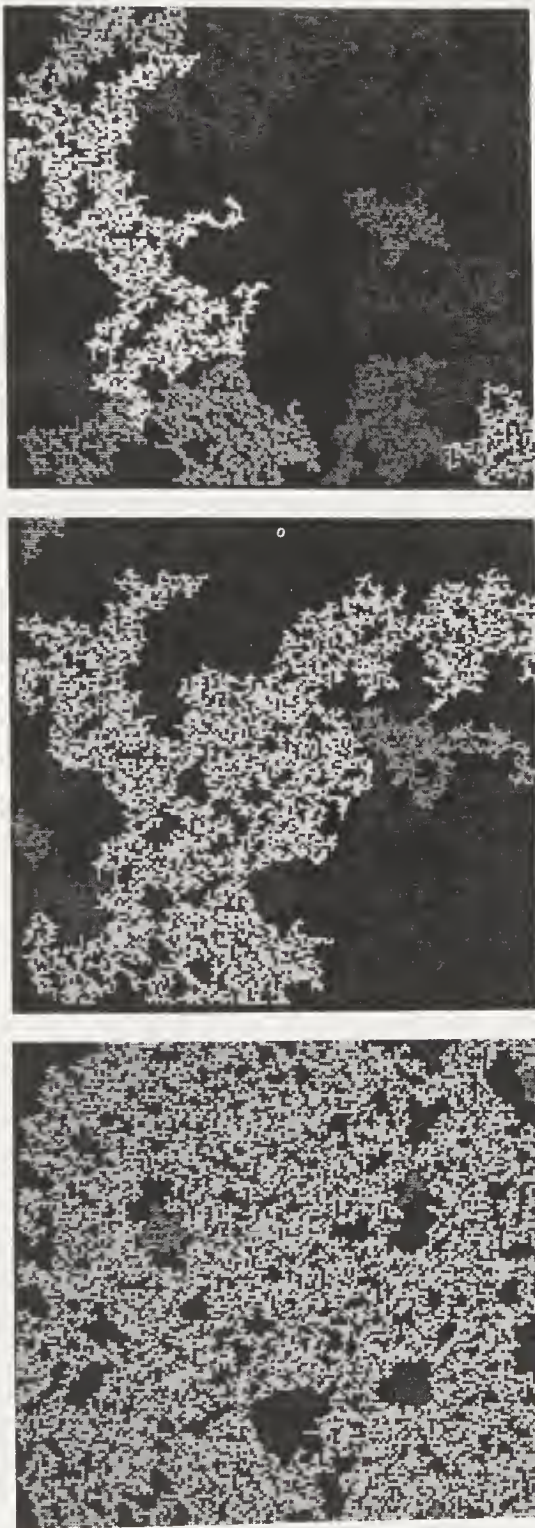
FIGURE 7.2: The effect of increasing the occupation probability p on a 160 \times 160 quadratic lattice. From top to bottom we have p = 0.58, 0.6 and 0.62 . In each of the three figures the largest cluster is shown in a light color. Smaller clusters are shown in darker shades. Unoccupied sites are black. A color version of this figure is included in the insert that follows the Contents.
