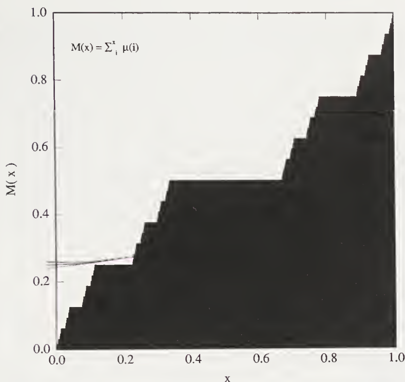
FIGURE 6.2: The mass of the triadic Cantor bar as a function of position along the bar. The curve is called a Devil's staircase .
