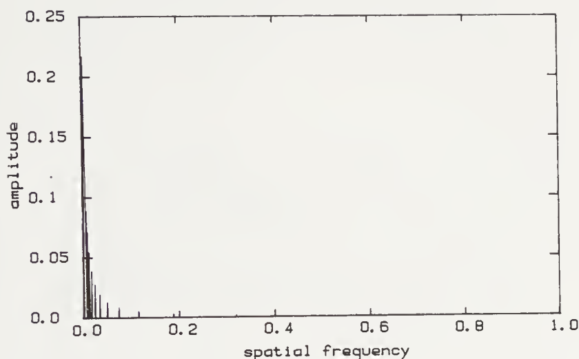
FIGURE 13.4: The amplitude spectrum for f_0 = 0.004 , \alpha = 1.1 and \beta = 1.1 .
