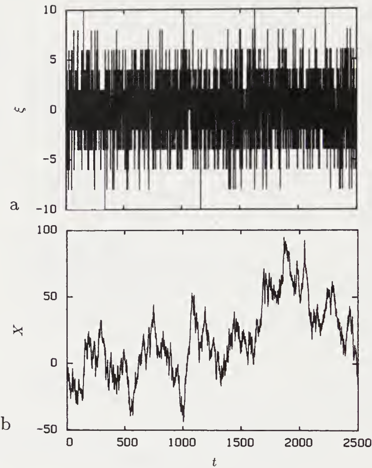
FIGURE 8.5: (a) A sequence of independent random numbers \xi(t) generated by ‘flipping’ 10 ‘coins’ 2500 times. (b) The accumulated deviation from the mean (zero) X(t) = \sum_{u=1}^t \xi(u) .
