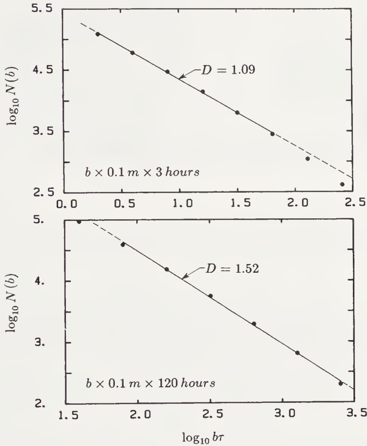
FIGURE 11.6: The number of ‘boxes’ N(b) of size b \times (a, \tau) as a function of the box scale factor b for the cumulative normalized wave-height X(t) , representing one data point every 3 hours, recorded at Tromsøflaket in the period 1980–1983. The top figure uses a minimum box of a = 0.1 \text{ m} and \tau = 3 \text{ hours} . The curve is a fit of N \sim b^{-D} with D = 1.09 \pm 0.02 . The bottom figure also uses a = 0.1 \text{ m} but a time width \tau = 120 \text{ hours} . The fit gives D = 1.52 \pm 0.03 (Frøyland et al., 1988).
