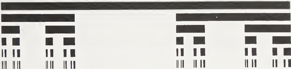
FIGURE 5.3: A two-scale Cantor bar construction with l_1 = 1/4 and l_2 = 2/5 . The fractal dimension of the Cantor set is D = 0.6110 .
