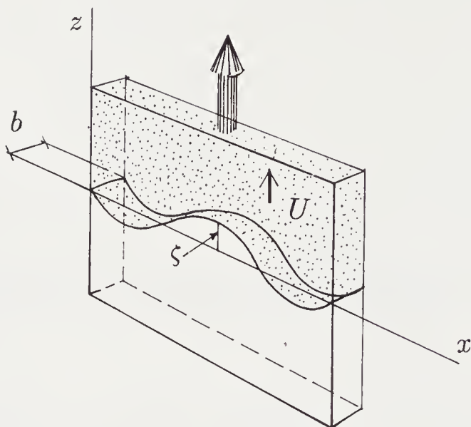
FIGURE 4.1: The geometry of the Hele-Shaw channel.
