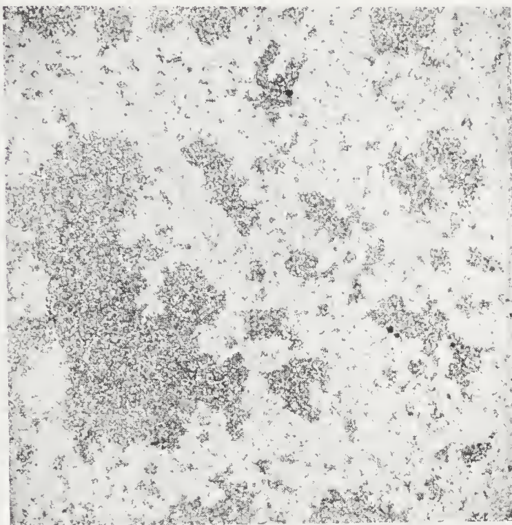
FIGURE 7.20: Displacement of the wetting fluid (black) by the nonwetting fluid (white) injected on the left-hand side of the network. On the right-hand side, a semipermeable membrane prevents the nonwetting fluid from flowing outside (Lenormand and Zarcone, 1985a).
