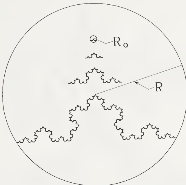
FIGURE 3.2: Triadic Koch clusters.
