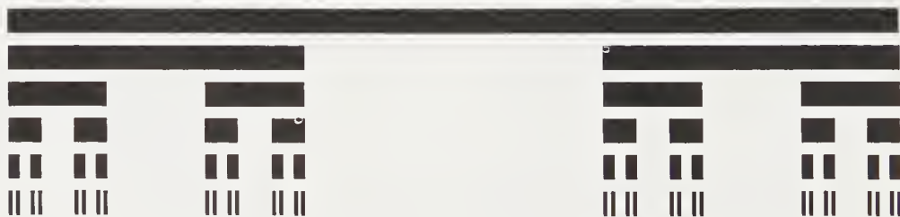
FIGURE 5.1: Construction of the triadic Cantor set. The initiator is the unit interval [0, 1] . The generator removes the open middle third. The figure shows the construction of the five first generations. D = \ln 2 / \ln 3 = 0.6309 .
