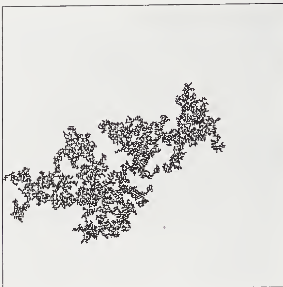
FIGURE 7.17: An invasion percolation (without trapping) cluster grown from the central site on a 300 \times 300 lattice until it reaches one of the edges of the lattice. The cluster contains 7656 sites.
