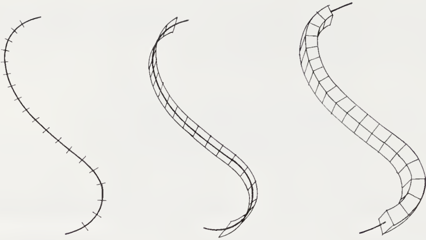
FIGURE 2.5: Measuring the 'size' of curves.
