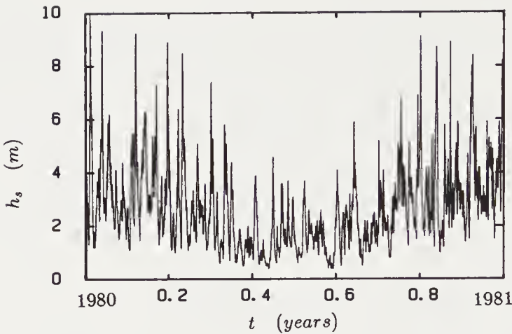
FIGURE 11.1: The maximum significant wave-height h_s at Tromsøflaket, observed every 3 hours in 1980 (The Norwegian Institute of Meteorology).
