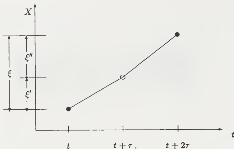
FIGURE 9.2: The increment \xi in the position of a Brownian particle at time step 2\tau is the sum of two independent increments \xi' and \xi'' .
