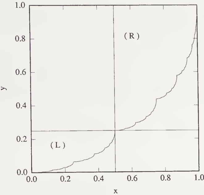
FIGURE 10.3: Two affine transformations of the coordinate system mapping the unit square into rectangles by the L and R transformations given in equation (10.10). A combination of the two transformations reproduces the original self-affine curve y = M(x) , calculated for p = 0.25 .
