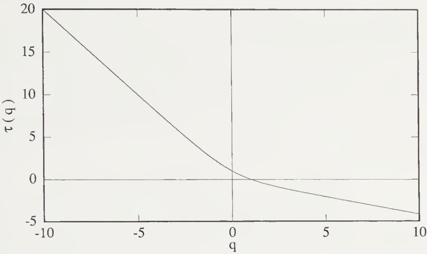
FIGURE 6.6: The sequence of mass exponents \tau(q) as a function of moment order q , for the measure M_d(q, \delta) for the binomial multiplicative process with p = 0.25 .
