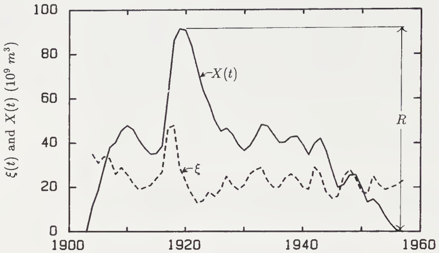
FIGURE 8.1: Lake Albert annual discharge \xi(t) (broken line), and accumulated departures from the mean discharge X(t) (full line). The range is indicated by R (after Hurst et al., 1965).
