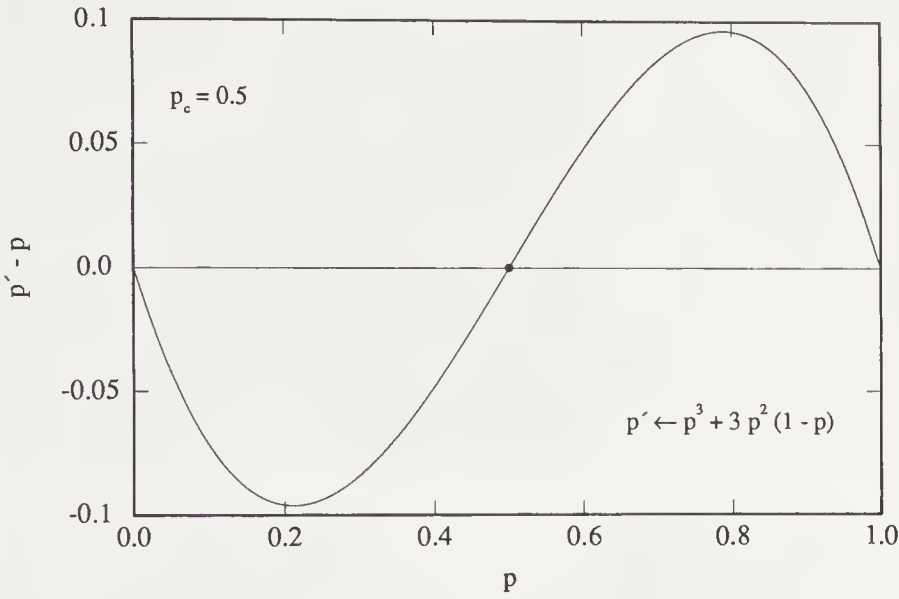
FIGURE 7.8: The change in the concentration of occupied sites, p' - p , as a function of the concentration of occupied sites, p , on the triangular lattice before a rescaling of the lattice by a factor of b = \sqrt{3} .
