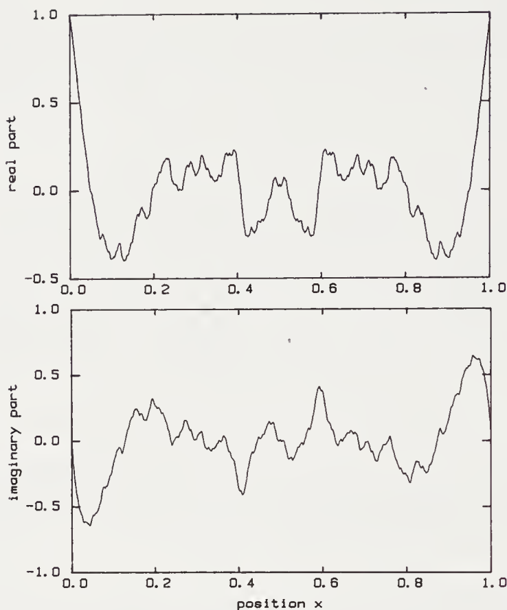
FIGURE 13.5: The real and imaginary parts of \mathcal{Z} as functions of position x for f_0 = 0.004 , \alpha = 1.1 and \beta = 1.1 .
