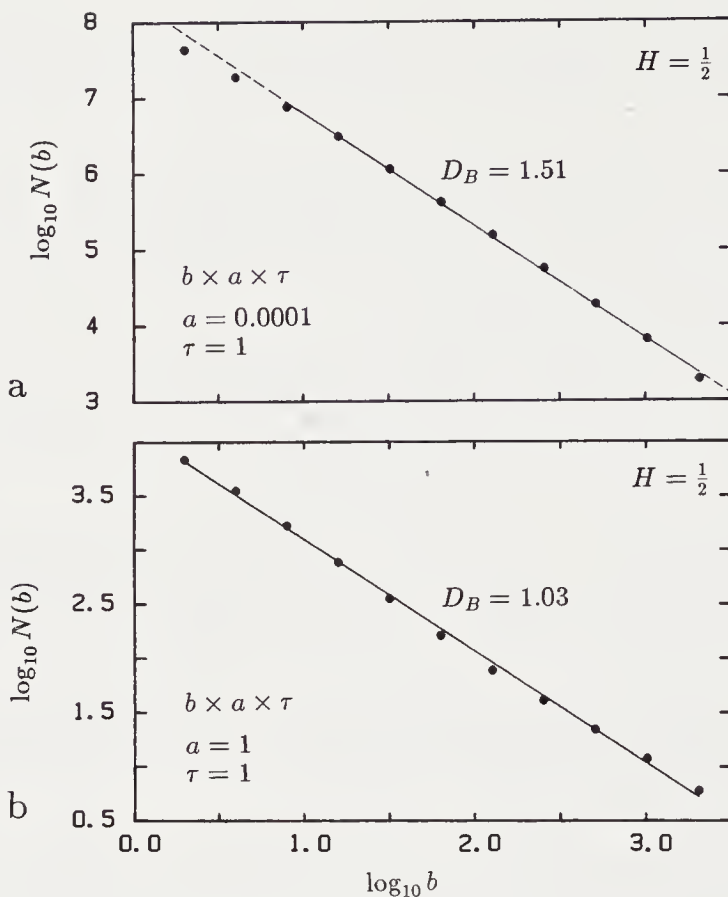
FIGURE 10.1: The number of boxes N(b; a, \tau) of size b \times (a, \tau) as a function of the box scale factor b for the record B(t) of an independent Gaussian process consisting of 7500 steps. (a) Using a = 0.0001 and \tau = 1 we find a fit with D_B = 1.51 \pm 0.02 . (b) Using a = 1 and \tau = 1 we find D_B = 1.03 \pm 0.02 .
