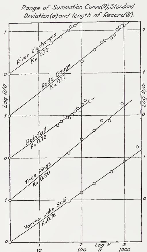
FIGURE 8.4: Rescaled range analysis for various natural phenomena. The lag is \tau = N , the number of years (Hurst et al., 1965).
