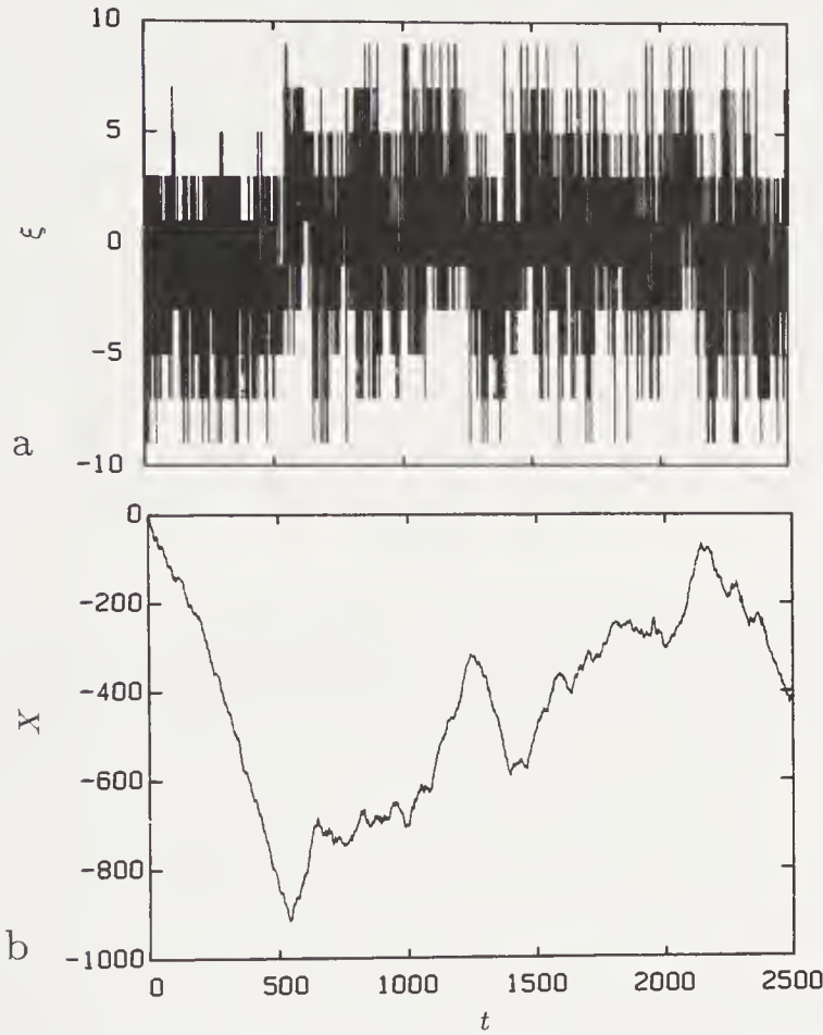
FIGURE 8.7: (a) A sequence of biased random numbers \xi(t) generated by drawing 'cards' from a biased 'hand' generated by the Hurst process, repeated 2500 times. (b) The accumulated deviation from the (zero) mean X(t) = \sum_{u=1}^t \xi(u) .
