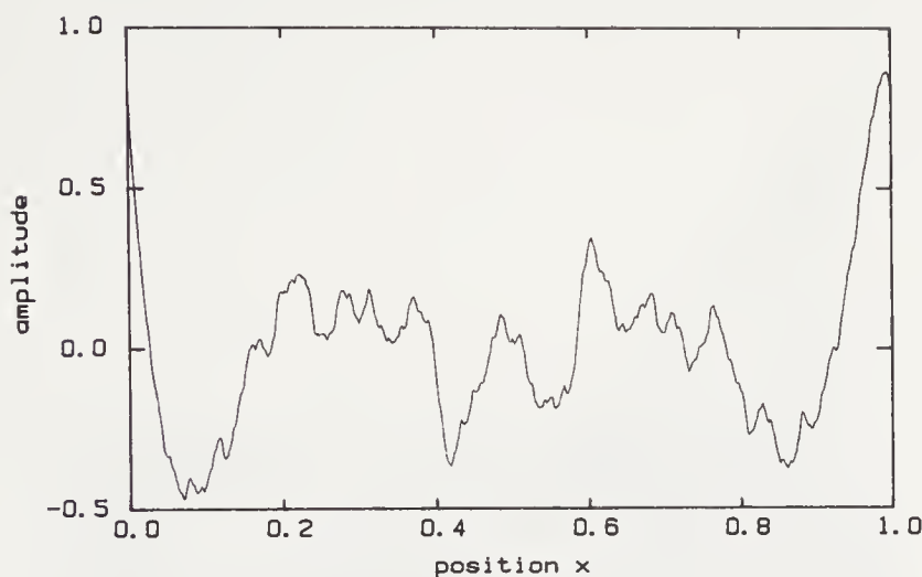
FIGURE 13.6: The profile z(x, 0 \mid \psi = 0.616) .
