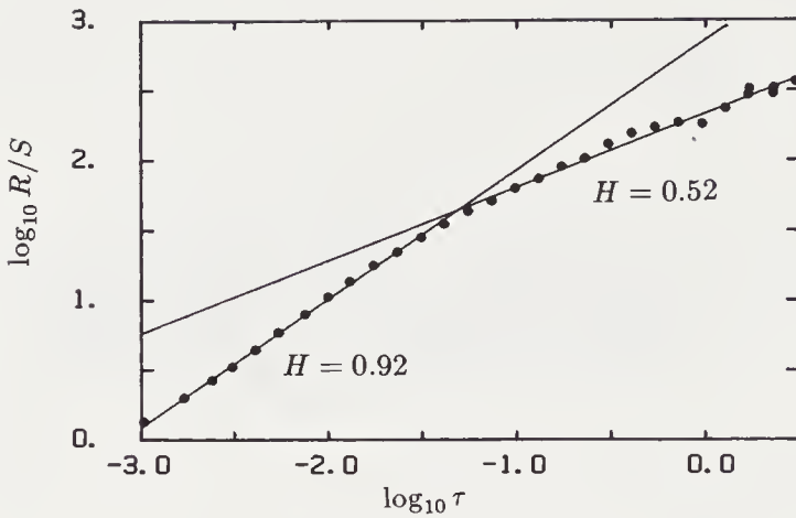
FIGURE 11.5: R/S as a function of the lag \tau (in years), for a process where the seasonally adjusted and normalized significant wave-height \xi for Tromsøflaket is considered to be the step in a (fractional) random walk. The lines are fits of the Hurst law R/S \sim \tau^H . The fit for \tau < 10 days gives H = 0.92 \pm 0.02 , and the fit for \tau > 20 days gives H = 0.52 \pm 0.02 (Frøyland et al., 1988).
