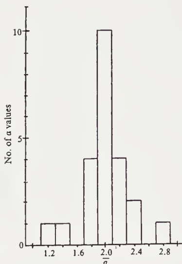
FIGURE 14.2: Histogram for the exponent \alpha for the 23 sets of data in the previous figure (Sayles and Thomas, 1978b).
