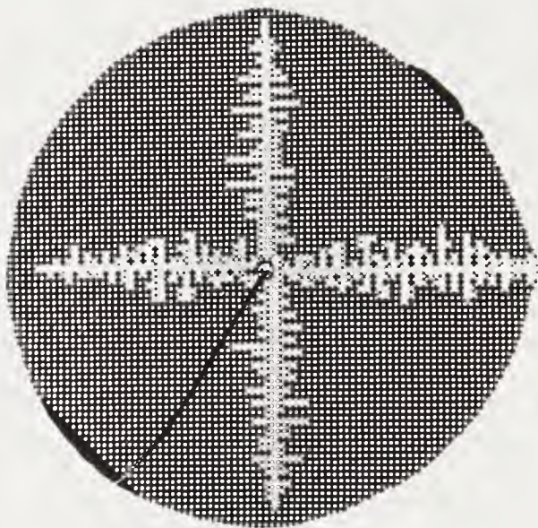
FIGURE 4.9: Viscous fingering of air displacing glycerol in a two-dimensional porous medium consisting of a regular square array of cylinders 1 mm in diameter between two plastic plates. The capillary number is Ca = 0.05 (Feder et al., 1986).
