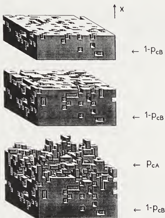
FIGURE 7.26: Picture of a 19 \times 19 \times 19 -site system. The particles are shown as cubes, and the probability of having a site occupied decreases from 1 at the bottom of the sample to 0 at the top. Only sites occupied by particles connected to the bottom are shown. (a) The top figure shows the bottom six layers in the high-density part of the sample. (b) The top layer in the middle figure is at a concentration corresponding to the percolation threshold of the quadratic lattice. (c) The bottom figure shows all the sites connected to the bottom plane. The arrows indicate the planes where the occupation probability is given by 1 - p_{cB} and by p_{cA} (Rosso et al., 1986).
