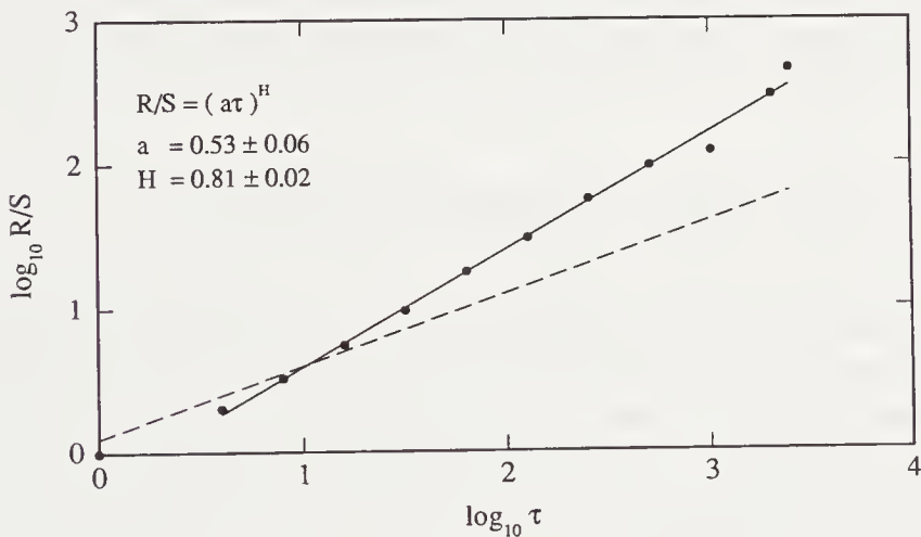
FIGURE 9.8: R/S as a function of the lag \tau for the fractal Brownian function B_H(t) with H = 0.9 . The dotted line is the asymptotic result for an independent Gaussian process R/S = \sqrt{\pi\tau/2} . The line is the fitted curve R/S = (a\tau)^H with H = 0.81 \pm 0.02 and a = 0.53 \pm 0.06 .
