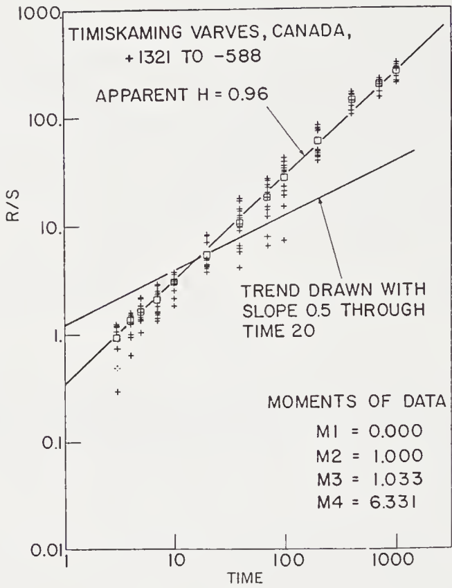
FIGURE 8.10: R/S diagram for the thickness of the varves in Timiskaming, Canada, as a function of the lag \tau in years (Mandelbrot and Wallis, 1969a).
