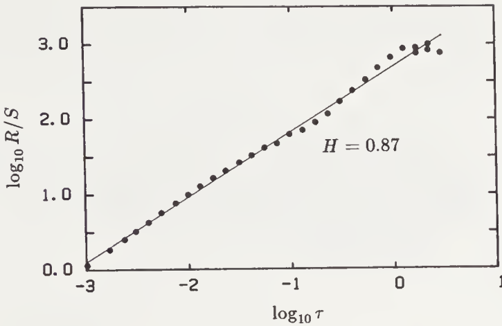
FIGURE 11.2: R/S as a function of the lag \tau , for a process where the significant wave-height h_s for Tromsøflaket is considered to be the random process \{\xi\} . The line represents a fit of the Hurst law R/S \sim \tau^H to the data with H = 0.87 \pm 0.01 (Frøyland et al., 1988).
