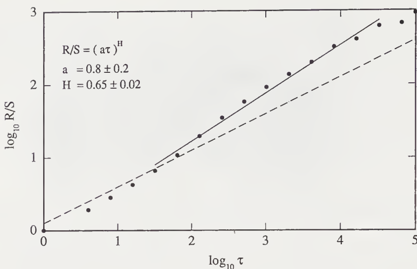
FIGURE 8.8: R/S as a function of the lag \tau (filled circles) for a random variable \xi(t) generated by cutting cards from a biased hand by the Hurst procedure, repeated T = 100,000 times. The Gaussian asymptotic behavior R/S = \sqrt{\pi\tau/2} is shown as the broken line. The fit (full line) of the form R/S = (a\tau)^H to the observed values of R/S shown was obtained with the parameter values a = 0.8 \pm 0.2 , and H = 0.65 \pm 0.02 .
