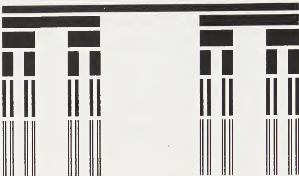
FIGURE 6.1: The triadic Cantor bar. A bar of unit length and mass is divided into two and hammered to a reduced length so that the density increases. The height of the bars in the n -th generation is proportional to the density \rho_i . The Lipschitz-Hölder exponent is \alpha = (\ln 2)/(\ln 3) , and the fractal dimension of the support of the mass is f = D = (\ln 2)/(\ln 3) .
