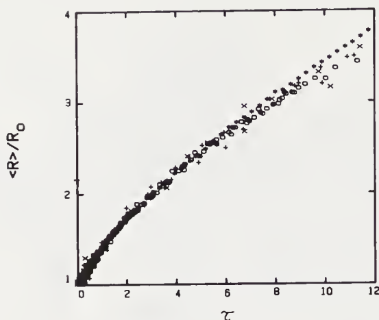
FIGURE 3.5: The effective hydrodynamic radius of IgG aggregates as a function of the reduced time \tau = \gamma t , for various temperatures and concentrations. Cluster fractal dimension D = 2.56 \pm 0.3 (Feder et al., 1984).
