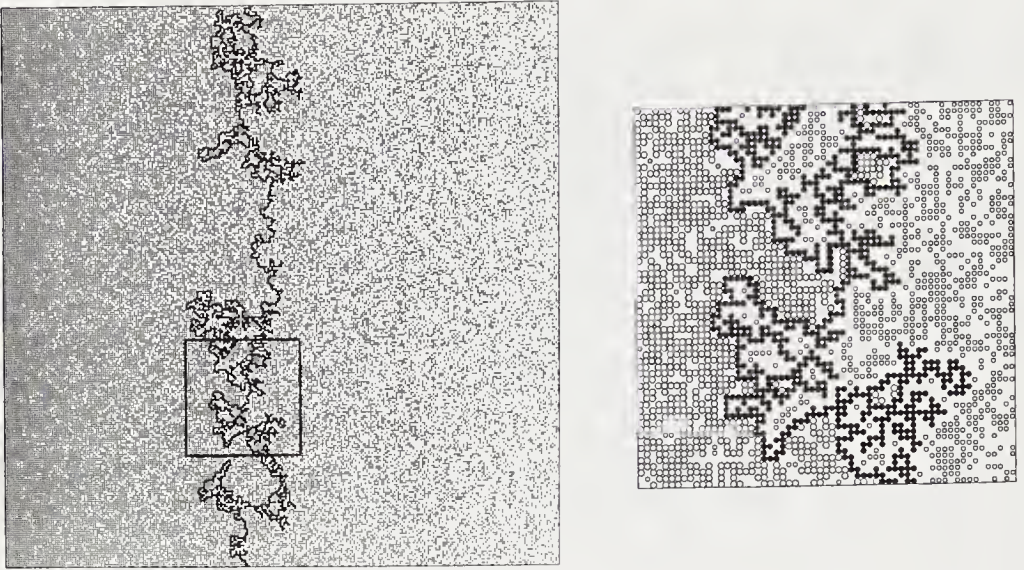
FIGURE 7.22: Diffusion of ‘particles’ (filled circles) from a source at the left-hand edge of a lattice consisting of sites (empty squares). The particles (filled squares) that are both connected to the source and neighbors to sites connected to the right-hand edge constitute the hull of the diffusing particles. The right-hand figure is a blow-up of the region marked by a square in the left-hand figure. Here the hull is shown as filled circles, sites connected to the source as large circles and the remaining occupied sites as small circles. A color version of the left-hand part of this figure is included in the insert that follows the Contents.
