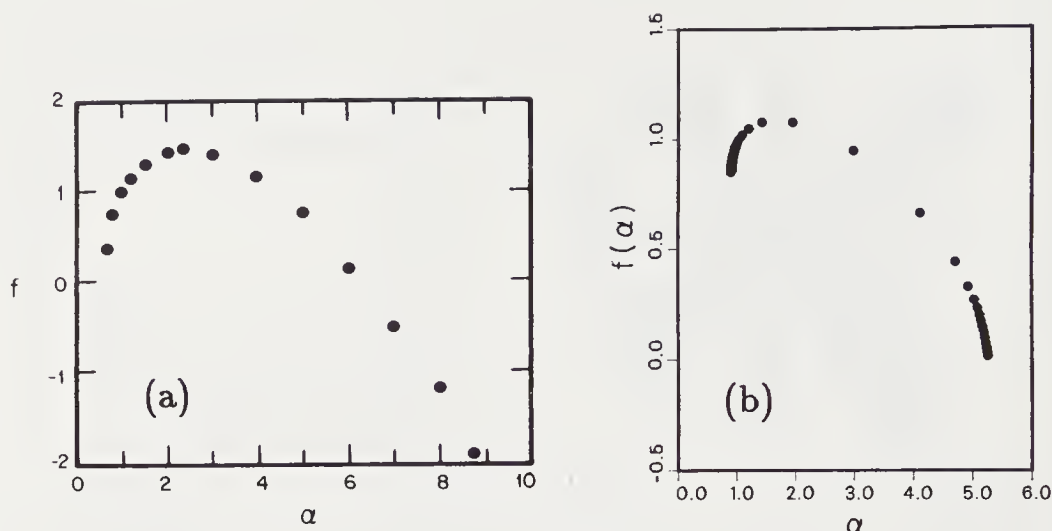
FIGURE 6.13: (a) The f(\alpha) curve for the harmonic measure on DLA clusters. The largest cluster used in the estimate contained 150 particles (Amirtrano et al., 1986). (b) The f(\alpha) curve for the harmonic measure calculated for a viscous fingering structure (similar to the one shown in figure 4.5b) observed in a Hele-Shaw cell (Nittmann et al., 1987).
