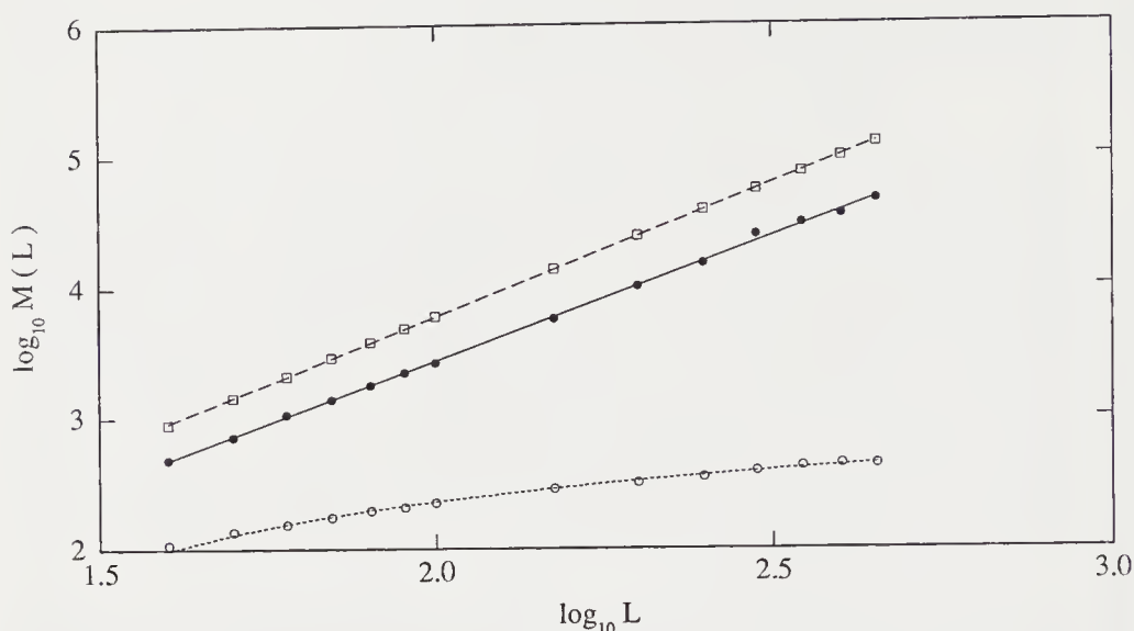
FIGURE 7.4: The mass of the largest cluster as a function of the linear dimension L of the quadratic lattice. Filled circles are for p = p_c = 0.593 . The solid line is M(L) = AL^D with D = 1.89 . For p = 0.65 (open boxes) a fit (dashed line) gives D = 2.03 . The results for p = 0.5 , i.e., below p_c , have been fitted to the form M(L) = A + B \ln L , shown as the dotted line through the open circles.
