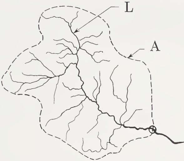
FIGURE 12.5: Drainage area A and the length L of the longest river above a given location.
