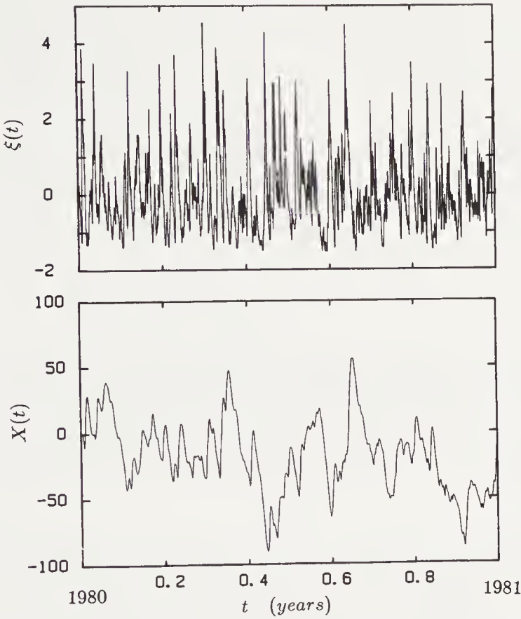
FIGURE 11.4: The normalized seasonally adjusted wave-height \xi(t) as a function of time for the observations of h_s on Tromsøflaket. The bottom figure shows the cumulative sum X(t) = \sum_{u=0}^t \xi(u) as a function of time (Frøyland et al., 1988).
