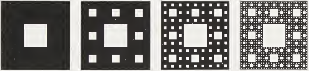
FIGURE 2.16: Construction of the Sierpinski carpet. The initiator is a square and the generator (shown on the left-hand side) is made of N = 8 squares. They are obtained by contractions of ratio r = 1/3 . The right-hand side of the figure shows the fourth construction stage. The similarity dimension is D = \ln 8 / \ln 3 = 1.89 \dots
