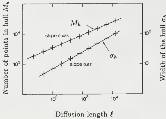
FIGURE 7.24: Variation of the number of points in the hull, M_h , and of the width \sigma_h , as functions of the diffusion length \ell (Sapoval et al., 1985).
