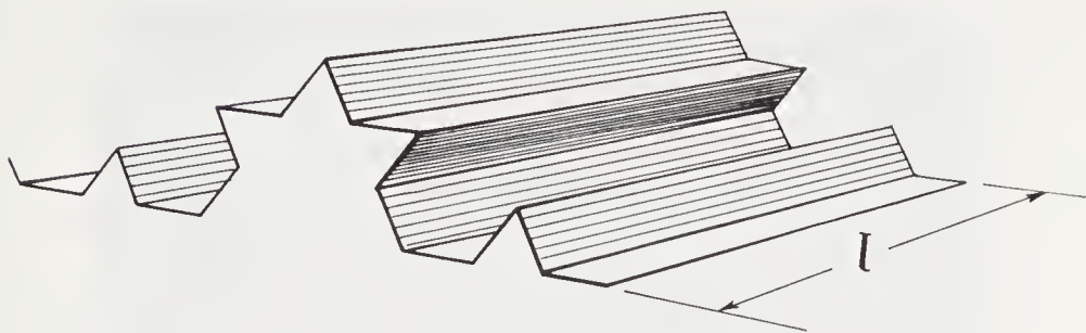
FIGURE 13.1: A triadic Koch surface. D = 2.262 \dots
