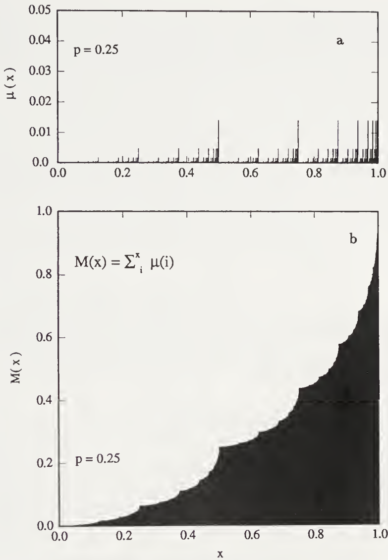
FIGURE 6.3: The measure M(x) for the binominal multiplicative process after n = 11 generations with \mu_0 = p = 0.25 and \mu_1 = 1 - p = 0.75 . (a) The measure or content \mu of a cell as a function of the segment number (position) x = i \cdot 2^{-11} . (b) The measure M(x) for the interval [0, x] as a function of x .
