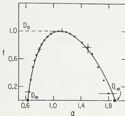
FIGURE 6.11: The f(\alpha) curve for thermal convection. The points are estimated from the observed time series. The curve is the f(\alpha) curve for the critical circle map. Note that there are no free parameters and the observations fit the theory remarkably well (Jensen et al., 1985).
