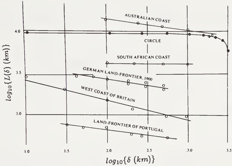
FIGURE 2.3: The length of coastlines as a function of yardstick length (Mandelbrot, 1982).
