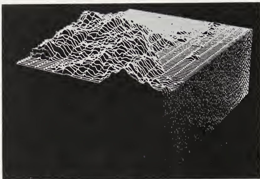
FIGURE 13.2: The first example of fractal Brownian islands. D = 2.5 (Mandelbrot, 1975b).
