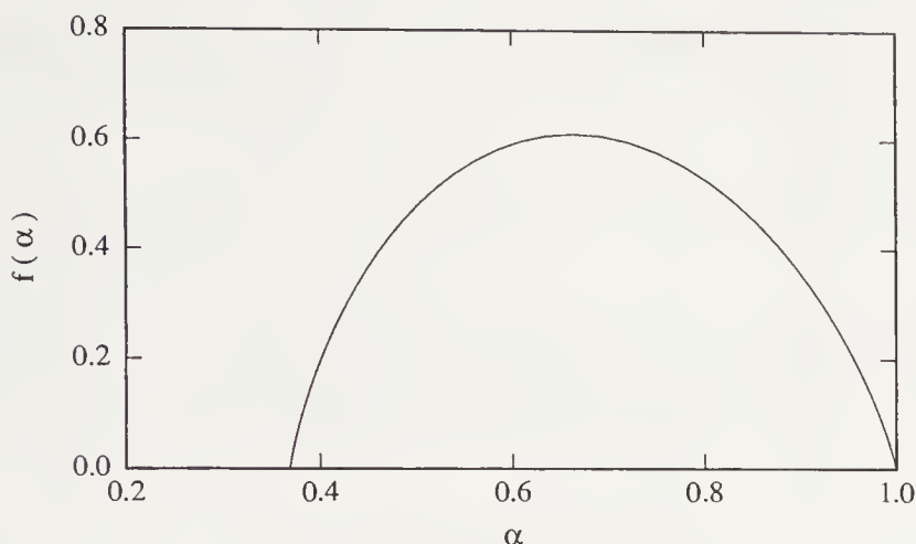
FIGURE 6.8: The f(\alpha) curve for the two-scale fractal measure on a Cantor bar \mathcal{S} , with l_0 = 1/4 , l_1 = 2/5 and weights p_0 = 3/5 and p_1 = 2/5 . This represents the fractal dimension, f , of the subsets \mathcal{S}_\alpha with Lipschitz-Hölder exponent \alpha as function of \alpha .
