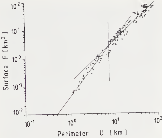
FIGURE 12.3: Log-log plot of the perimeter-area relation for hail storms. Every point corresponds to a particular time during the temporal evolution of a storm. From the linear fits (shown as full lines) of 24 different hail storms the averaged fractal dimensions in equation (12.3) were obtained (Rys and Waldvogel, 1986).
