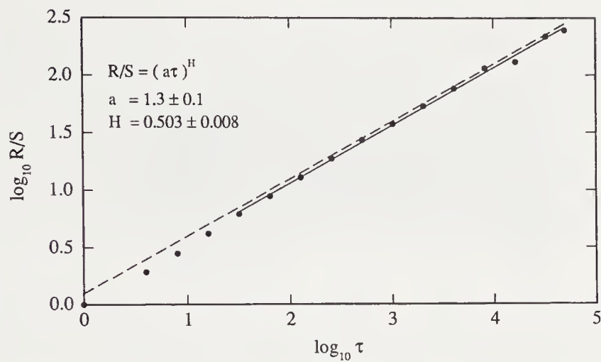
FIGURE 8.6: R/S as a function of lag \tau (filled circles), for a random variable \xi(t) given as the difference between the number of ‘heads’ and ‘tails’ in tosses of 10 coins repeated T = 50,000 times. The Gaussian asymptotic behavior R/S = \sqrt{\pi\tau/2} , is shown as the broken line. The line represents a fit of R/S = (a\tau)^H to the observed R/S . The parameters of the fit are a = 1.3 \pm 0.1 and H = 0.503 \pm 0.008 .
