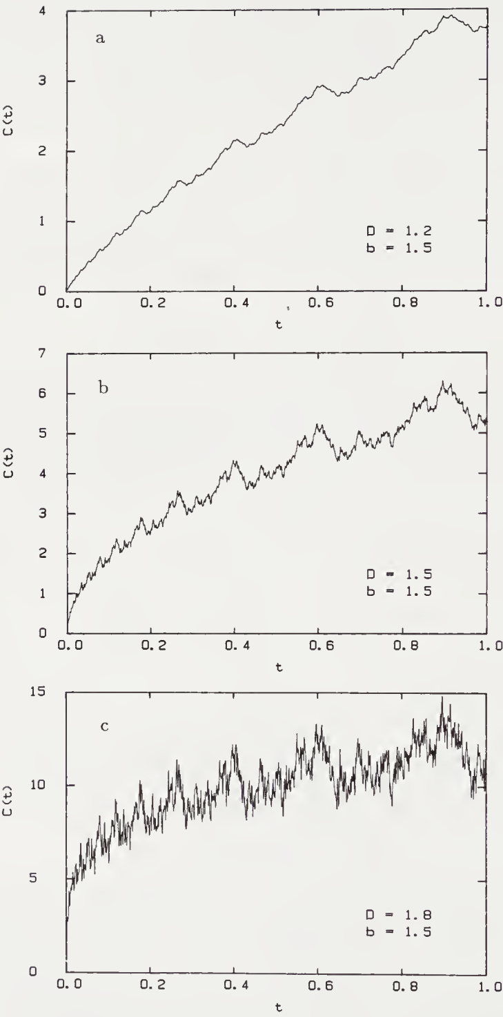
FIGURE 2.17: The Weierstrass-Mandelbrot fractal function C(t) with b = 1.5 . (a) D = 1.2 . (b) D = 1.5 . (c) D = 1.8 .
