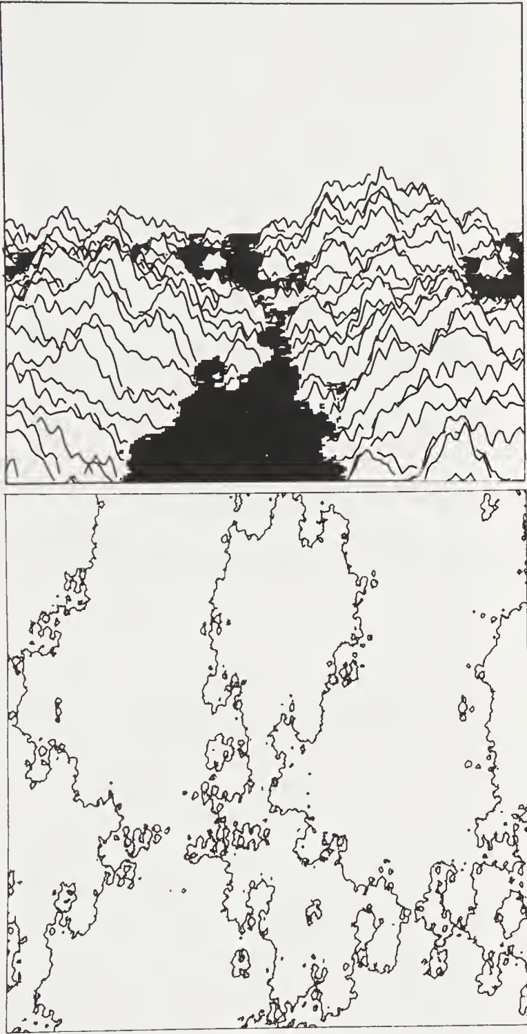
FIGURE 13.10: Weierstrass-Mandelbrot landscape. \beta = 0.59 , b = 4.7 . Coastline fractal dimension D = 1.35 .
