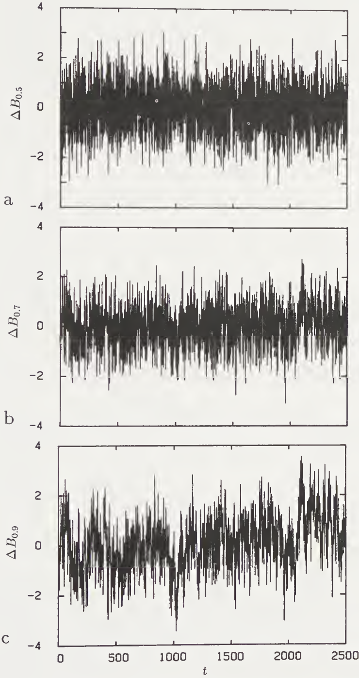
FIGURE 9.4: Fractal noise or increments of the fractal Brownian function B_H evaluated with M = 700 , n = 8 . (a) Ordinary Brownian increments for H = 1/2 . (b) Fractional increments for H = 0.7 . (c) Fractional increments for H = 0.9 .
