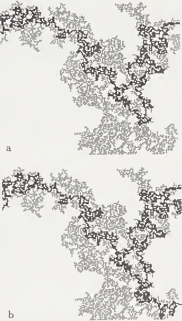
FIGURE 7.15: Backbones of the percolation cluster on the quadratic lattice at p_c shown in figure 7.2b. (a) The backbone connecting a single site on the left-hand edge to a single site on the right-hand edge of the 160 \times 160 lattice. (b) The backbone connecting all the sites on the left-hand edge to all the sites on the right-hand edge.
