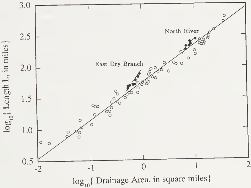
FIGURE 12.6: Relation between stream length and drainage area (Hack, 1957).
