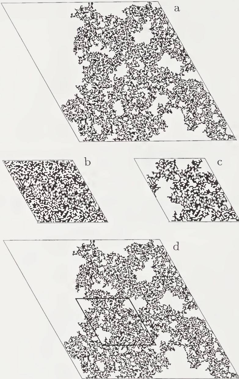
FIGURE 7.9: Self-similarity and the effect of coarse-graining on the triangular lattice at the percolation threshold. The scale is changed by a factor b = 3 , using the renormalization procedure illustrated in figure 7.7 twice. (a) The percolation cluster at threshold on the original 180 \times 180 lattice. (b) The occupied sites obtained after a scaling of the original lattice in (a) by a factor b = 3 . (c) The percolation cluster of the scaled lattice in (b). (d) The scaled lattice is inserted into the original lattice in the region marked by a frame. The figure shows the resulting percolation cluster.
