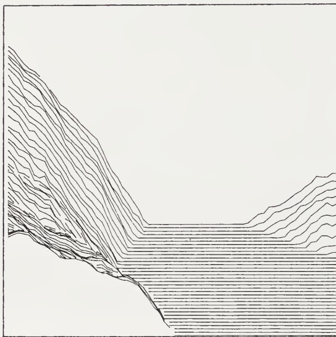
FIGURE 13.7: A landscape generated by 12 layers. \alpha = 1.1 , \beta = 1.1 .
