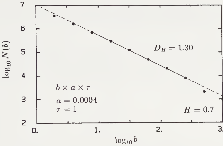
FIGURE 10.2: The number of boxes N(b; a, \tau) of size b \times (4 \cdot 10^{-4}, 1) as a function of the box scale factor b for the record B_H(t) of an H = 0.7 fractal Brownian function of 2500 steps. The curve is a fit with D_B = 1.30 \pm 0.02 .
