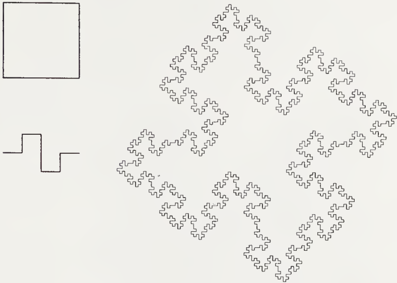
FIGURE 2.9: Construction of the quadratic Koch curve.
