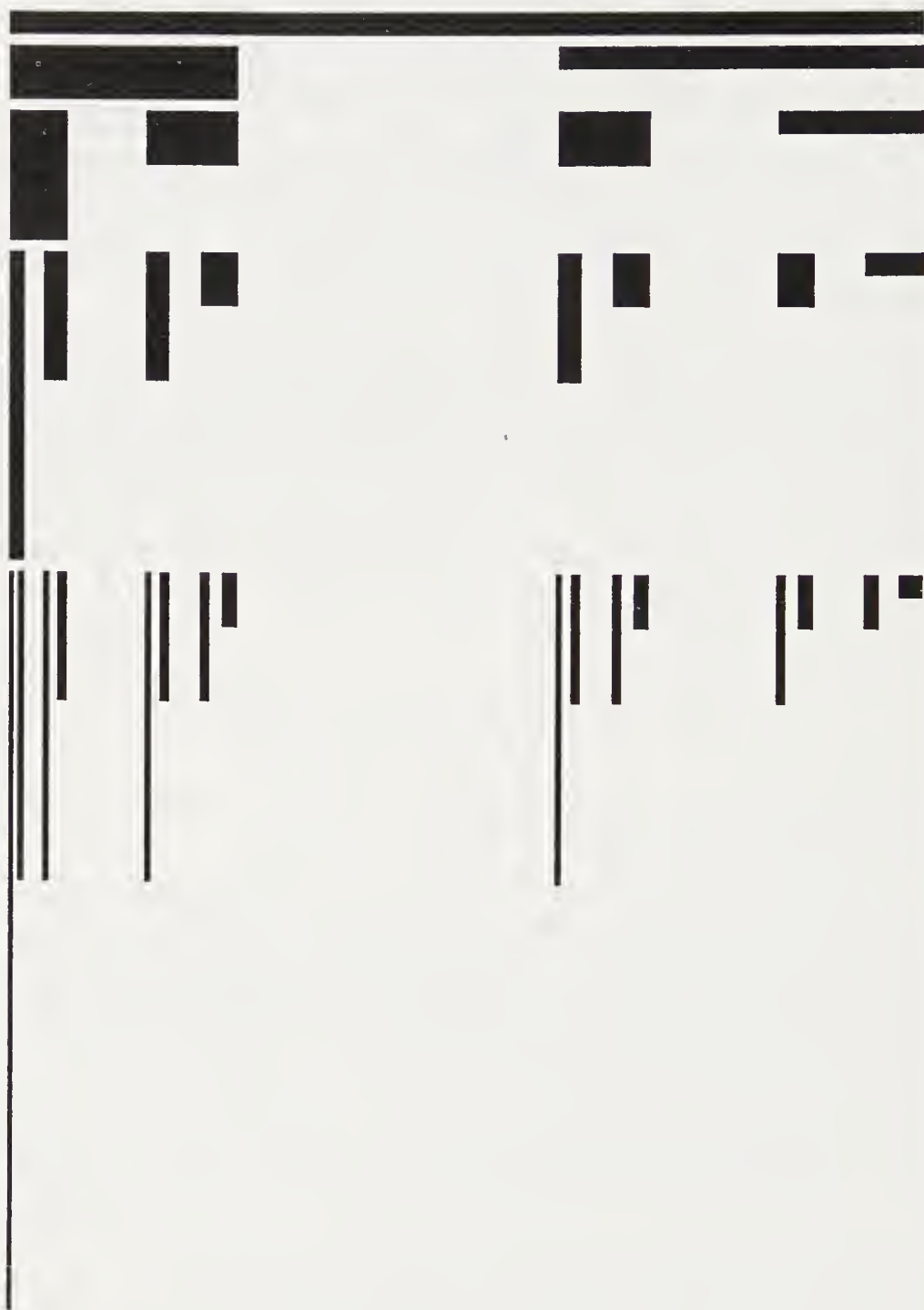
FIGURE 6.7: A two-scale fractal measure on a Cantor bar with l_0 = 0.25 and weight p_0 = 0.6 , and l_1 = 0.4 with p_1 = 0.4 . The height of the bars in the n -th generation is proportional to the density \rho_i = \mu_i/l_i . The fractal dimension of the Cantor dust supporting the measure is D = 0.6110 .
