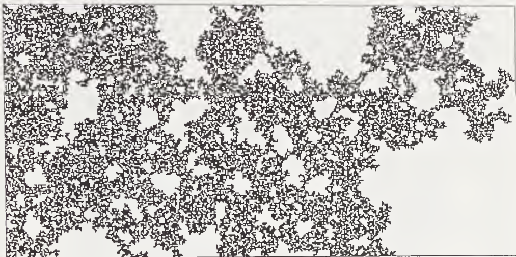
FIGURE 7.18: Invasion percolation (without trapping) on a 100 \times 200 quadratic lattice. The invader (black) enters from sites on the left-hand edge and the defender escapes through the right-hand edge. At 'break-through' the invader just reaches the right-hand edge.
