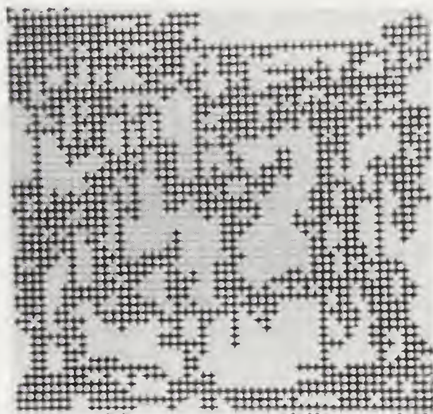
FIGURE 7.16: Invasion percolation of water (black) displacing air in a model consisting of a regular array of cylinders 2 mm in diameter and 0.7 mm high separating parallel plates. The water does not wet the model. The water enters at the upper left corner and exits at the lower right corner. The displacement is at Ca \simeq 10^{-5} (Feder et al., 1986).
