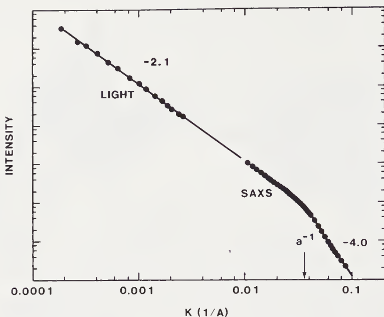
FIGURE 3.9: Combined small-angle X-ray scattering and light scattering intensity results for silica aggregates. D = 2.12 \pm 0.05 (Schaefer et al., 1984).
