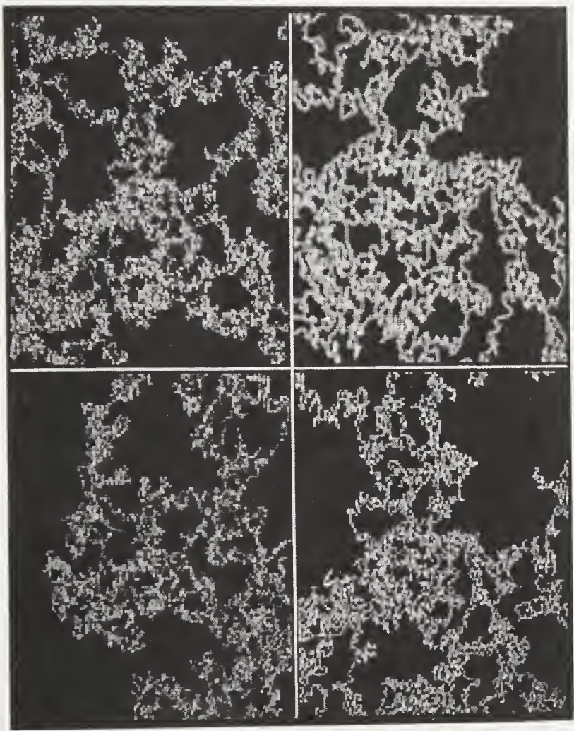
FIGURE 7.23: Self-similarity of the diffusion front. The hull is shown as a series of magnifications of a central part. The magnification is a factor of two each time. The self-similarity is apparent in the fact that it calls for a rather close inspection of the four figures if one wants to order the figures according to magnification (Sapoval et al., 1986).
