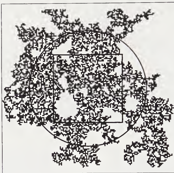
FIGURE 7.10: A finite cluster on the square lattice at p_c . The radius of the circle is the radius of gyration, R_g(s) = 51 , of a cluster containing 6700 sites. The box indicated in the figure has a side L = 60 . The side of the smallest box that contains the cluster is L_s = 150 .
