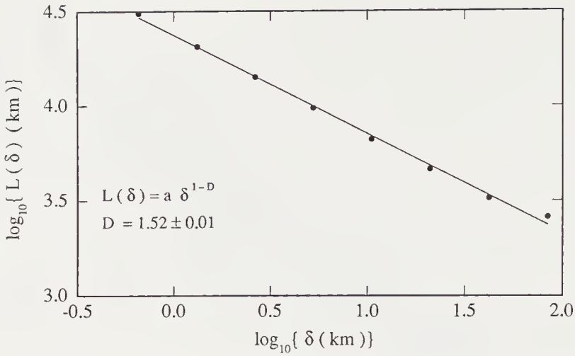
FIGURE 2.2: The measured length of the coastline shown in figure 2.1, as a function of the size \delta of the \delta \times \delta squares used to cover the coastline on the map. The straight line in this log-log plot corresponds to the relation L(\delta) = a \cdot \delta^{1-D} , with D \simeq 1.52 .
