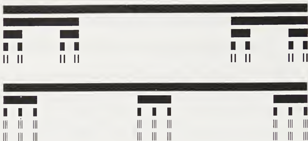
FIGURE 5.2: Two constructions of the Cantor set with D = 1/2 . Top figure: N = 2 and r = 1/4 . Bottom figure: N = 3 and r = 1/9 .
