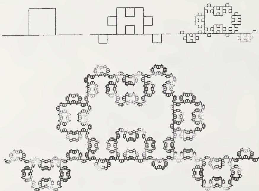
FIGURE 2.14: Construction of a Mandelbrot-Given curve without branches. This curve is obtained using a generator with a single loop. The fractal dimension is D_B = \ln 6 / \ln 3 = 1.63 \dots
