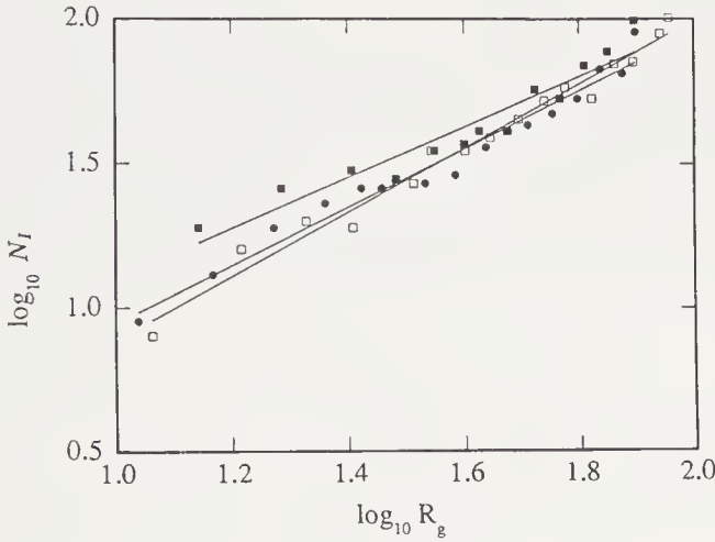
FIGURE 6.16: The number growth sites as a function of the radius of gyration for three experiments in which air displaces glycerol. The straight lines represent fits of equation (6.66) to the observed values. The parameters of the fit are : \bullet - a = 0.9 \pm 0.2 , D_I = 1.01 \pm 0.05 . \blacksquare - a = 1.7 \pm 0.6 , D_I = 0.87 \pm 0.08 . \square - a = 0.6 \pm 0.1 , D_I = 1.11 \pm 0.04 . The fractal dimension of the growing interface is D_I = 1.0 \pm 0.1 .
