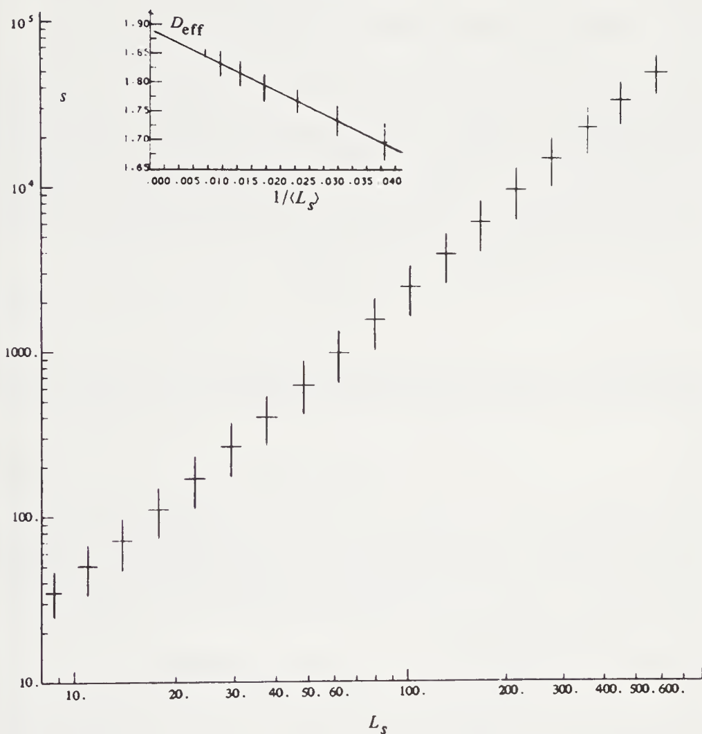
FIGURE 7.11: Dependence of the cluster masses s (number of sites) on their linear size L_s , for the square lattice at p_c = 0.5927 . The error bars indicate one standard deviation around the average. The insert shows the extrapolation of the local slope D_{\text{eff}} = \partial \ln s / \partial \ln L_s to s \rightarrow \infty , where D = 1.89 \pm 0.01 (Aharony, 1986).
