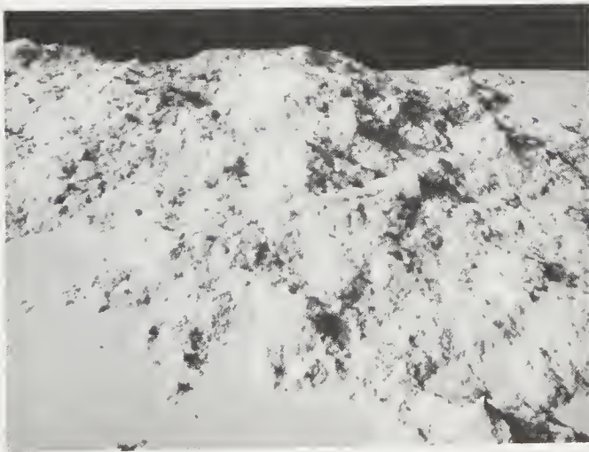
FIGURE 13.11: Fractal landscapes generated using Voss's successive random addition algorithm. The landscapes were generated on a 1025 \times 1025 square grid. The variance of the additions was \sigma^2 = (1/\sqrt{2})^{2nH} in the n -th generation for 18 generations. The Hurst exponents used were H = 0.5 , 0.7 and 0.9 , in the top, middle and bottom figures, respectively (Boger et al., 1987).
