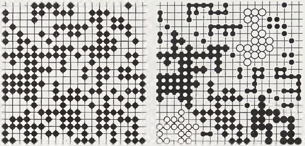
FIGURE 7.1: A quadratic lattice with one half of the nodes occupied by ‘pores’ is shown to the left. Connected regions, or ‘clusters’ are shown to the right. The largest clusters are distinguished by using different symbols for the pores. The lattice consists of L \times L nodes with L = 20 .
