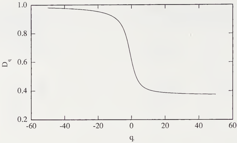
FIGURE 6.9: The spectrum of fractal dimensions D_q as a function of the moment order q for the triadic Cantor dust with l_0 = 1/4 , l_1 = 2/5 and weights p_0 = 3/5 and p_1 = 2/5 . D_\infty = \ln p_0 / \ln l_0 = 0.3685 and D_{-\infty} = \ln p_1 / \ln l_1 = 1 .
