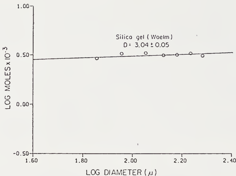
FIGURE 14.7: Measured monolayer mole numbers n of tertiary amyl alcohol as a function of adsorbent particle diameter ( 2R ) ( \mu\text{m} ) (Pfeifer et al., 1984).
