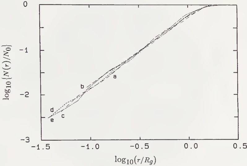
FIGURE 4.8: The normalized finger structure volume N(r)/N_0 as a function of the reduced radius (r/R_g) for the structures shown in the previous figure. (a) R_g = 1.7 cm. (b) R_g = 2.9 cm. (c) R_g = 5.2 cm. (d) R_g = 6.6 cm. (e) Another experiment with air displacing glycerol at Ca = 0.15 , in a 40-cm disk of 1-mm spheres and R_g = 6.7 cm (Måløy et al., 1985a,b).
