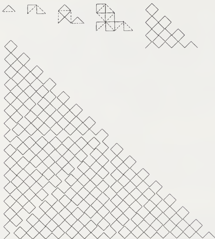
FIGURE 2.10: Triangle sweep with D = 1.944 . For the first few generations we also show the previous generation as dashed lines. Each of the generations shown is magnified so that the structure of the curve becomes apparent.
