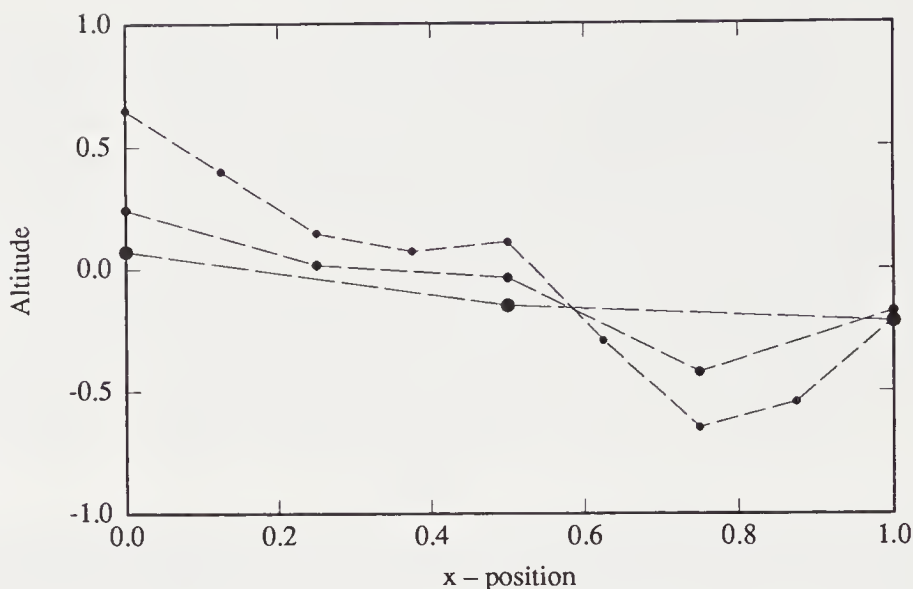
FIGURE 9.9: The process of successive random additions. The lines connect points of the same generation. The three largest circles represent the first random additions to three altitudes that initially were zero. The five next largest circles are obtained by interpolation of the first three values at the midpoints, and then adding smaller random increments to all five points. The next generation produces the values at nine points, marked with the smallest dots.
