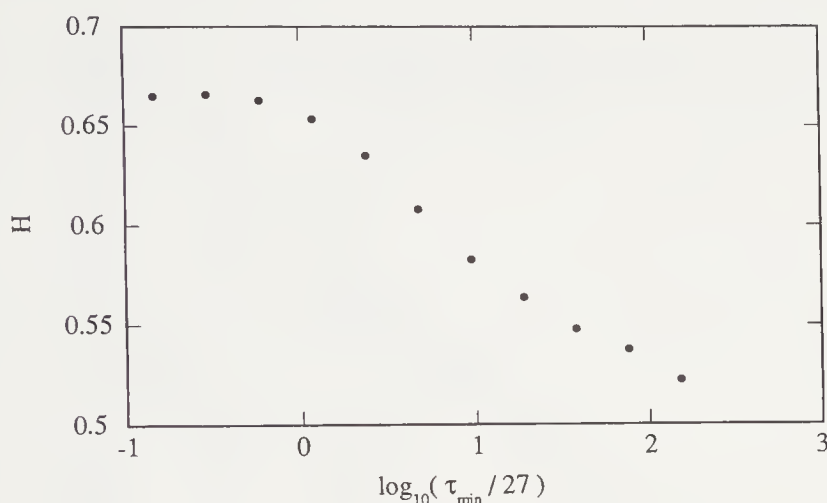
FIGURE 8.9: The apparent Hurst exponent H as a function of the minimum lag \tau_{\min} used in fitting a trend line to the R/S versus \tau data in figure 8.9, for a sequence of 100,000 dependent variables generated by the biased Hurst process.
