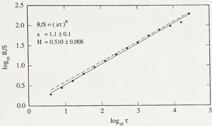
FIGURE 9.7: R/S as a function of the lag \tau for a normalized independent Gaussian variable \xi . The dotted line is the asymptotic theoretical expectation R/S = \sqrt{\pi\tau/2} . The line is the fitted curve R/S = (a\tau)^H with H = 0.510 \pm 0.008 and a = 1.1 \pm 0.1 .
