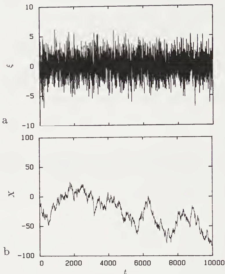
FIGURE 9.3: A sequence of independent Gaussian random variables with zero mean and unit variance — ‘observed’ at every fourth time step, i.e., at intervals of length 4\tau . (a) The independent random steps of the ‘particle.’ (b) The position of the particle. The time is in units of the ‘atomistic’ time \tau between steps.
