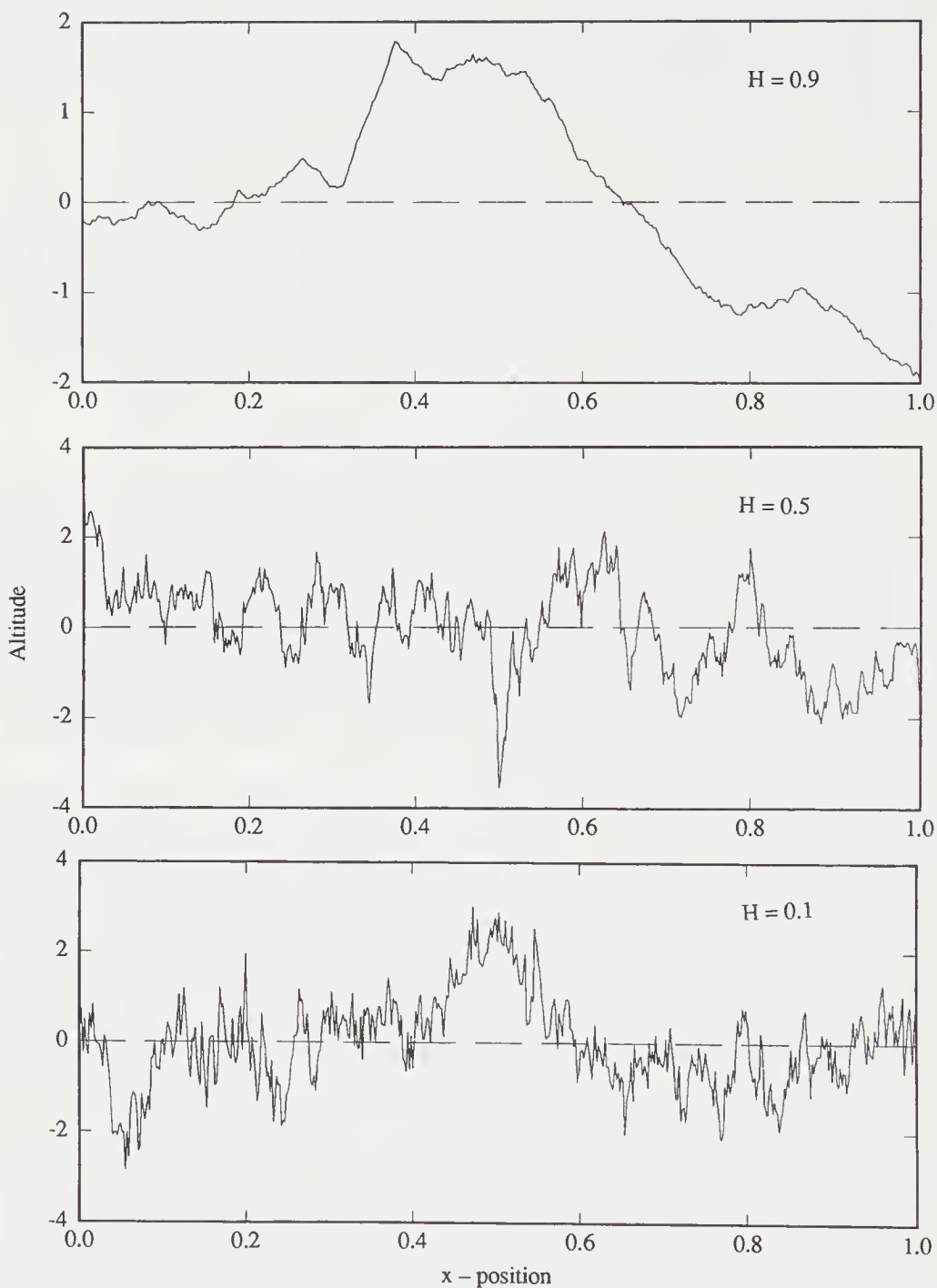
FIGURE 9.10: Fractional Brownian curves generated using Voss's successive random addition algorithm with different values for the Hurst exponent H . The fractal dimension of the curves is D = 2 - H . The curves have been calculated with a resolution of 1/2048 .
