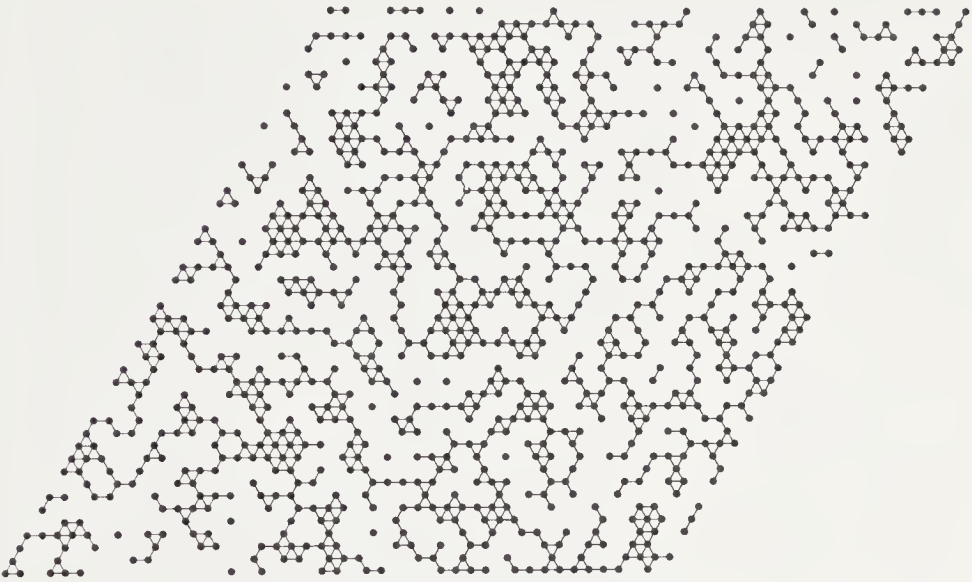
FIGURE 7.6: Site percolation clusters on the triangular lattice at the threshold p_c = 1/2 .
