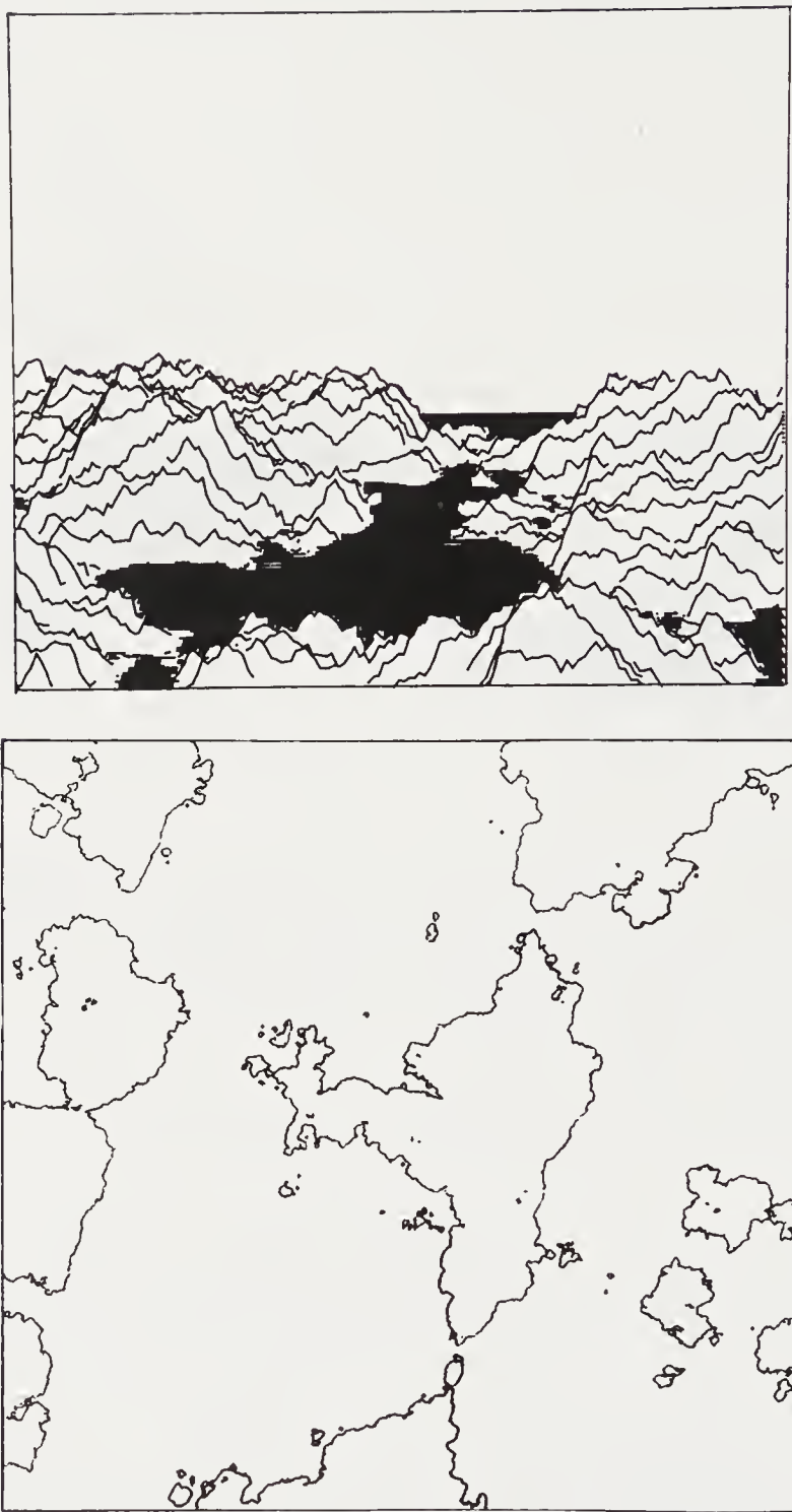
FIGURE 13.9: Fractal landscape with coastline map. \alpha = 0.8 , \beta = 2.0 . Coastline fractal dimension D = 1.15 .
