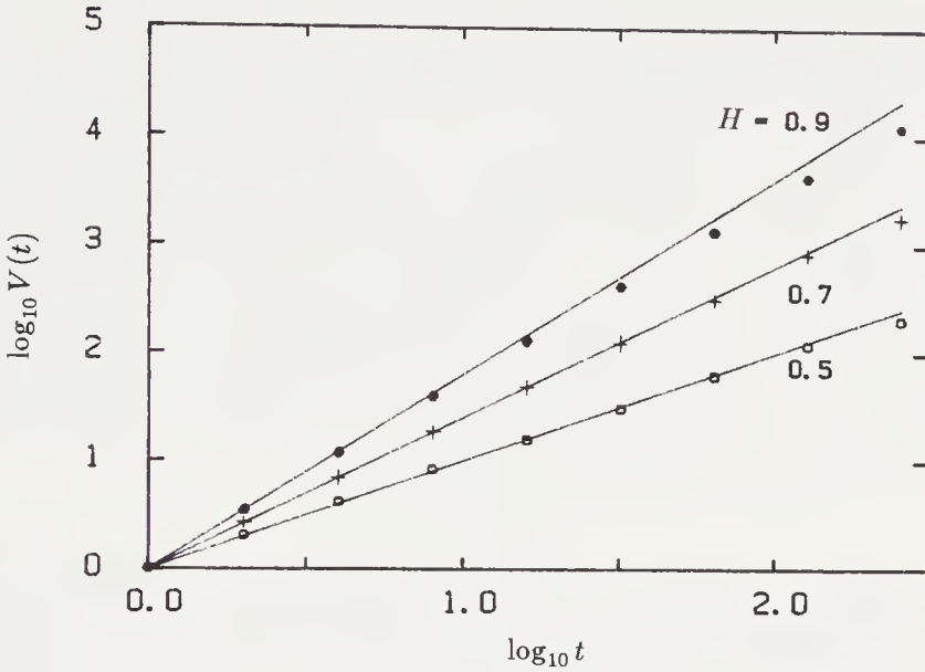
FIGURE 9.6: The correlation of increments for fractal Brownian function V(t) evaluated with M = 700 , n = 8 and with B_H(0) = 0 . The lines correspond to V(t) = |t|^{2H} , with H = 0.5, 0.7, 0.9 .
