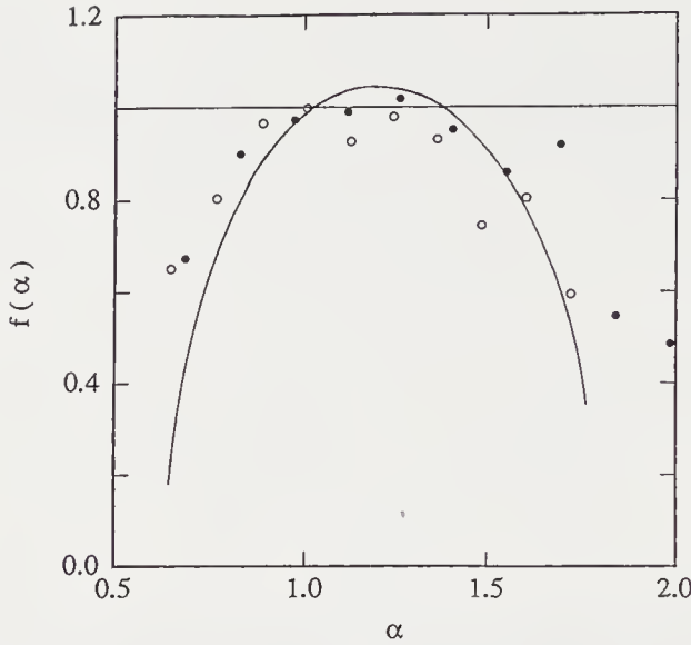
FIGURE 6.17: The f(\alpha) curve for the fractal new-growth measure describing the dynamics of viscous fingering in porous models. Filled and open circles correspond to structures having R_g/\delta \sim 170 and 80 pixels, respectively. The curve is the f(\alpha) obtained from \tau(q) (Måløy et al., 1987b).
