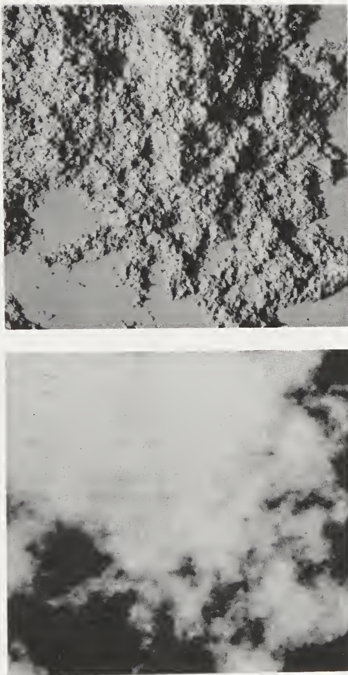
FIGURE 13.13: Fractal landscape with H = 0.7 . The top figure is the landscape shown in figure 13.11 seen from above. The bottom figure renders this landscape as 'clouds.' The altitudes below sea level (see figure 13.12) are black. The gray scale used is proportional to the logarithm of the altitude above sea level. For a color version of the cloud see the insert following the Contents (Boger et al., 1987).
