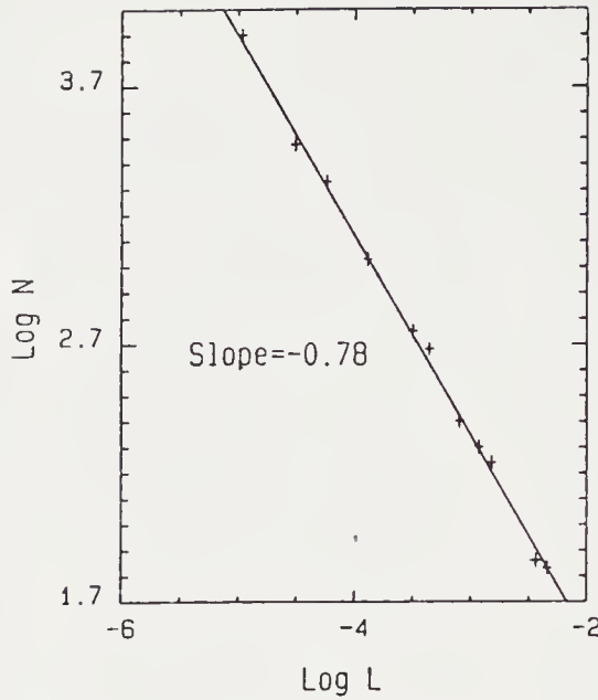
FIGURE 14.10: The number N(L) of geometric features of size L per unit length versus the size L (cm) for Coconino sandstone (Katz and Thompson, 1985).
