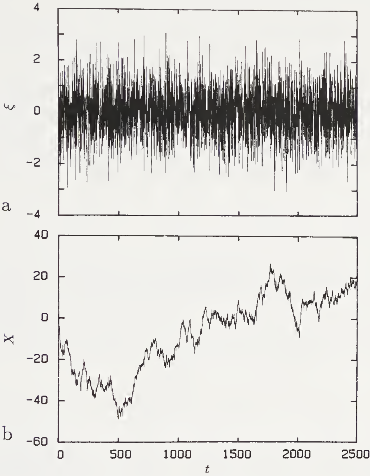
FIGURE 9.1: A sequence of independent Gaussian random variables with zero mean and unit variance. (a) The independent random steps of the ‘particle.’ (b) The position of the particle. The time is in units of the ‘atomistic’ time \tau between steps.
