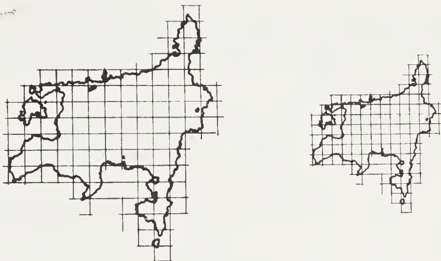
FIGURE 12.1: Two similar islands measured with area-dependent yardsticks.
