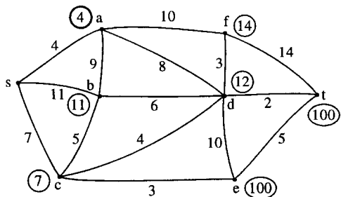
Figure 19.20 Stage 2 of solving the shortest path problem.
