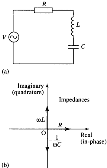
Figure 10.13 (a) The circuit for Example 10.13. (b) The impedances of the circuit elements shown on an Argand diagram. As the elements are in series, the resultant is found by taking the sum of the impedances of the components.
