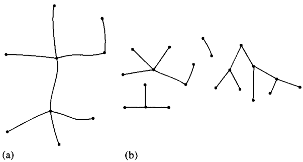
Figure 19.13 (a) A tree is a connected graph with no cycles. (b) A forest has no cycles, but may or may not be connected.
