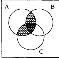
(b) A \cap B (diagonal lines) A \cap C (diagonal lines) (A \cap B) \cup (A \cap C) (diagonal lines)
