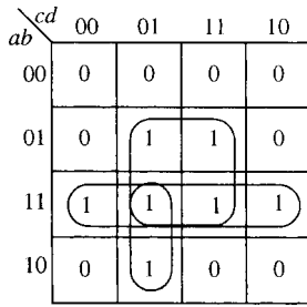
Figure 4.12 A four-variable Karnaugh map representing ab\bar{c} + \bar{a}bd + abcd + ab\bar{c}d + abc .
