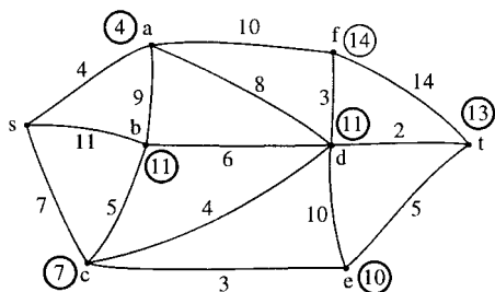
Figure 19.25 The solution to the shortest path problem. Vertex t now has a permanent label, showing that the length of the shortest path from s to t is 13. By working backwards from t to s we find that the actual path must be scdt.
