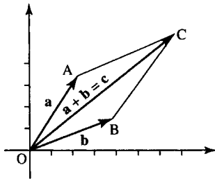
Figure 9.8 The resultant or vector sum of a and b .
