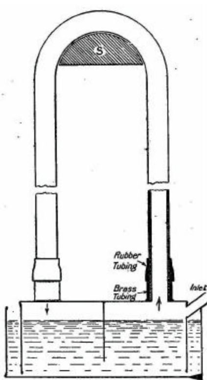
FIG. 191.—Vertical section of condenser.
