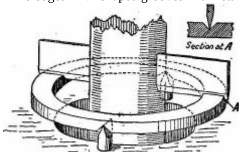
FIG. 172.—Knife-edge universal-motion gimbal.
