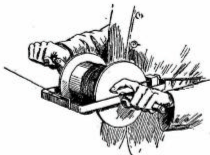
FIG. 125.—String winder in operation.
