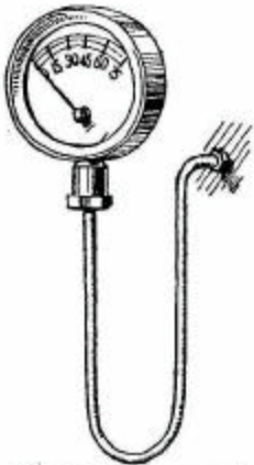
FIG. 90.—Steam gauge and siphon.
