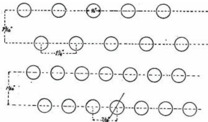
FIG. 88.—Two arrangements for tube holes in multitubular boiler.
