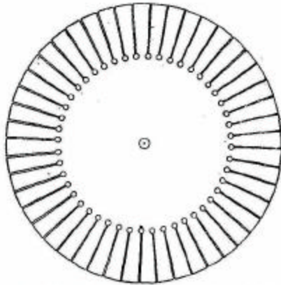
FIG. 75.—Wheel of steam top, ready for blades to be bent. A hole is drilled at the inner end of every slit to make bending easier.
