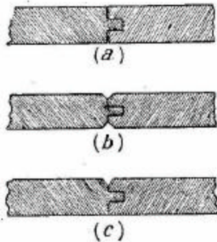
FIG. 17.—Types of match boarding: (a) square joint; (b) double-V; (c) single-V.
