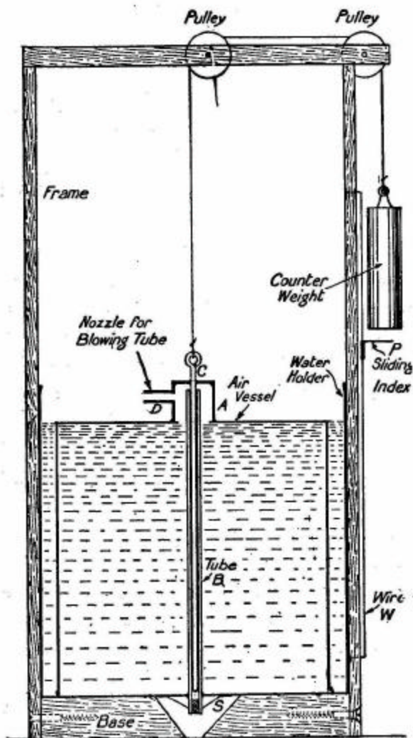
FIG. 166. -- Section of lung-capacity tester.
