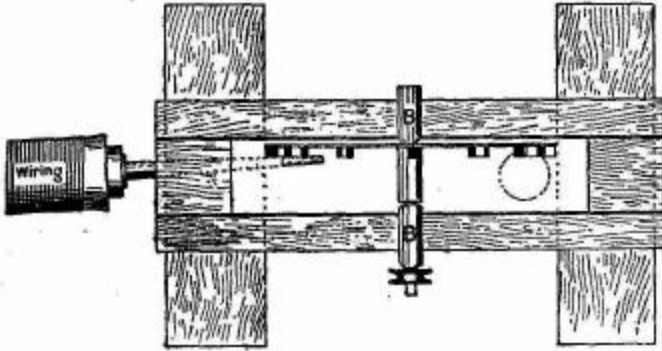
FIG. 107.—Plan of water turbine, showing arrangement of nozzle.
