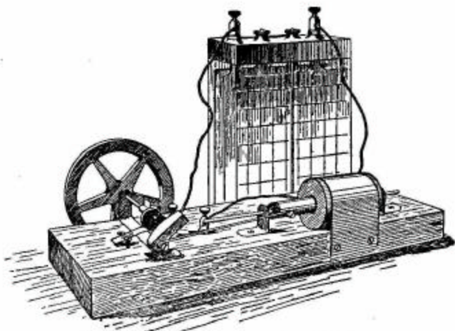
FIG. 37.—Electric reciprocating engine and battery.
