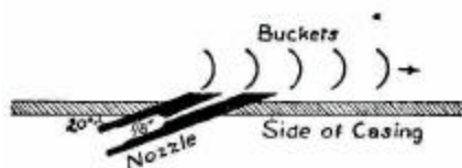
FIG. 72.—Nozzle of turbine, showing its position relatively to buckets.
