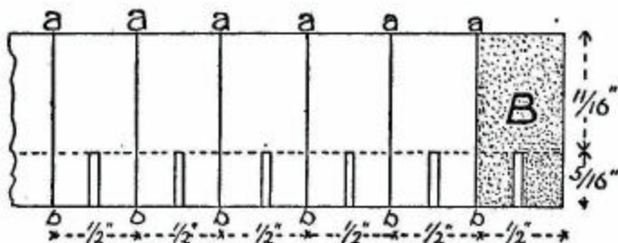
FIG. 71.—Plate marked out for turbine wheel blades. B is blade as it appears before being curved.
