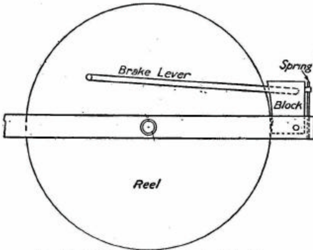
FIG. 124.--End view of string winder, showing brake and lever.
