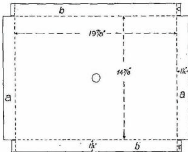
FIG. 12.—Showing how the tray for sink is marked out.
