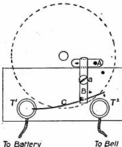
FIG. 39.—Plan of release gear of electric alarm, as attached to clock.
