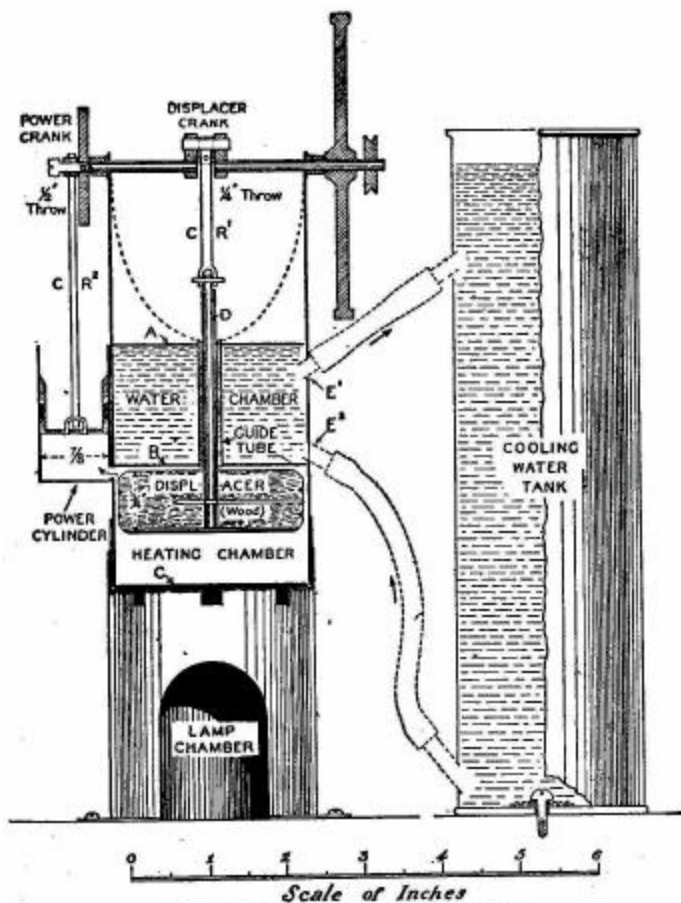
FIG. 97.—Vertical section of hot-air engine.
