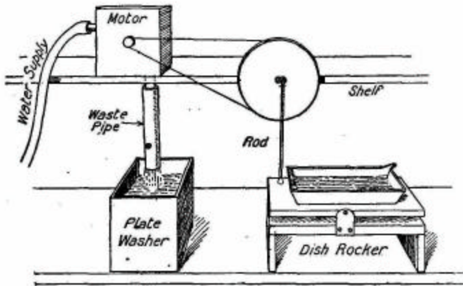
FIG. 108.—Water motor working a photographic dish-rocker.
