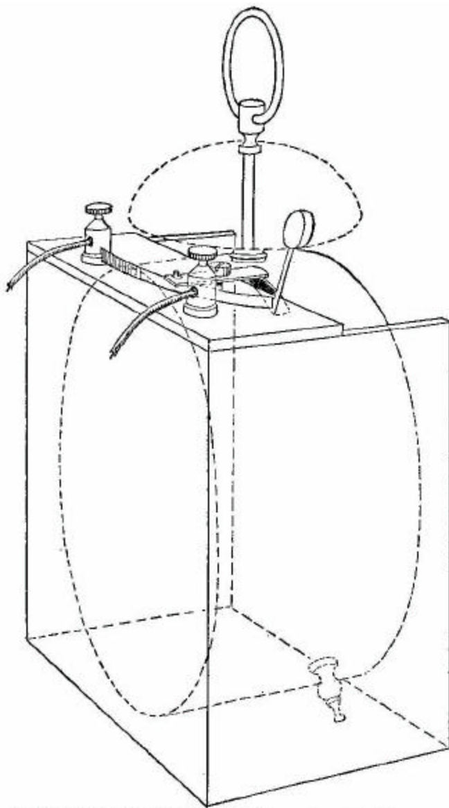
FIG. 40.—Electric alarm releaser, as attached to separate wooden clock casing.
