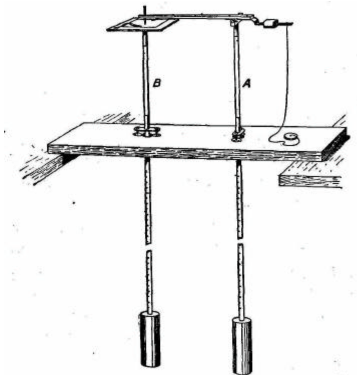
FIG. 168.—Simple Rectilinear Harmonograph.
