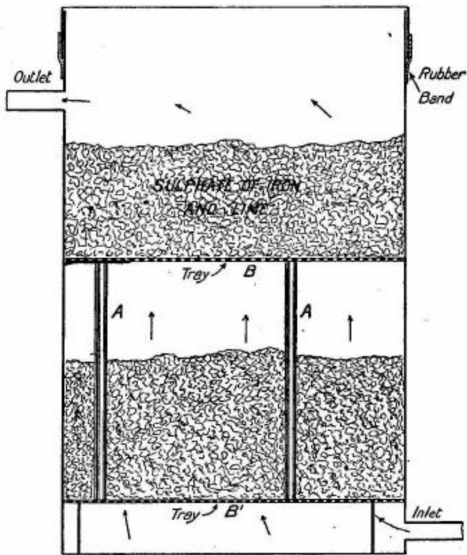
FIG. 193.--Vertical section of purifier.
