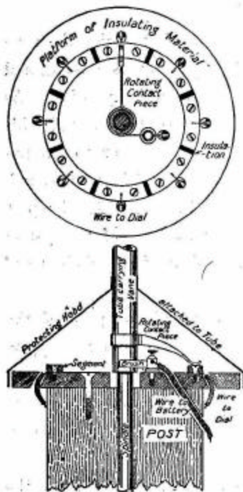
FIG. 158.—Plan and elevation of electric contact on vane post.
