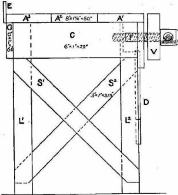
FIG. 5.—End elevation of joiner's bench.
