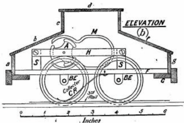
FIG. 47.—Plan and elevation of electric locomotive.
