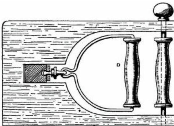
FIG. 163.—Grips of strength tester.
