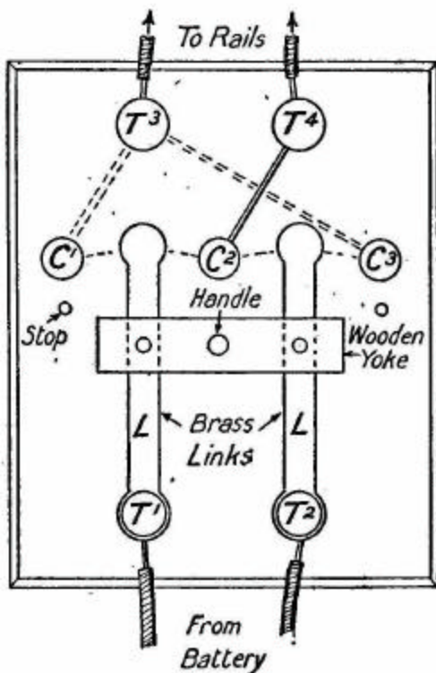
FIG. 48.—Reversing switch.
