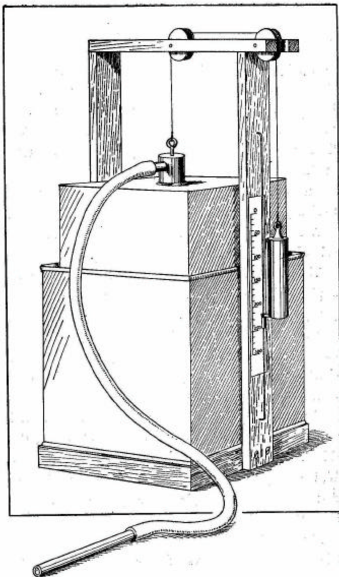
FIG. 166.—Perspective view of lung-capacity tester.
