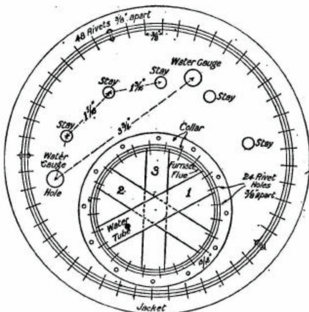
FIG. 83.—End of horizontal boiler, showing position of holes for stays and fittings.
