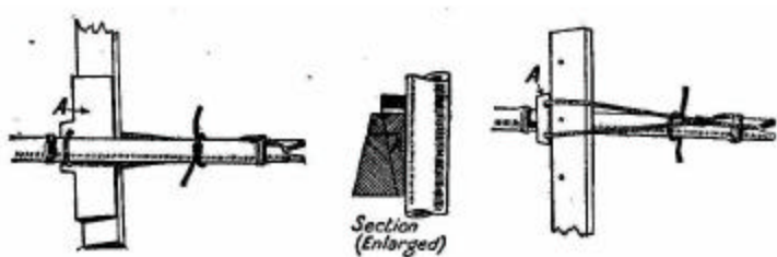
FIG. 115. -- Details of stretcher attachment for diamond-shaped box kites.
