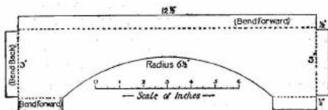
FIG. 55.—Standards of bedplate.
