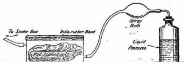
FIG. 150.—Smoke-making apparatus.
