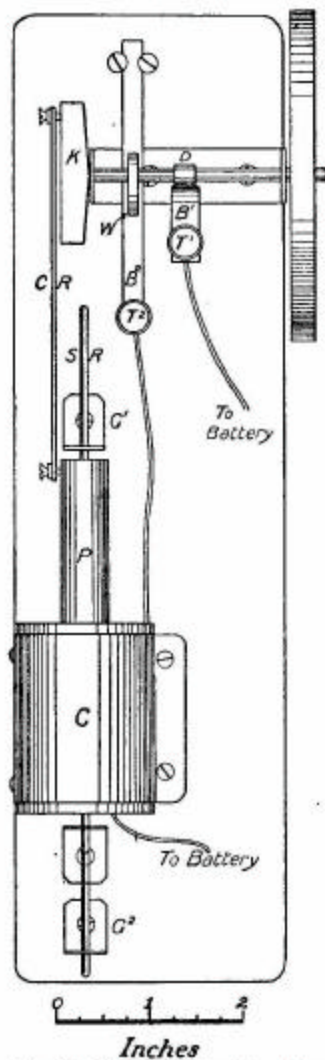
FIG. 38.—Plan of electric reciprocating engine.
