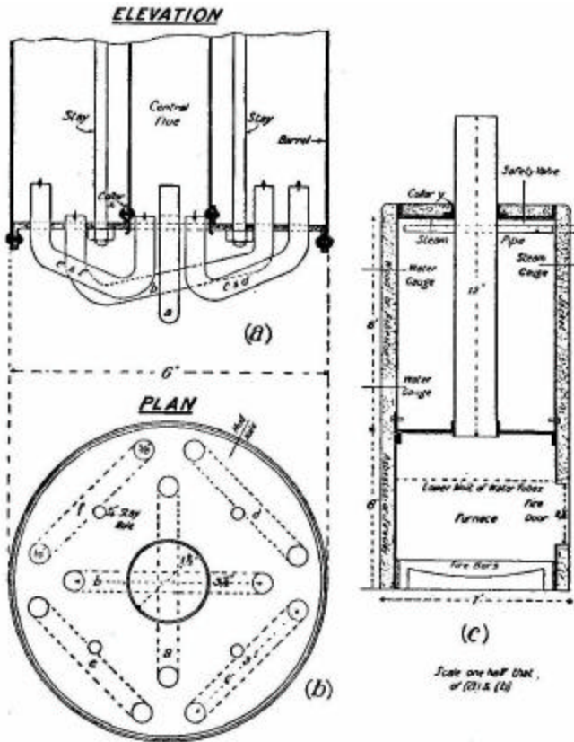
FIG. 80.—Details of vertical boiler.
