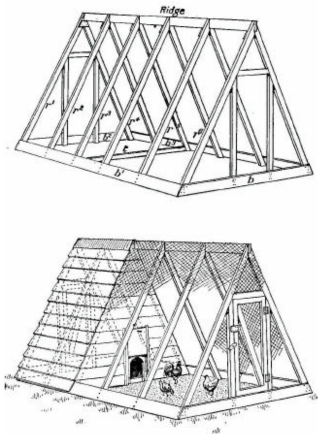
FIG. 13.—Frame for poultry house and run (above). Completed house and run (below).
