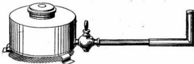
FIG. 104.—Spirit lamp for hot-air engine, with regulating tap.
