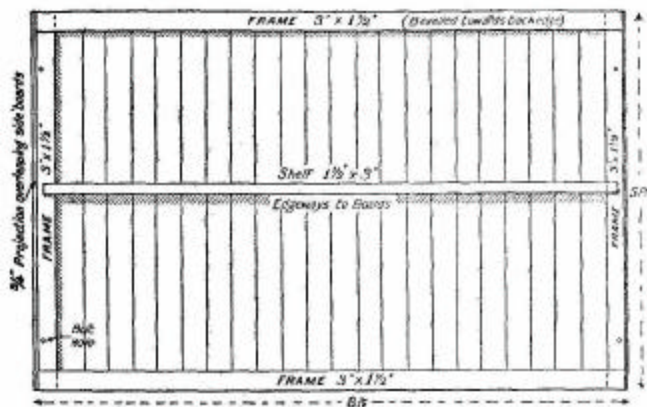
FIG. 20.—Back of cycle shed.
