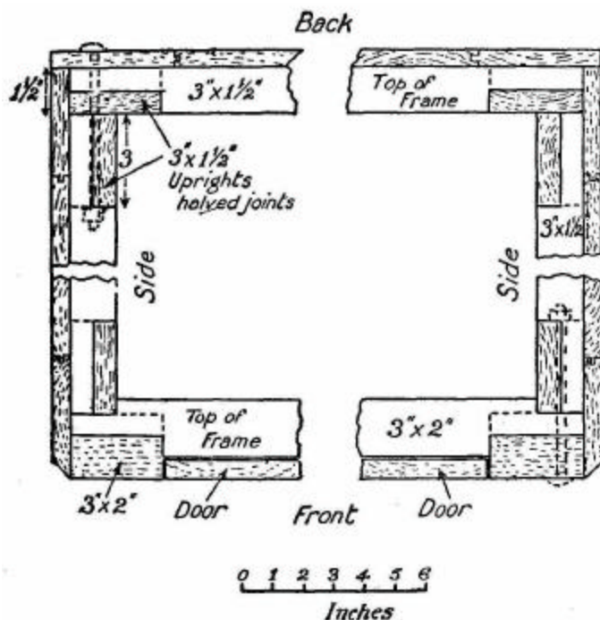
FIG. 16.—Plan of corner joints of cycle shed.
