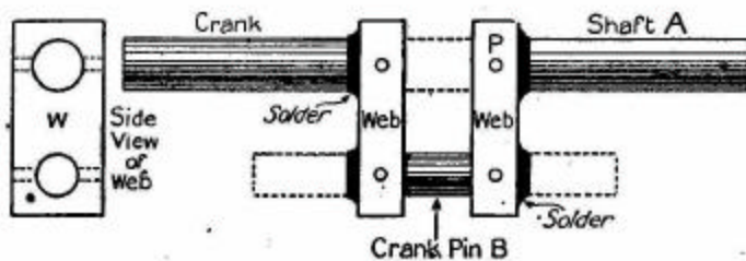
FIG. 101.—Details of built-up crank.
