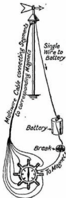
FIG. 161.—General arrangement of electric wind recorder.
