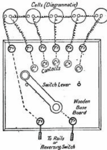
FIG. 49.—Multiple battery switch.
