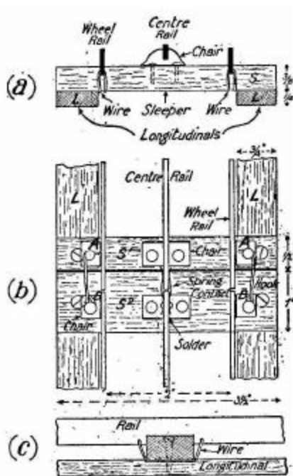
FIG. 42.—Details of rails for electric track.
