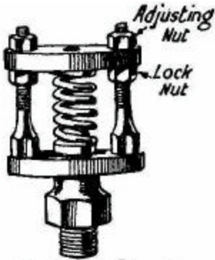
FIG. 89.—Safety valve.
