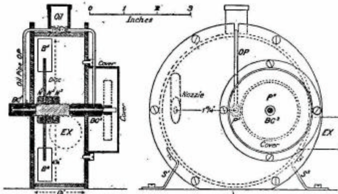
FIG. 70.—Vertical section of steam turbine with formed blades (left); outside view of turbine, gear side (right).
