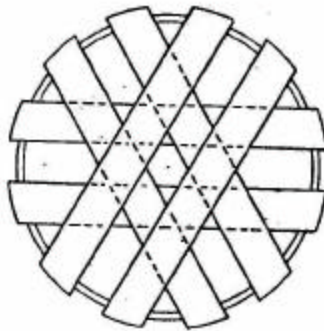
FIG. 84.—Doubled cross tubes in horizontal boiler flue.
