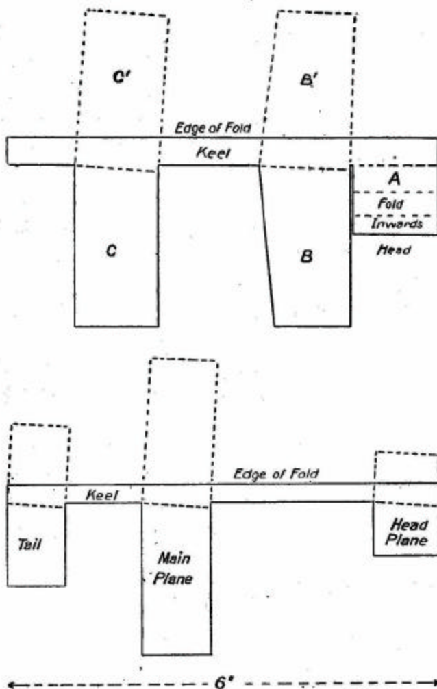
FIG. 128.—Details of paper gliders: Model "B" above, Model "C" below.
