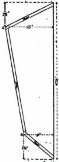
FIG. 120.—Wing for box kite.
