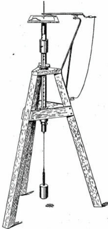
FIG. 170.—Benham's miniature Twin Elliptic Pendulum Harmonograph.
