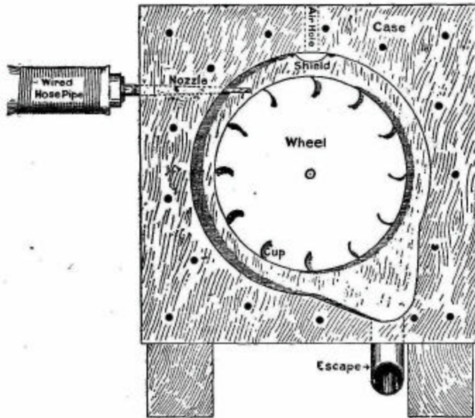
FIG. 106.—Water turbine, with pulley side of casing removed.
