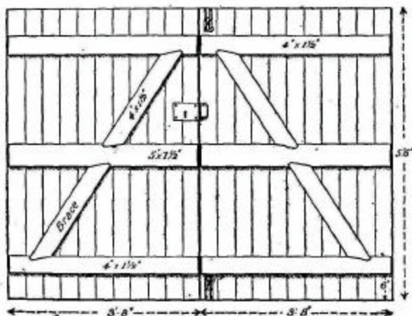
FIG. 22.—Doors of shed.
