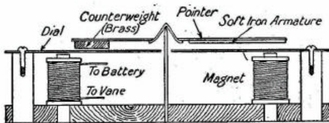
FIG. 159. -- Magnetic recording dial.
