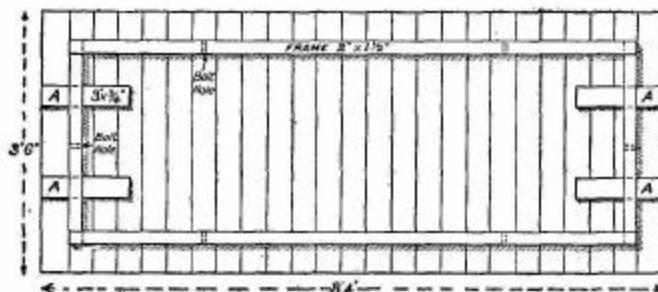
FIG. 24.—Top of cycle shed.
