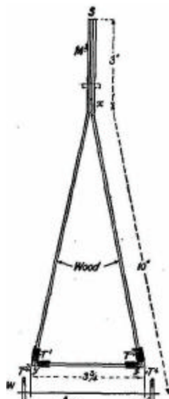
FIG. 131.—Front elevation of chassis.
