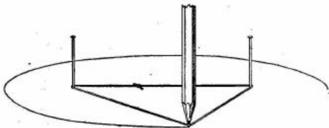
FIG. 180.—Showing how to draw an ellipse.
