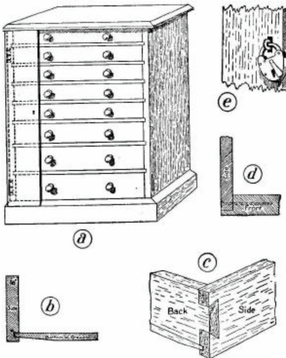
FIG. 30.--Large cabinet (a), details of drawer joints (b, c, d), and padlock fastening (e).
