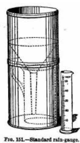
FIG. 151. -- Standard rain-gauge.
