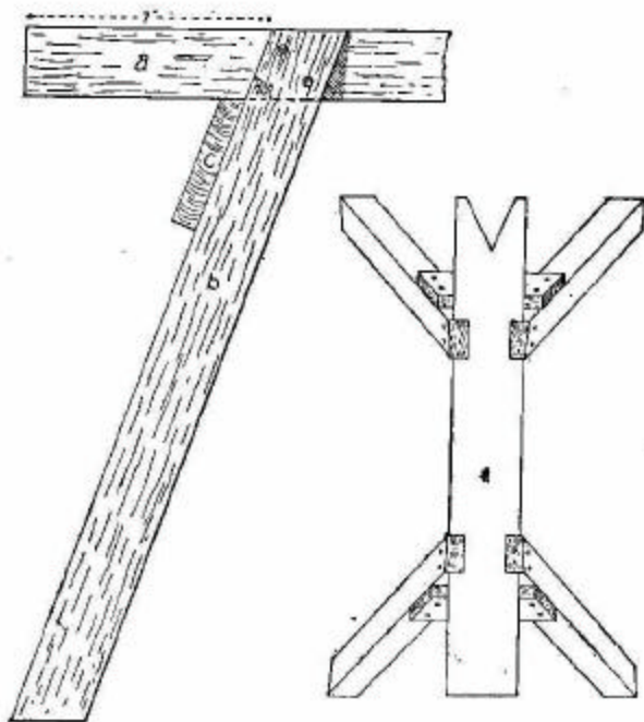
FIG. 1.—Leg of sawing trestle (left). Trestle seen from above (right).
