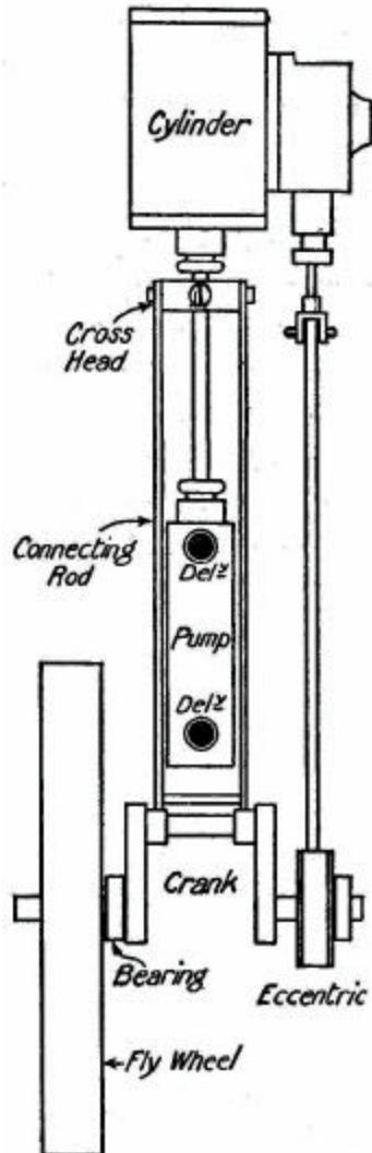
FIG. 114.—Plan of steam pump with fly wheel.
