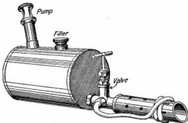
FIG. 94.—Benzoline lamp for model central-flue boiler.
