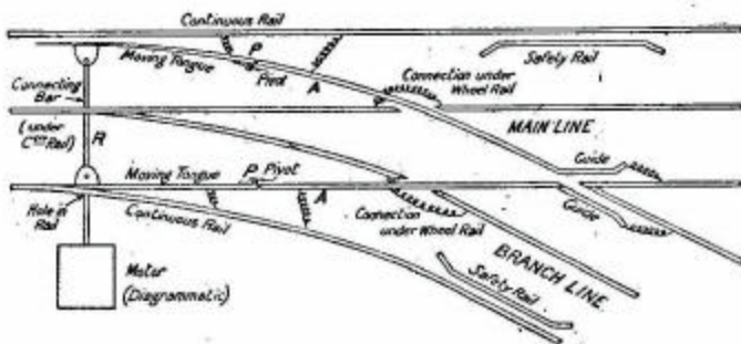
FIG. 45.--Points for electric railway.
