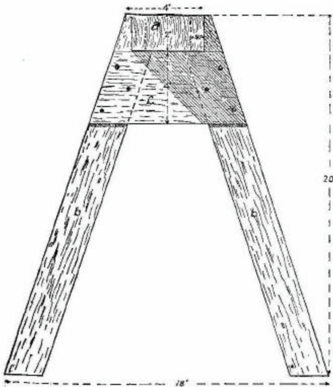
FIG. 3.—End elevation of sawing trestle.
