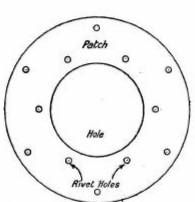
FIG. 85.--Showing how to mark out strengthening patch round steam dome hole.
