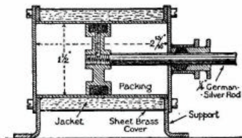
FIG. 57.--Vertical section of cylinder.
