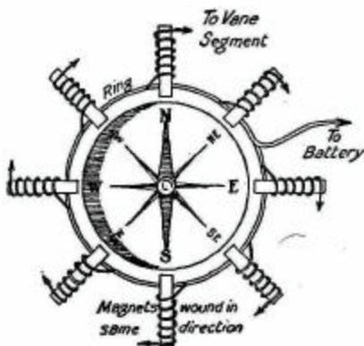
FIG. 160.—Another type of electric dial with compass needle for pointer.
