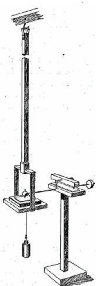
FIG. 169.—Goold's Twin Elliptic Pendulum Harmonograph.
