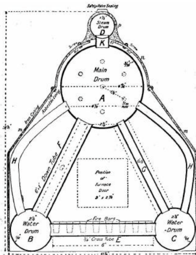
FIG. 86. -- Cross section of multitubular boiler.
