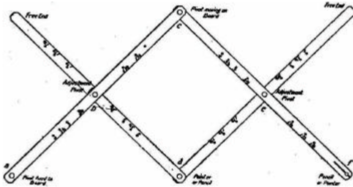
FIG. 186. -- Details of simple pantograph.
