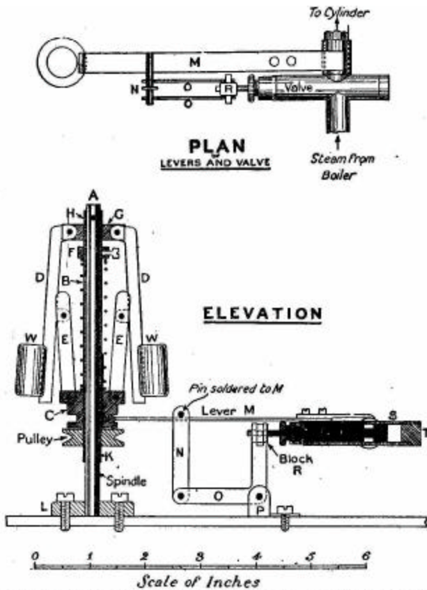
FIG. 66.—Elevation of governor for horizontal engine. Above is plan of valve and rod gear.
