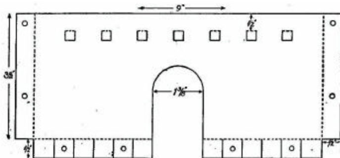
FIG. 103.—Plate for lamp chamber cut out ready for bending.
