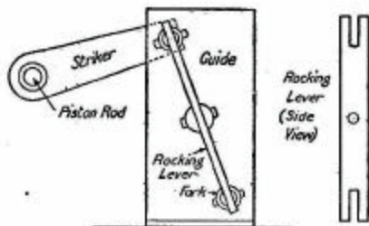
FIG. 113.—End view of striking mechanism of steam pump.
