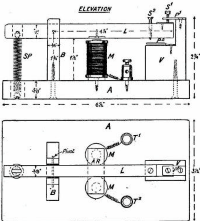
FIG. 35.—Elevation and plan of telegraphic sounder.
