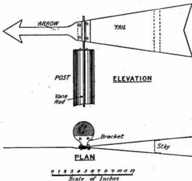
FIG. 156.—Elevation and plan of vane.
