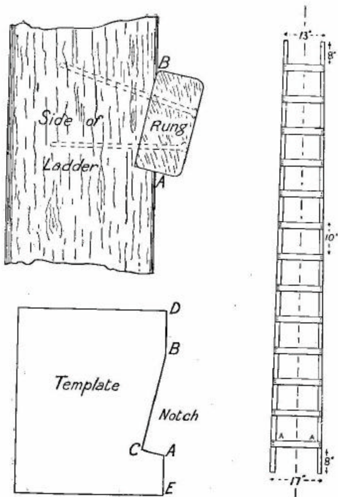
FIG. 10.—House ladder and details of letting in a rung.
