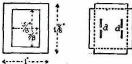
FIG. 63.—Parts of slide valve.
