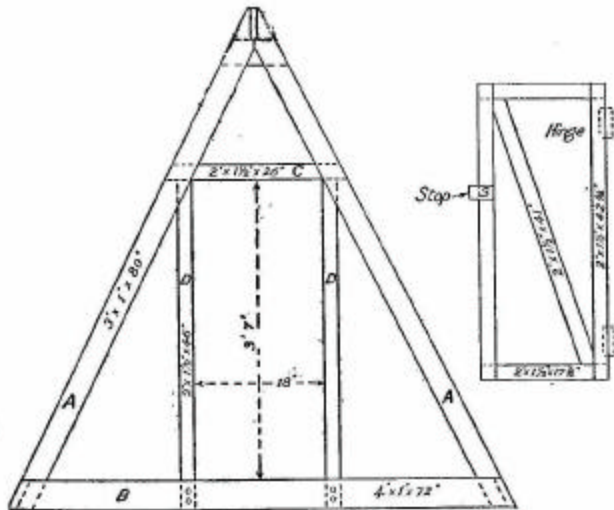
FIG. 14.—On left, elevation of end of run ; on right, door for run.
