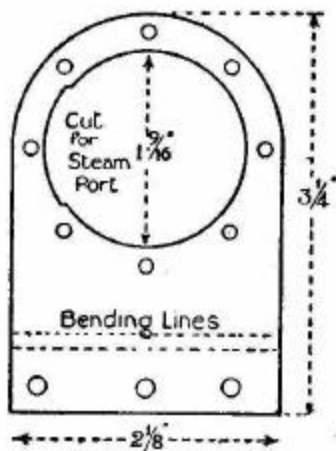
FIG. 56.—Cylinder standard before being bent.
