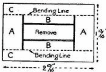
FIG. 60.—Piece for steam ways.
