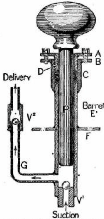
FIG. 109.—Vertical section of force pump.
