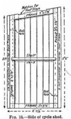
FIG. 18.—Side of cycle shed.
