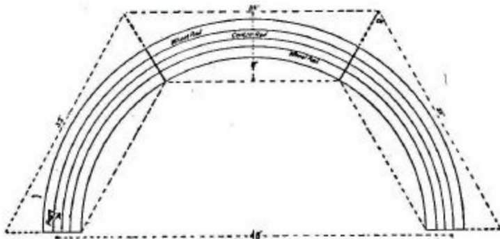
FIG. 44. -- Laying out a curve for electric track.
