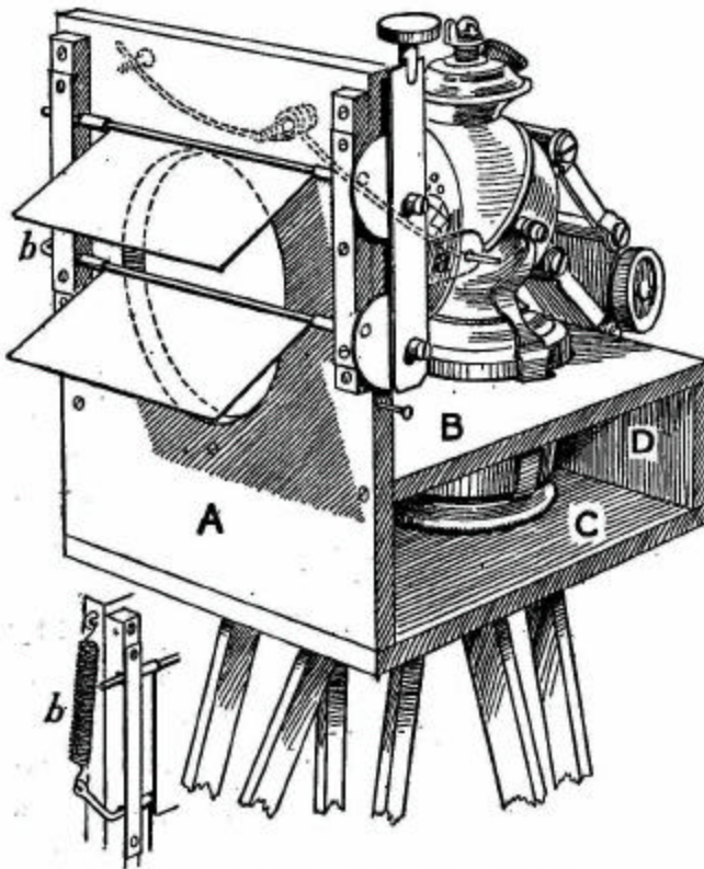
FIG. 189.—Signalling lamp with quick-moving shutter.
