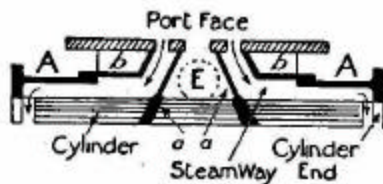
FIG. 61.—Valve plate and steam ways in section.
