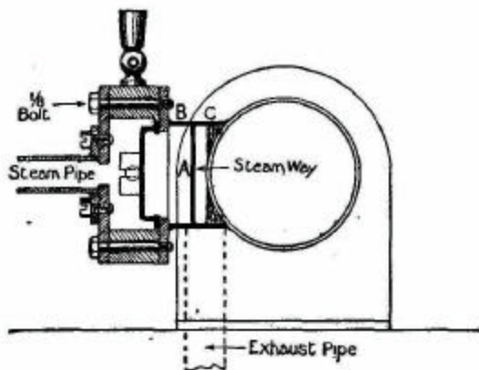
FIG. 62.—Cross section of cylinder and valve chest.
