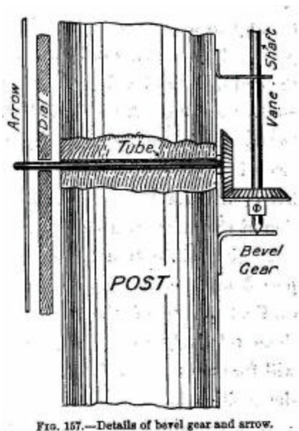
FIG. 157. -- Details of bevel gear and arrow.
