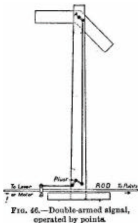
Fig. 46. -- Double-armed signal, operated by points.
