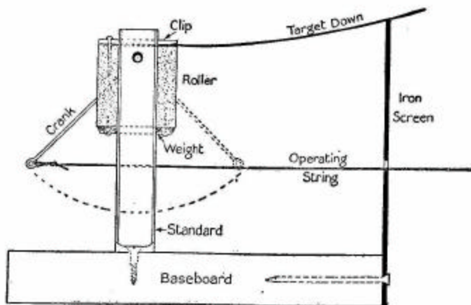
FIG. 26.—Side elevation of disappearing target apparatus.
