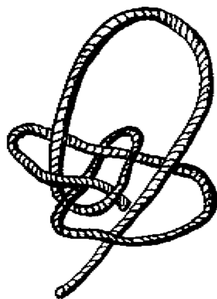
g Running Bowline. For making a running loop in the end of a rope.
