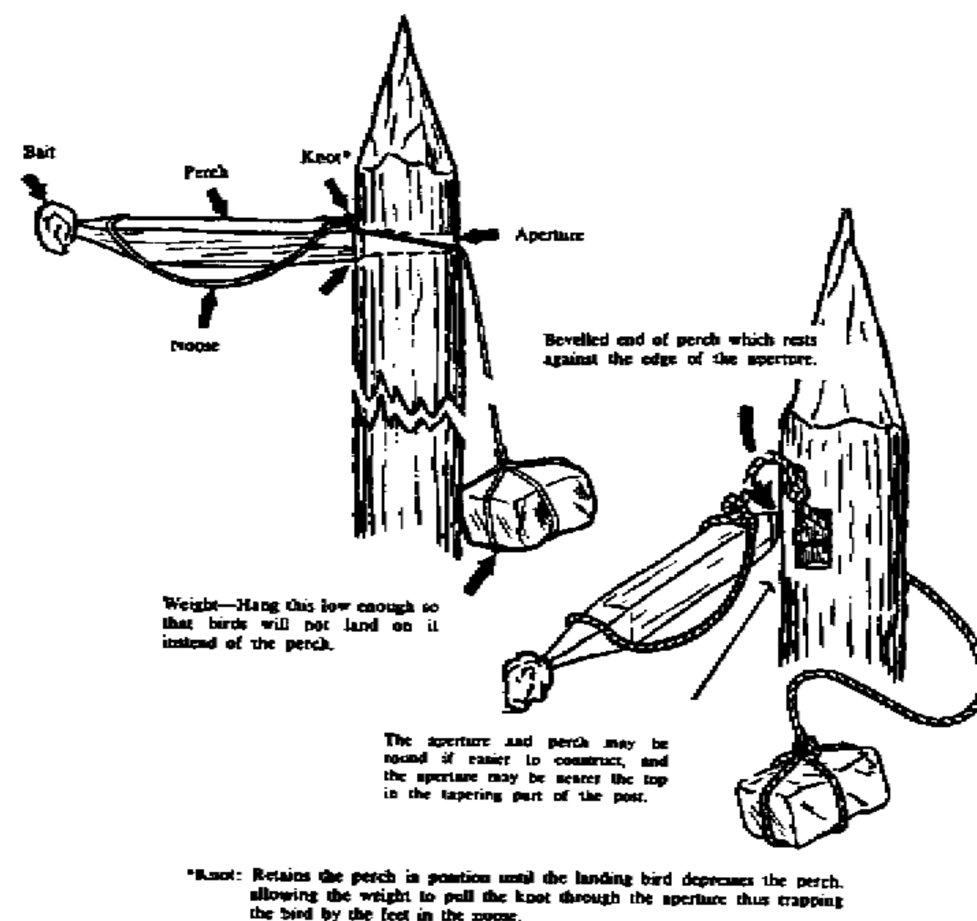
Ojibwa Bird Snare
