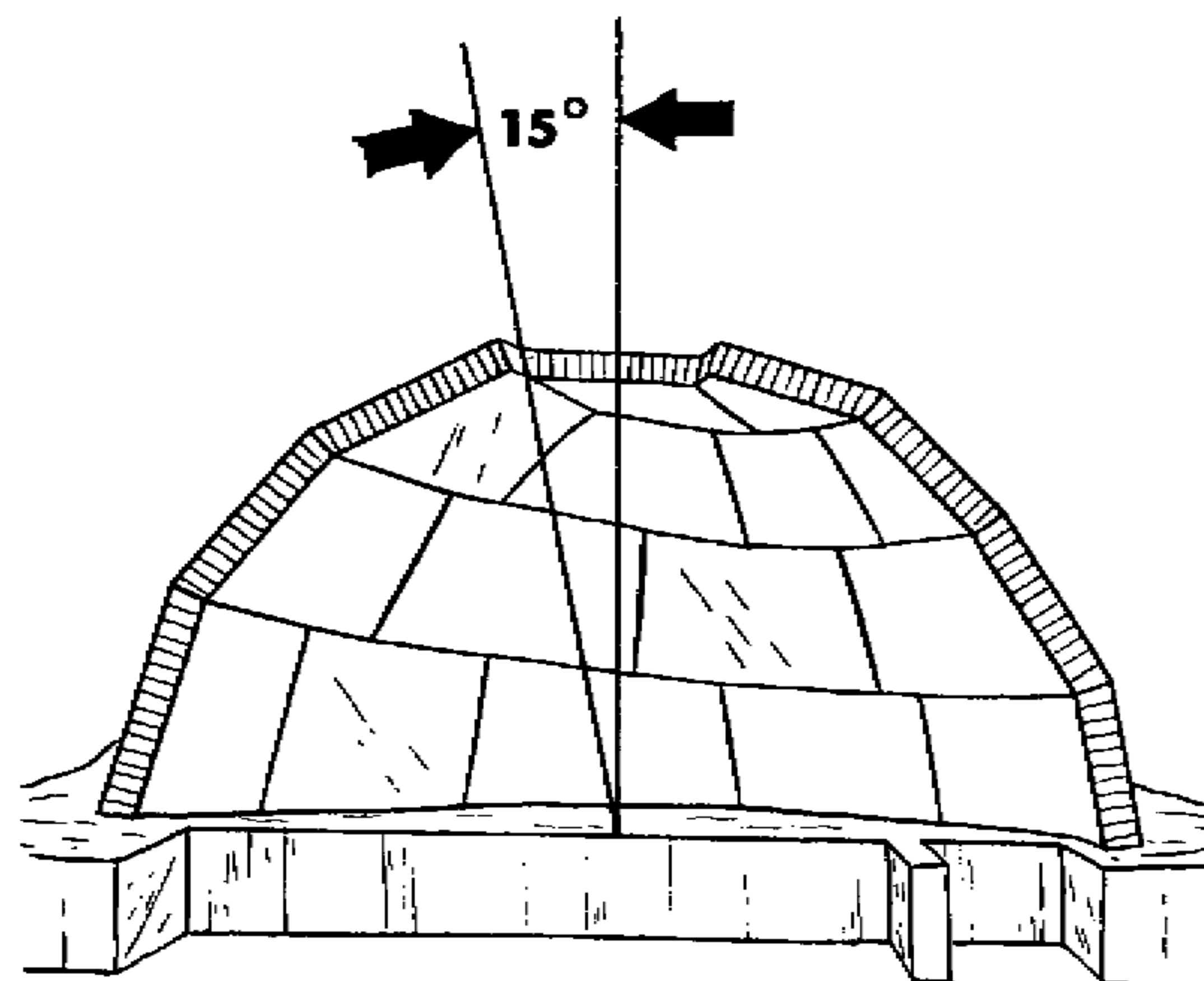
Fitting the Key Block
