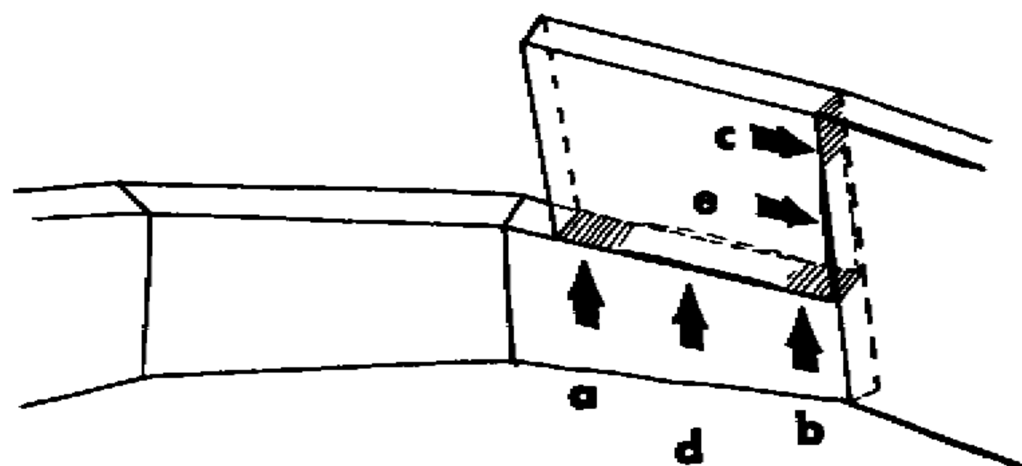
Bearing Surfaces of the Block
